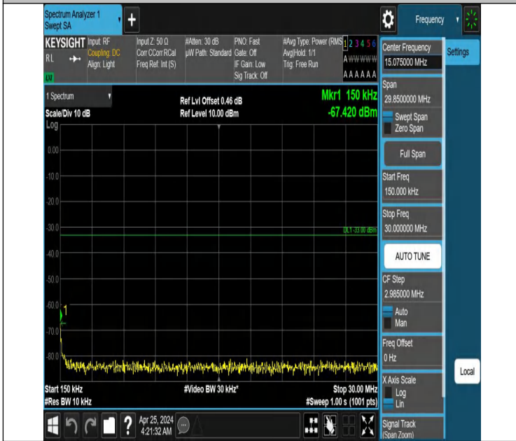
Band66_10MHz_QPSK_132322_1RB#49_0.15~30_0.15~30
