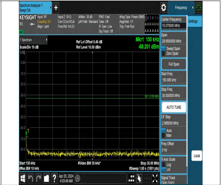
Band66_3MHz_QPSK_132322_1RB#0_0.15~30_0.15~30
