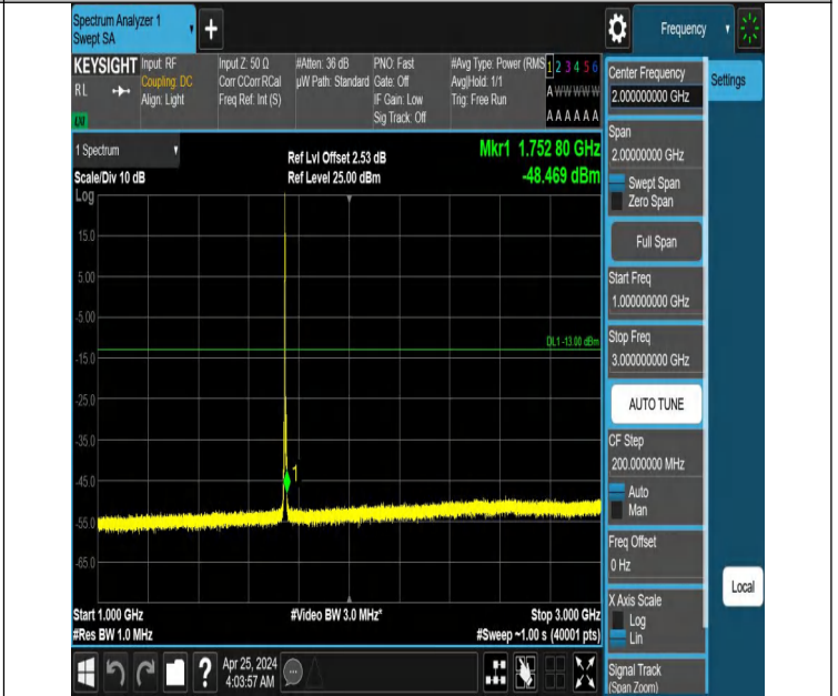
Band66_3MHz_QPSK_132322_1RB#0_1000~3000_1000~3000
