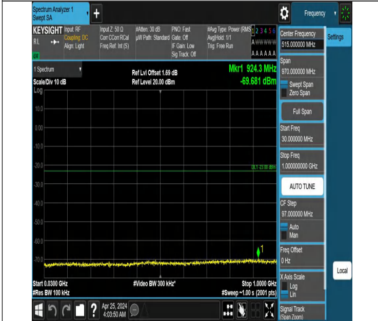
Band66_3MHz_QPSK_132322_1RB#0_30~1000_30~1000
