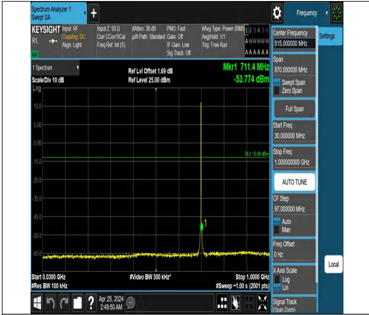
Band12_1.4MHz_QPSK_23095_1RB#0_30~1000_30~1000
