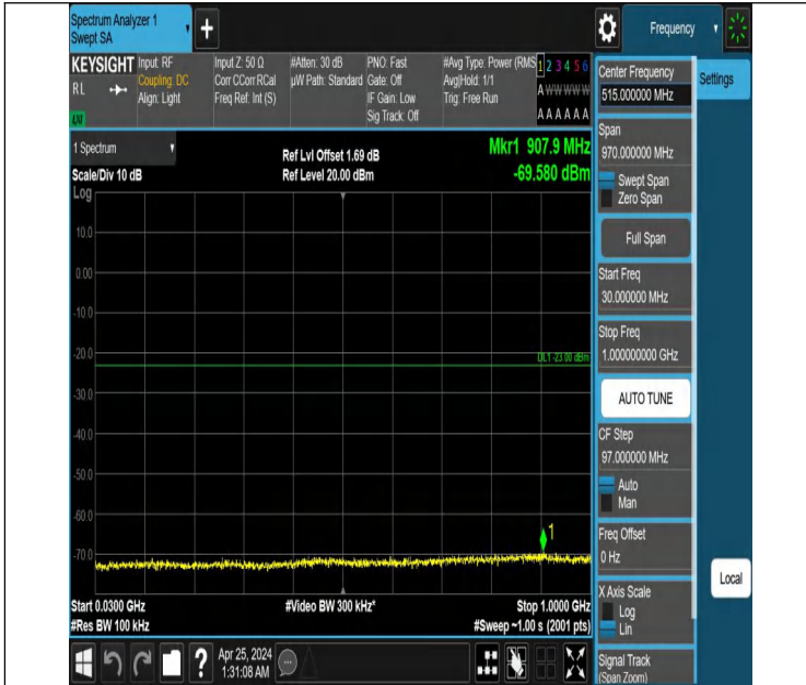
Band4_3MHz_QPSK_20385_1RB#0_30~1000_30~1000
