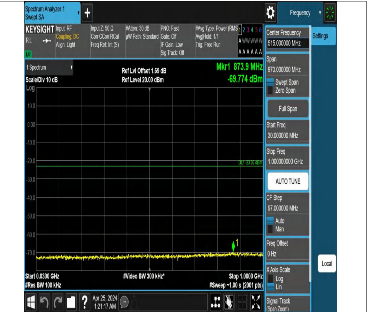
Band4_1.4MHz_QPSK_20175_1RB#5_30~1000_30~1000
