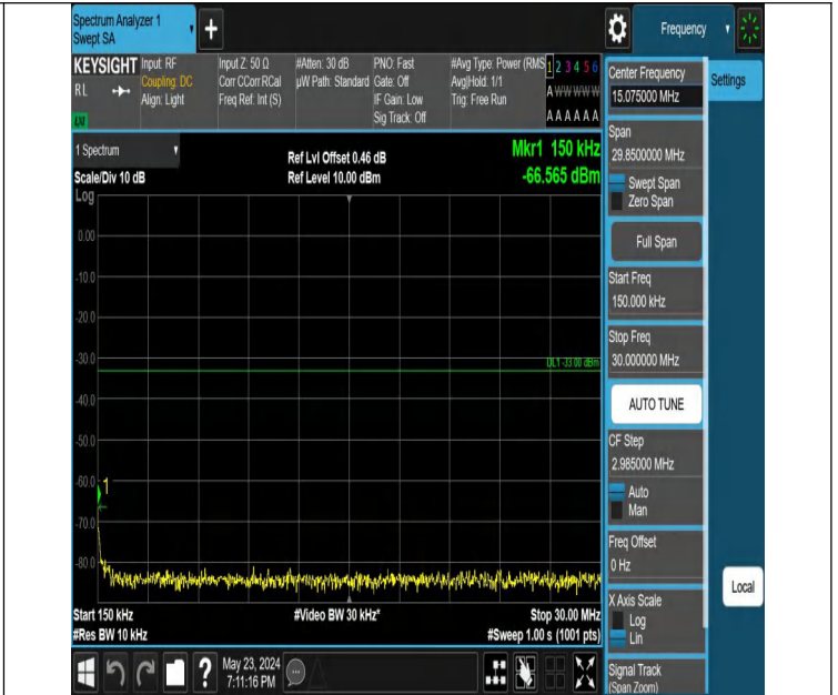
Band66_5MHz_QPSK_131997_1RB#0_0.15~30_0.15~30
