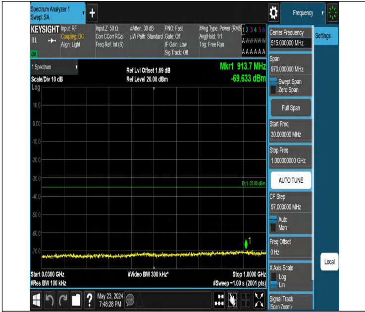
Band7_10MHz_QPSK_21400_1RB#0_30~1000_30~1000
