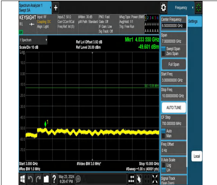
Band5_1.4MHz_QPSK_20407_1RB#0_3000~10000_3000~10000
