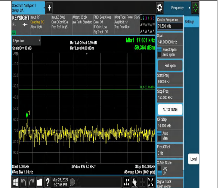
Band5_1.4MHz_QPSK_20525_1RB#5_0.009~0.15_0.009~0.15
