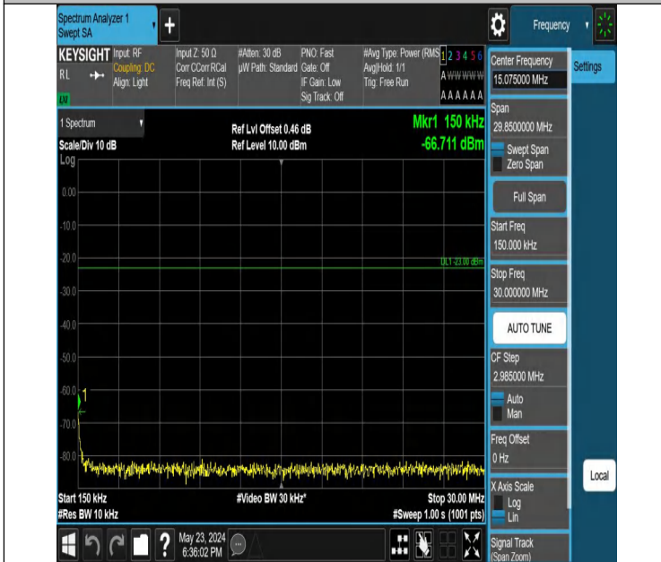
Band5_3MHz_QPSK_20525_1RB#14_0.15~30_0.15~30
