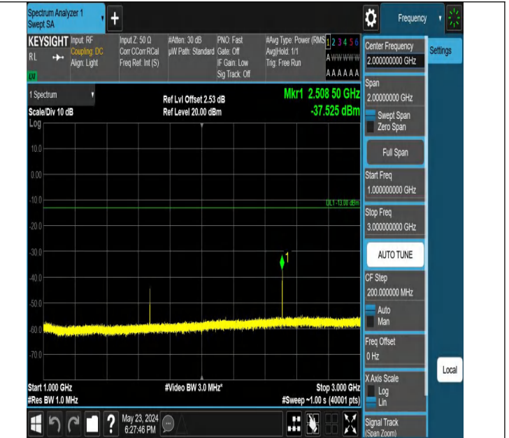
Band5_1.4MHz_QPSK_20525_1RB#0_1000~3000_1000~3000
