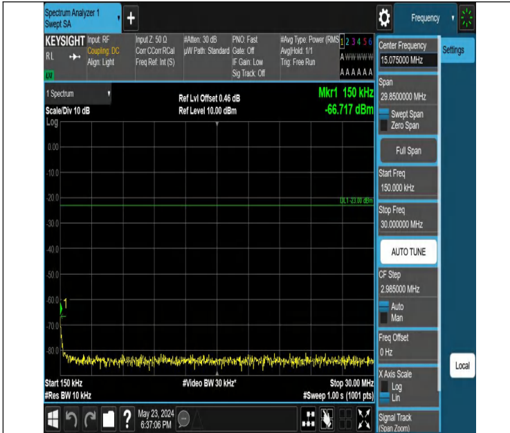
Band5_3MHz_QPSK_20635_1RB#14_0.15~30_0.15~30
