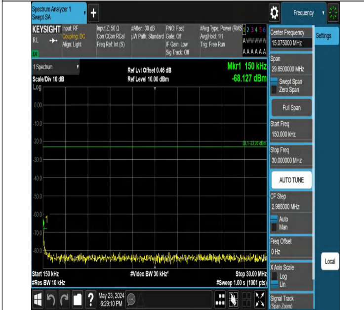
Band5_1.4MHz_QPSK_20643_1RB#5_0.15~30_0.15~30
