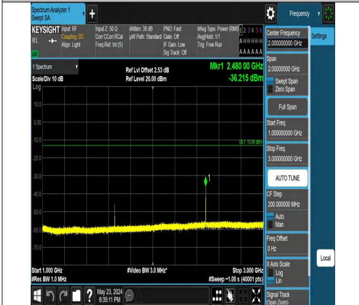
Band5_3MHz_QPSK_20415_1RB#14_1000~3000_1000~3000
