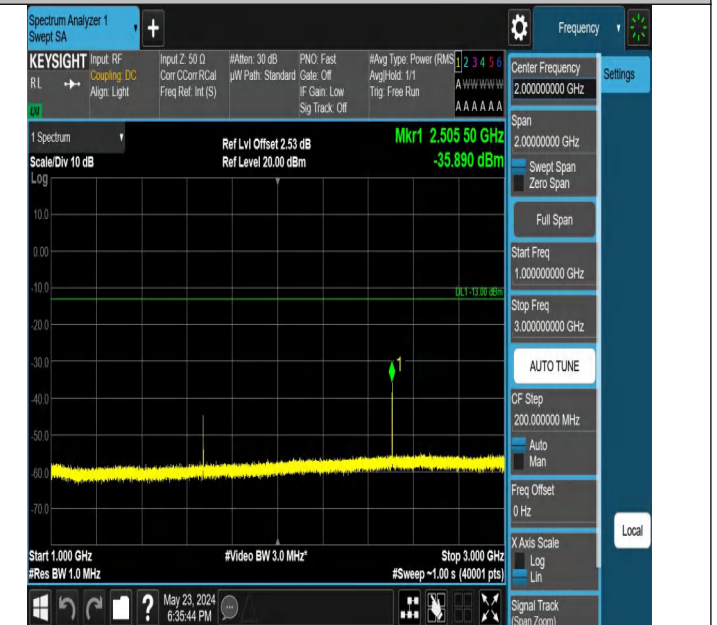
Band5_3MHz_QPSK_20525_1RB#0_1000~3000_1000~3000
