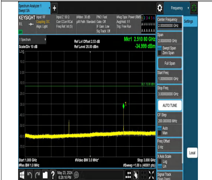
Band5_1.4MHz_QPSK_20525_1RB#5_1000~3000_1000~3000
