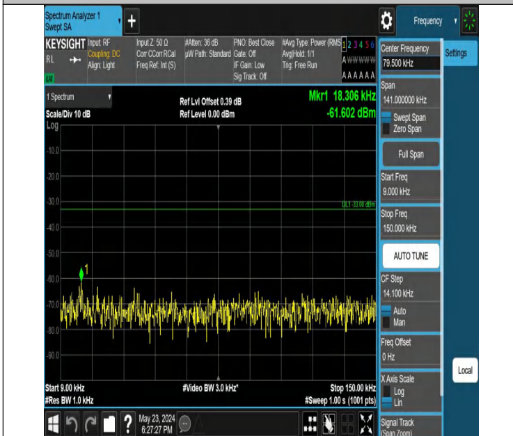
Band5_1.4MHz_QPSK_20525_1RB#0_0.009~0.15_0.009~0.15
