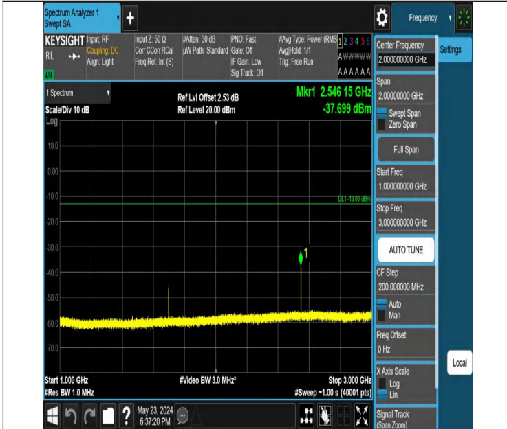
Band5_3MHz_QPSK_20635_1RB#14_1000~3000_1000~3000
