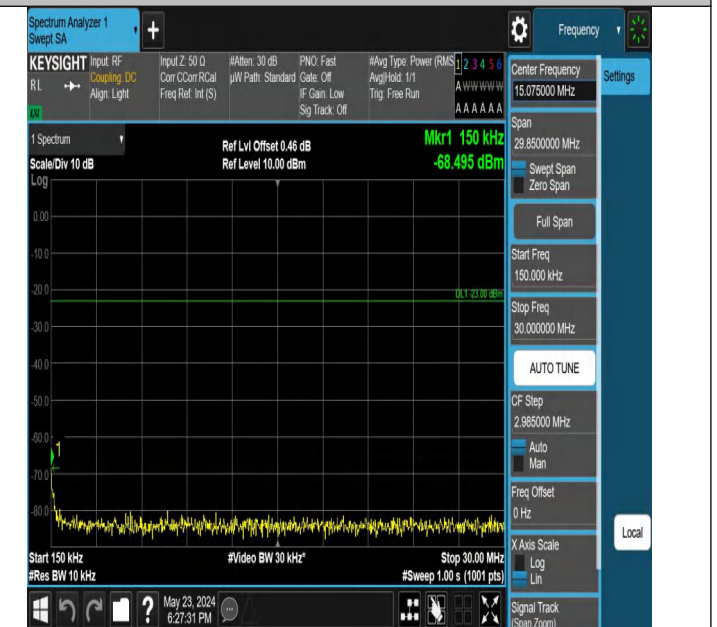
Band5_1.4MHz_QPSK_20525_1RB#0_0.15~30_0.15~30
