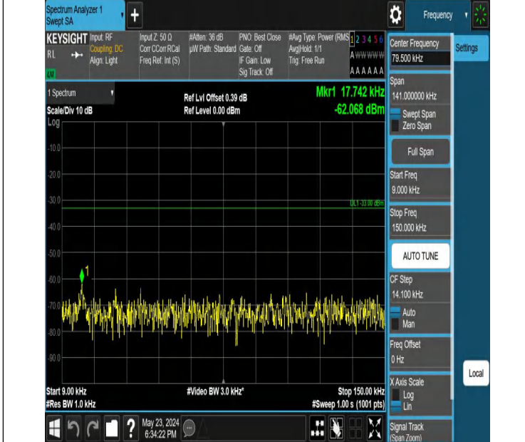
Band5_3MHz_QPSK_20415_1RB#0_0.009~0.15_0.009~0.15
