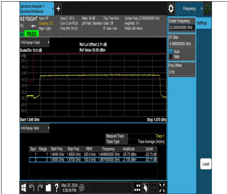
Band2_20MHz_QPSK_18700_100RB#0
