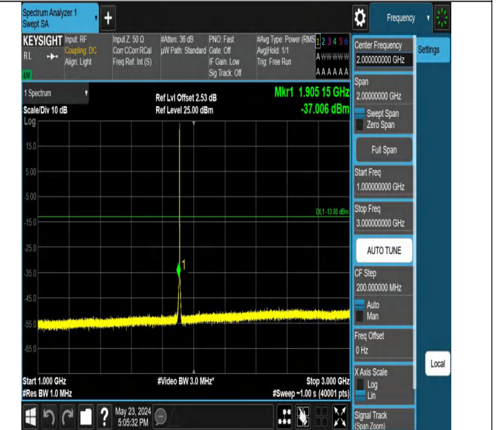
Band2_1.4MHz_QPSK_19193_1RB#0_1000~3000_1000~3000
