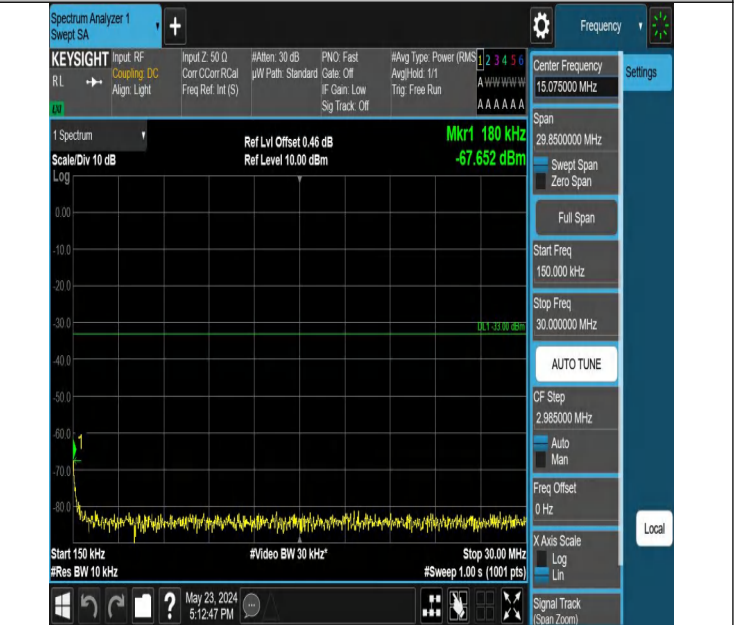
Band2_3MHz_QPSK_19185_1RB#0_0.15~30_0.15~30
