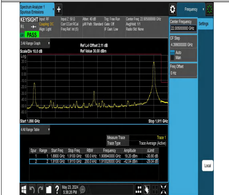
Band2_20MHz_QPSK_19100_1RB#99
