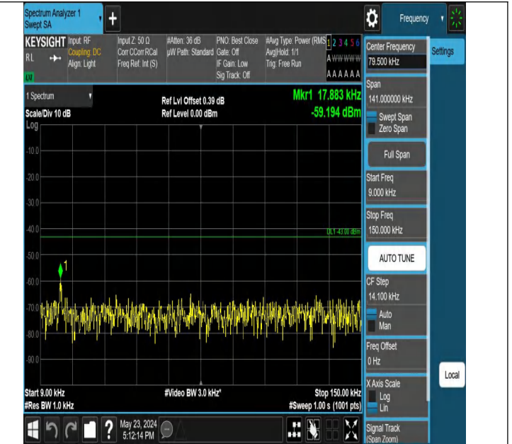
Band2_3MHz_QPSK_18900_1RB#14_0.009~0.15_0.009~0.15
