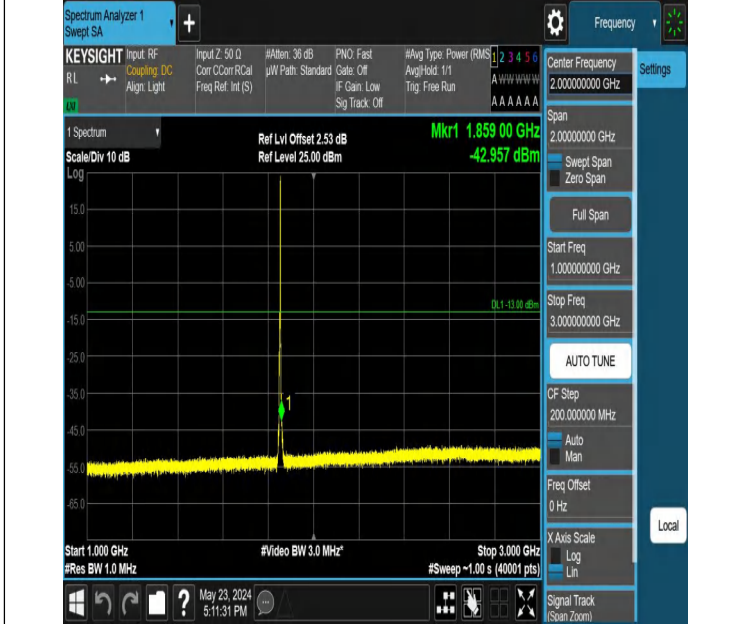
Band2_3MHz_QPSK_18615_1RB#14_1000~3000_1000~3000
