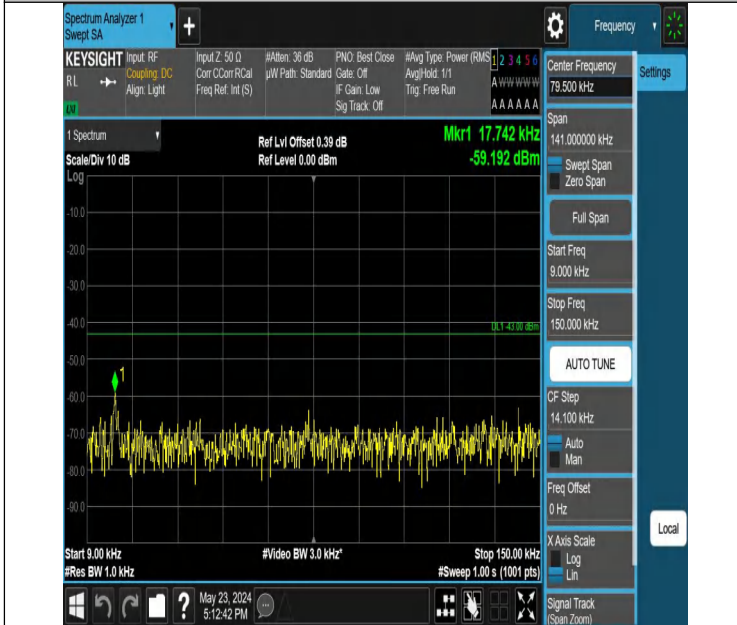
Band2_3MHz_QPSK_19185_1RB#0_0.009~0.15_0.009~0.15
