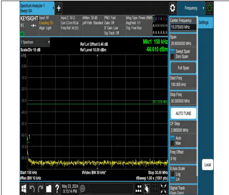
Band2_3MHz_QPSK_19185_1RB#14_0.15~30_0.15~30
