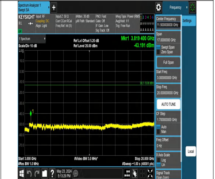
Band2_3MHz_QPSK_19185_1RB#14_3000~20000_3000~20000
