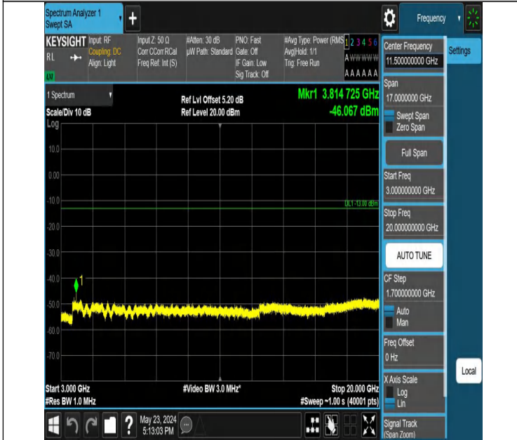
Band2_3MHz_QPSK_19185_1RB#0_3000~20000_3000~20000
