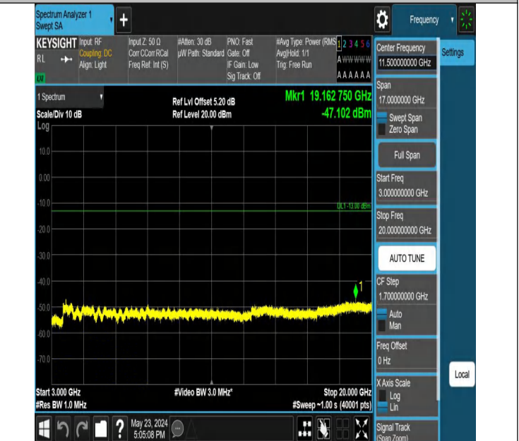
Band2_1.4MHz_QPSK_18900_1RB#5_3000~20000_3000~20000
