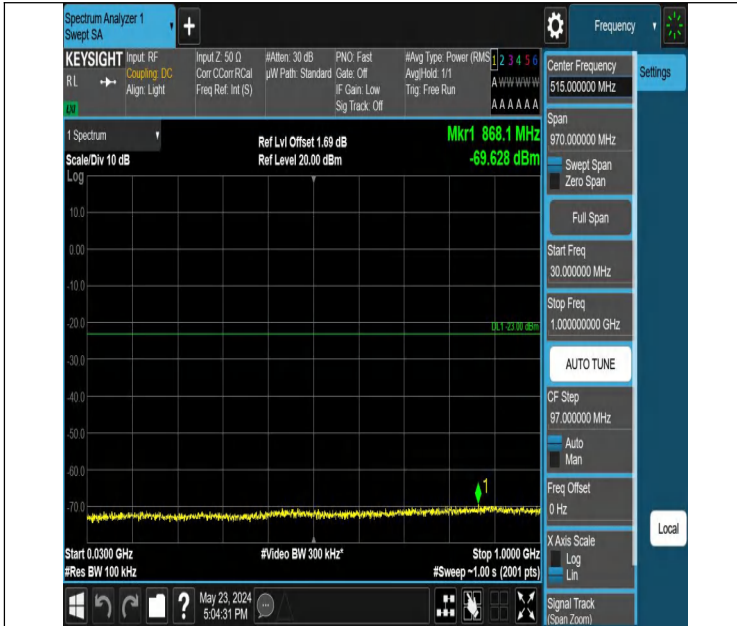
Band2_1.4MHz_QPSK_18900_1RB#0_30~1000_30~1000
