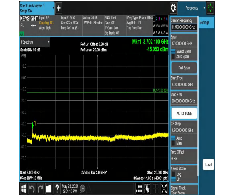
Band2_1.4MHz_QPSK_18607_1RB#5_3000~20000_3000~20000
