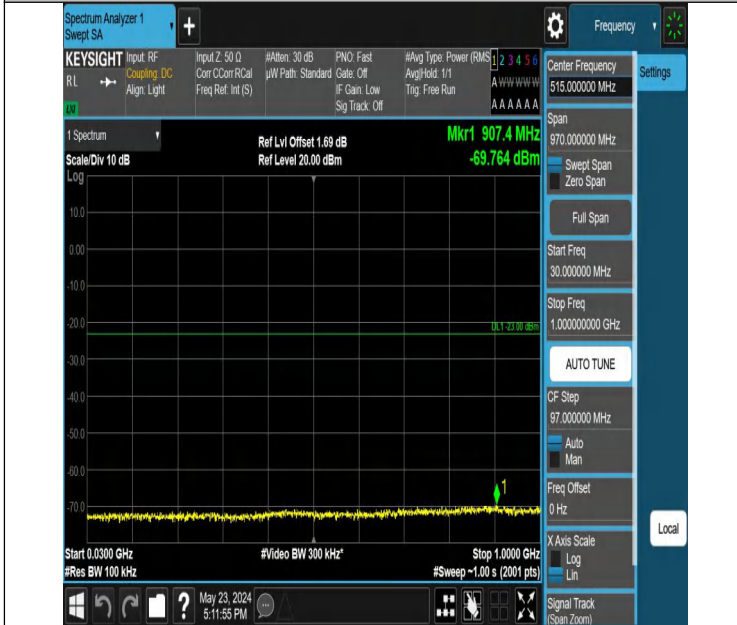
Band2_3MHz_QPSK_18900_1RB#0_30~1000_30~1000
