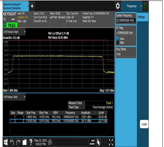
Band2_15MHz_QPSK_19125_75RB#0
