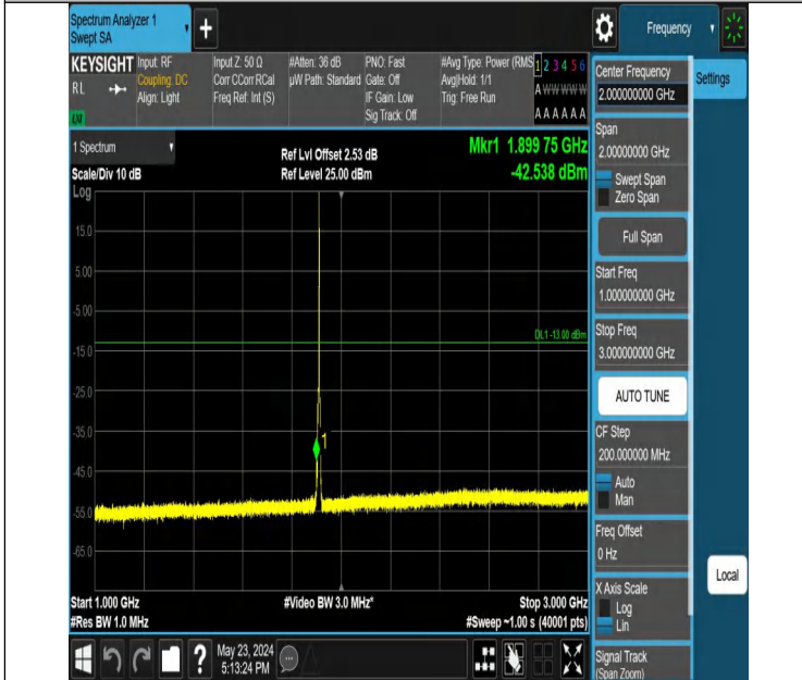
Band2_3MHz_QPSK_19185_1RB#14_1000~3000_1000~3000
