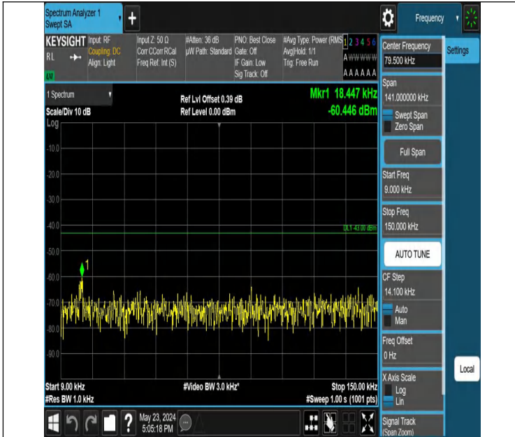
Band2_1.4MHz_QPSK_19193_1RB#0_0.009~0.15_0.009~0.15
