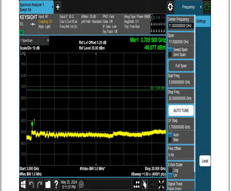
Band2_3MHz_QPSK_18615_1RB#14_3000~20000_3000~20000
