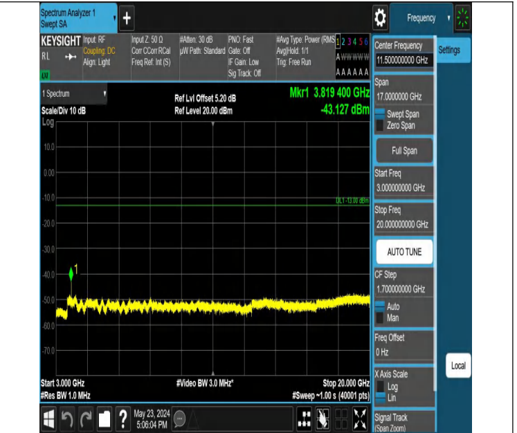
Band2_1.4MHz_QPSK_19193_1RB#5_3000~20000_3000~20000
