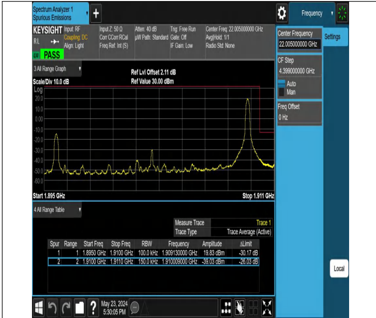
Band2_15MHz_QPSK_19125_1RB#74
