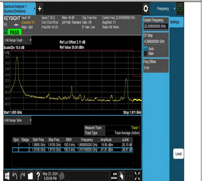
Band2_15MHz_QPSK_19125_1RB#0
