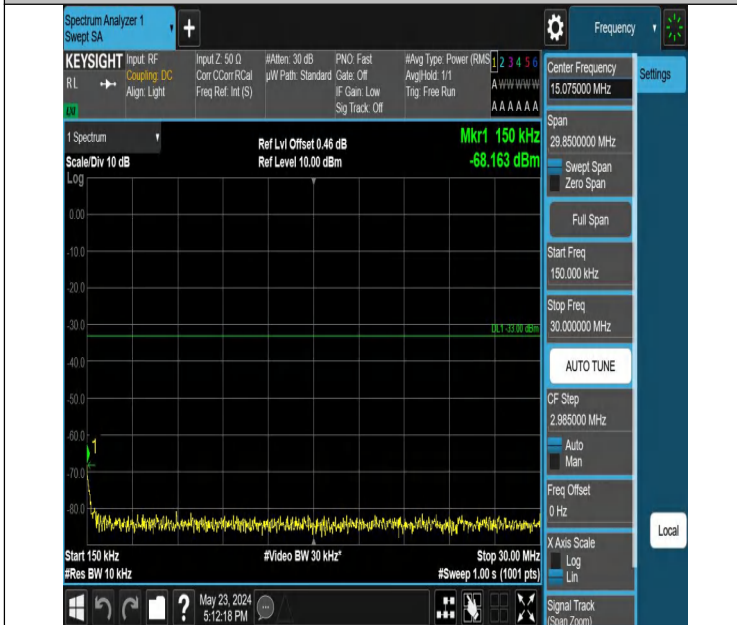
Band2_3MHz_QPSK_18900_1RB#14_0.15~30_0.15~30
