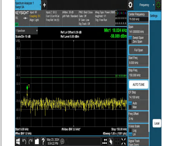
Band2_1.4MHz_QPSK_18900_1RB#0_0.009~0.15_0.009~0.15
