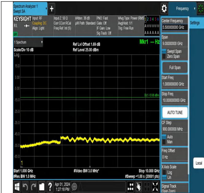
Band5-4 182-1-1000~10000MHz-PASS
