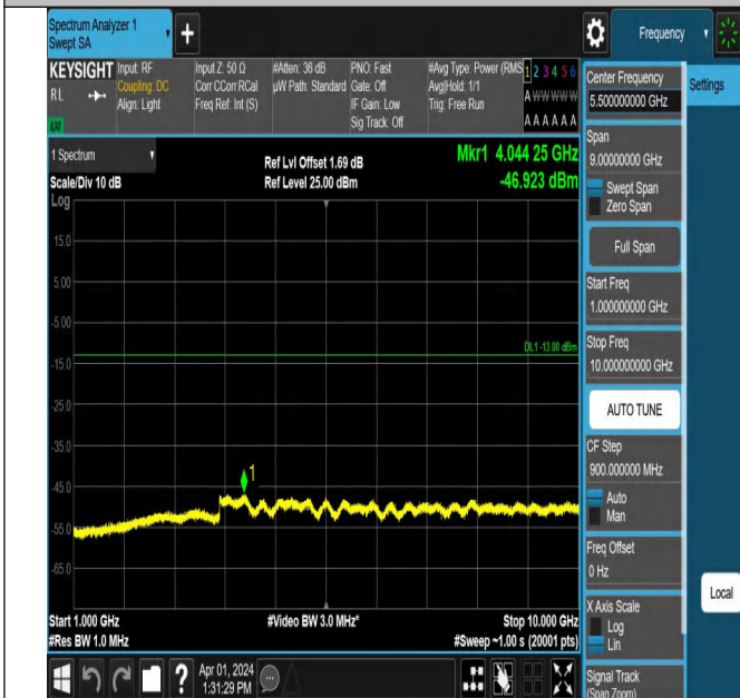
Band5-4 182-3-1000~10000MHz-PASS
