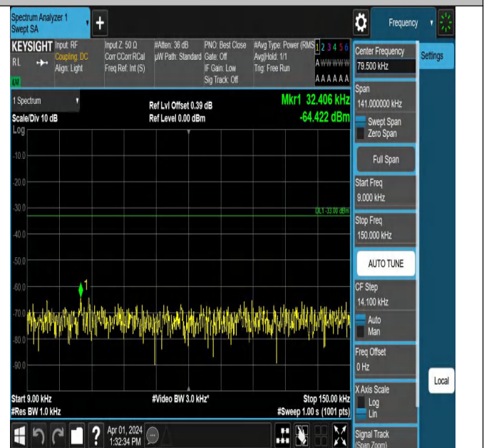
Band5-4132-4-0.009~0.15MHz-PASS
