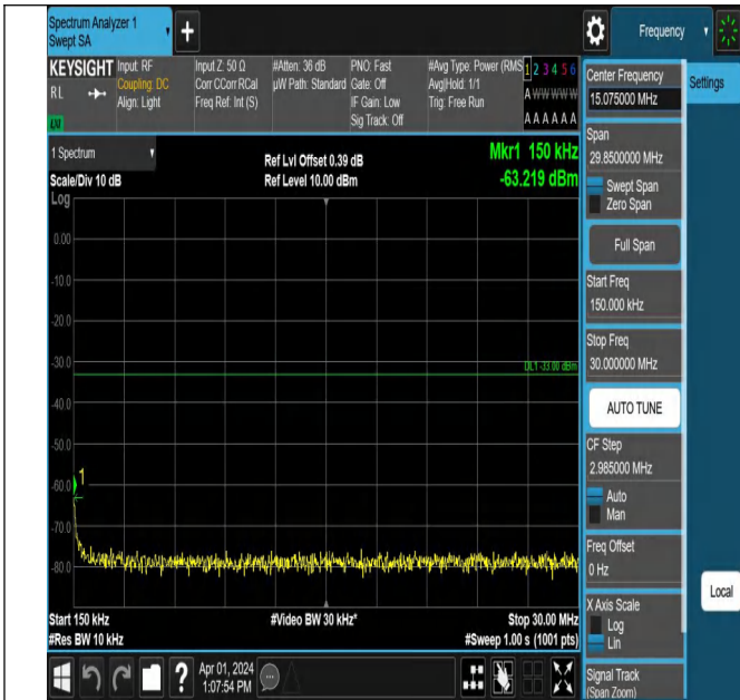
Band4-1312-4-0.15~30MHz-PASS
