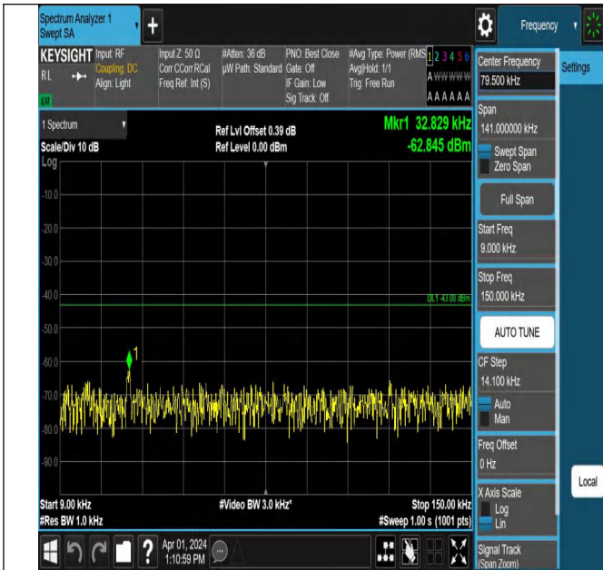
Band4-1413-5-0.009~0.15MHz-PASS
