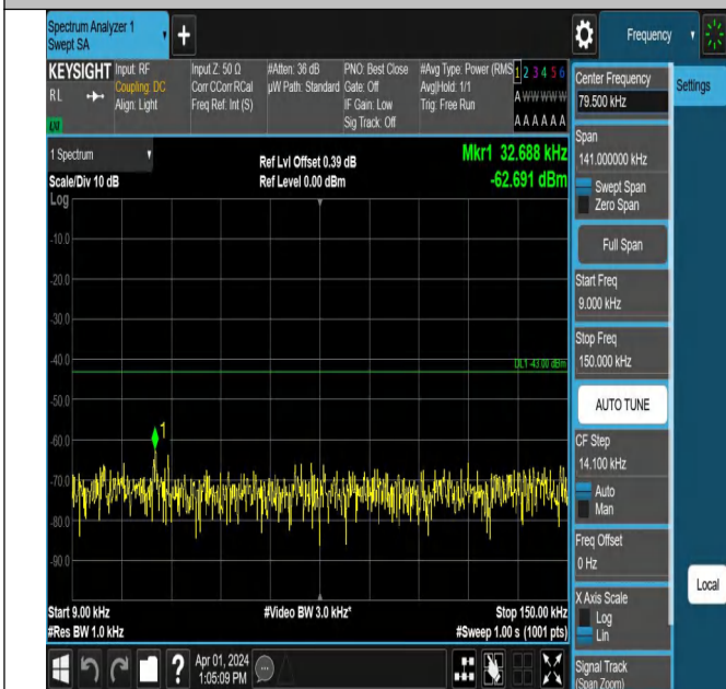
Band4-1312-3-0.009~0.15MHz-PASS
