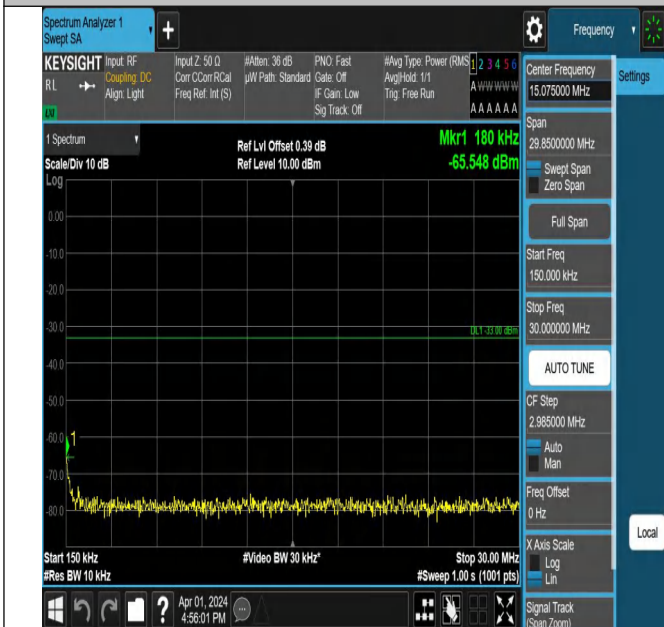
Band4-1513-3-0.15~30MHz-PASS
