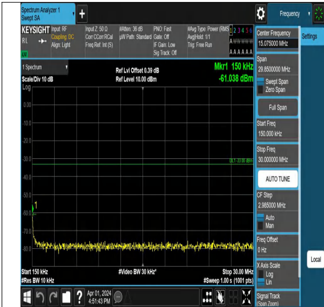
Band4-1513-1-0.15~30MHz-PASS
