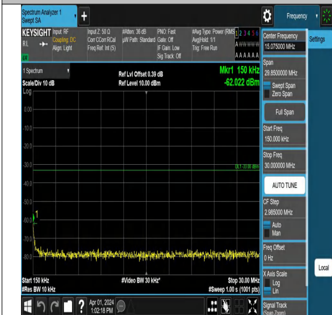
Band4-1312-2-0.15~30MHz-PASS
