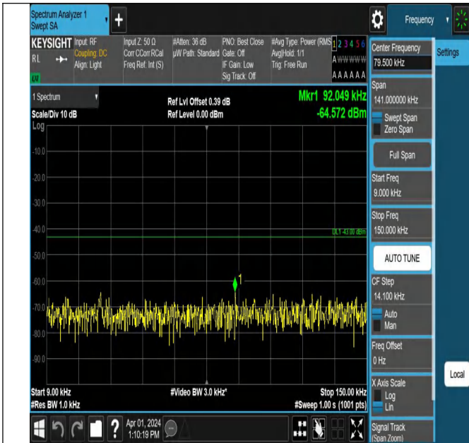
Band4-1312-5-0.009~0.15MHz-PASS
