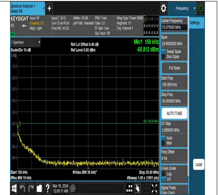
Band43_5MHz_QPSK_43615_1RB#0_0.15~30_0.15~30
