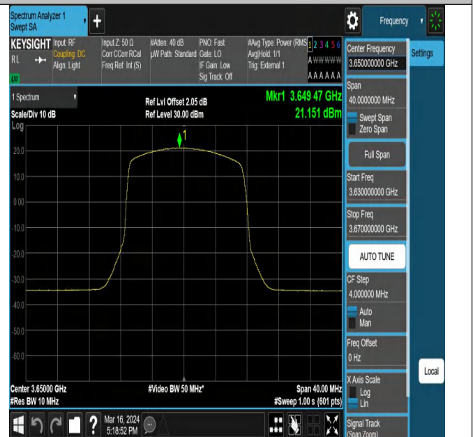
43(3600-3700)-20MHz-16QAM-44090-1RB#49-PASS
