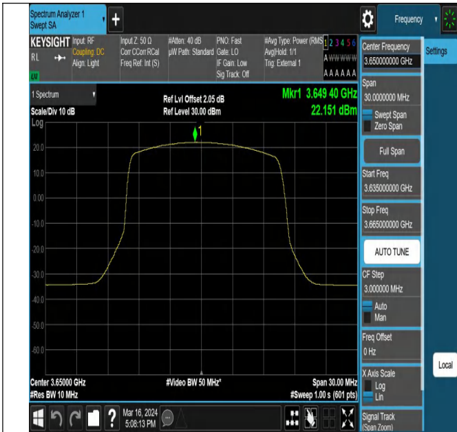
43(3600-3700)-15MHz-QPSK-44090-1RB#38-PASS
