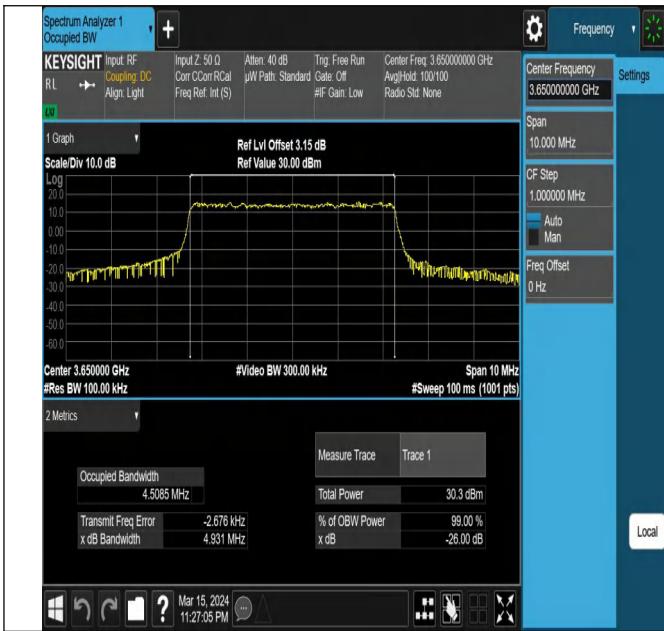
43(3600-3700)-5MHz-QPSK-44090-25RB#0-PASS
