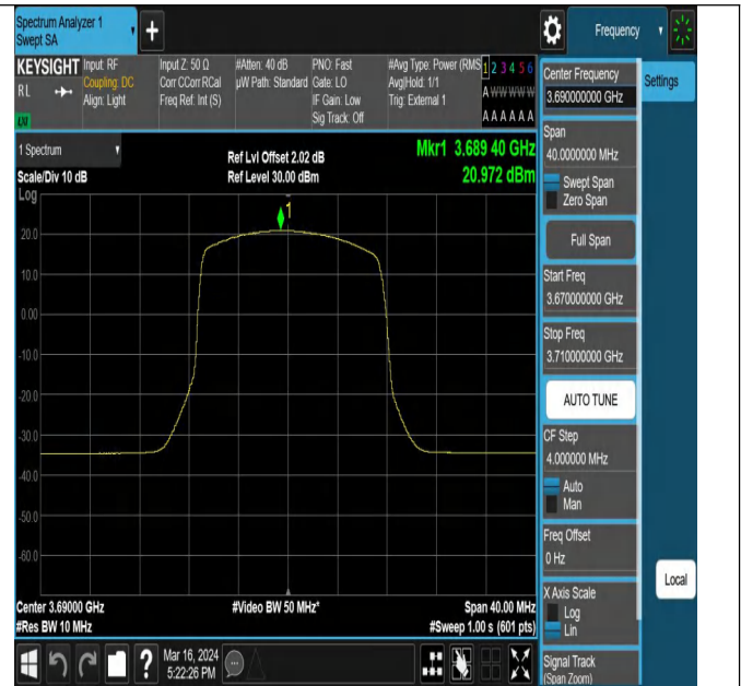
43(3600-3700)-20MHz-16QAM-44490-1RB#49-PASS
