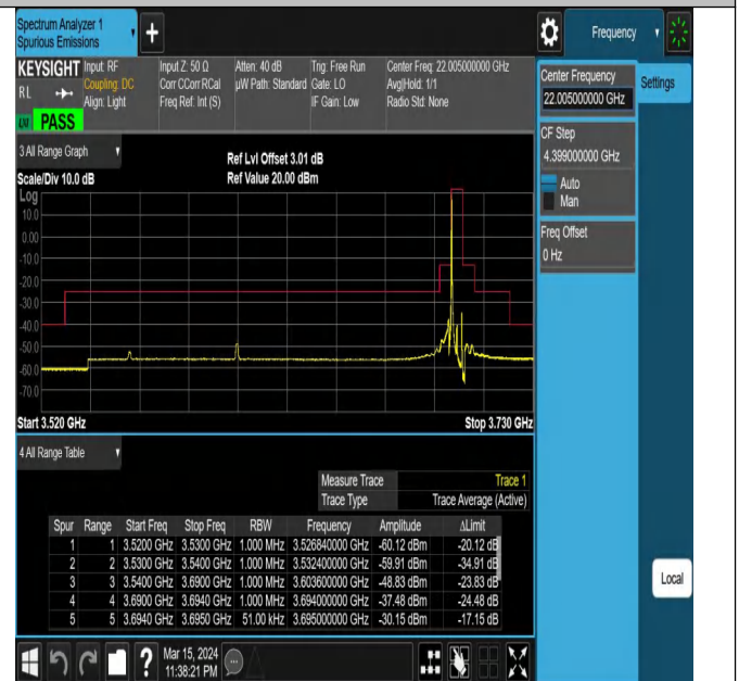
Band43_5MHz_QPSK_44565_1RB#0
