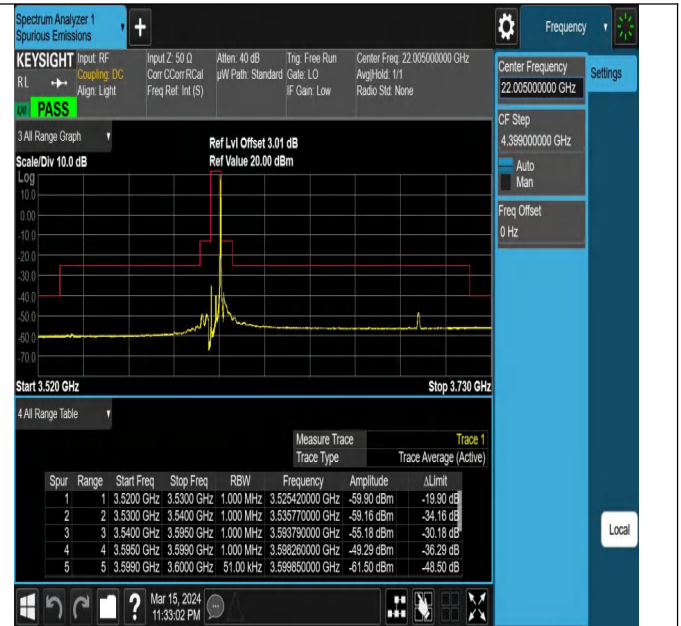
Band43_5MHz_QPSK_43615_1RB#24
