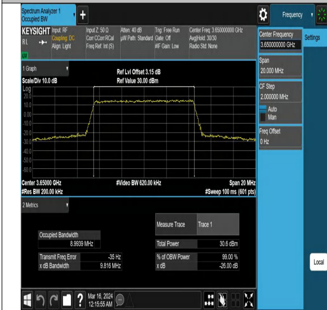
43(3600-3700)-10MHz-QPSK-44090-50RB#0-PASS
