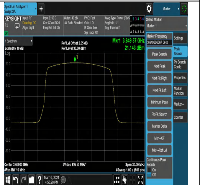
43(3600-3700)-10MHz-16QAM-44090-1RB#24-PASS
