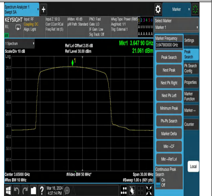
43(3600-3700)-5MHz-16QAM-44090-1RB#0-PASS
