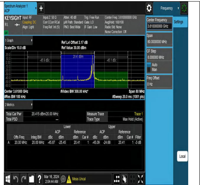
43(3600-3700)-20MHz-16QAM-43690-1RB#99-PASS
