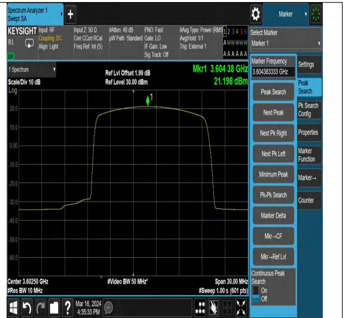
43(3600-3700)-5MHz-16QAM-43615-1RB#24-PASS
