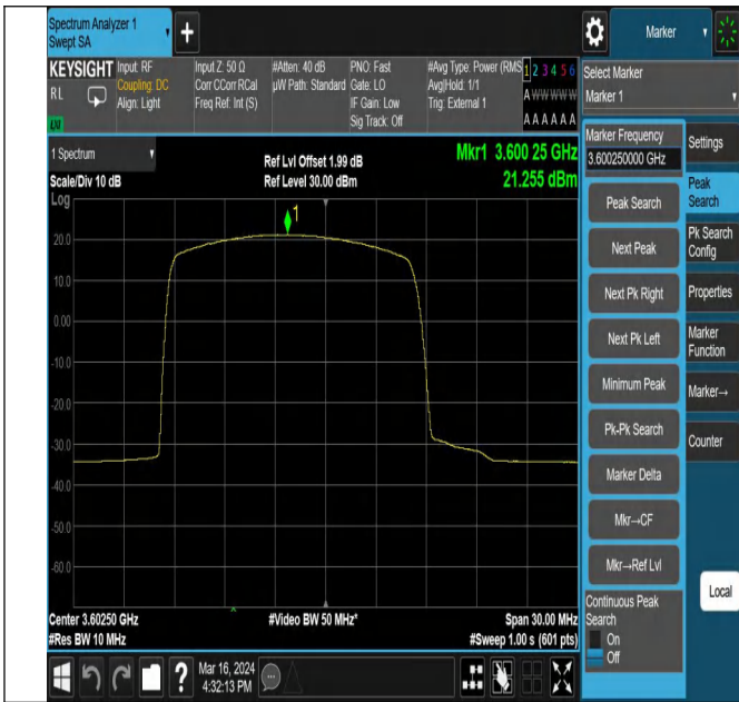
43(3600-3700)-5MHz-16QAM-43615-1RB#0-PASS
