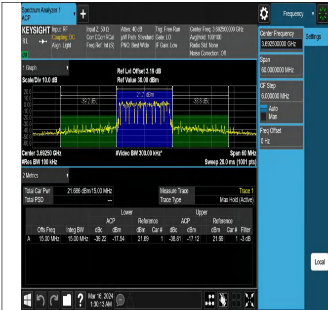
43(3600-3700)-15MHz-QPSK-44515-75RB#0-PASS
