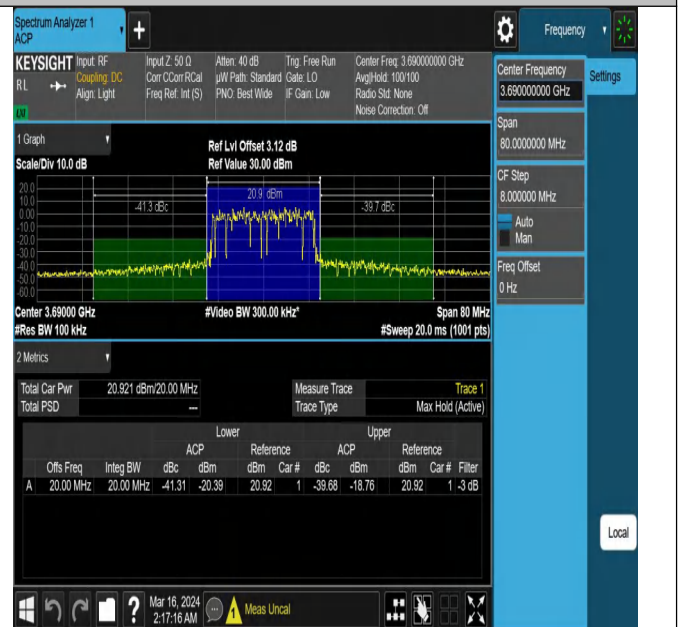
43(3600-3700)-20MHz-16QAM-44490-100RB#0-PASS
