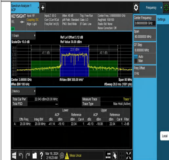
43(3600-3700)-20MHz-QPSK-44490-100RB#0-PASS
