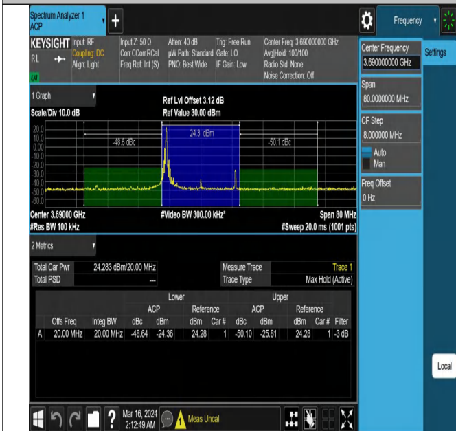
43(3600-3700)-20MHz-QPSK-44490-1RB#0-PASS
