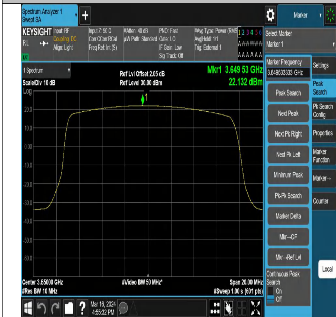
43(3600-3700)-10MHz-QPSK-44090-1RB#24-PASS
