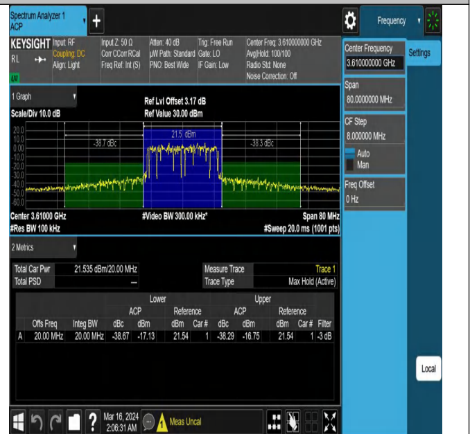
43(3600-3700)-20MHz-16QAM-43690-100RB#0-PASS
