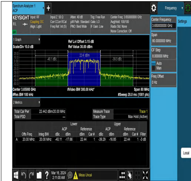
43(3600-3700)-20MHz-QPSK-44090-100RB#0-PASS
