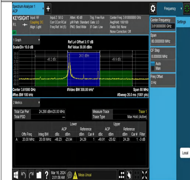
43(3600-3700)-20MHz-QPSK-43690-1RB#0-PASS
