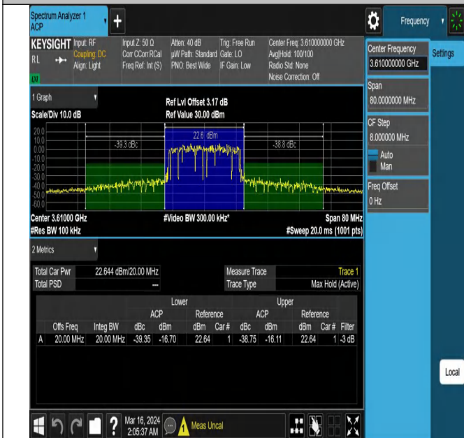
43(3600-3700)-20MHz-QPSK-43690-100RB#0-PASS
