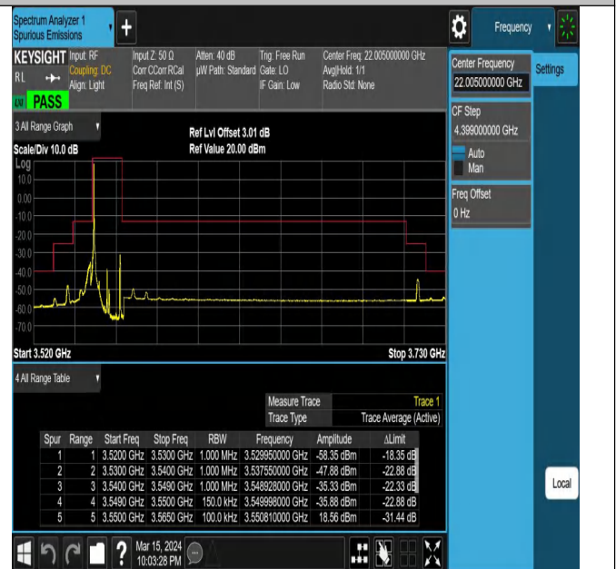
Band42_15MHz_QPSK_43165_1RB#0
