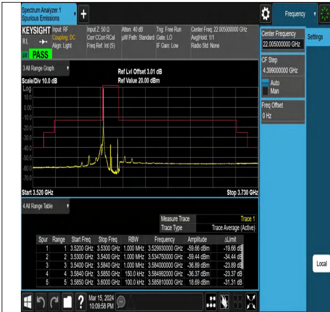
Band42_15MHz_QPSK_43515_1RB#0
