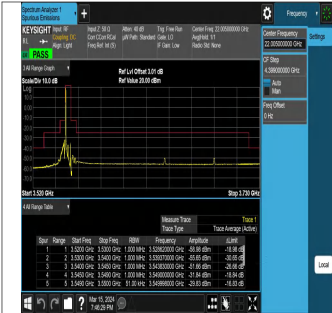
Band42_5MHz_QPSK_43115_1RB#0
