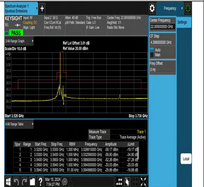
Band42_5MHz_QPSK_43565_1RB#0
