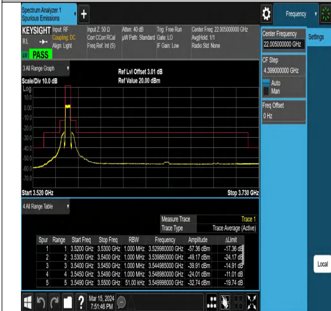
Band42_5MHz_QPSK_43115_25RB#0
