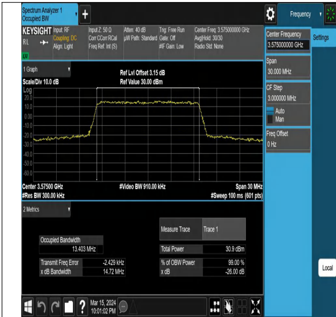
42(3550-3600)-15MHz-QPSK-43340-75RB#0-PASS
