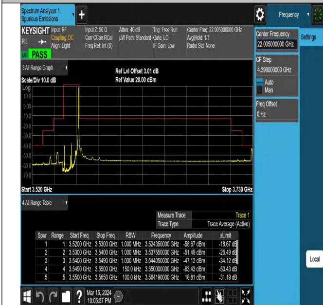
Band42_15MHz_QPSK_43165_1RB#74
