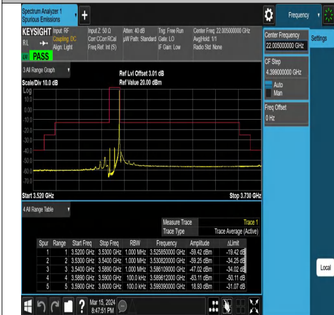
Band42_10MHz_QPSK_43540_1RB#49
