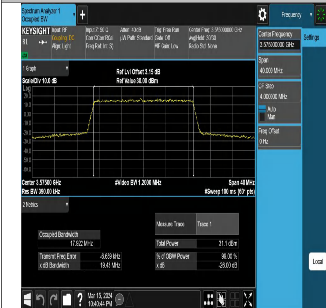
42(3550-3600)-20MHz-QPSK-43340-100RB#0-PASS
