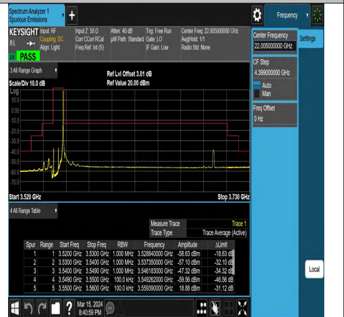
Band42_10MHz_QPSK_43140_1RB#49
