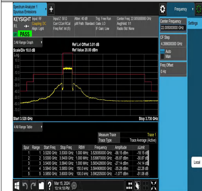
Band42_15MHz_QPSK_43515_75RB#0
