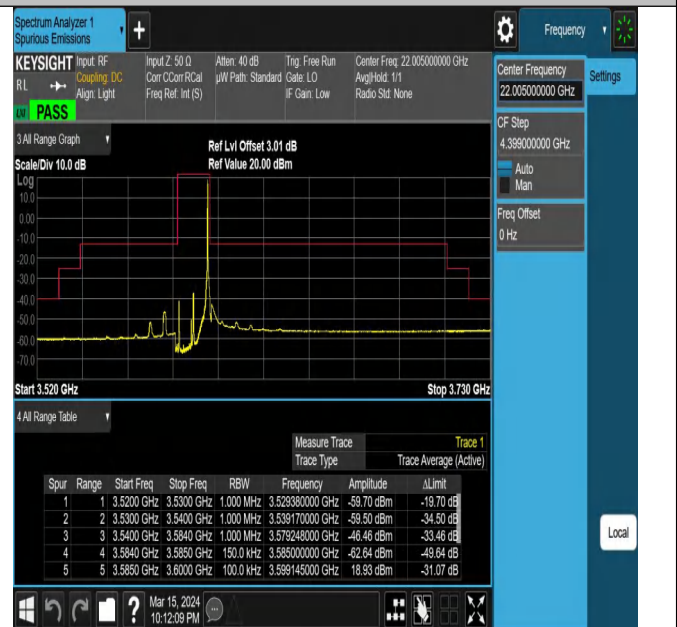
Band42_15MHz_QPSK_43515_1RB#74
