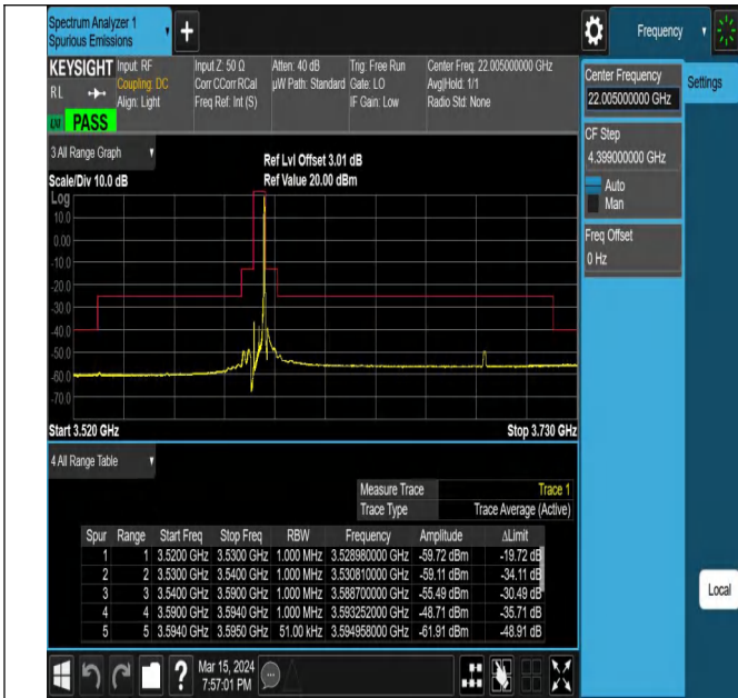
Band42_5MHz_QPSK_43565_1RB#24
