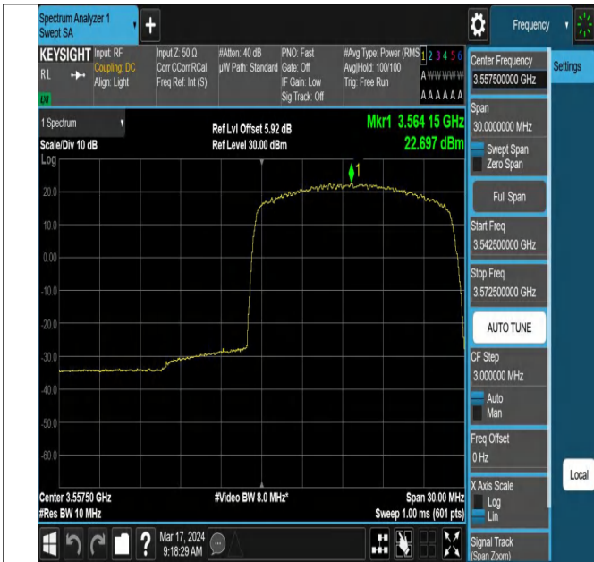
42(3550-3600)-15MHz-QPSK-43165-1RB#74-PASS
