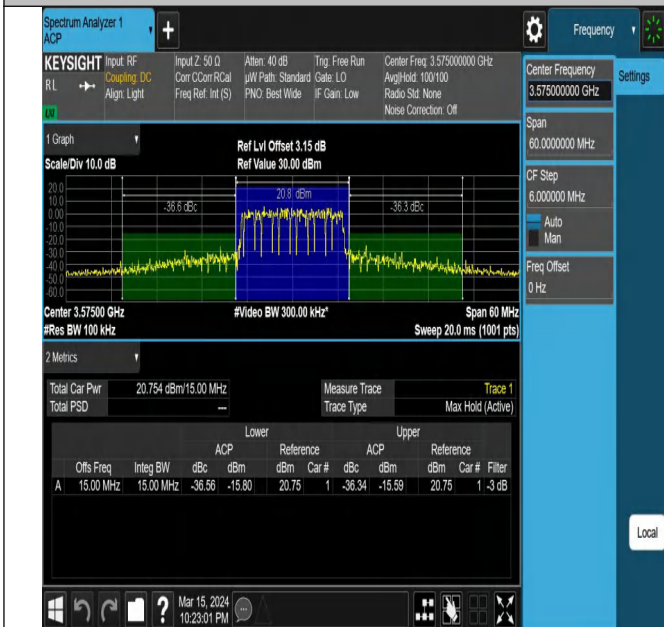
42(3550-3600)-15MHz-16QAM-43340-75RB#0-PASS
