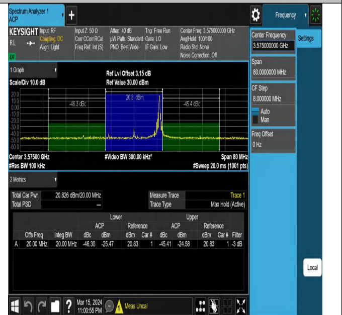
42(3550-3600)-20MHz-16QAM-43340-1RB#99-PASS
