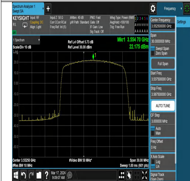
42(3550-3600)-5MHz-QPSK-43115-1RB#24-PASS
