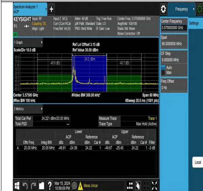
42(3550-3600)-20MHz-16QAM-43340-1RB#0-PASS
