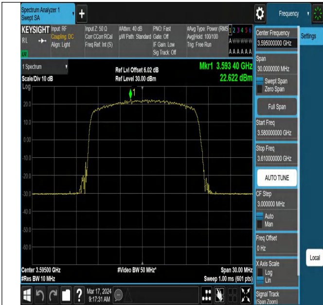
42(3550-3600)-10MHz-QPSK-43540-1RB#24-PASS
