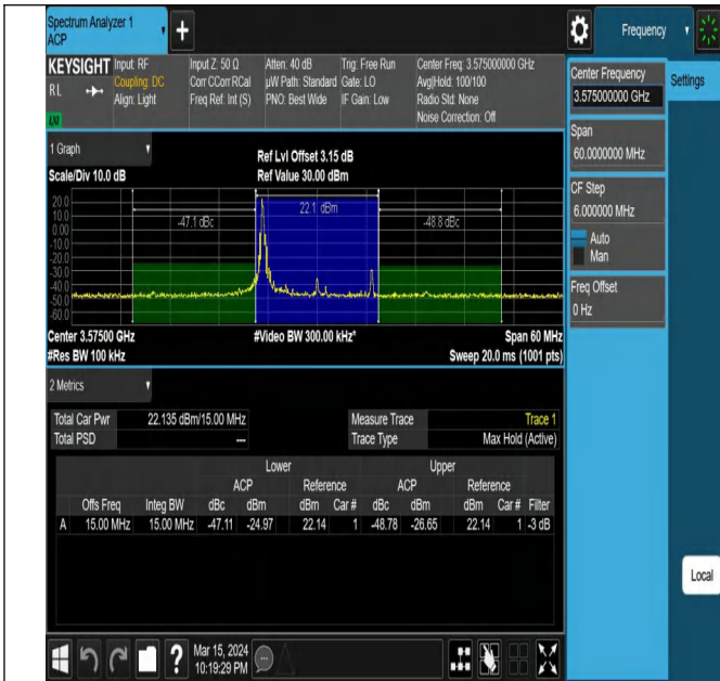
42(3550-3600)-15MHz-16QAM-43340-1RB#0-PASS
