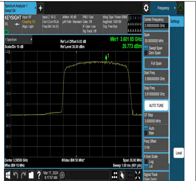
42(3550-3600)-10MHz-QPSK-43540-1RB#49-PASS
