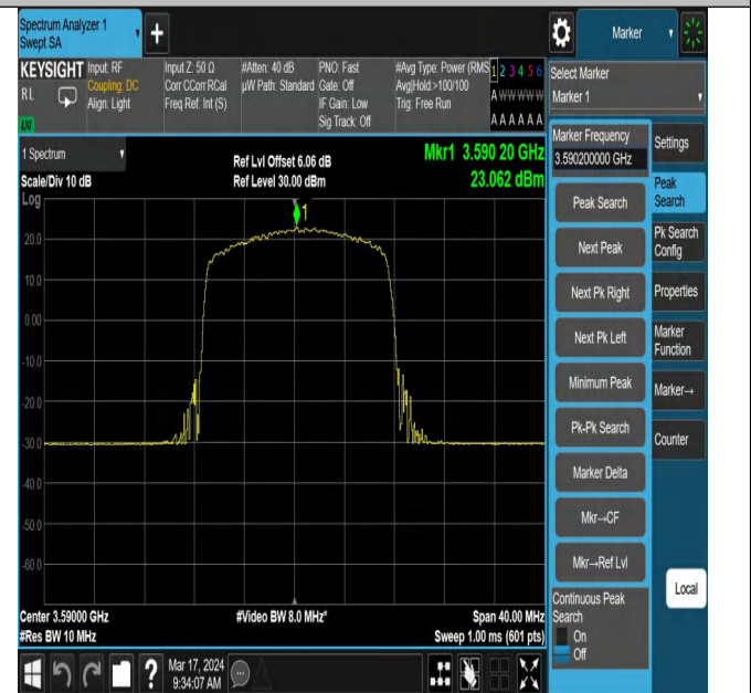
42(3550-3600)-20MHz-QPSK-43490-1RB#49-PASS
