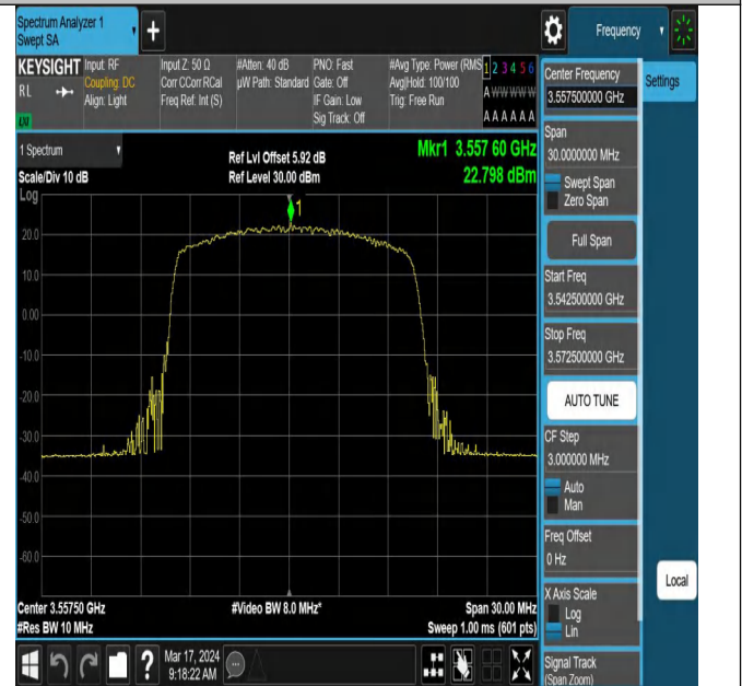
42(3550-3600)-15MHz-QPSK-43165-1RB#38-PASS
