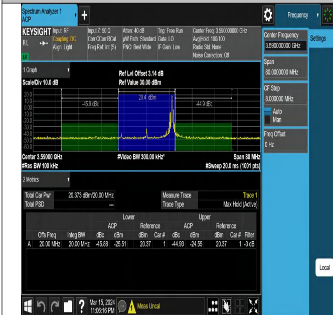
42(3550-3600)-20MHz-16QAM-43490-1RB#99-PASS
