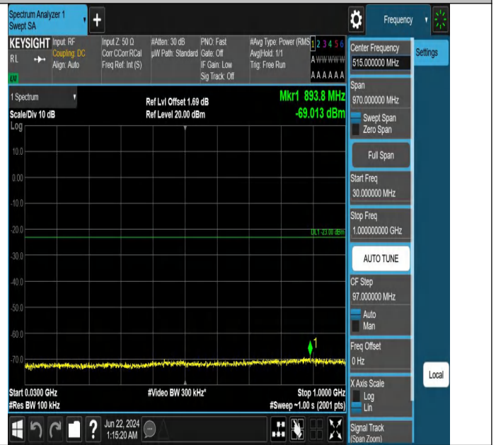
Band2_10MHz_QPSK_18650_50RB#0_30~1000_30~1000
