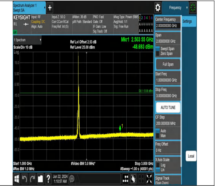
Band2_10MHz_QPSK_18900_1RB#0_1000~3000_1000~3000
