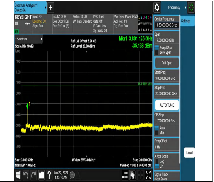
Band2_10MHz_QPSK_19150_1RB#0_3000~20000_3000~20000
