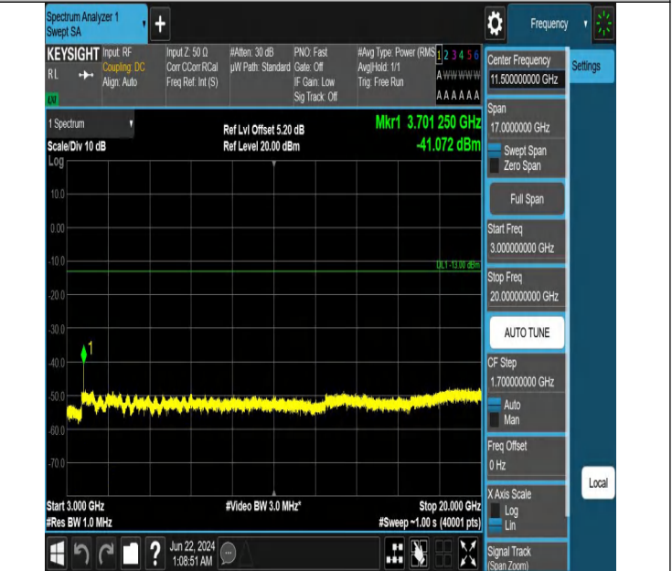
Band2_10MHz_QPSK_18650_1RB#0_3000~20000_3000~20000
