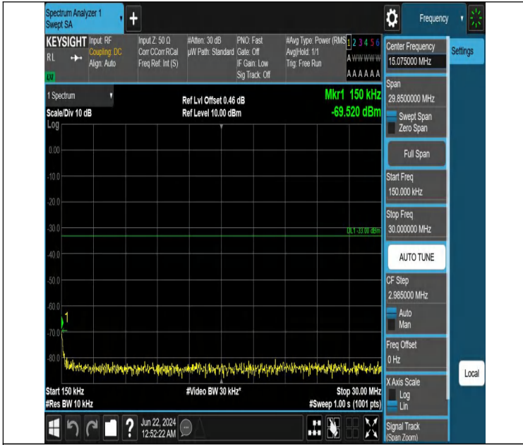
Band2_5MHz_QPSK_18900_1RB#24_0.15~30_0.15~30
