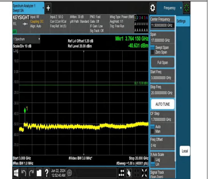
Band2_5MHz_QPSK_18900_1RB#24_3000~20000_3000~20000
