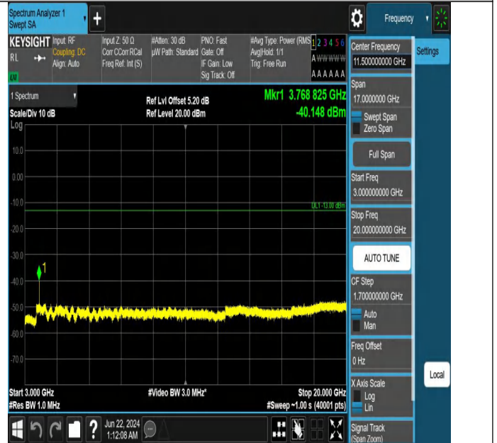
Band2_10MHz_QPSK_18900_1RB#49_3000~20000_3000~2000
