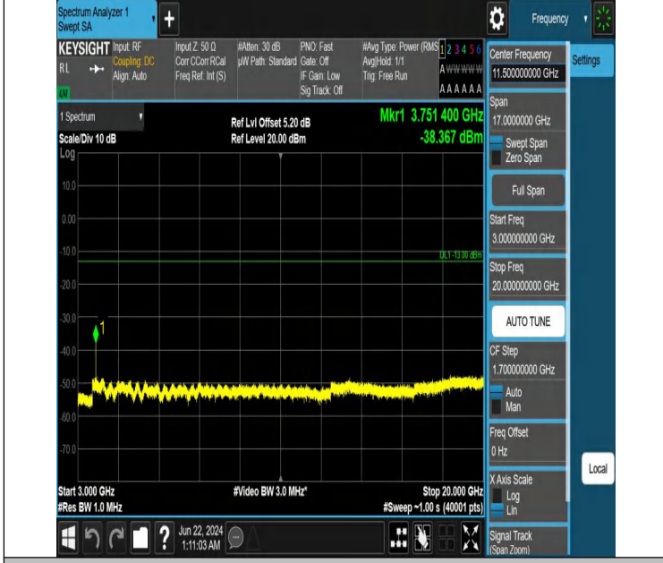
Band2_10MHz_QPSK_18900_1RB#0_3000~20000_3000~20000
