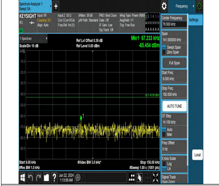
Band2_10MHz_QPSK_19150_1RB#49_0.009~0.15_0.009~0.15
