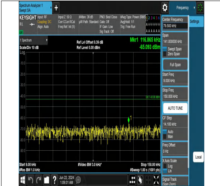
Band2_10MHz_QPSK_18650_1RB#49_0.009~0.15_0.009~0.15
