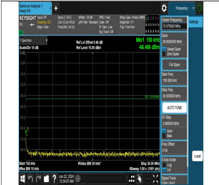
Band2_3MHz_QPSK_19185_1RB#14_0.15~30_0.15~30
