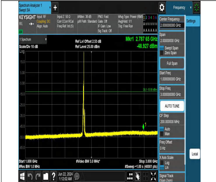
Band2_10MHz_QPSK_18900_1RB#49_1000~3000_1000~3000
