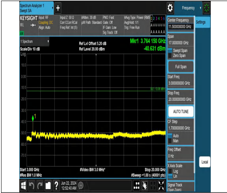
Band2_5MHz_QPSK_18900_1RB#24_3000~20000_3000~20000
