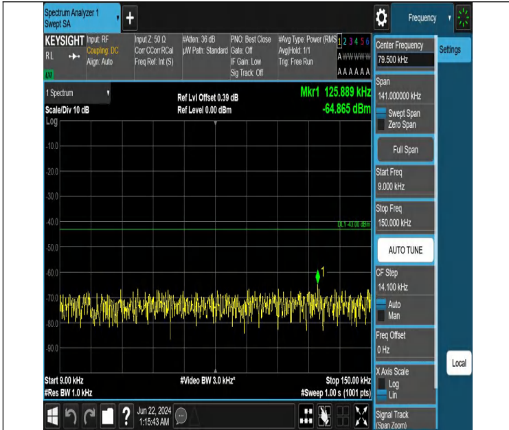
Band2_10MHz_QPSK_18900_50RB#0_0.009~0.15_0.009~0.15
