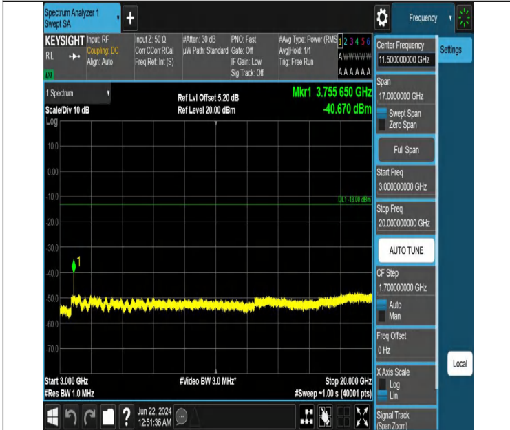
Band2_5MHz_QPSK_18900_1RB#0_3000~20000_3000~20000
