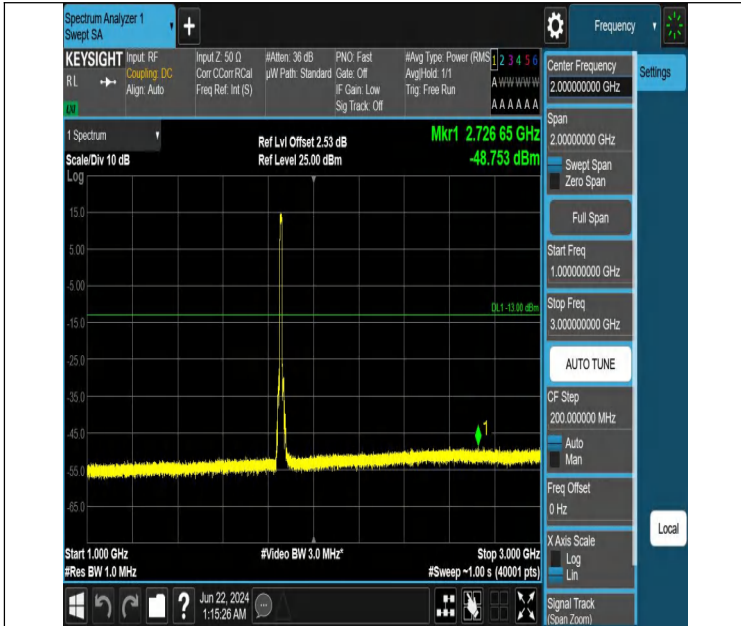
Band2_10MHz_QPSK_18650_50RB#0_1000~3000_1000~3000
