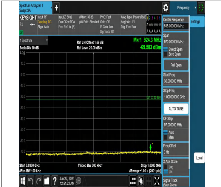
Band2_5MHz_QPSK_18900_1RB#0_30~1000_30~1000
