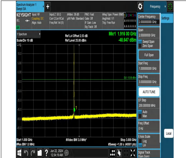
Band2_3MHz_QPSK_19185_1RB#14_1000~3000_1000~3000
