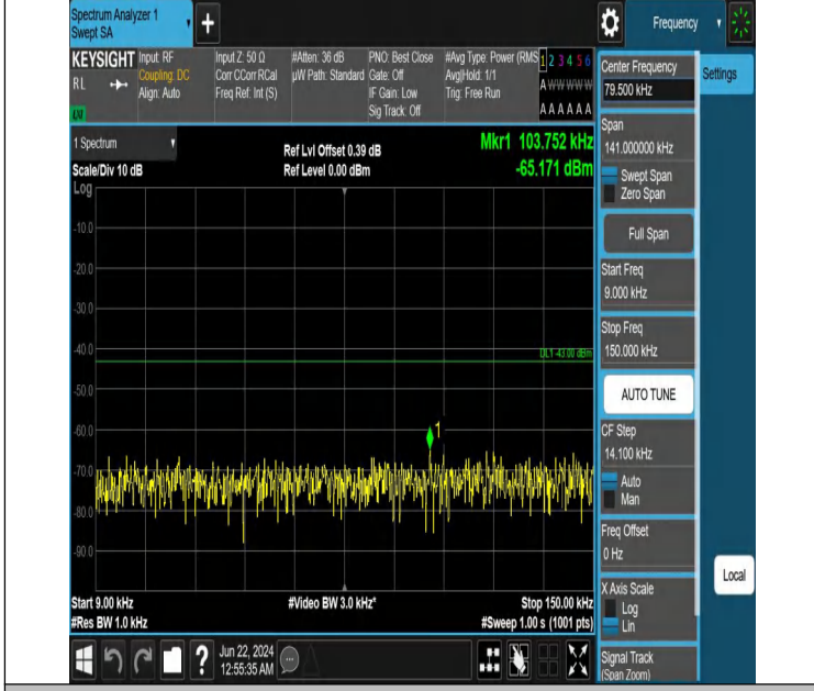
Band2_5MHz_QPSK_19175_1RB#24_0.009~0.15_0.009~0.15
