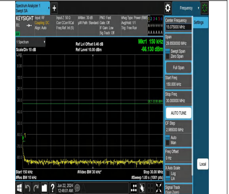
Band2_5MHz_QPSK_18625_1RB#0_0.15~30_0.15~30
