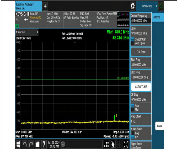
Band2_10MHz_QPSK_18650_1RB#49_30~1000_30~1000
