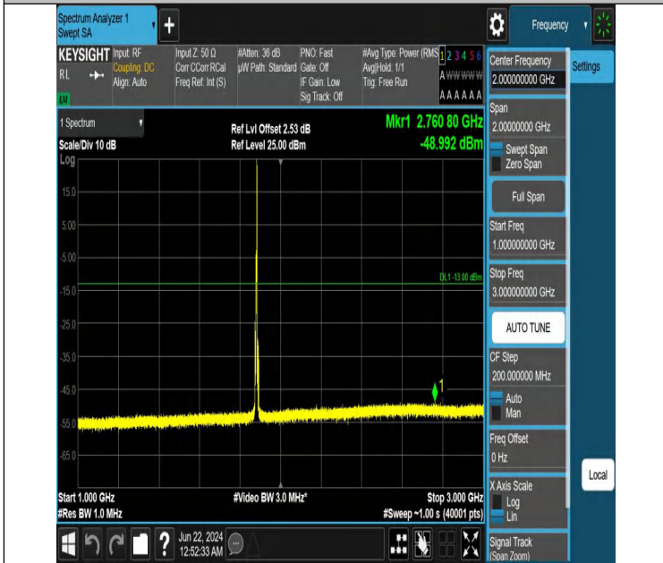
Band2_5MHz_QPSK_18900_1RB#24_1000~3000_1000~3000
