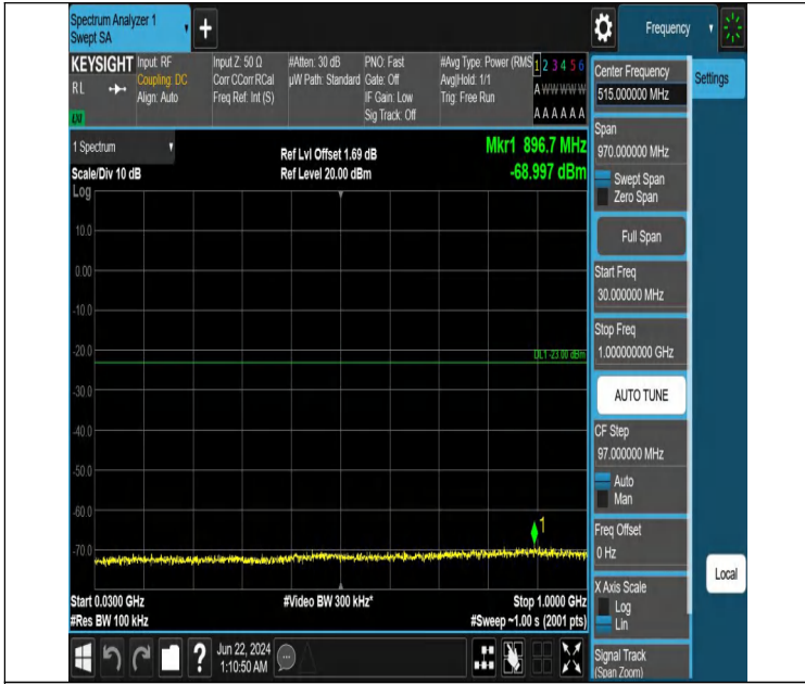
Band2_10MHz_QPSK_18900_1RB#0_30~1000_30~1000
