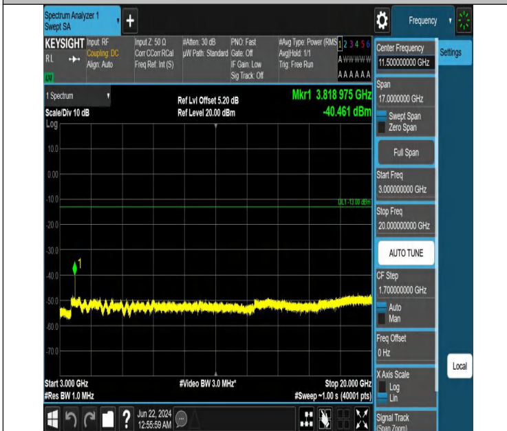
Band2_5MHz_QPSK_19175_1RB#24_3000~20000_3000~20000
