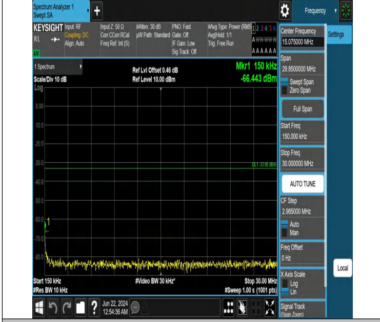
Band2_5MHz_QPSK_19175_1RB#0_0.15~30_0.15~30
