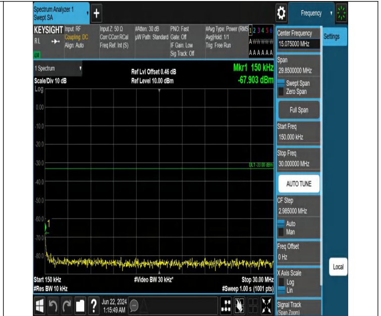
Band2_10MHz_QPSK_18900_50RB#0_0.15~30_0.15~30
