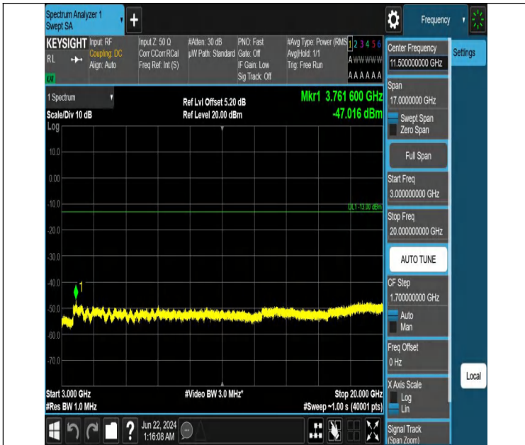
Band2_10MHz_QPSK_18900_50RB#0_3000~20000_3000~2000
