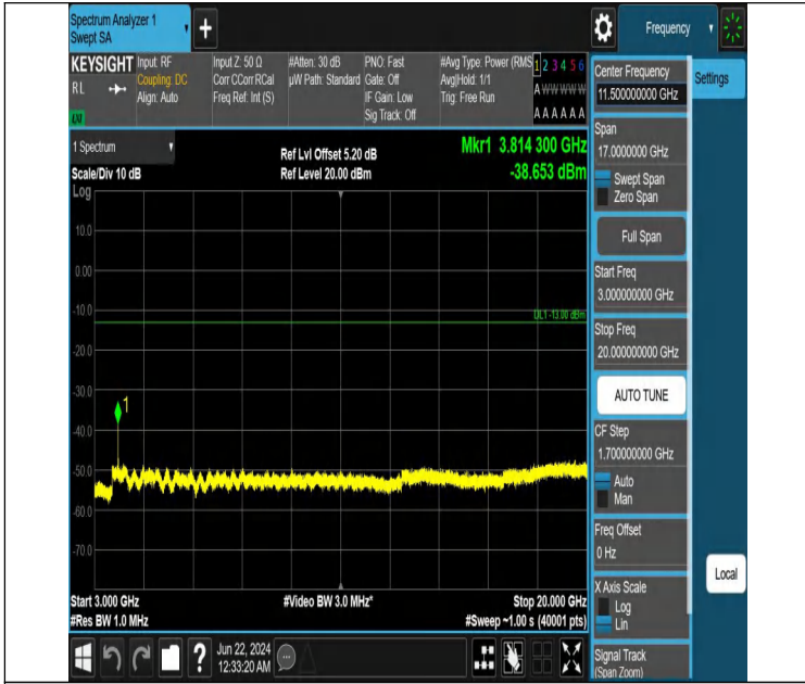
Band2_3MHz_QPSK_19185_1RB#0_3000~20000_3000~20000
