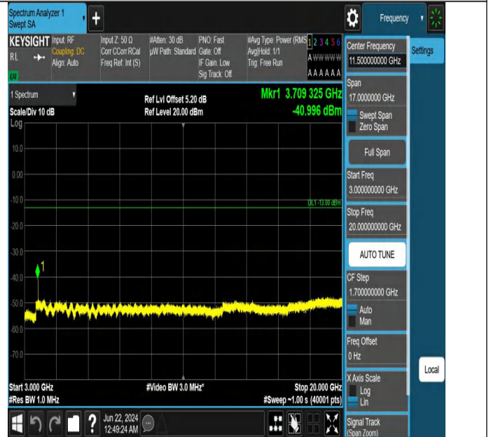
Band2_5MHz_QPSK_18625_1RB#24_3000~20000_3000~20000
