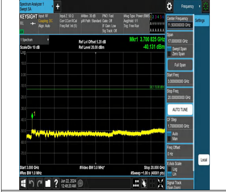
Band2_5MHz_QPSK_18625_1RB#0_3000~20000_3000~20000
