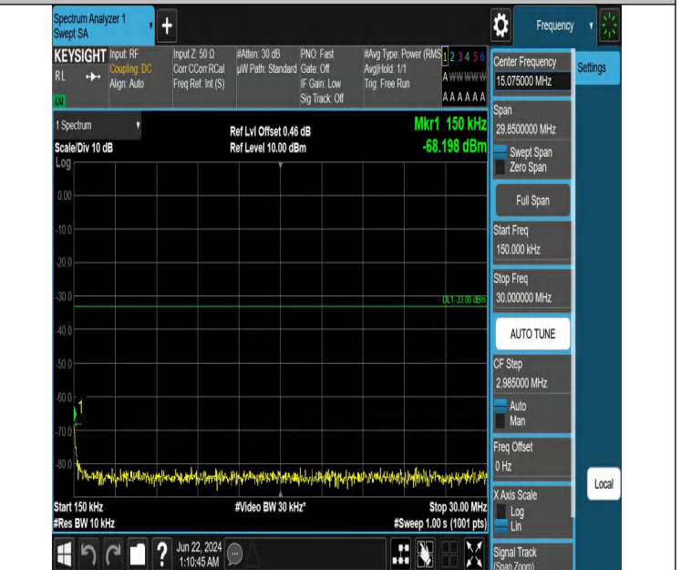
Band2_10MHz_QPSK_18900_1RB#0_0.15~30_0.15~30
