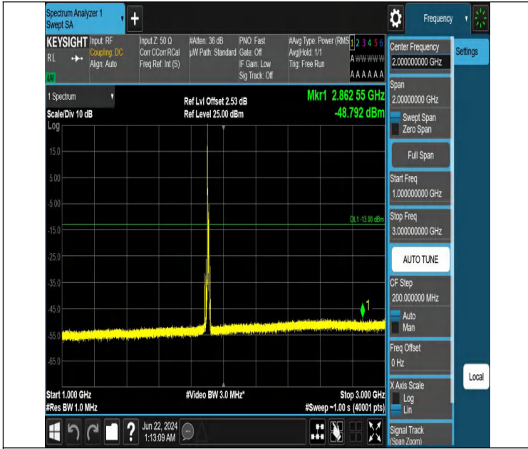
Band2_10MHz_QPSK_19150_1RB#0_1000~3000_1000~3000
