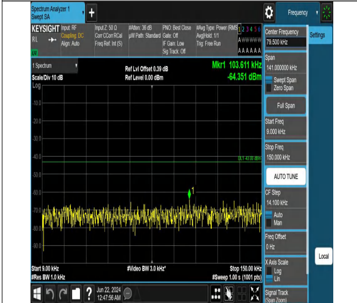
Band2_5MHz_QPSK_18625_1RB#0_0.009~0.15_0.009~0.15
