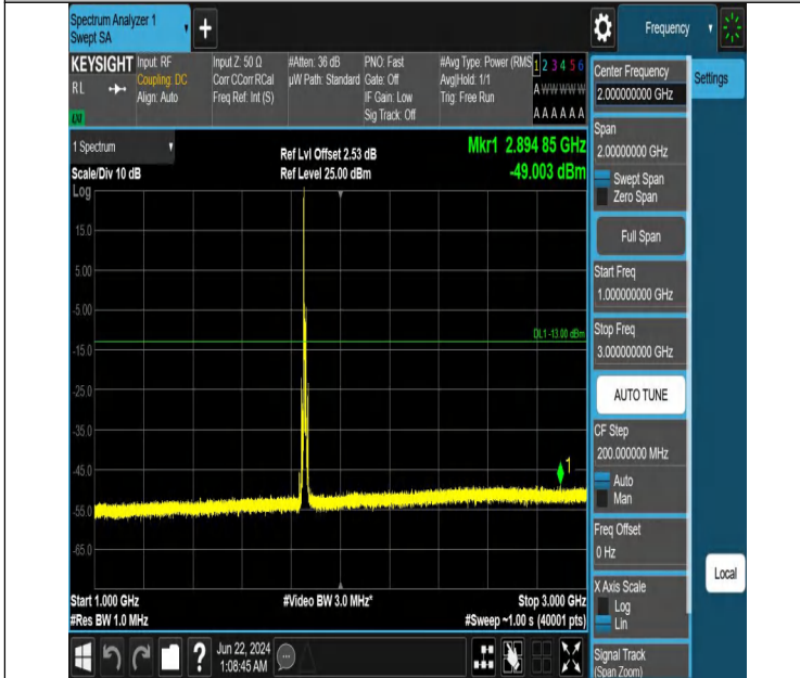
Band2_10MHz_QPSK_18650_1RB#0_1000~3000_1000~3000
