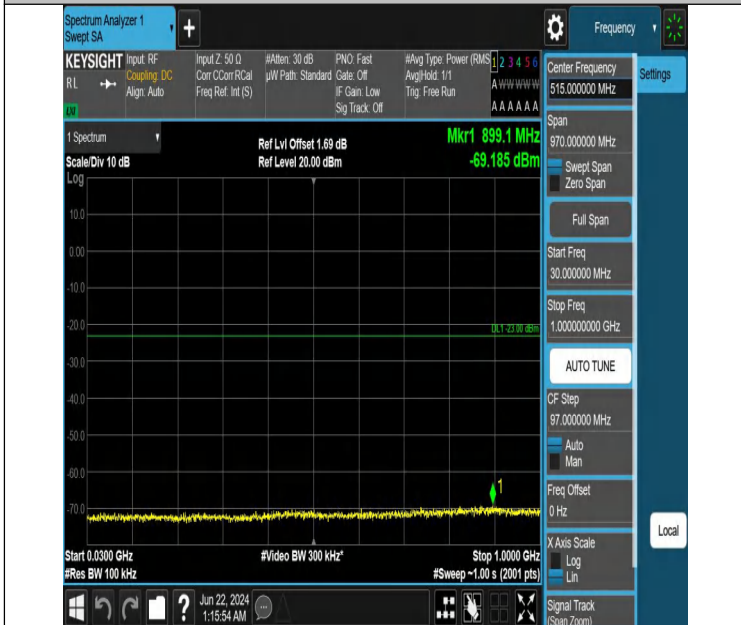
Band2_10MHz_QPSK_18900_50RB#0_30~1000_30~1000
