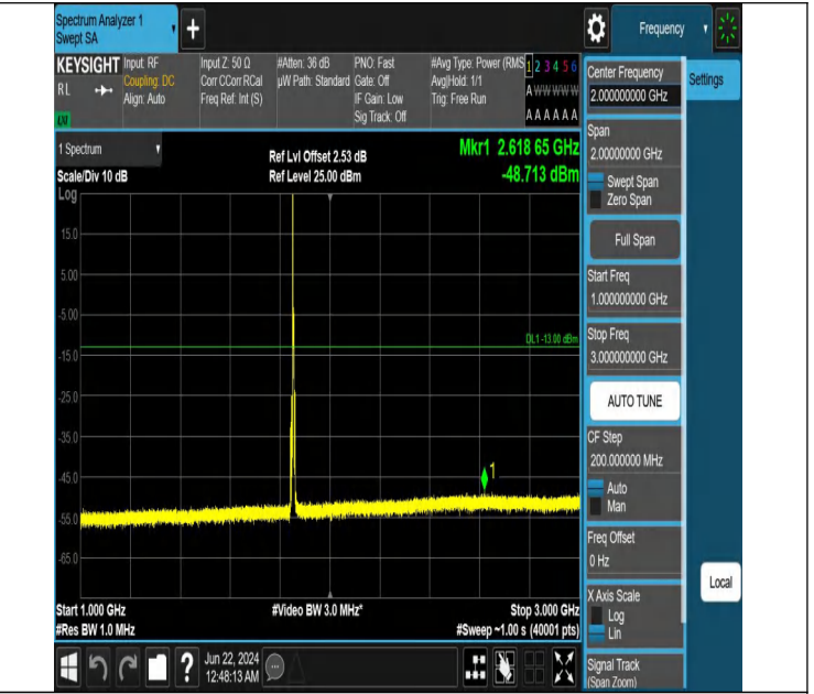
Band2_5MHz_QPSK_18625_1RB#0_1000~3000_1000~3000
