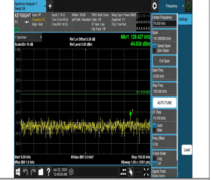
Band2_5MHz_QPSK_18625_1RB#24_0.009~0.15_0.009~0.15
