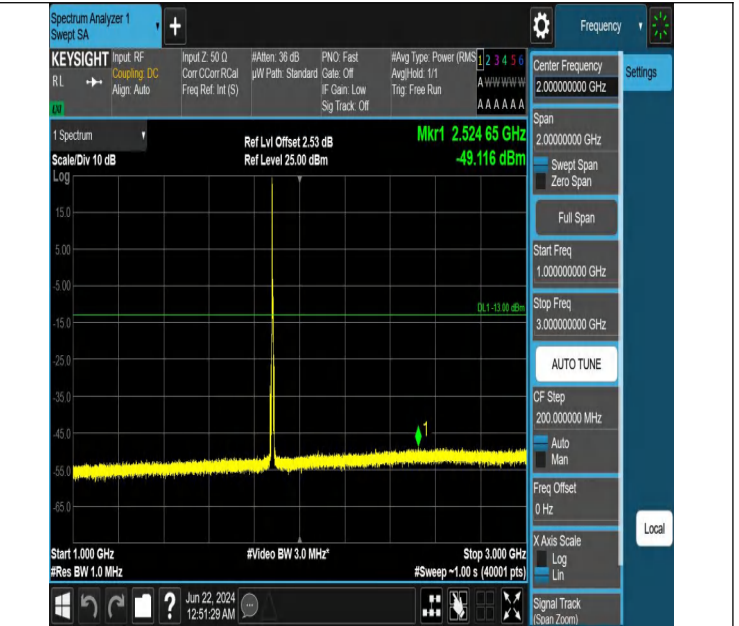
Band2_5MHz_QPSK_18900_1RB#0_1000~3000_1000~3000
