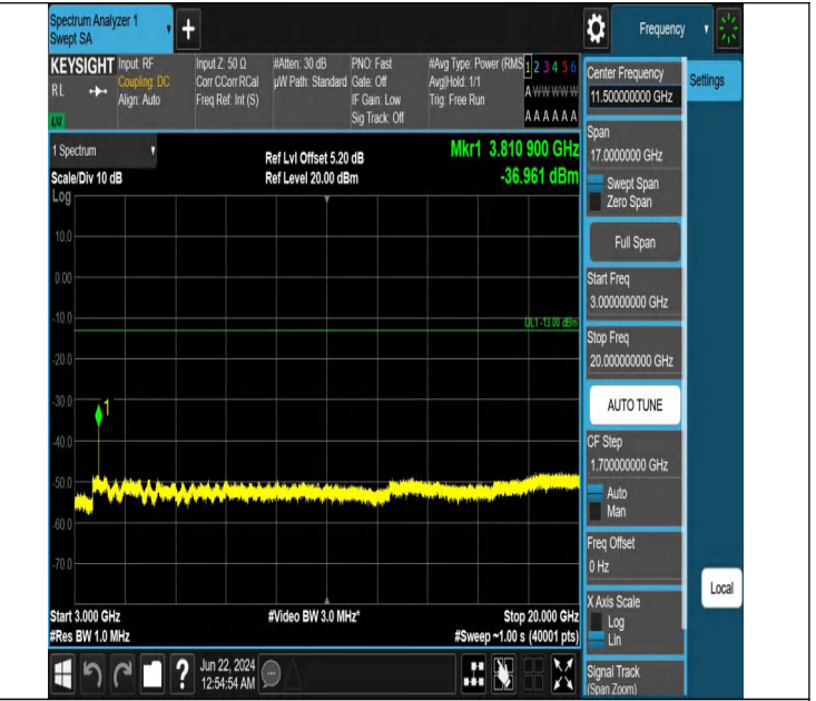
Band2_5MHz_QPSK_19175_1RB#0_3000~20000_3000~20000
