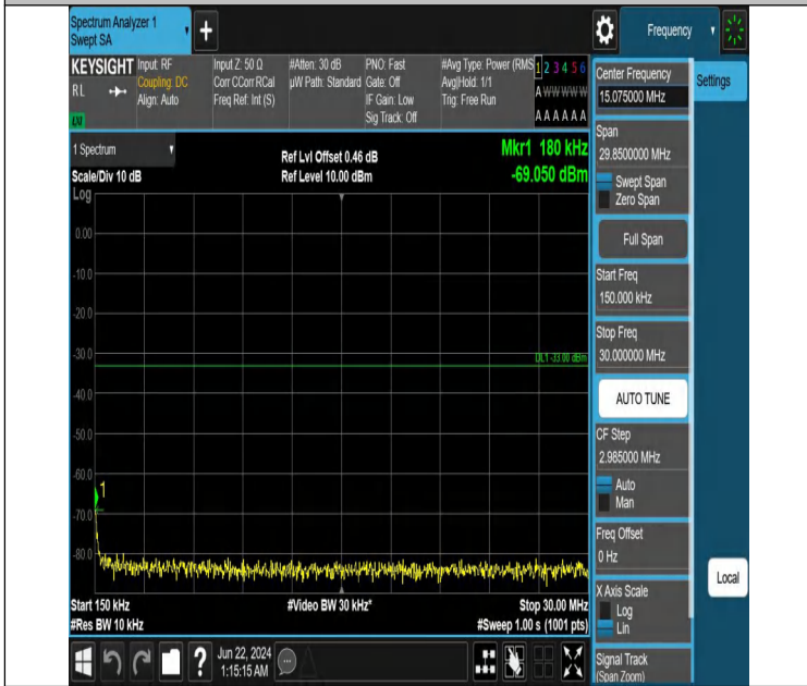
Band2_10MHz_QPSK_18650_50RB#0_0.15~30_0.15~30
