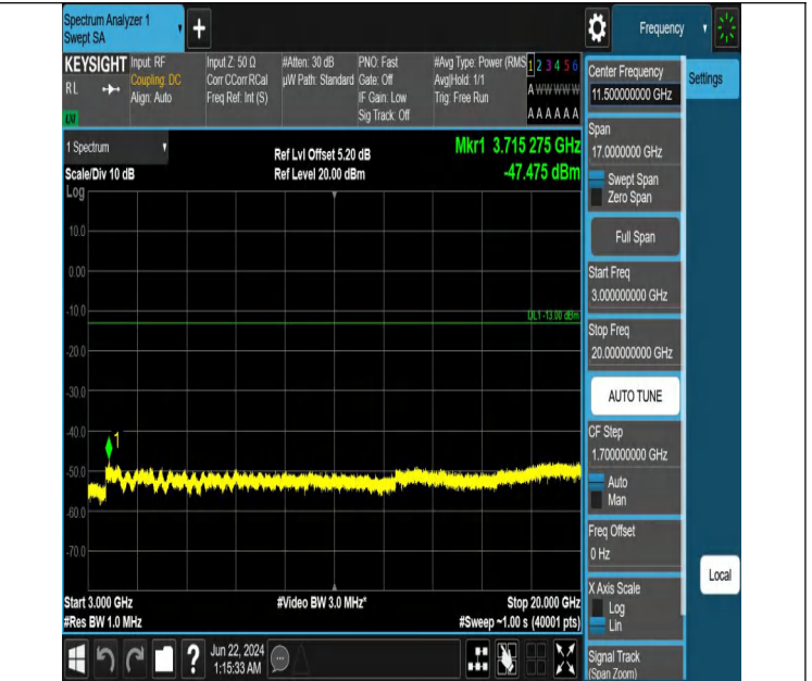
Band2_10MHz_QPSK_18650_50RB#0_3000~20000_3000~2000
