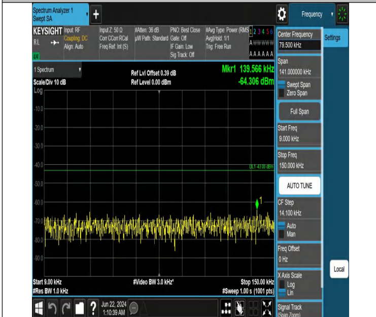
Band2_10MHz_QPSK_18900_1RB#0_0.009~0.15_0.009~0.15
