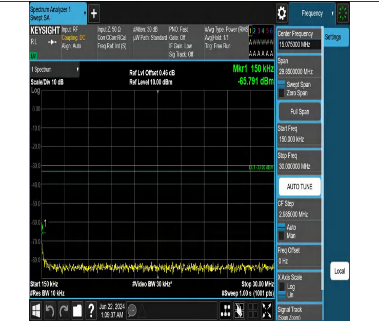
Band2_10MHz_QPSK_18650_1RB#49_0.15~30_0.15~30
