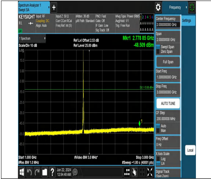
Band2_5MHz_QPSK_19175_1RB#0_1000~3000_1000~3000
