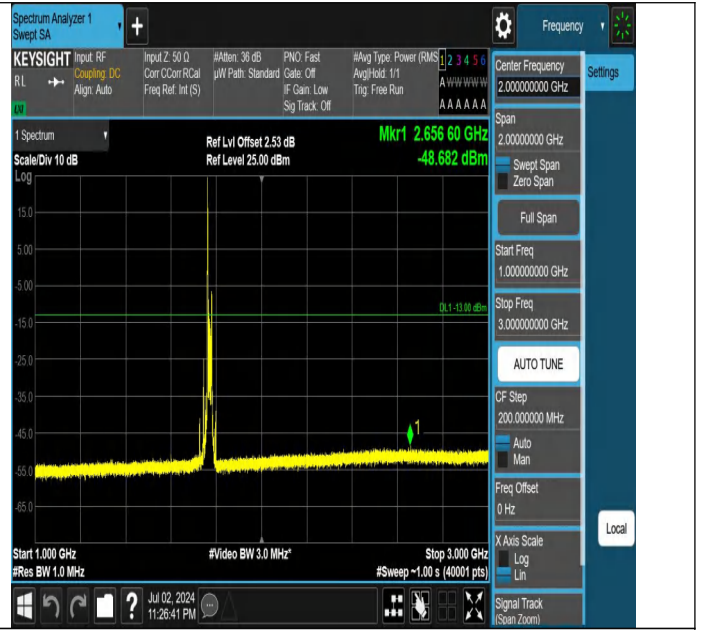
Band66-20MHz-QPSK-132572-1RB#0-1000~3000-PASS
