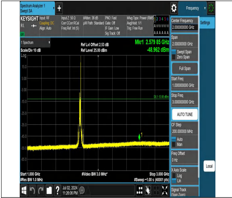
Band66-20MHz-QPSK-132322-1RB#99-1000~3000-PASS
