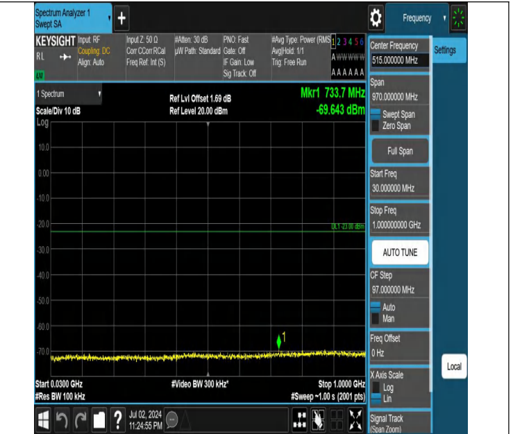
Band66-20MHz-QPSK-132072-1RB#99-30~1000-PASS
