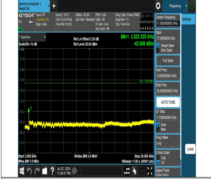
Band66-20MHz-QPSK-132572-1RB#0-3000~20000-PASS
