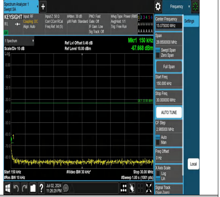
Band66-20MHz-QPSK-132572-1RB#0-0.15~30-PASS
