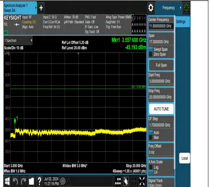
Band66-20MHz-QPSK-132572-1RB#99-3000~20000-PASS
