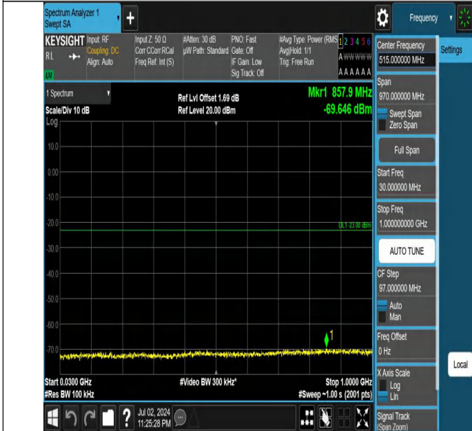
Band66-20MHz-QPSK-132322-1RB#0-30~1000-PASS
