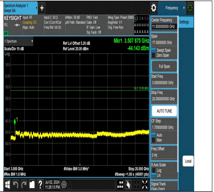
Band66-20MHz-QPSK-132322-1RB#99-3000~20000-PASS
