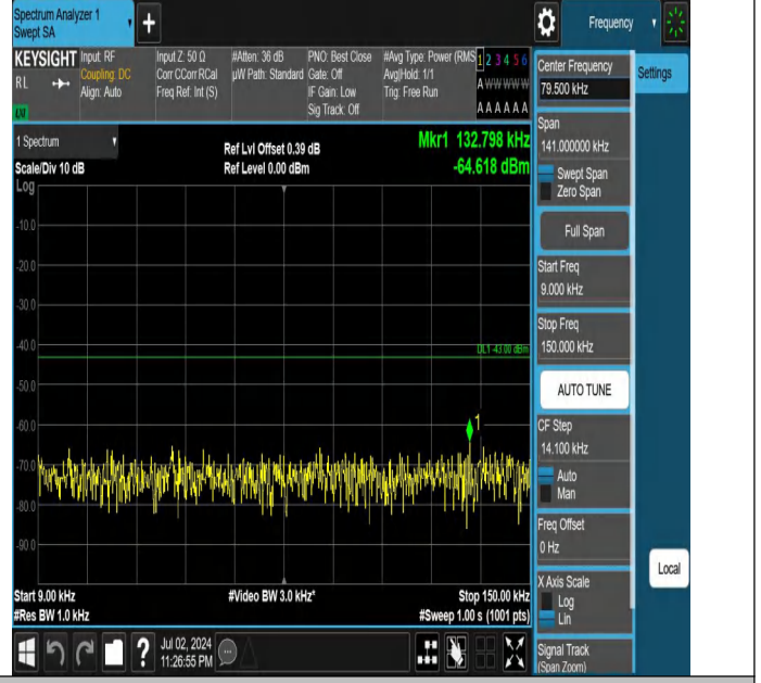
Band66-20MHz-QPSK-132572-1RB#99-0.009~0.15-PASS
