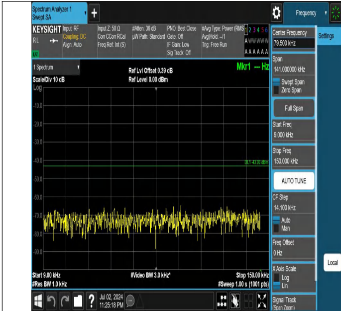
Band66-20MHz-QPSK-132322-1RB#0-0.009~0.15-PASS
