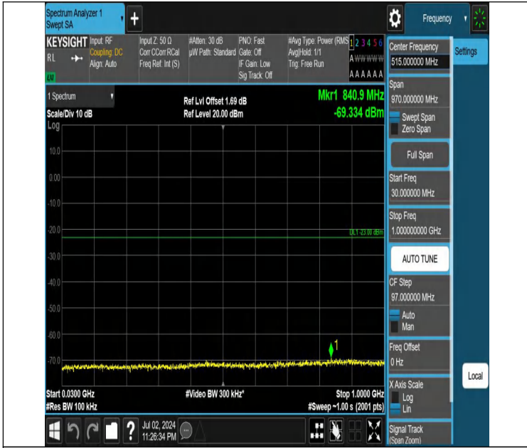
Band66-20MHz-QPSK-132572-1RB#0-30~1000-PASS
