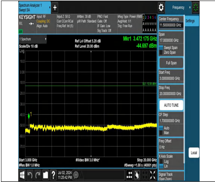
Band66-20MHz-QPSK-132322-1RB#0-3000~20000-PASS
