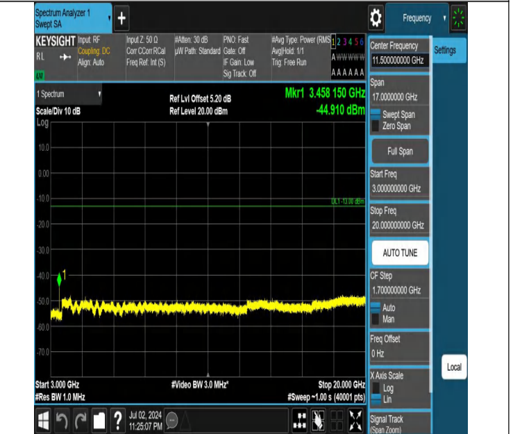
Band66-20MHz-QPSK-132072-1RB#99-3000~20000-PASS
