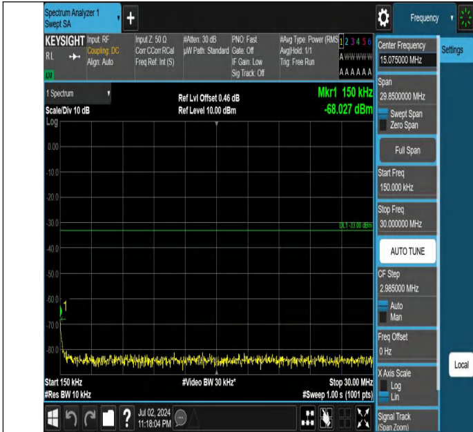
Band66-10MHz-QPSK-132022-1RB#49-0.15~30-PASS
