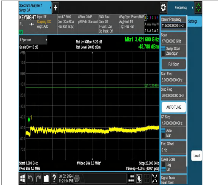
Band66-15MHz-QPSK-132047-1RB#0-3000~20000-PASS
