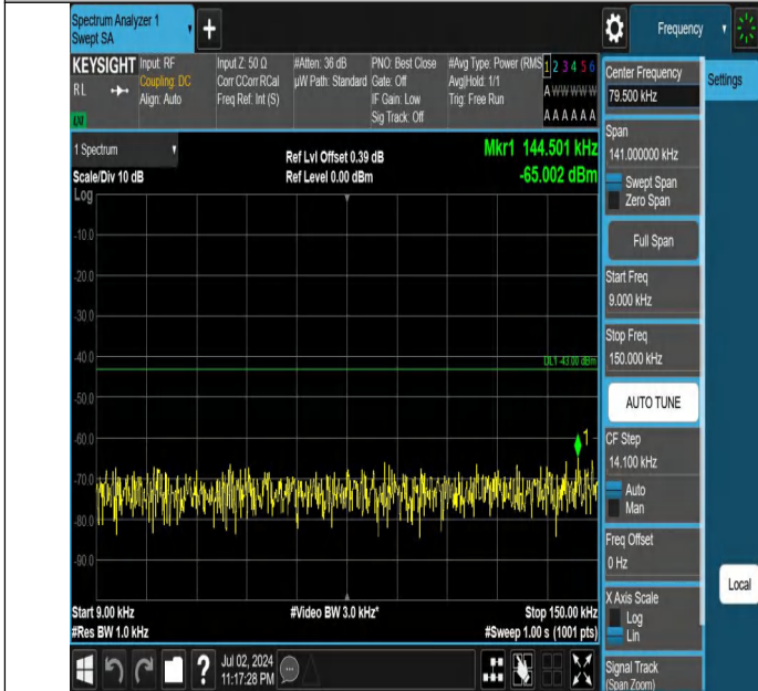
Band66-10MHz-QPSK-132022-1RB#0-0.009~0.15-PASS
