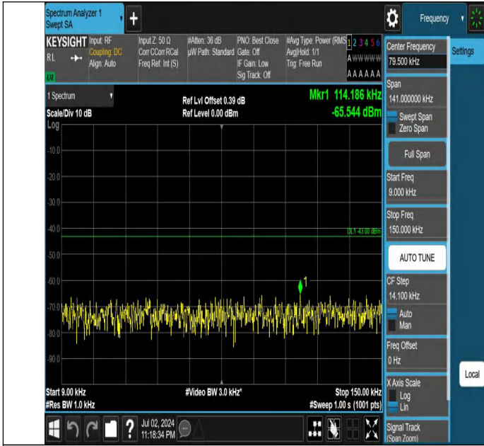
Band66-10MHz-QPSK-132322-1RB#0-0.009~0.15-PASS
