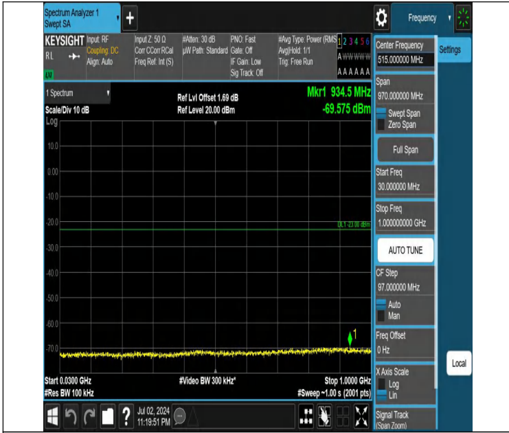
Band66-10MHz-QPSK-132622-1RB#0-30~1000-PASS
