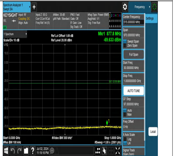
Band66-10MHz-QPSK-132322-1RB#49-30~1000-PASS
