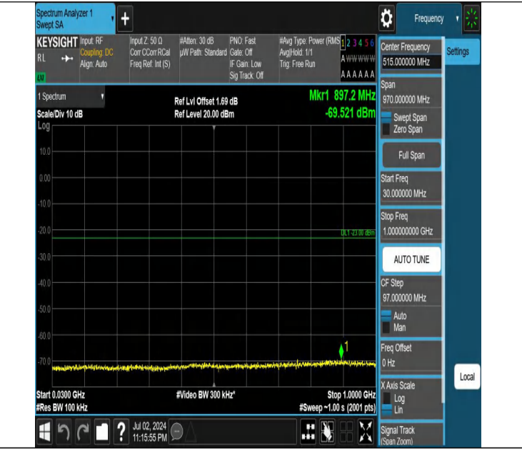
Band66-5MHz-QPSK-132322-1RB#24-30~1000-PASS
