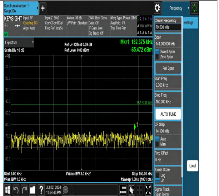
Band66-20MHz-QPSK-132072-1RB#99-0.009~0.15-PASS
