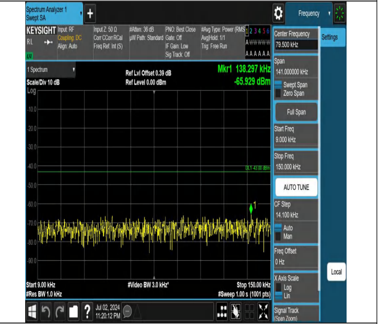
Band66-10MHz-QPSK-132622-1RB#49-0.009~0.15-PASS
