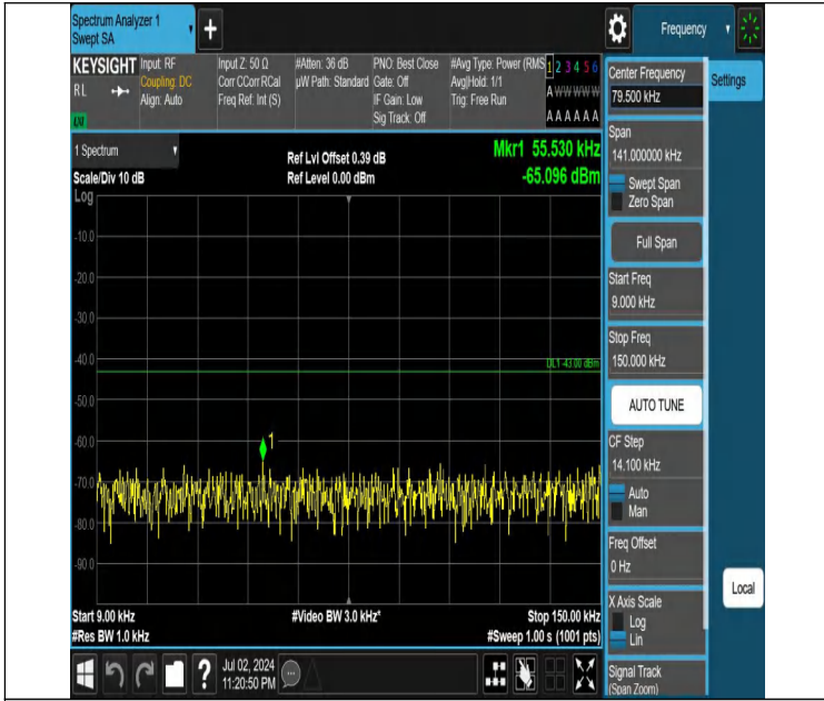
Band66-15MHz-QPSK-132047-1RB#0-0.009~0.15-PASS
