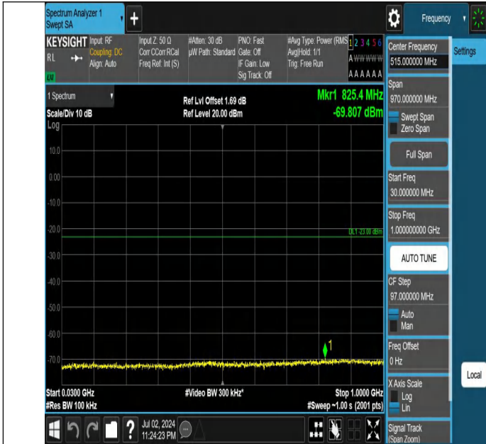
Band66-20MHz-QPSK-132072-1RB#0-30~1000-PASS
