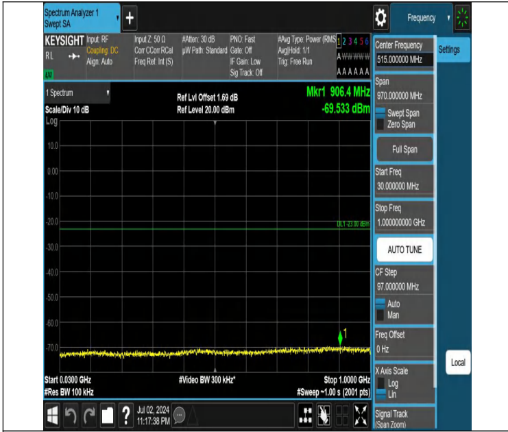
Band66-10MHz-QPSK-132022-1RB#0-30~1000-PASS
