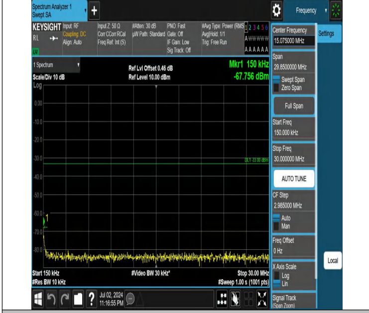
Band66-5MHz-QPSK-132647-1RB#24-0.15~30-PASS
