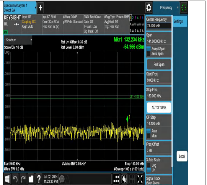
Band66-15MHz-QPSK-132597-1RB#74-0.009~0.15-PASS
