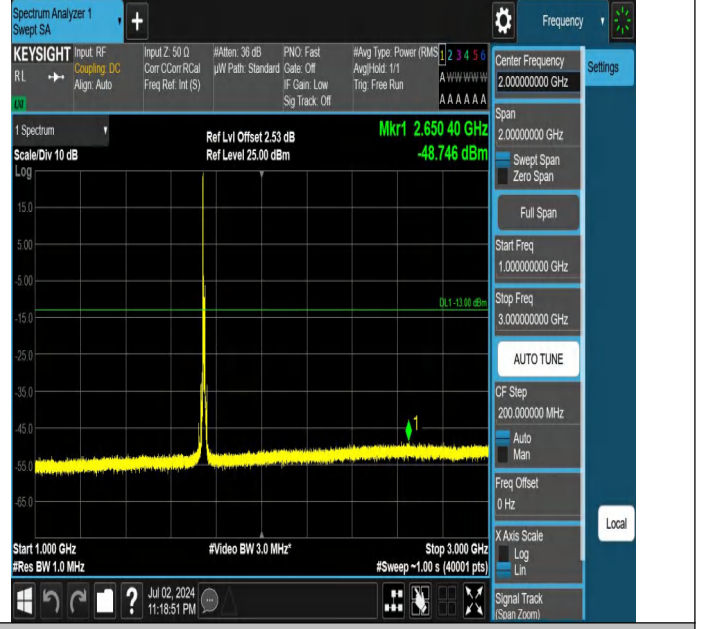
Band66-10MHz-QPSK-132322-1RB#0-1000~3000-PASS
