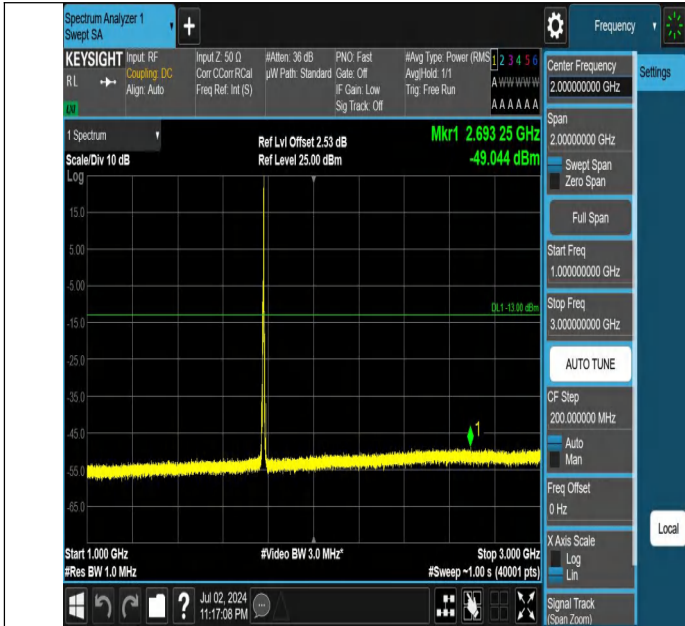
Band66-5MHz-QPSK-132647-1RB#24-1000~3000-PASS
