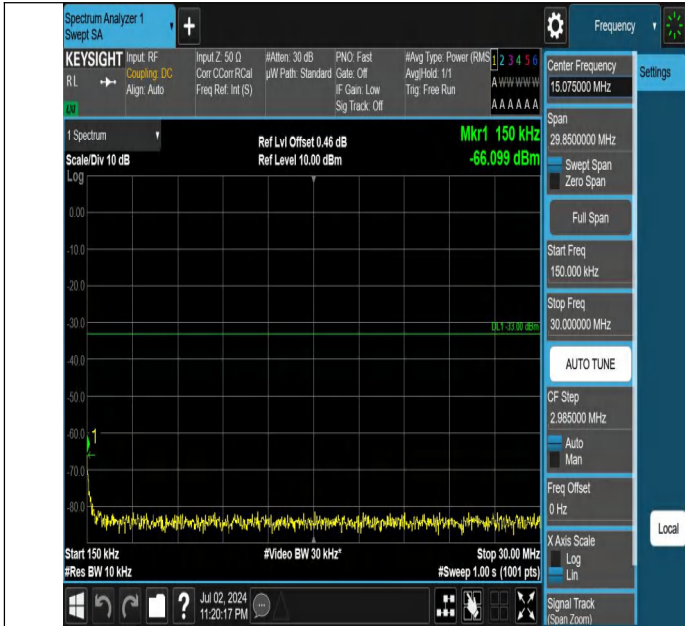
Band66-10MHz-QPSK-132622-1RB#49-0.15~30-PASS
