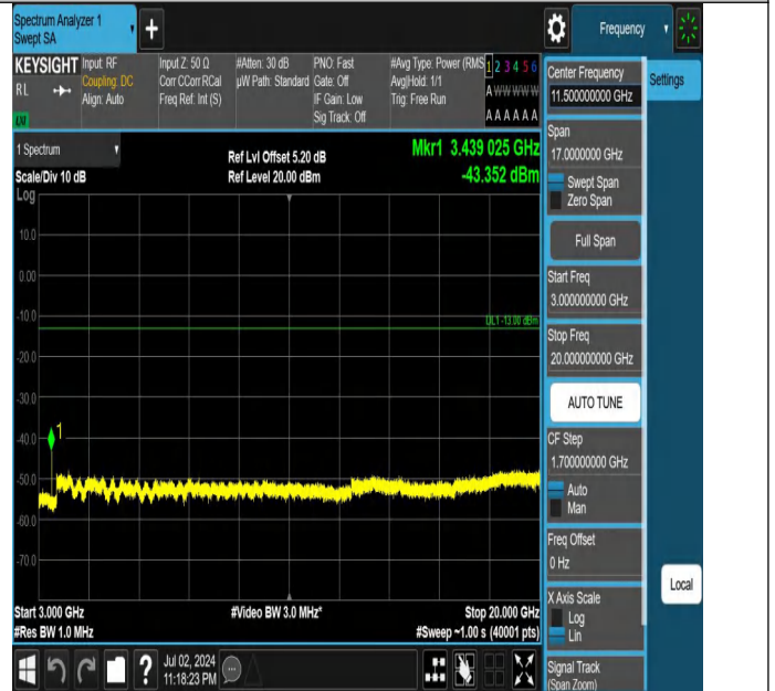
Band66-10MHz-QPSK-132022-1RB#49-3000~20000-PASS
