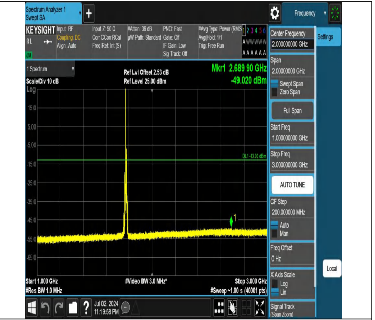
Band66-10MHz-QPSK-132622-1RB#0-1000~3000-PASS
