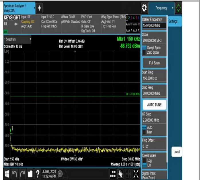
Band66-10MHz-QPSK-132622-1RB#0-0.15~30-PASS
