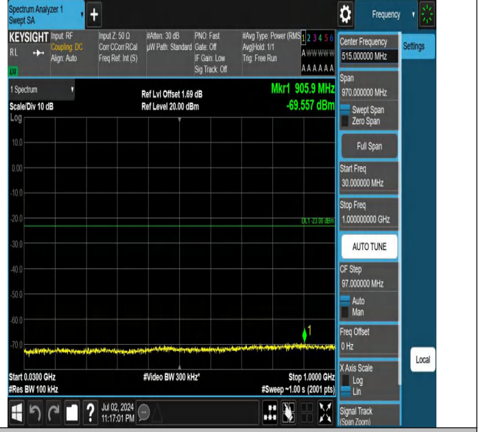
Band66-5MHz-QPSK-132647-1RB#24-30~1000-PASS
