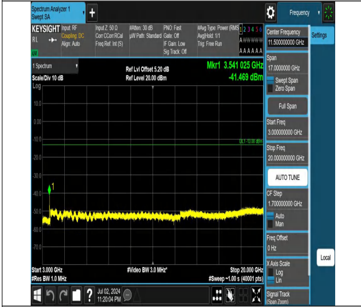
Band66-10MHz-QPSK-132622-1RB#0-3000~20000-PASS
