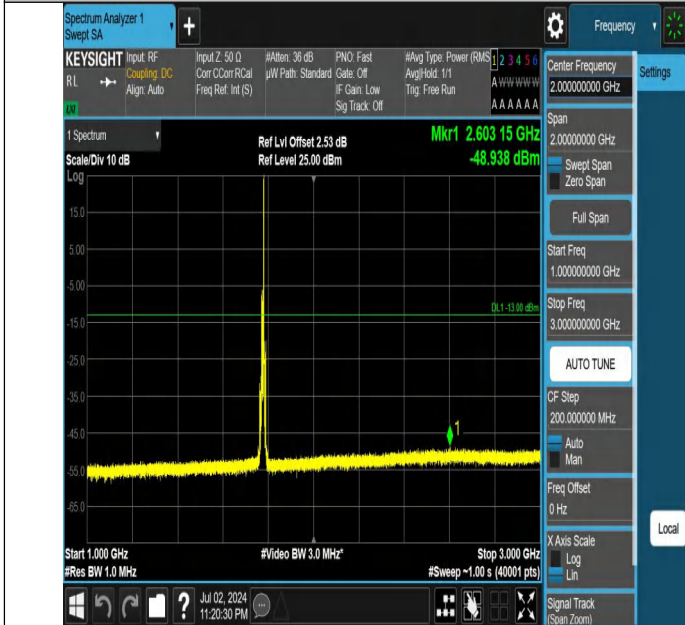
Band66-10MHz-QPSK-132622-1RB#49-1000~3000-PASS
