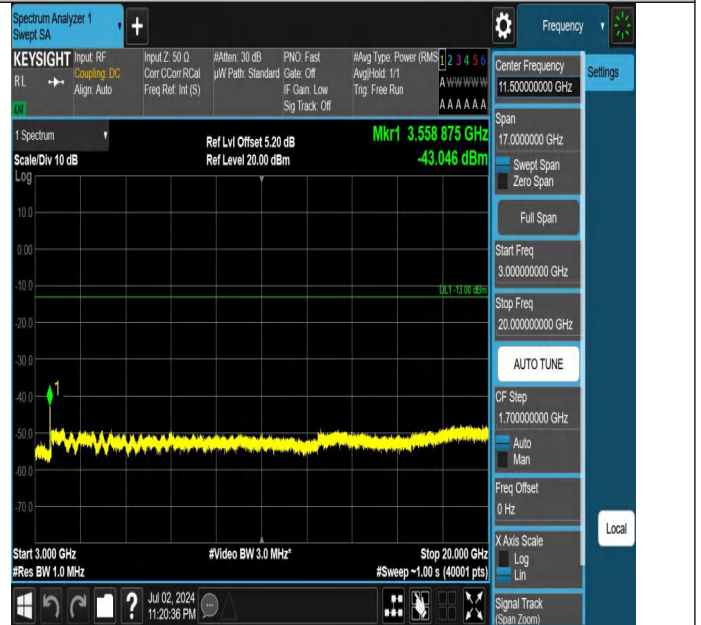
Band66-10MHz-QPSK-132622-1RB#49-3000~20000-PASS
