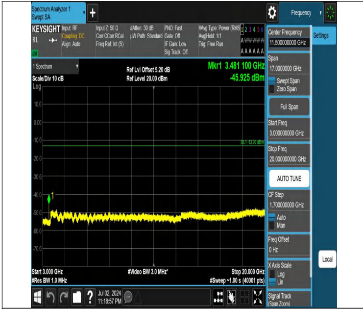
Band66-10MHz-QPSK-132322-1RB#0-3000~20000-PASS
