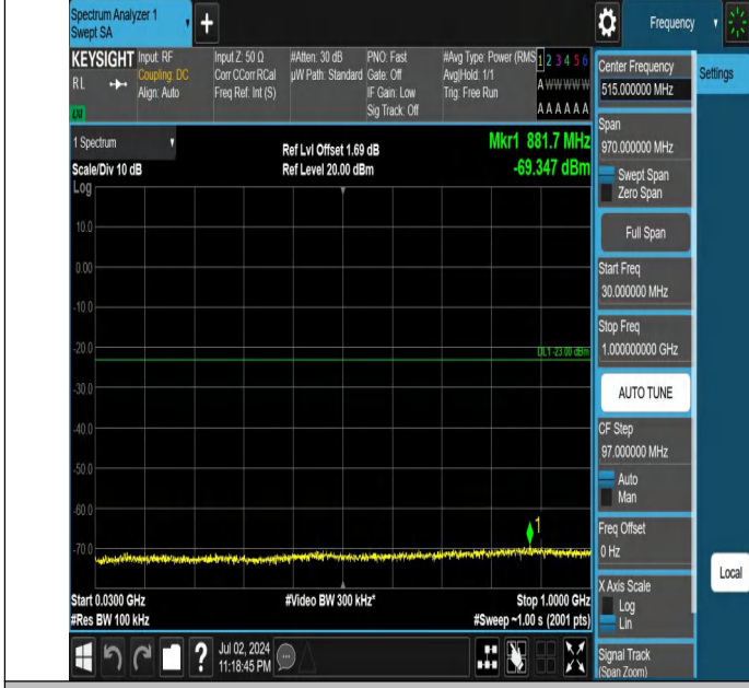
Band66-10MHz-QPSK-132322-1RB#0-30~1000-PASS
