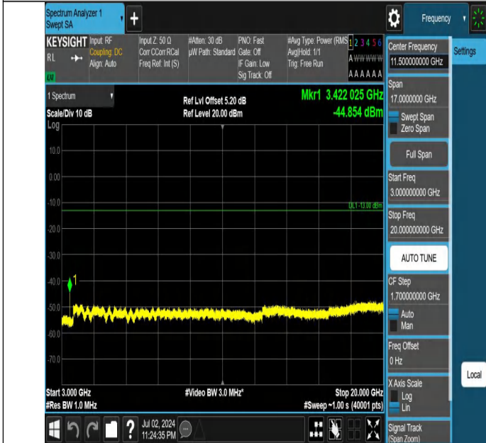
Band66-20MHz-QPSK-132072-1RB#0-3000~20000-PASS
