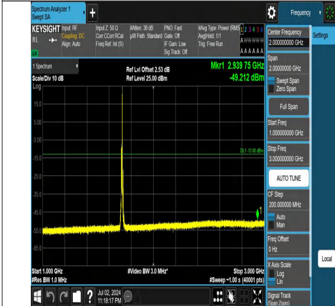
Band66-10MHz-QPSK-132022-1RB#49-1000~3000-PASS
