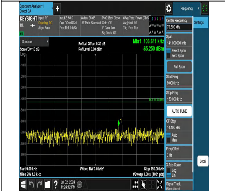
Band66-20MHz-QPSK-132072-1RB#0-0.009~0.15-PASS
