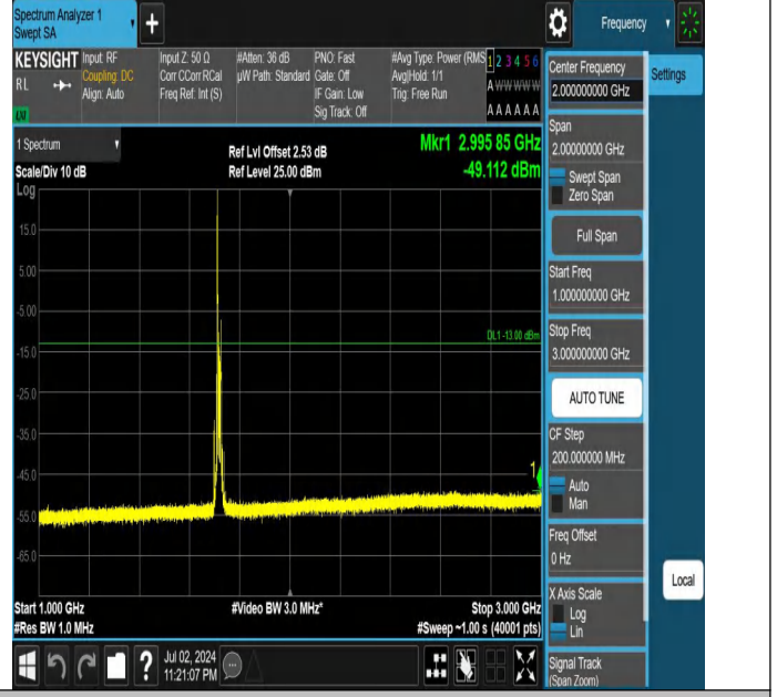
Band66-15MHz-QPSK-132047-1RB#0-1000~3000-PASS
