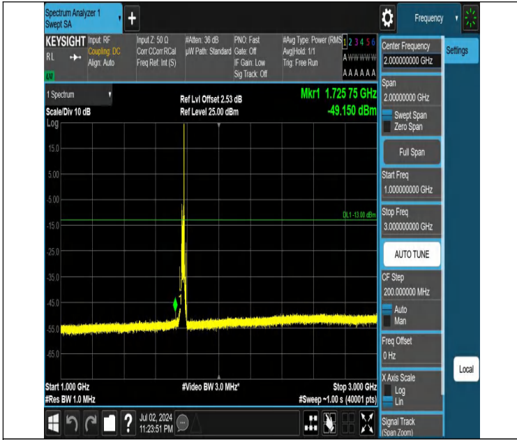
Band66-15MHz-QPSK-132597-1RB#74-1000~3000-PASS
