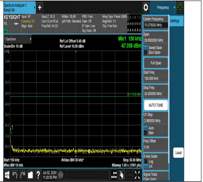
Band66-15MHz-QPSK-132047-1RB#0-0.15~30-PASS
