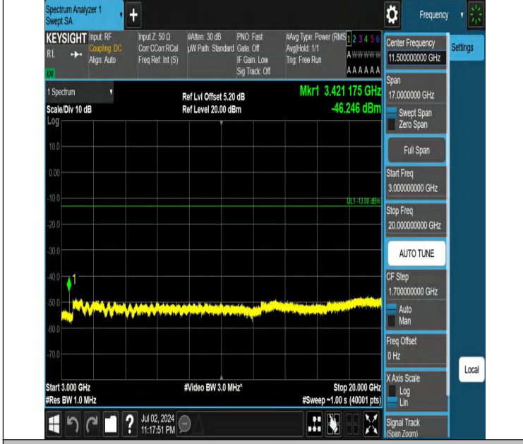
Band66-10MHz-QPSK-132022-1RB#0-3000~20000-PASS
