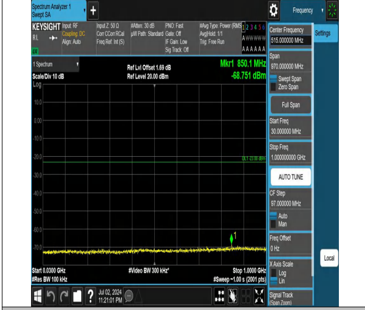
Band66-15MHz-QPSK-132047-1RB#0-30~1000-PASS
