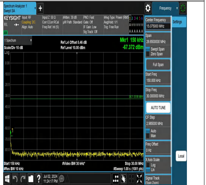
Band66-20MHz-QPSK-132072-1RB#0-0.15~30-PASS
