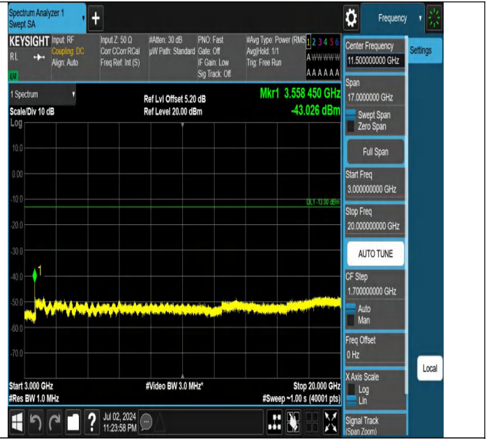
Band66-15MHz-QPSK-132597-1RB#74-3000~20000-PASS
