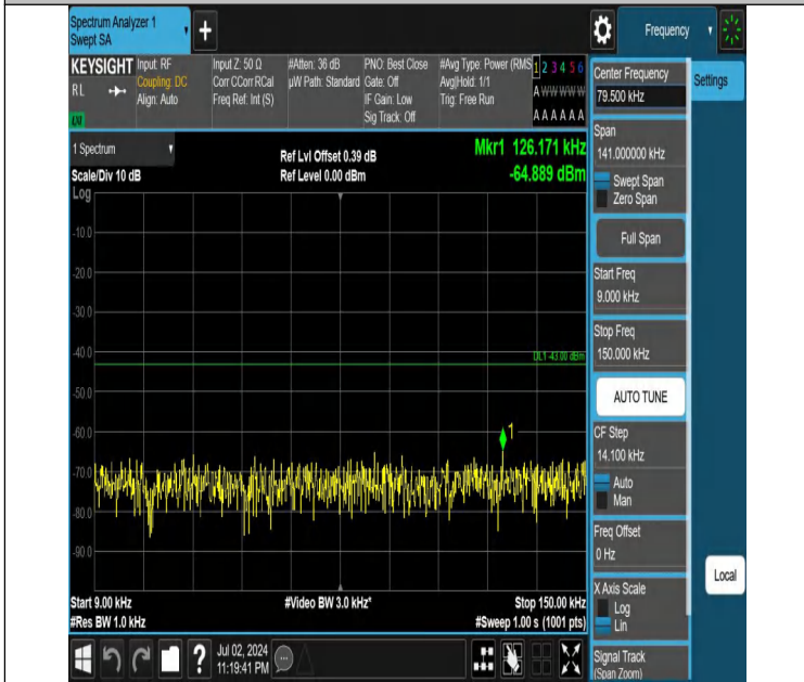
Band66-10MHz-QPSK-132622-1RB#0-0.009~0.15-PASS
