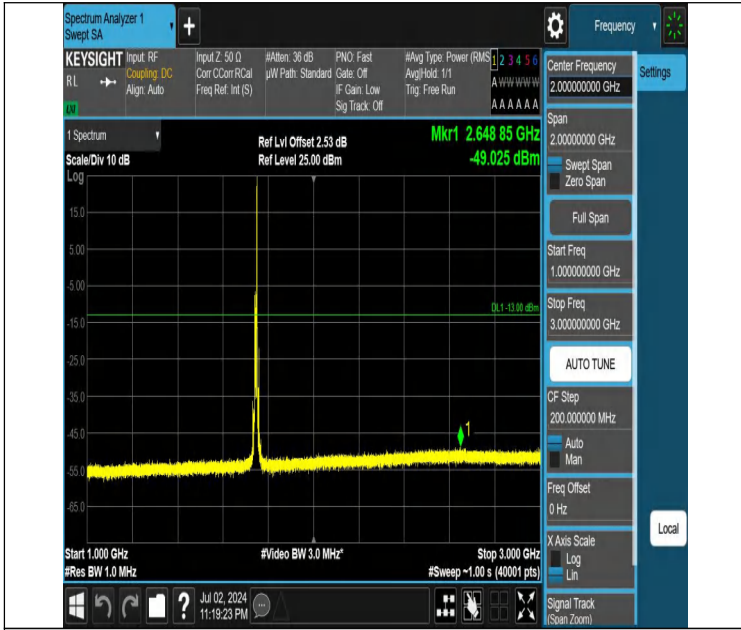
Band66-10MHz-QPSK-132322-1RB#49-1000~3000-PASS
