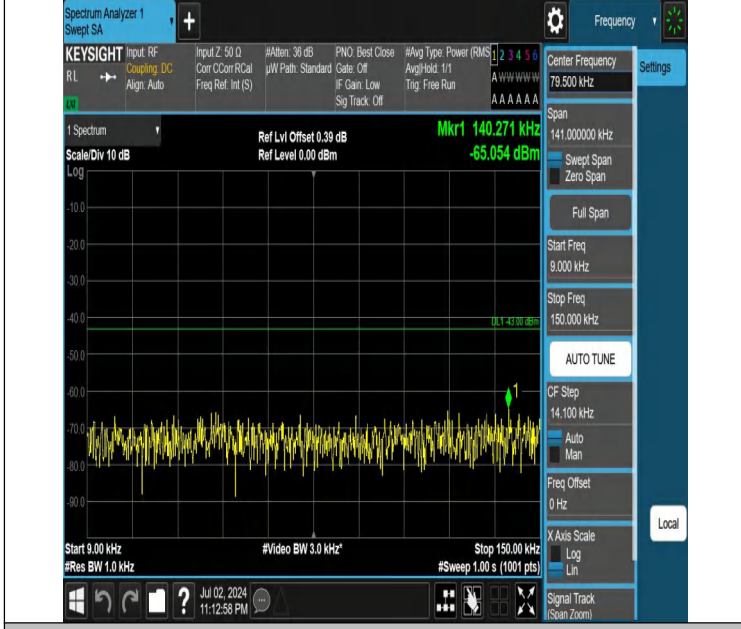
Band66-3MHz-QPSK-132657-1RB#0-0.009~0.15-PASS
