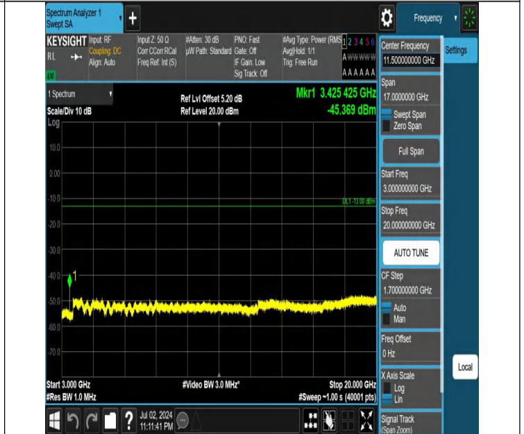
Band66-3MHz-QPSK-131987-1RB#14-3000~20000-PASS
