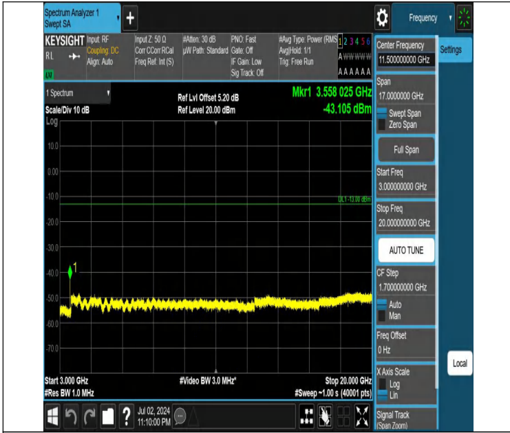
Band66-1.4MHz-QPSK-132665-1RB#0-3000~20000-PASS
