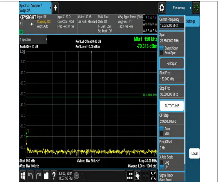
Band66-1.4MHz-QPSK-131979-1RB#0-0.15~30-PASS
