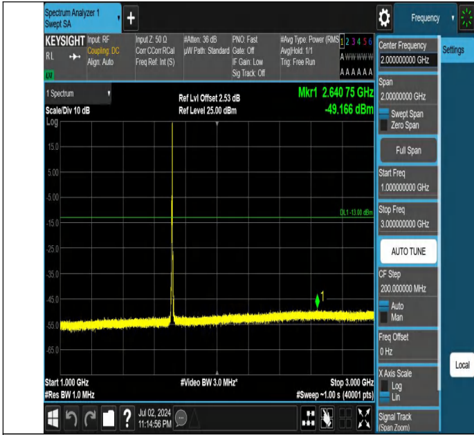
Band66-5MHz-QPSK-131997-1RB#24-1000~3000-PASS
