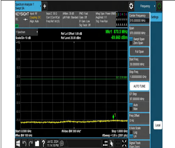
Band66-5MHz-QPSK-131997-1RB#0-30~1000-PASS
