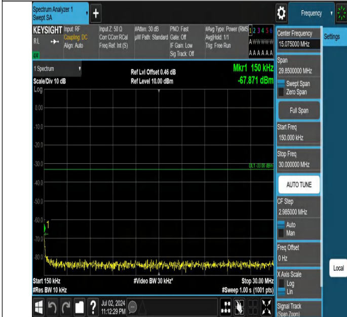
Band66-3MHz-QPSK-132322-1RB#14-0.15~30-PASS
