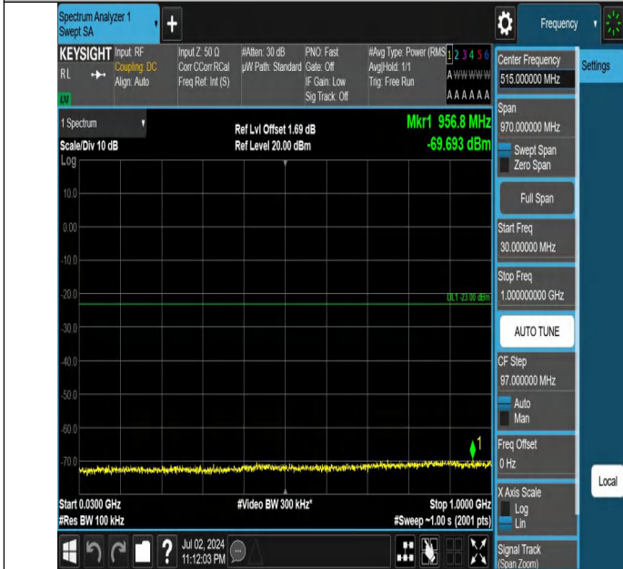
Band66-3MHz-QPSK-132322-1RB#0-30~1000-PASS
