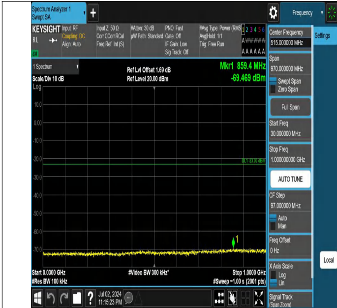
Band66-5MHz-QPSK-132322-1RB#0-30~1000-PASS
