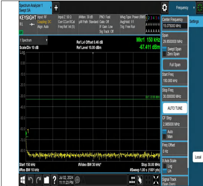
Band66-3MHz-QPSK-131987-1RB#14-0.15~30-PASS
