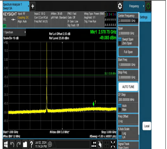
Band66-5MHz-QPSK-131997-1RB#0-1000~3000-PASS
