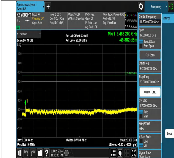
Band66-5MHz-QPSK-132322-1RB#0-3000~20000-PASS
