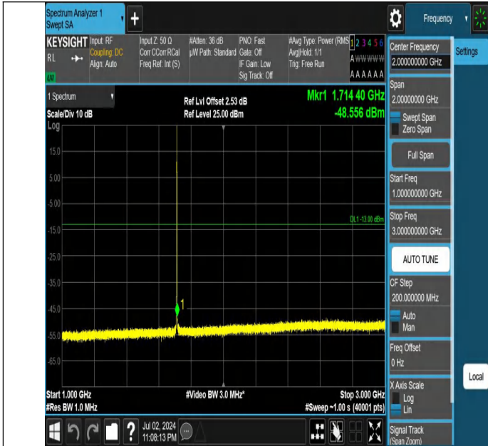
Band66-1.4MHz-QPSK-131979-1RB#5-1000~3000-PASS
