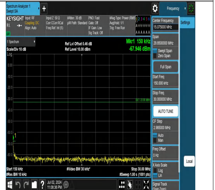
Band66-1.4MHz-QPSK-132322-1RB#0-0.15~30-PASS
