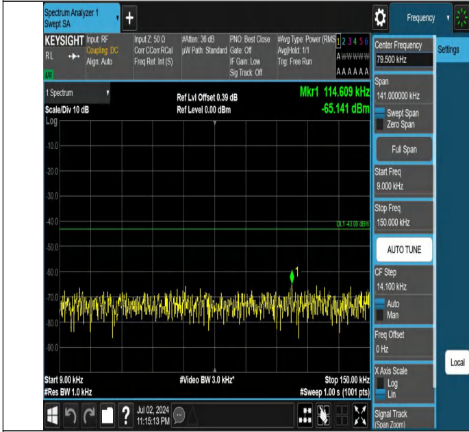
Band66-5MHz-QPSK-132322-1RB#0-0.009~0.15-PASS
