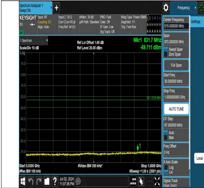
Band66-1.4MHz-QPSK-131979-1RB#0-30~1000-PASS
