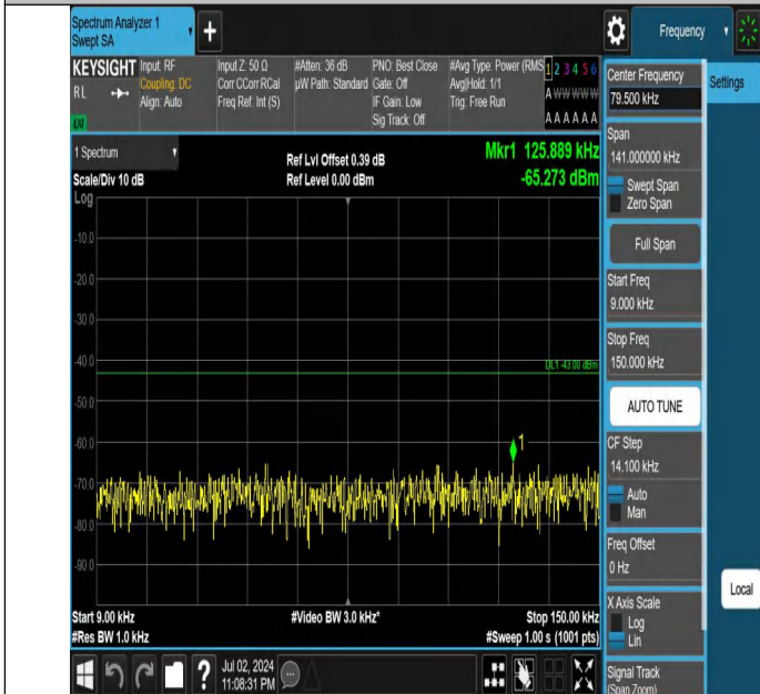
Band66-1.4MHz-QPSK-132322-1RB#0-0.009~0.15-PASS
