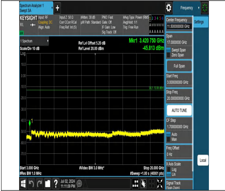
Band66-3MHz-QPSK-131987-1RB#0-3000~20000-PASS
