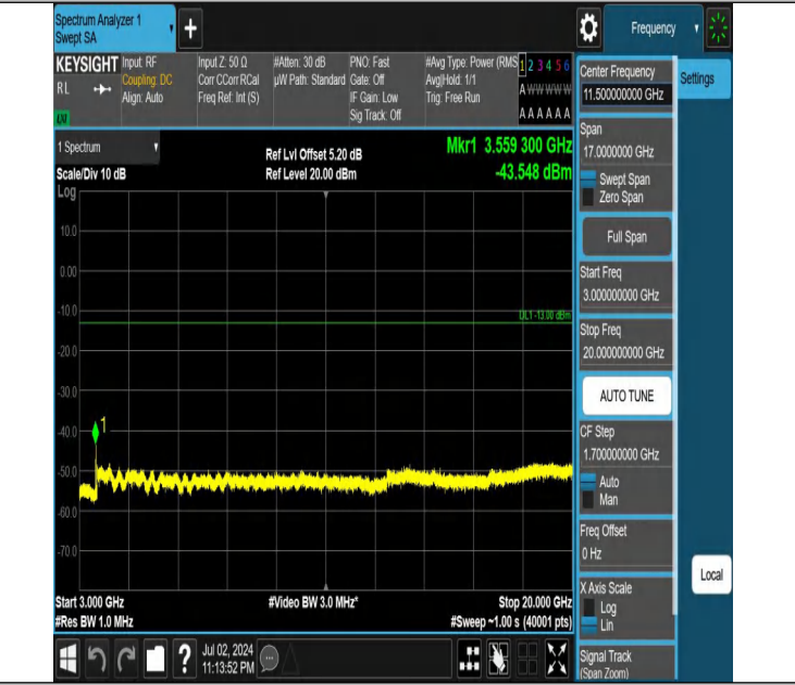
Band66-3MHz-QPSK-132657-1RB#14-3000~20000-PASS
