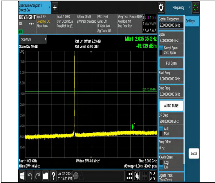
Band66-3MHz-QPSK-132322-1RB#14-1000~3000-PASS
