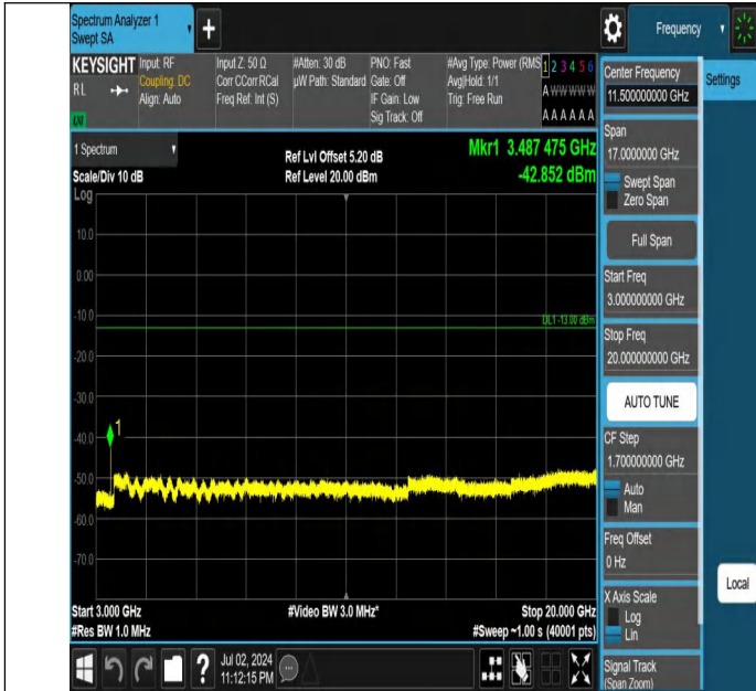
Band66-3MHz-QPSK-132322-1RB#0-3000~20000-PASS
