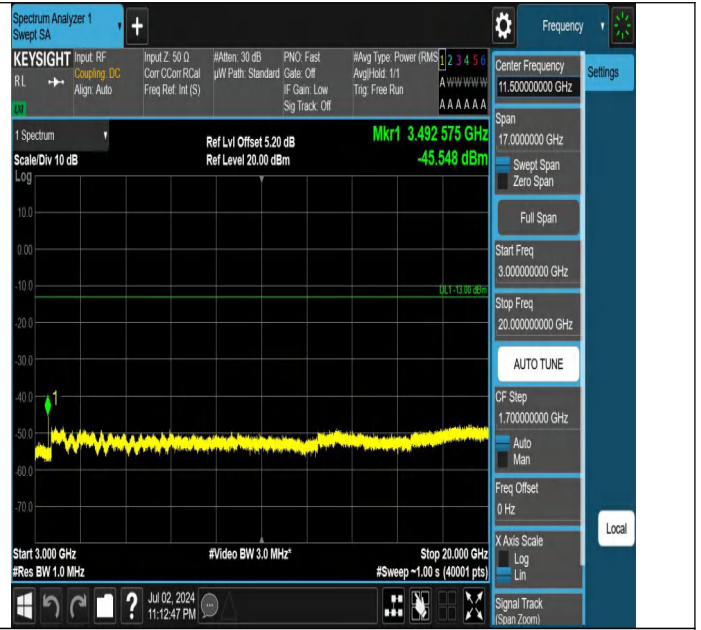
Band66-3MHz-QPSK-132322-1RB#14-3000~20000-PASS
