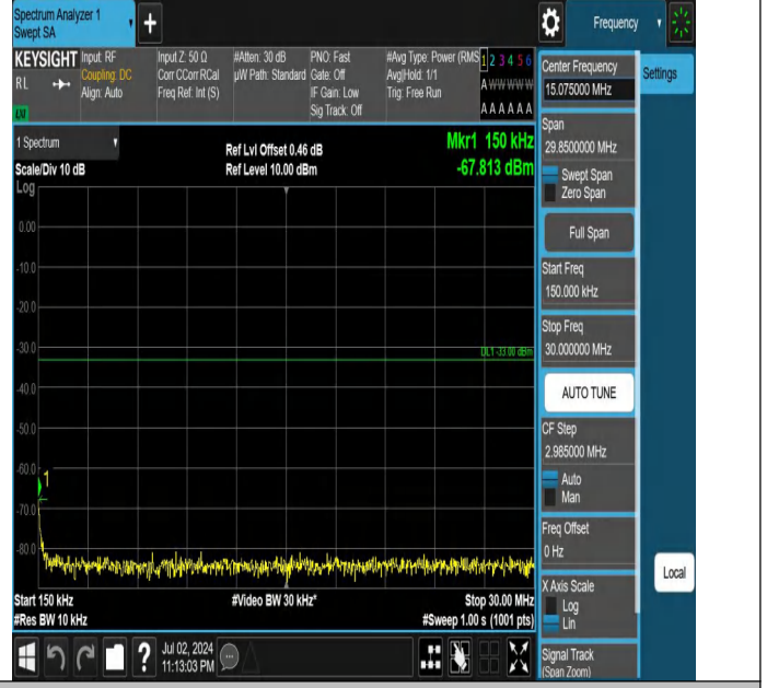
Band66-3MHz-QPSK-132657-1RB#0-0.15~30-PASS
