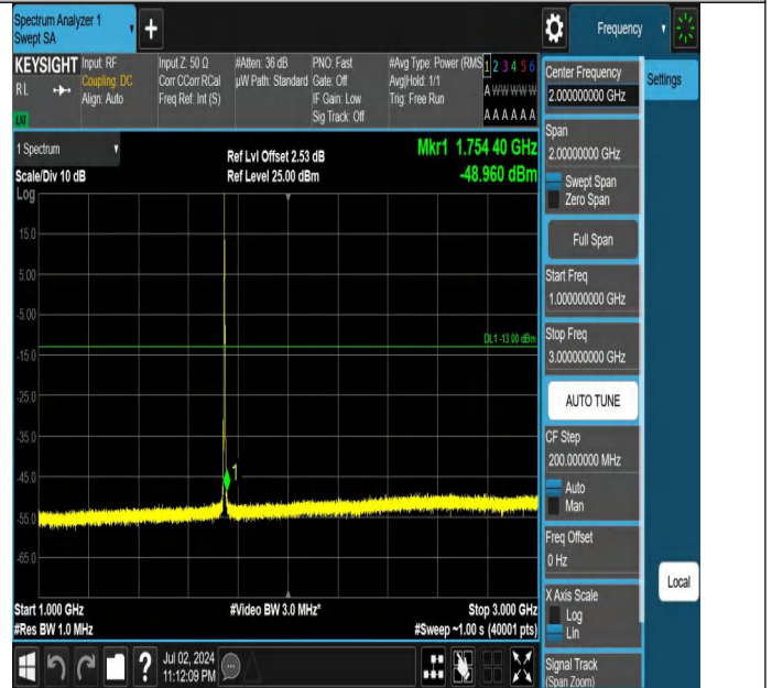
Band66-3MHz-QPSK-132322-1RB#0-1000~3000-PASS
