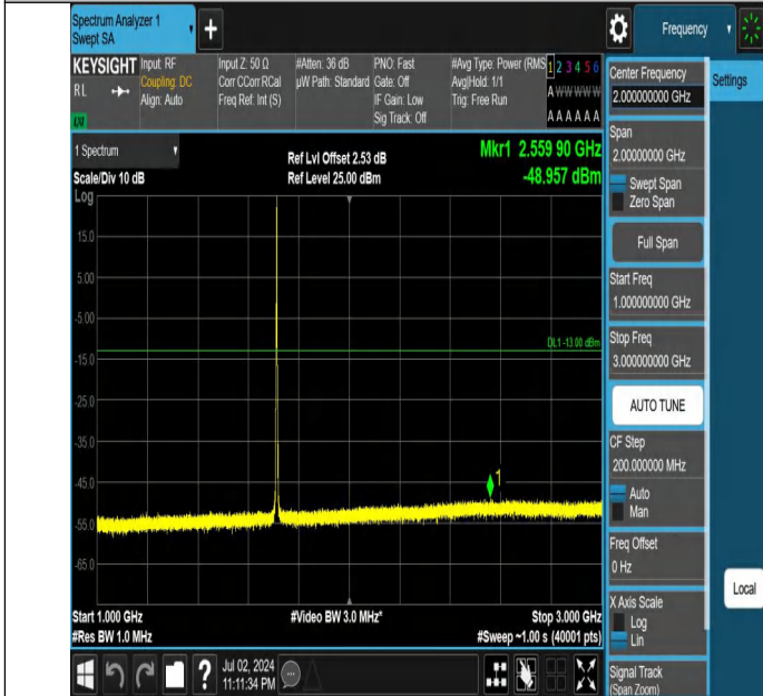
Band66-3MHz-QPSK-131987-1RB#14-1000~3000-PASS
