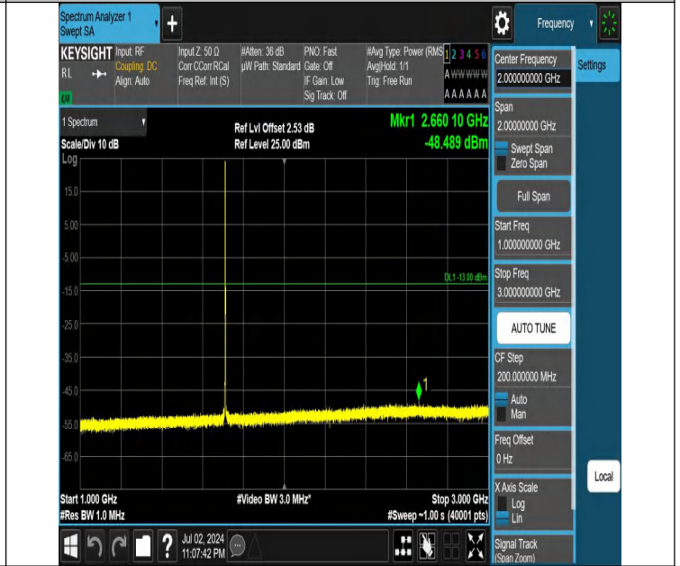
Band66-1.4MHz-QPSK-131979-1RB#0-1000~3000-PASS
