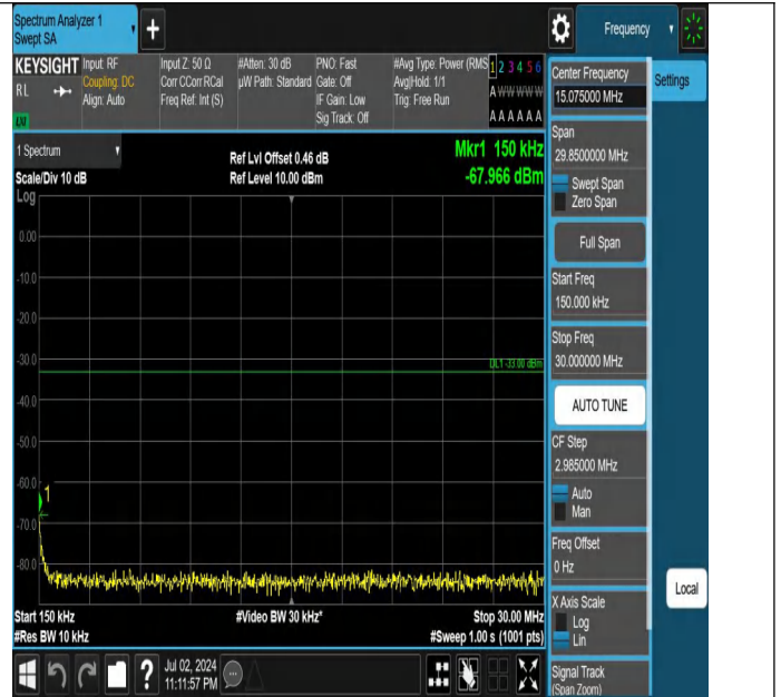
Band66-3MHz-QPSK-132322-1RB#0-0.15~30-PASS
