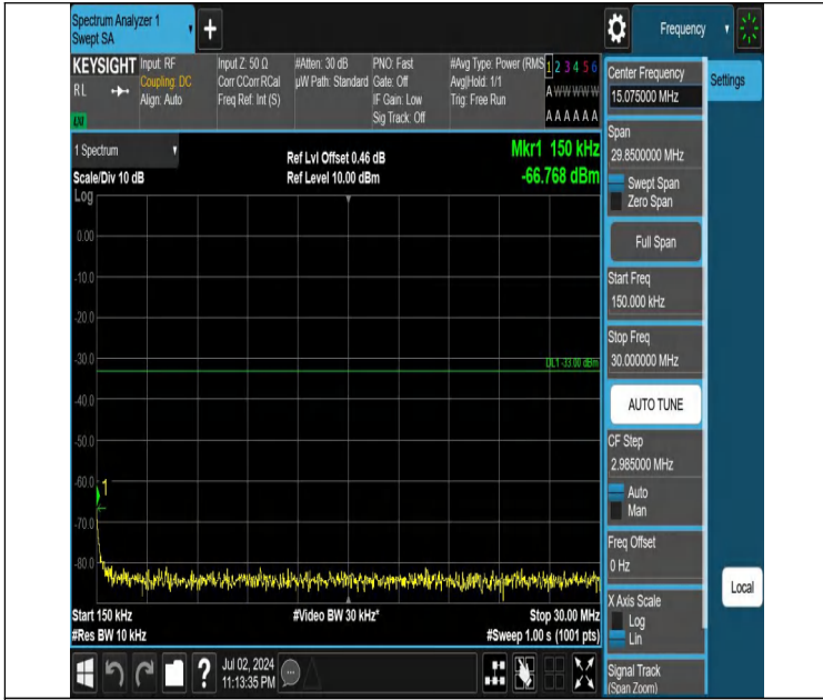
Band66-3MHz-QPSK-132657-1RB#14-0.15~30-PASS
