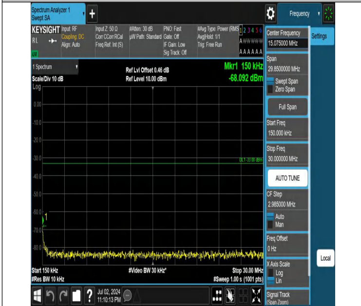
Band66-1.4MHz-QPSK-132665-1RB#5-0.15~30-PASS
