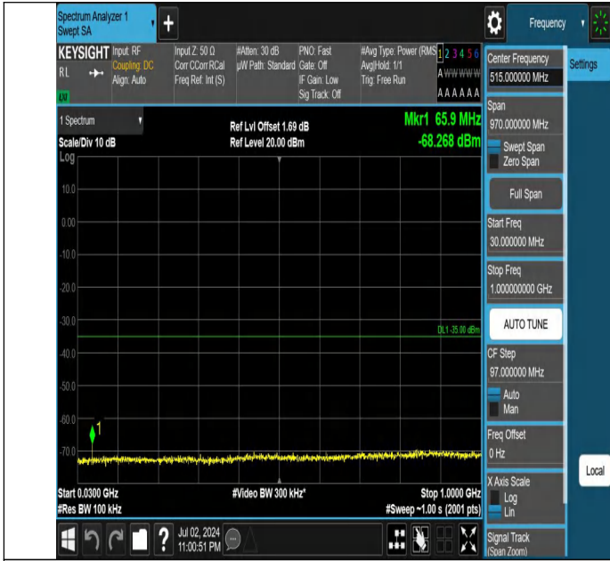
Band7-15MHz-QPSK-21100-1RB#0-30~1000-PASS
