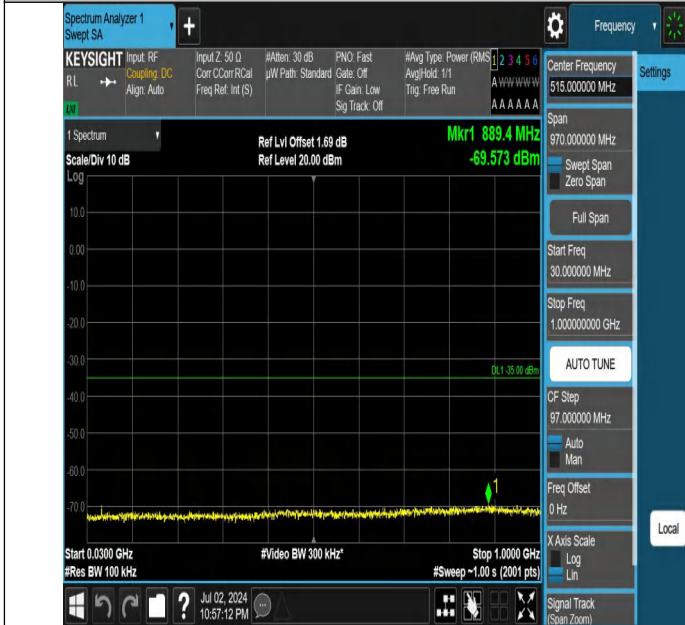
Band7-10MHz-21100-21100-1RB#0-30~1000-PASS
