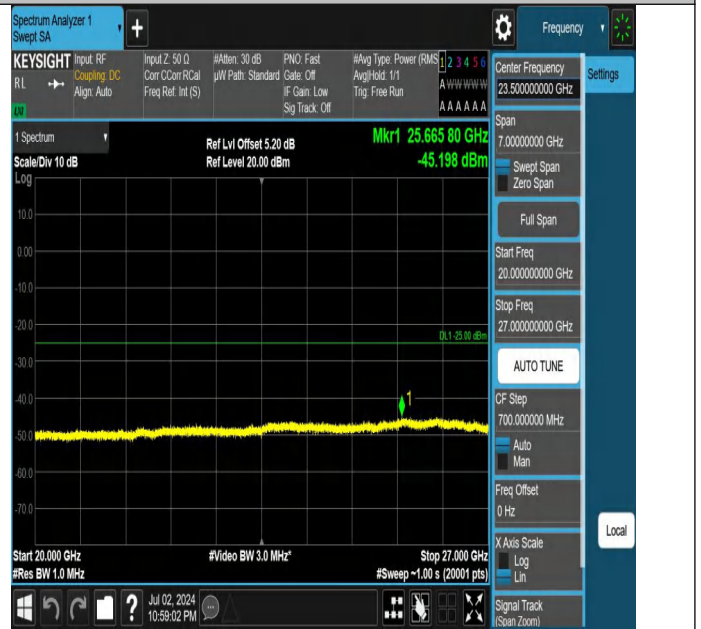
Band7-10MHz-21100-21400-1RB#49-20000~27000-PASS
