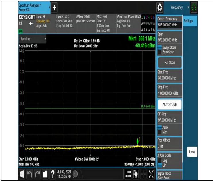
Band7-20MHz-QPSK-21350-1RB#0-30~1000-PASS
