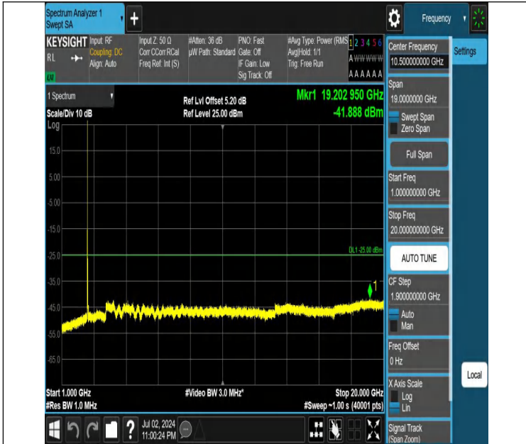
Band7-15MHz-QPSK-20825-1RB#74-1000~20000-PASS
