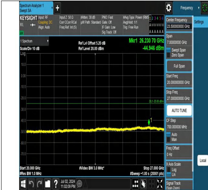
Band7-15MHz-QPSK-21375-1RB#0-20000~27000-PASS
