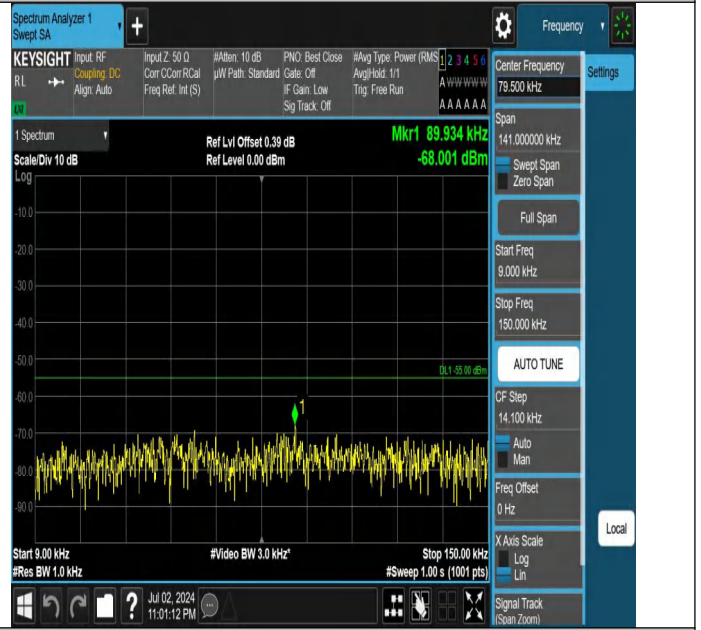
Band7-15MHz-QPSK-21100-1RB#74-0.009~0.15-PASS
