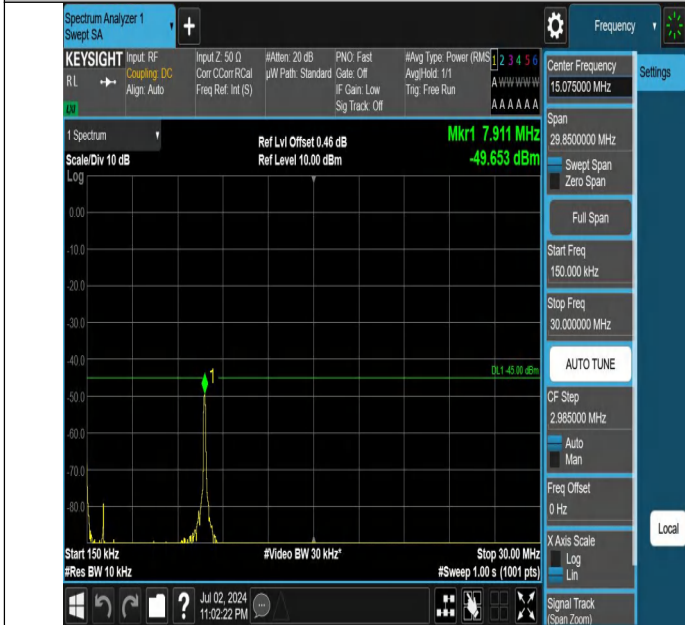
Band7-15MHz-QPSK-21375-1RB#74-0.15~30-PASS
