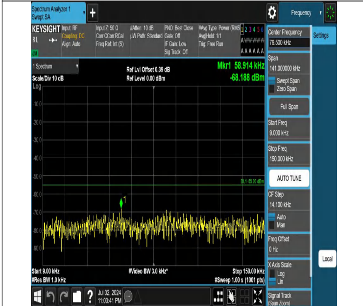
Band7-15MHz-QPSK-21100-1RB#0-0.009~0.15-PASS
