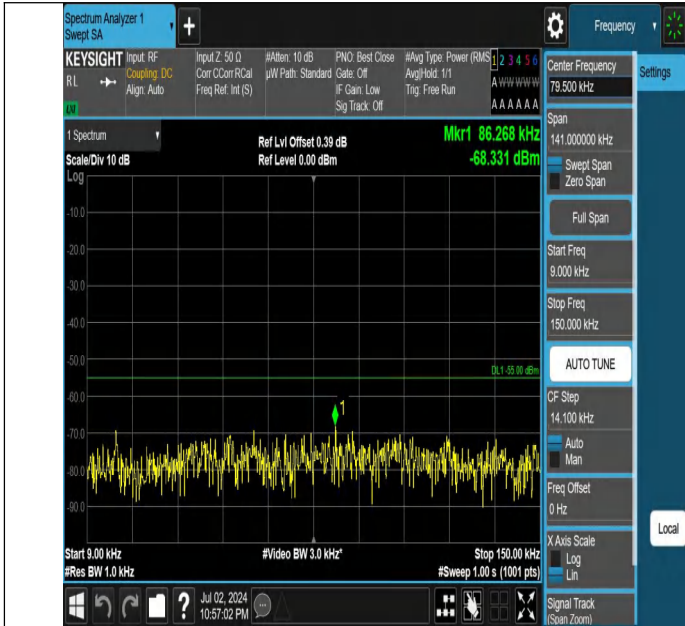
Band7-10MHz-21100-21100-1RB#0-0.009~0.15-PASS
