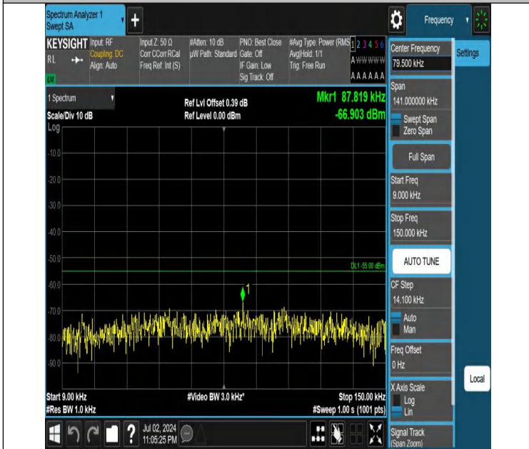
Band7-20MHz-QPSK-21350-1RB#0-0.009~0.15-PASS
