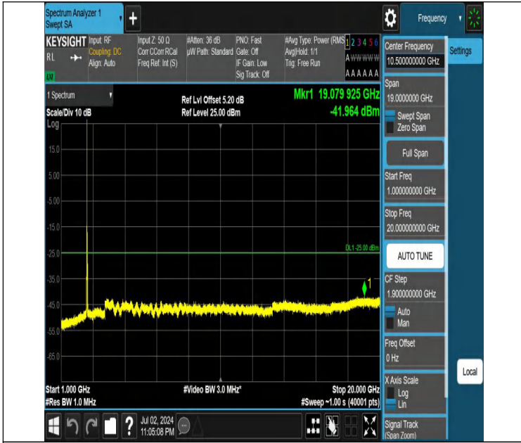
Band7-20MHz-QPSK-21100-1RB#99-1000~20000-PASS
