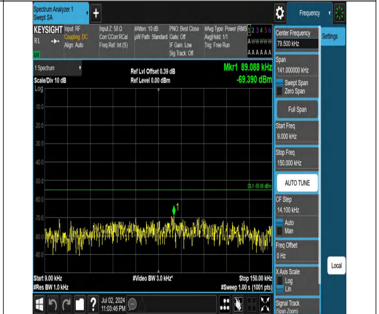
Band7-20MHz-QPSK-20850-1RB#99-0.009~0.15-PASS
