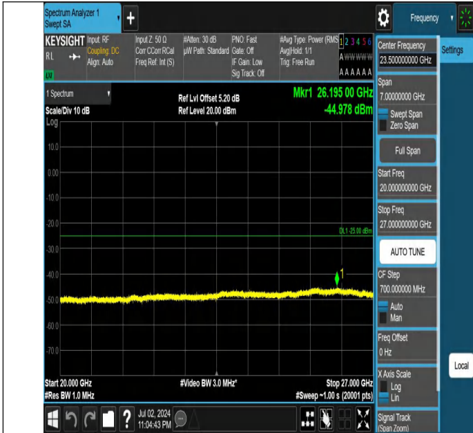
Band7-20MHz-QPSK-21100-1RB#0-20000~27000-PASS
