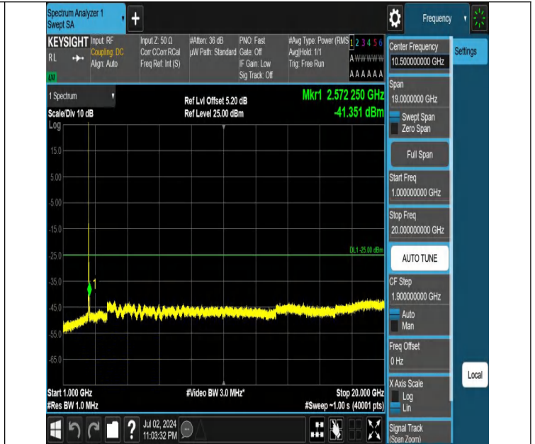
Band7-20MHz-QPSK-20850-1RB#0-1000~20000-PASS
