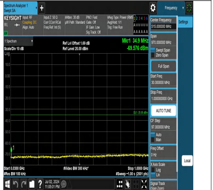
Band7-20MHz-QPSK-21100-1RB#99-30~1000-PASS
