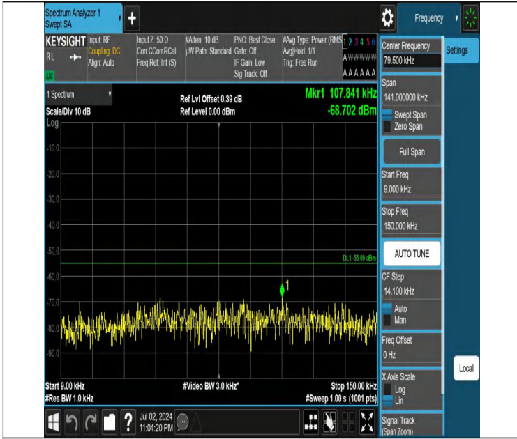
Band7-20MHz-QPSK-21100-1RB#0-0.009~0.15-PASS
