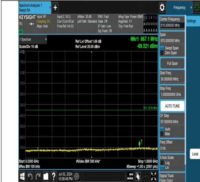
Band7-15MHz-QPSK-20825-1RB#0-30~1000-PASS
