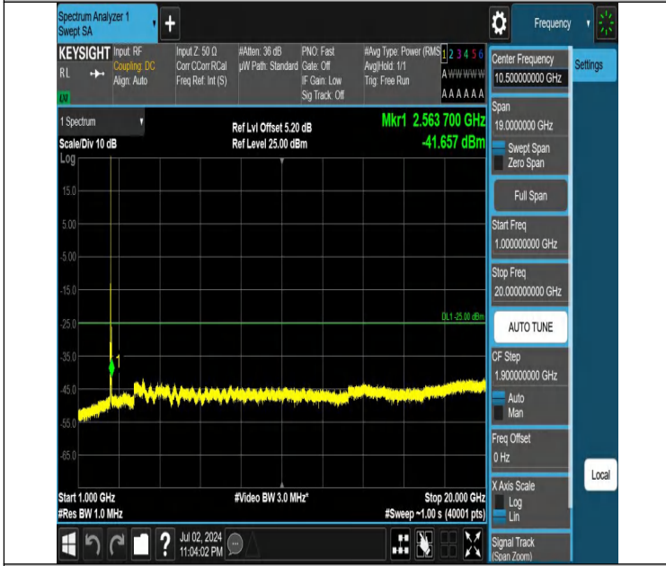
Band7-20MHz-QPSK-20850-1RB#99-1000~20000-PASS
