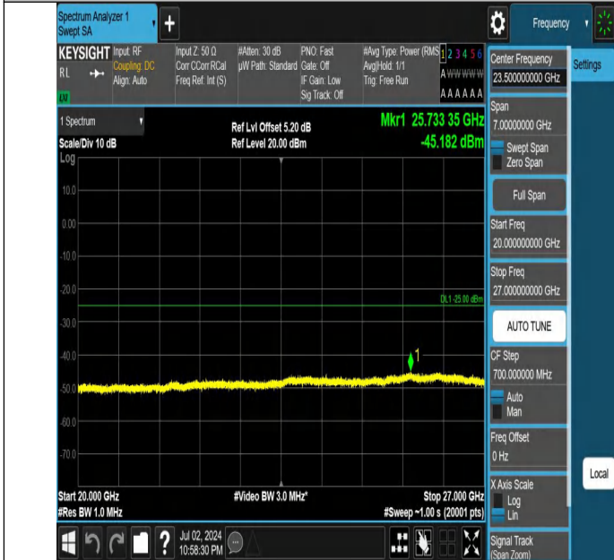
Band7-10MHz-21100-21400-1RB#0-20000~27000-PASS
