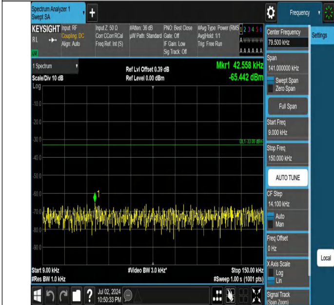
Band5-10MHz-QPSK-20600-1RB#0-0.009~0.15-PASS
