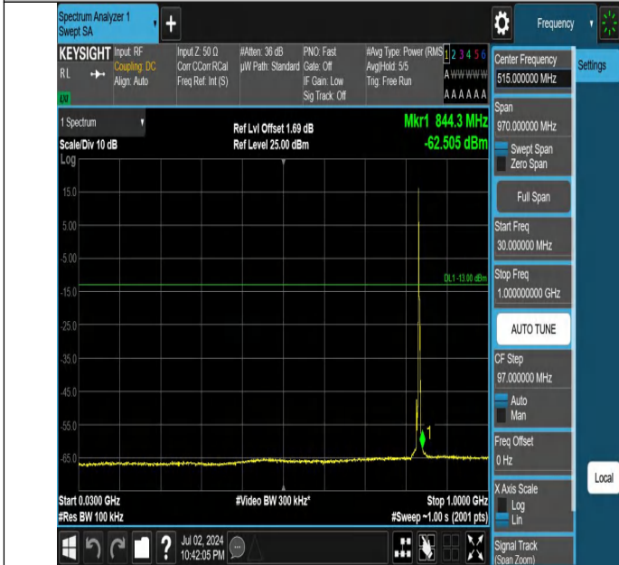
Band5-3MHz-QPSK-20525-1RB#0-30~1000-PASS
