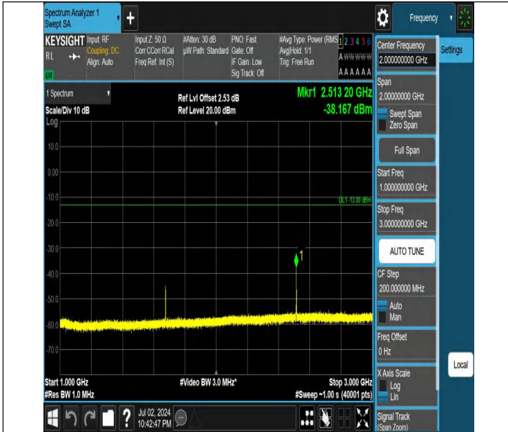
Band5-3MHz-QPSK-20525-1RB#14-1000~3000-PASS
