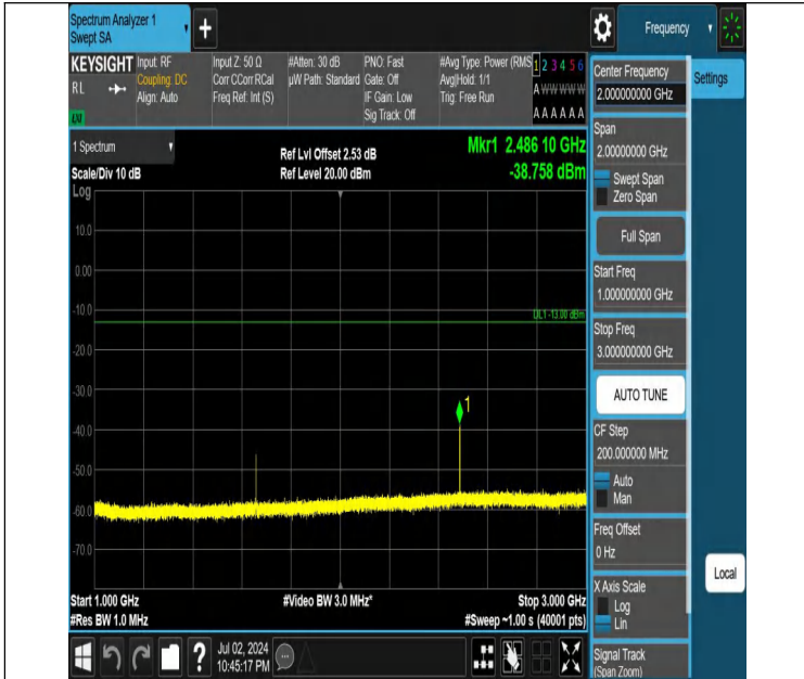
Band5-5MHz-QPSK-20425-1RB#24-1000~3000-PASS
