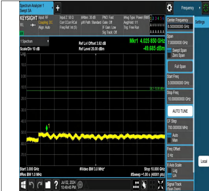
Band5-10MHz-QPSK-20525-1RB#0-3000~10000-PASS
