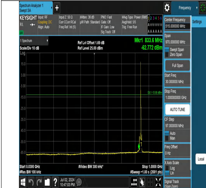
Band5-5MHz-QPSK-20625-1RB#0-30~1000-PASS
