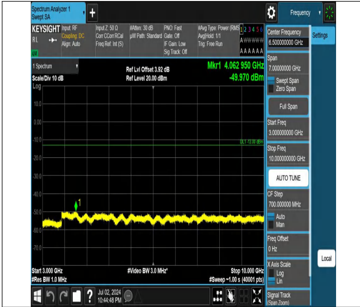
Band5-5MHz-QPSK-20425-1RB#0-3000~10000-PASS
