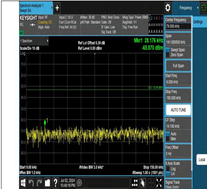
Band5-10MHz-QPSK-20525-1RB#0-0.009~0.15-PASS
