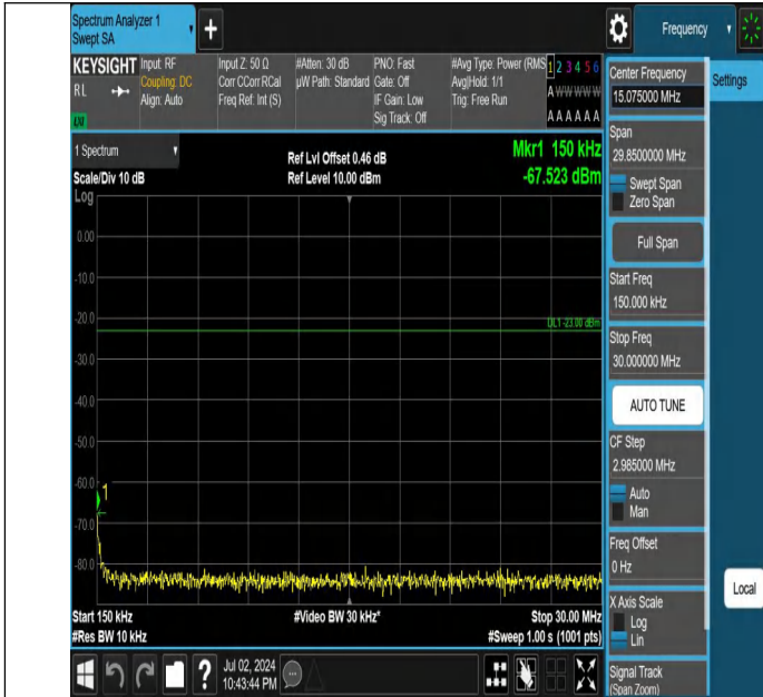
Band5-3MHz-QPSK-20635-1RB#14-0.15~30-PASS
