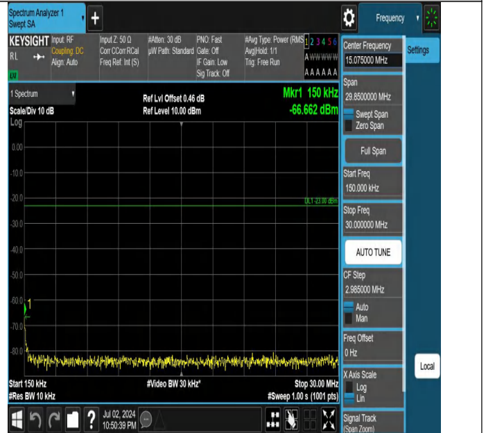
Band5-10MHz-QPSK-20600-1RB#0-0.15~30-PASS
