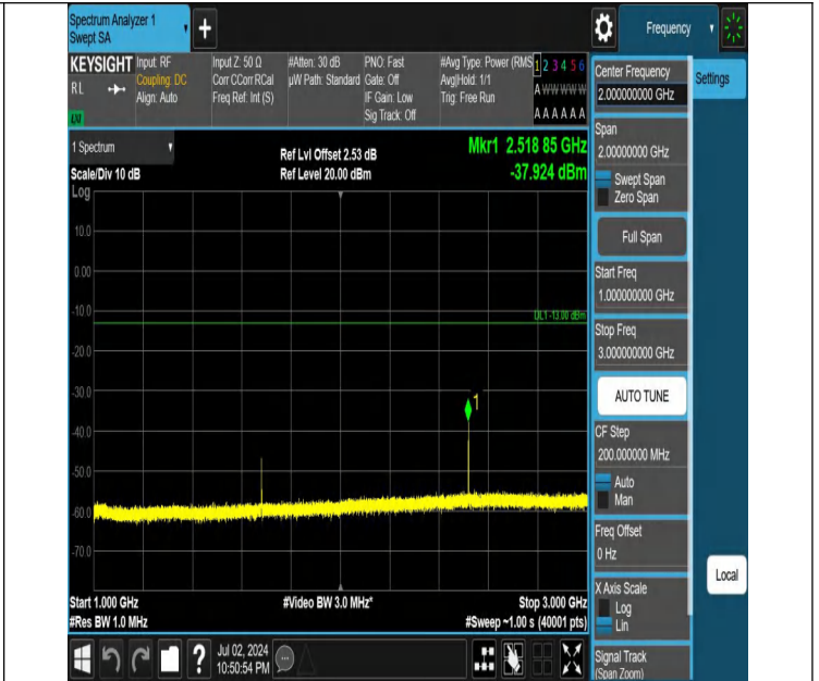
Band5-10MHz-QPSK-20600-1RB#0-1000~3000-PASS
