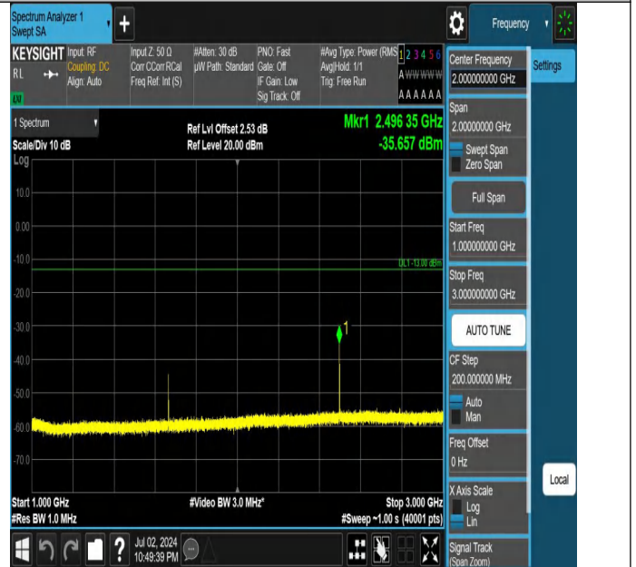
Band5-10MHz-QPSK-20525-1RB#0-1000~3000-PASS
