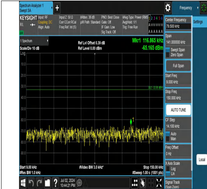
Band5-5MHz-QPSK-20425-1RB#0-0.009~0.15-PASS
