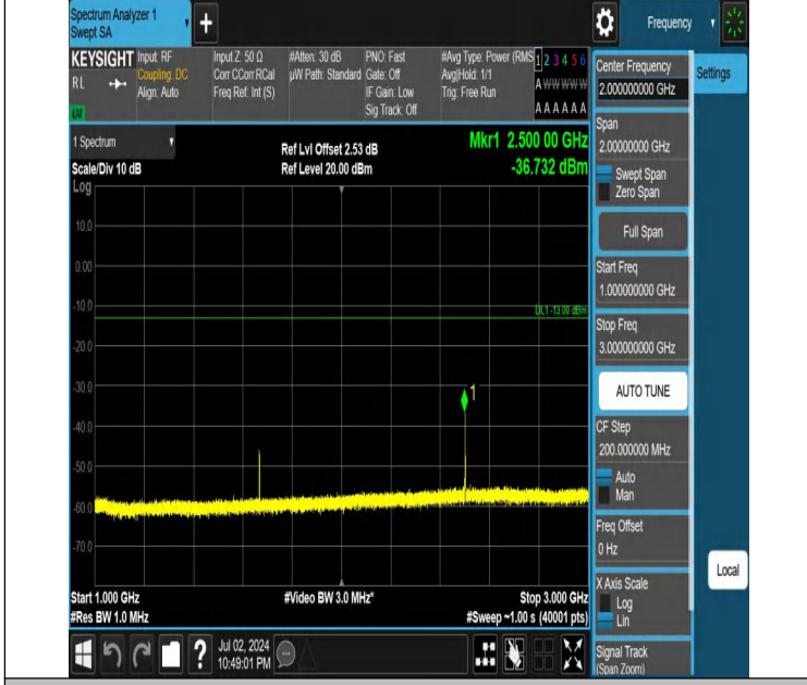
Band5-10MHz-QPSK-20450-1RB#49-1000~3000-PASS
