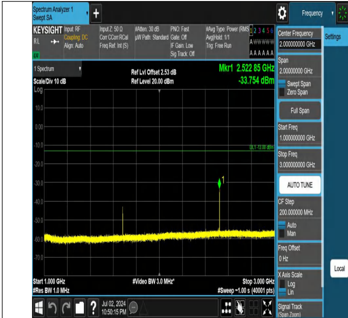
Band5-10MHz-QPSK-20525-1RB#49-1000~3000-PASS
