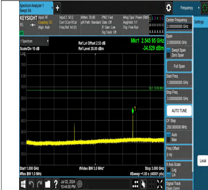
Band5-3MHz-QPSK-20635-1RB#14-1000~3000-PASS
