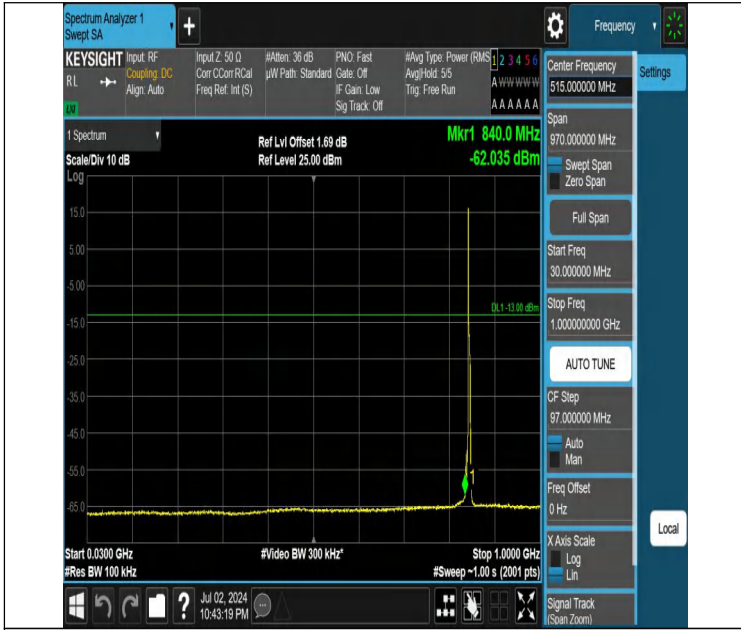
Band5-3MHz-QPSK-20635-1RB#0-30~1000-PASS
