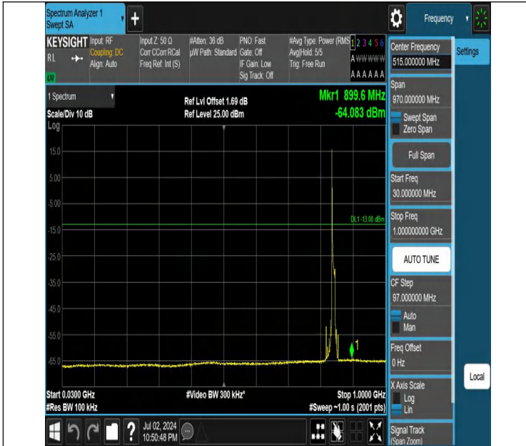
Band5-10MHz-QPSK-20600-1RB#0-30~1000-PASS
