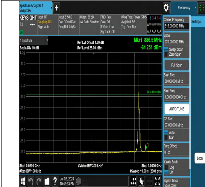
Band5-10MHz-QPSK-20525-1RB#0-30~1000-PASS
