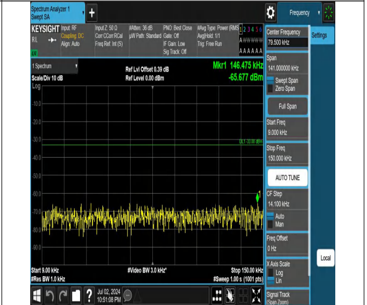
Band5-10MHz-QPSK-20600-1RB#49-0.009~0.15-PASS
