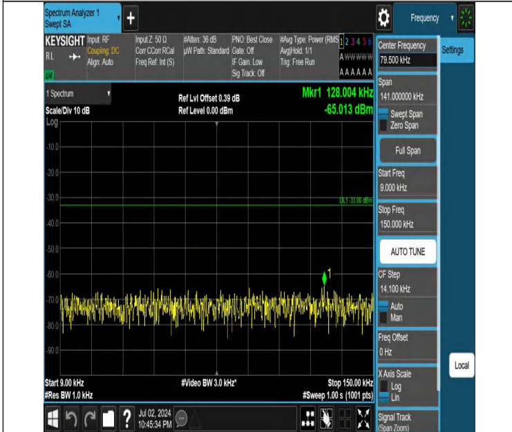
Band5-5MHz-QPSK-20525-1RB#0-0.009~0.15-PASS
