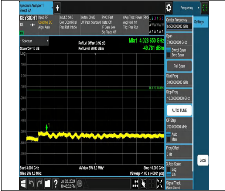
Band5-10MHz-QPSK-20450-1RB#0-3000~10000-PASS
