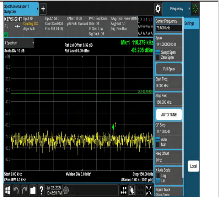
Band5-3MHz-QPSK-20635-1RB#14-0.009~0.15-PASS
