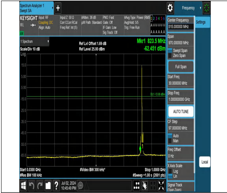
Band5-5MHz-QPSK-20525-1RB#0-30~1000-PASS
