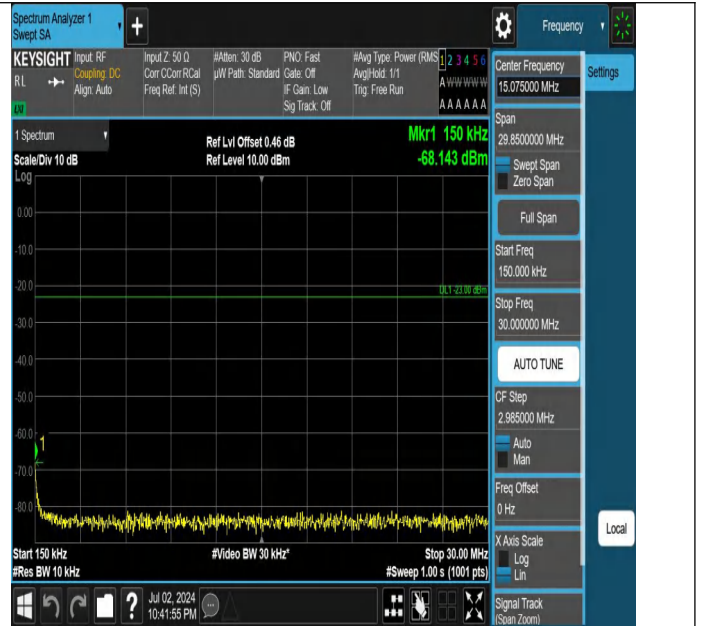
Band5-3MHz-QPSK-20525-1RB#0-0.15~30-PASS
