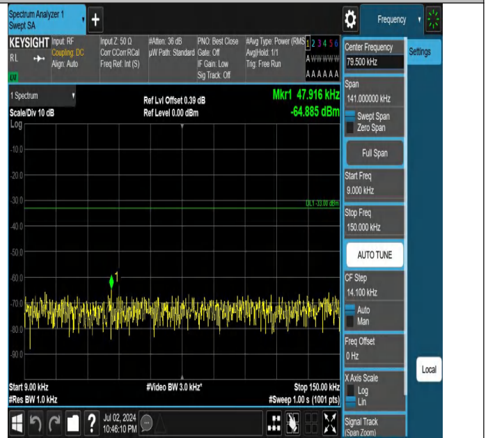
Band5-5MHz-QPSK-20525-1RB#24-0.009~0.15-PASS
