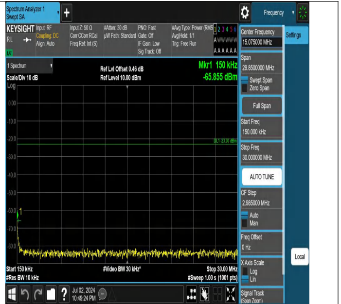
Band5-10MHz-QPSK-20525-1RB#0-0.15~30-PASS
