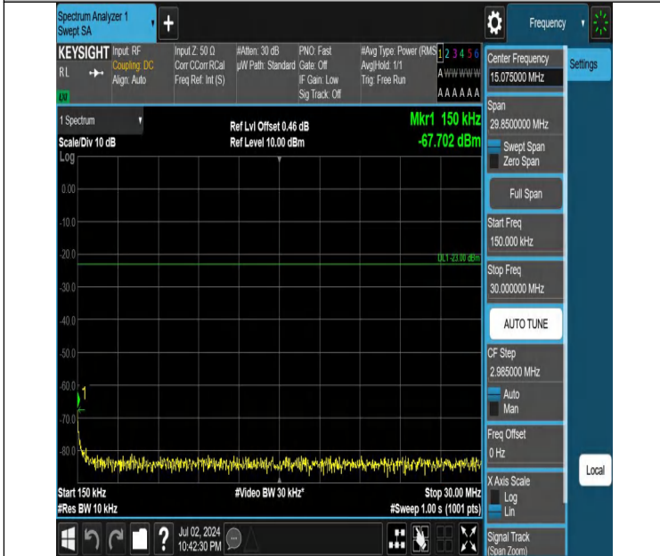
Band5-3MHz-QPSK-20525-1RB#14-0.15~30-PASS
