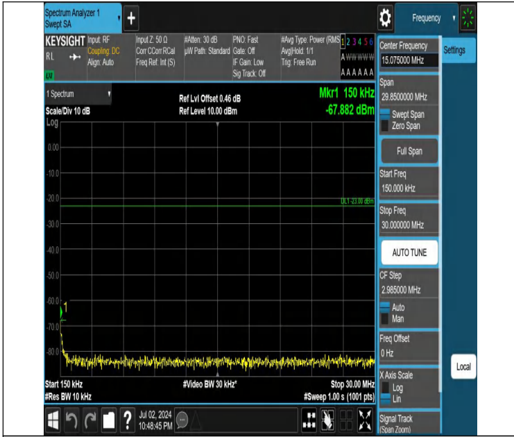
Band5-10MHz-QPSK-20450-1RB#49-0.15~30-PASS
