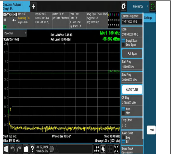
Band5-5MHz-QPSK-20625-1RB#0-0.15~30-PASS
