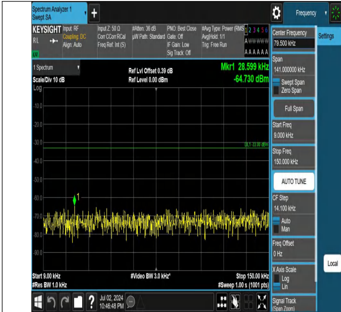
Band5-5MHz-QPSK-20625-1RB#0-0.009~0.15-PASS
