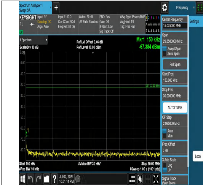
Band5-10MHz-QPSK-20600-1RB#49-0.15~30-PASS
