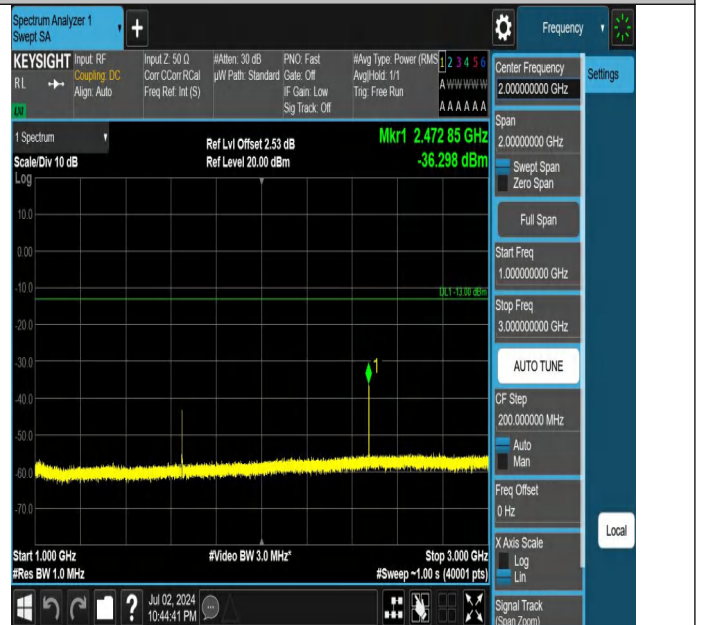
Band5-5MHz-QPSK-20425-1RB#0-1000~3000-PASS
