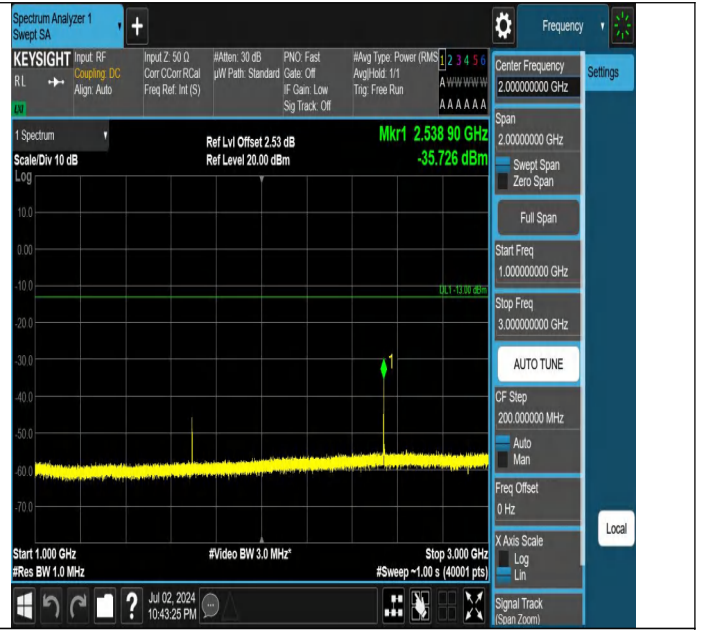
Band5-3MHz-QPSK-20635-1RB#0-1000~3000-PASS
