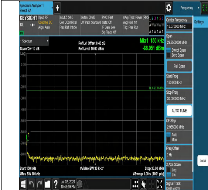
Band5-10MHz-QPSK-20525-1RB#49-0.15~30-PASS
