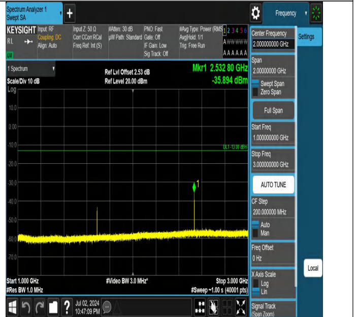
Band5-5MHz-QPSK-20625-1RB#0-1000~3000-PASS
