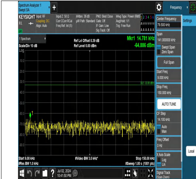
Band5-3MHz-QPSK-20525-1RB#0-0.009~0.15-PASS
