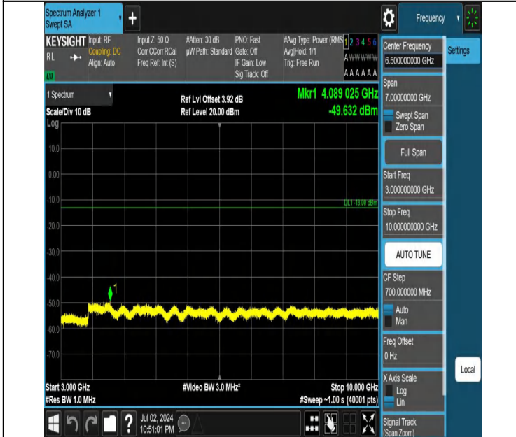
Band5-10MHz-QPSK-20600-1RB#0-3000~10000-PASS
