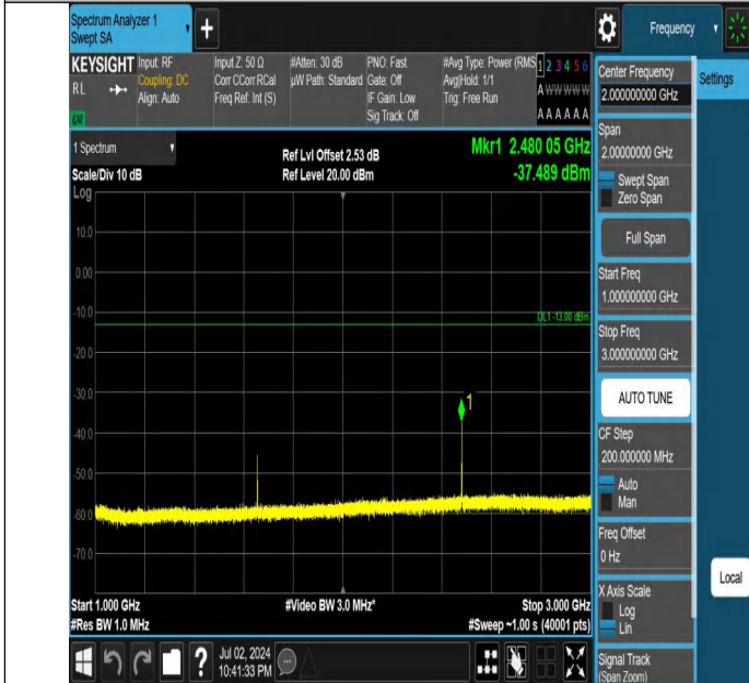
Band5-3MHz-QPSK-20415-1RB#14-1000~3000-PASS
