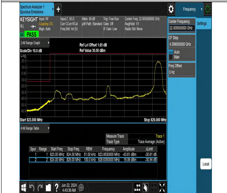
Band5-5MHz-QPSK-20425-1RB#24-PASS
