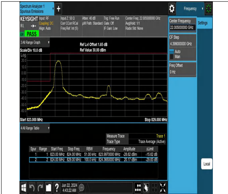
Band5-5MHz-QPSK-20425-1RB#0-PASS
