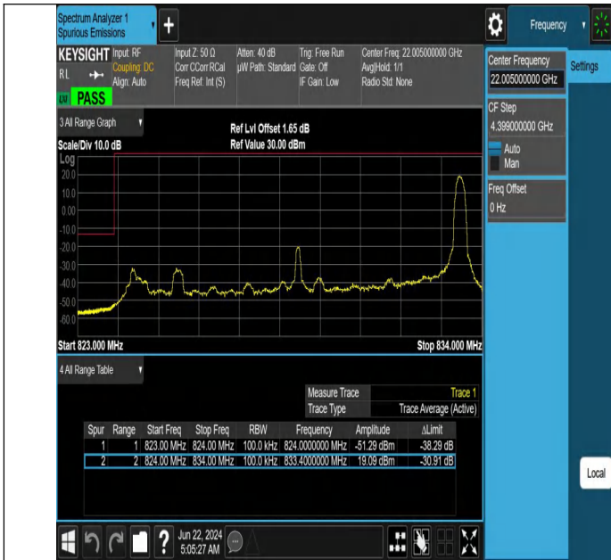
Band5-10MHz-QPSK-20450-1RB#49-PASS
