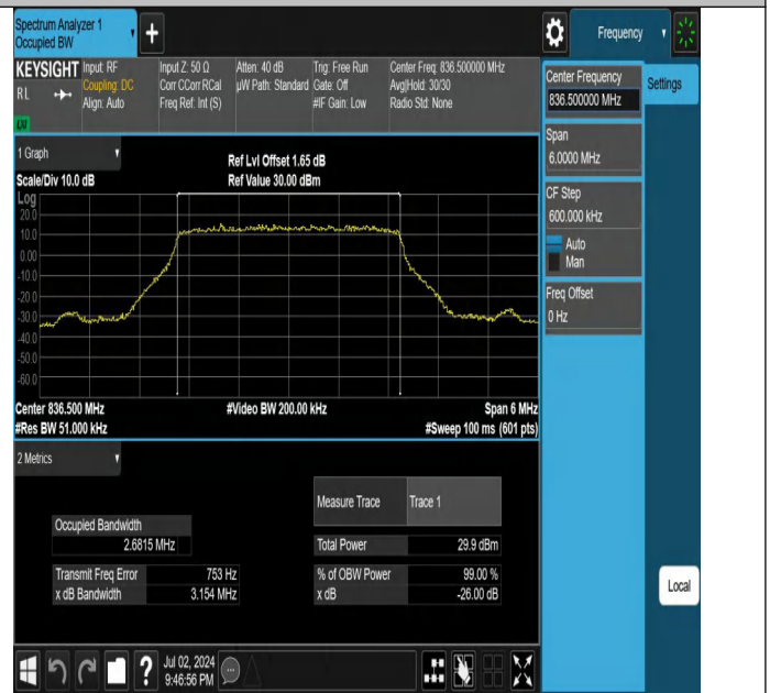
Band5-3MHz-16QAM-20525-15RB#0-PASS
