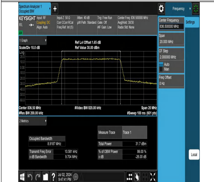
Band5-10MHz-QPSK-20525-50RB#0-PASS
