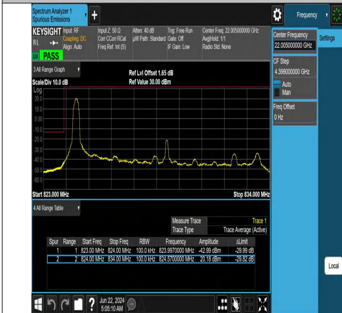
Band5-10MHz-QPSK-20450-1RB#0-PASS
