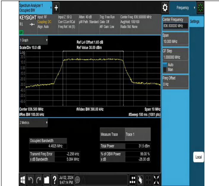
Band5-5MHz-QPSK-20525-25RB#0-PASS
