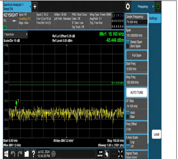
Band4-20MHz-QPSK-20175-1RB#99-0.009~0.15-PASS
