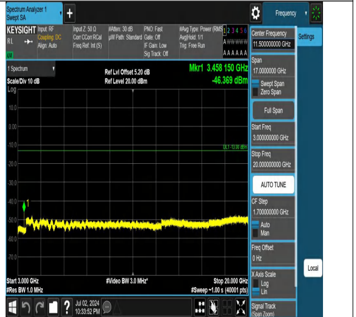
Band4-20MHz-QPSK-20050-1RB#99-3000~20000-PASS
