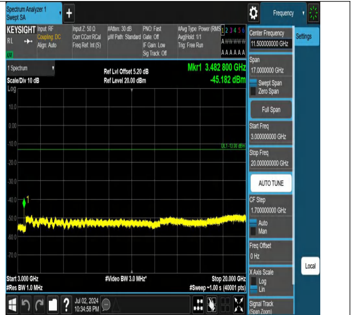
Band4-20MHz-QPSK-20175-1RB#99-3000~20000-PASS
