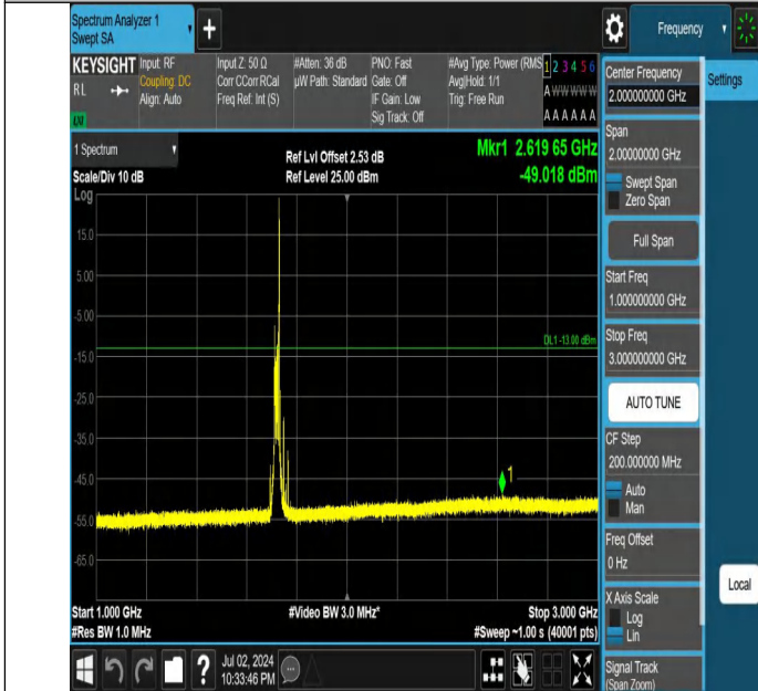
Band4-20MHz-QPSK-20050-1RB#99-1000~3000-PASS
