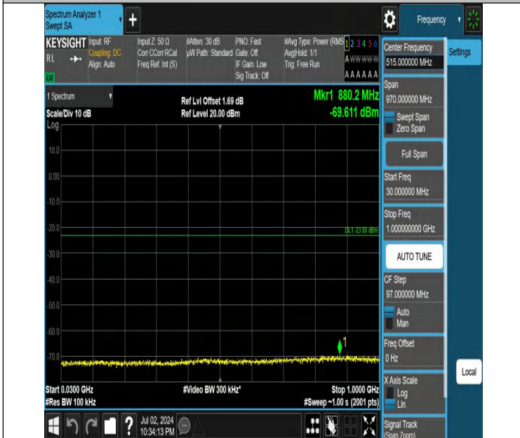
Band4-20MHz-QPSK-20175-1RB#0-30~1000-PASS
