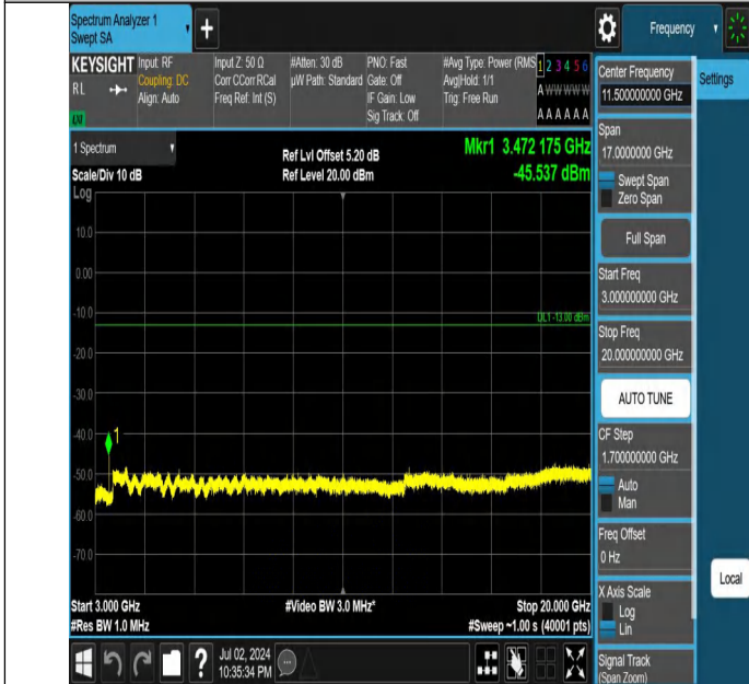
Band4-20MHz-QPSK-20300-1RB#0-3000~20000-PASS
