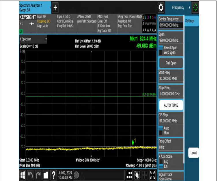
Band4-20MHz-QPSK-20300-1RB#99-30~1000-PASS
