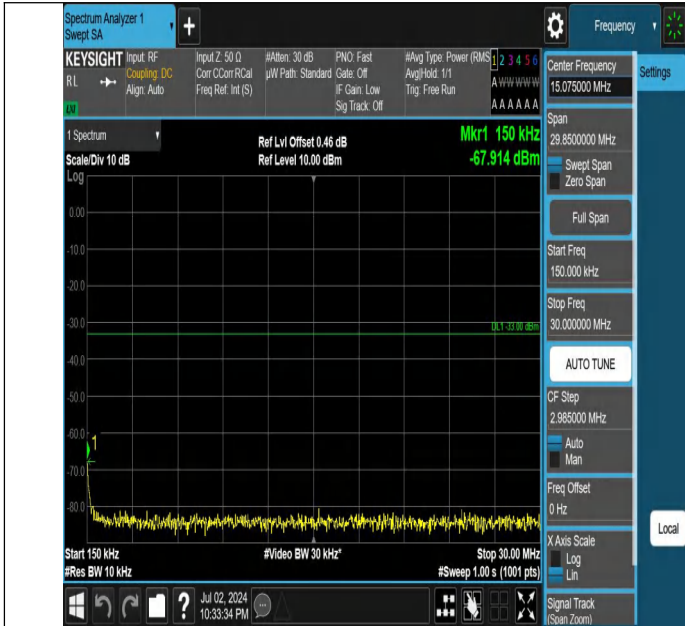
Band4-20MHz-QPSK-20050-1RB#99-0.15~30-PASS
