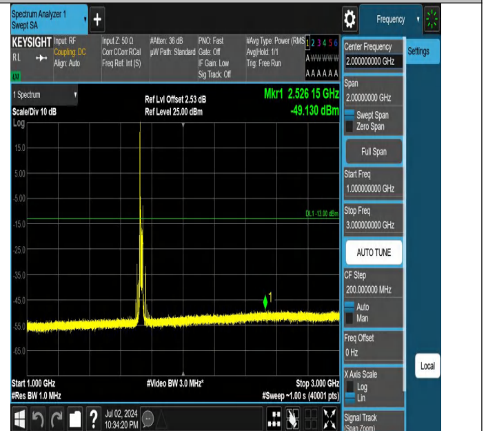
Band4-20MHz-QPSK-20175-1RB#0-1000~3000-PASS
