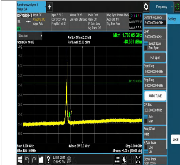
Band4-20MHz-QPSK-20175-1RB#99-1000~3000-PASS
