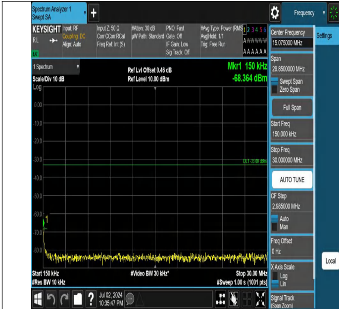
Band4-20MHz-QPSK-20300-1RB#99-0.15~30-PASS
