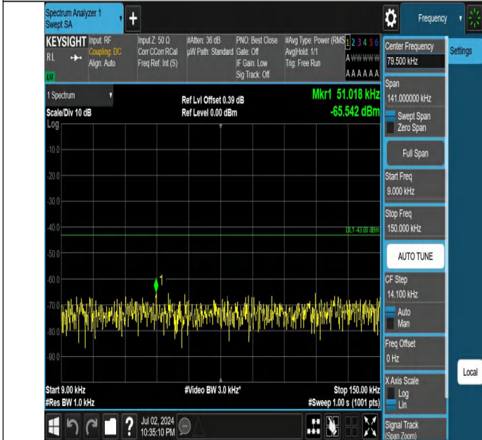
Band4-20MHz-QPSK-20300-1RB#0-0.009~0.15-PASS
