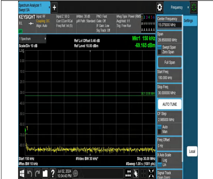
Band4-20MHz-QPSK-20175-1RB#99-0.15~30-PASS
