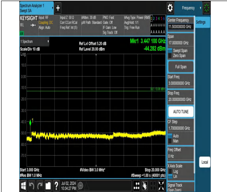
Band4-20MHz-QPSK-20175-1RB#0-3000~20000-PASS
