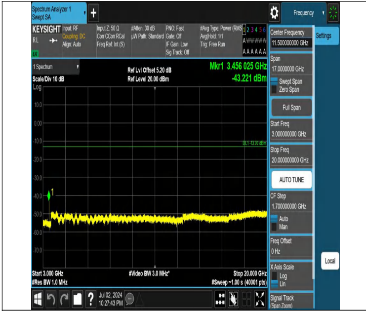
Band4-10MHz-QPSK-20175-1RB#0-3000~20000-PASS
