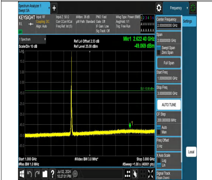
Band4-10MHz-QPSK-20000-1RB#49-1000~3000-PASS
