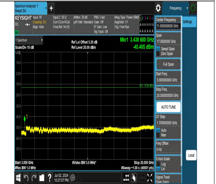
Band4-10MHz-QPSK-20000-1RB#49-3000~20000-PASS
