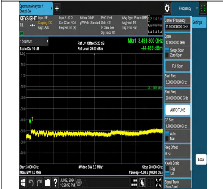
Band4-10MHz-QPSK-20350-1RB#0-3000~20000-PASS
