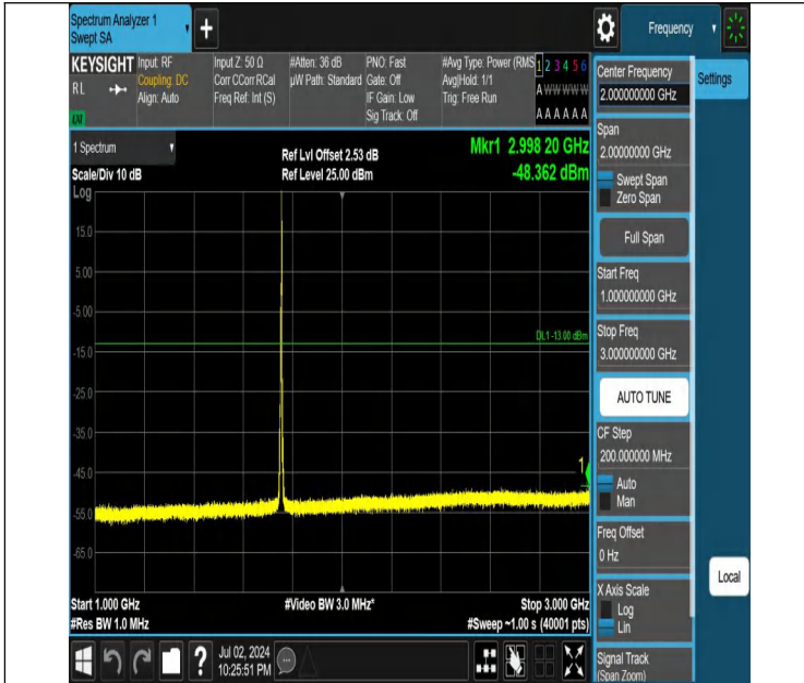
Band4-5MHz-QPSK-20375-1RB#24-1000~3000-PASS
