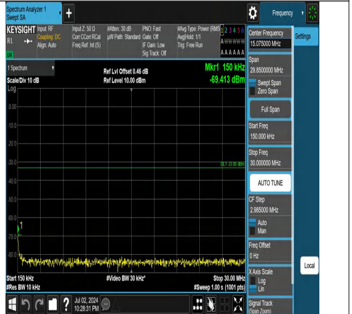
Band4-10MHz-QPSK-20350-1RB#0-0.15~30-PASS
