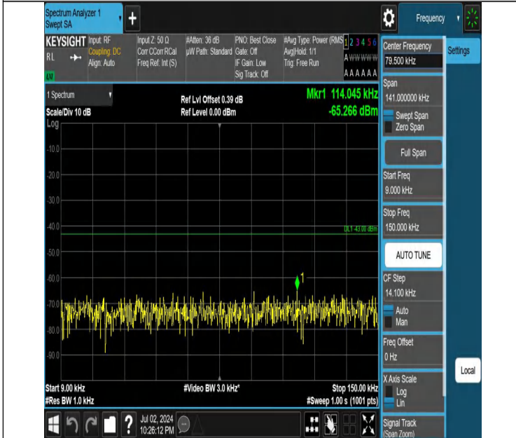
Band4-10MHz-QPSK-20000-1RB#0-0.009~0.15-PASS
