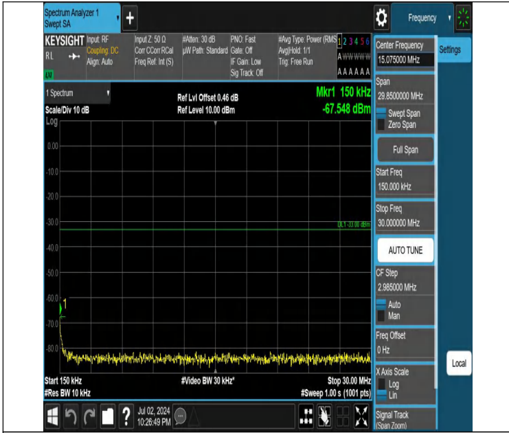
Band4-10MHz-QPSK-20000-1RB#49-0.15~30-PASS
