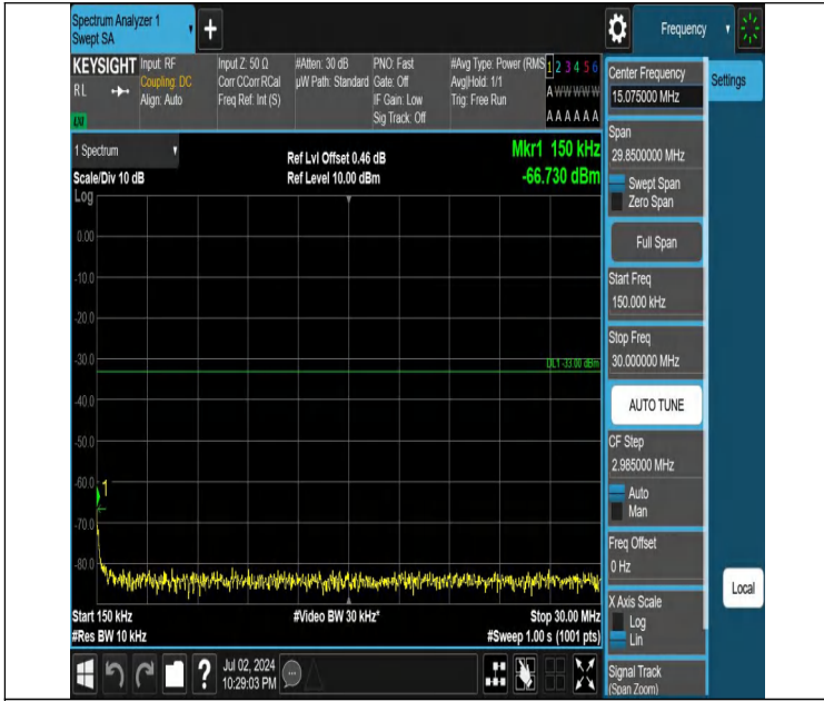
Band4-10MHz-QPSK-20350-1RB#49-0.15~30-PASS
