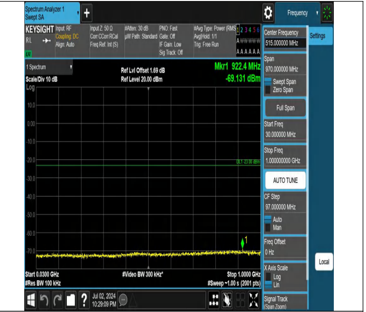
Band4-10MHz-QPSK-20350-1RB#49-30~1000-PASS
