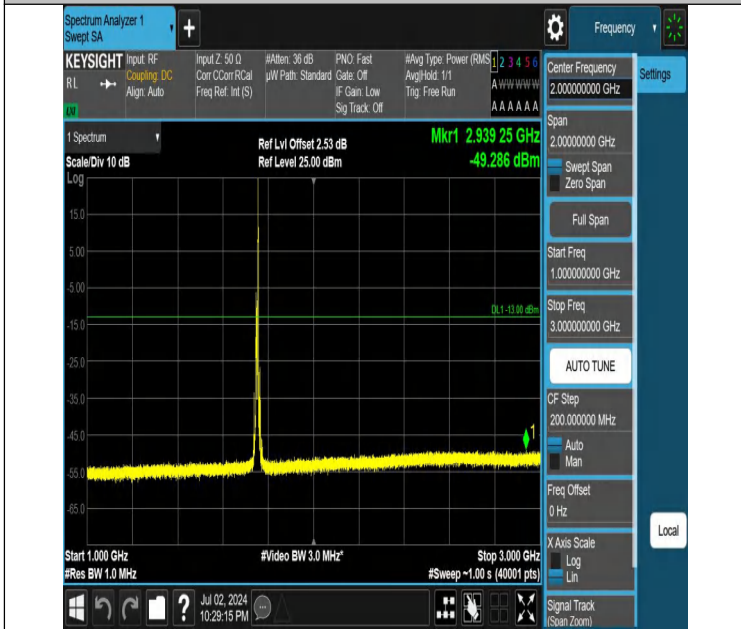
Band4-10MHz-QPSK-20350-1RB#49-1000~3000-PASS
