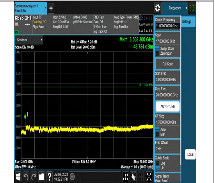
Band4-10MHz-QPSK-20350-1RB#49-3000~20000-PASS
