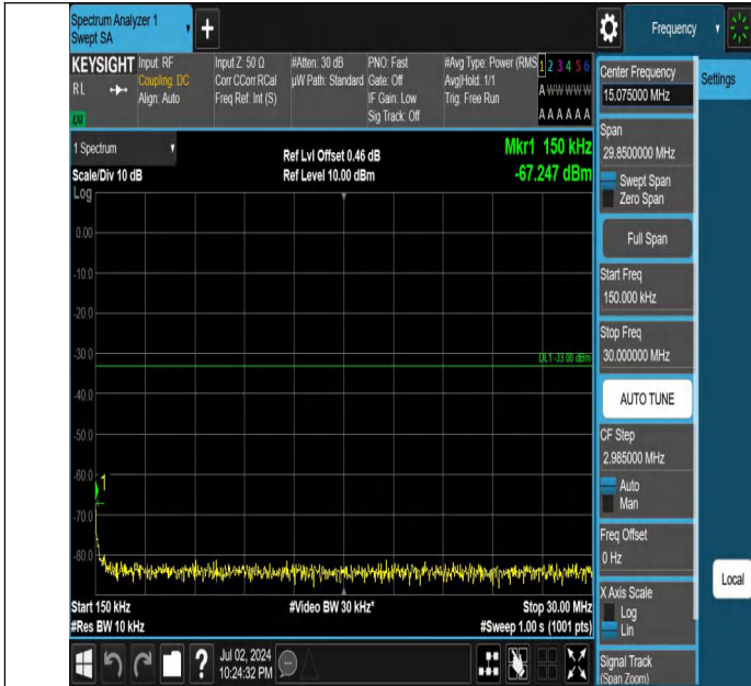
Band4-5MHz-QPSK-20175-1RB#24-0.15~30-PASS
