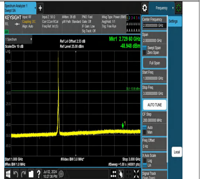
Band4-10MHz-QPSK-20175-1RB#0-1000~3000-PASS
