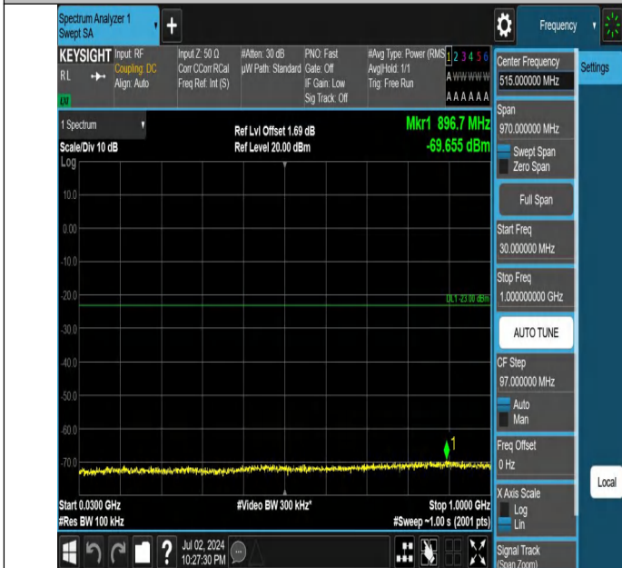
Band4-10MHz-QPSK-20175-1RB#0-30~1000-PASS
