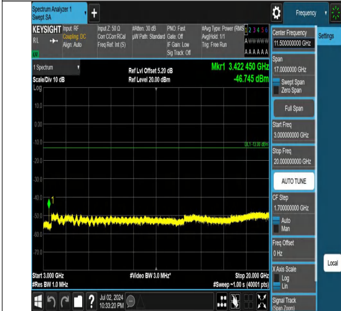
Band4-20MHz-QPSK-20050-1RB#0-3000~20000-PASS
