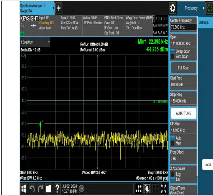
Band4-10MHz-QPSK-20175-1RB#0-0.009~0.15-PASS
