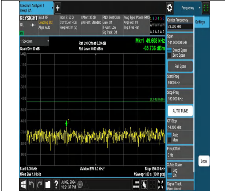
Band4-3MHz-QPSK-20385-1RB#0-0.009~0.15-PASS
