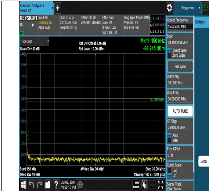
Band4-3MHz-QPSK-20385-1RB#14-0.15~30-PASS
