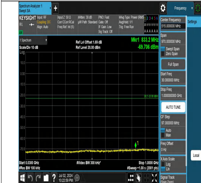
Band4-5MHz-QPSK-19975-1RB#0-30~1000-PASS
