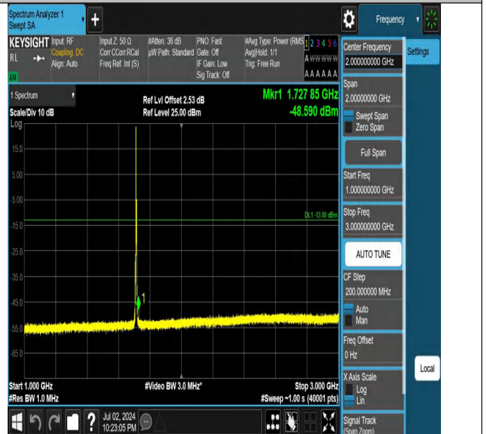
Band4-5MHz-QPSK-19975-1RB#0-1000~3000-PASS
