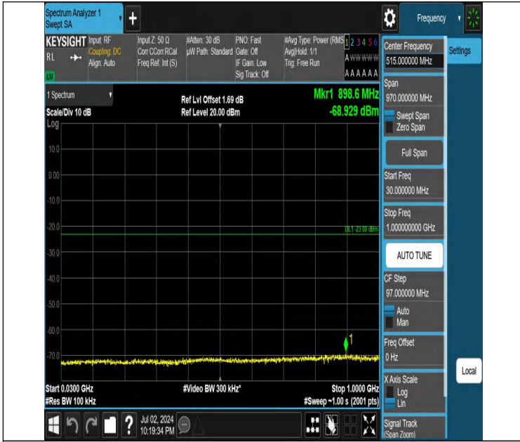
Band4-3MHz-QPSK-19965-1RB#0-30~1000-PASS
