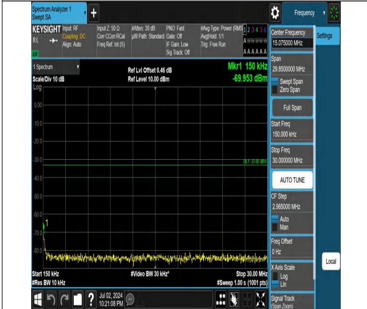
Band4-3MHz-QPSK-20175-1RB#14-0.15~30-PASS
