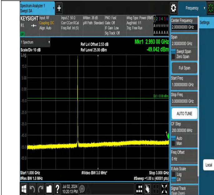
Band4-3MHz-QPSK-19965-1RB#14-1000~3000-PASS
