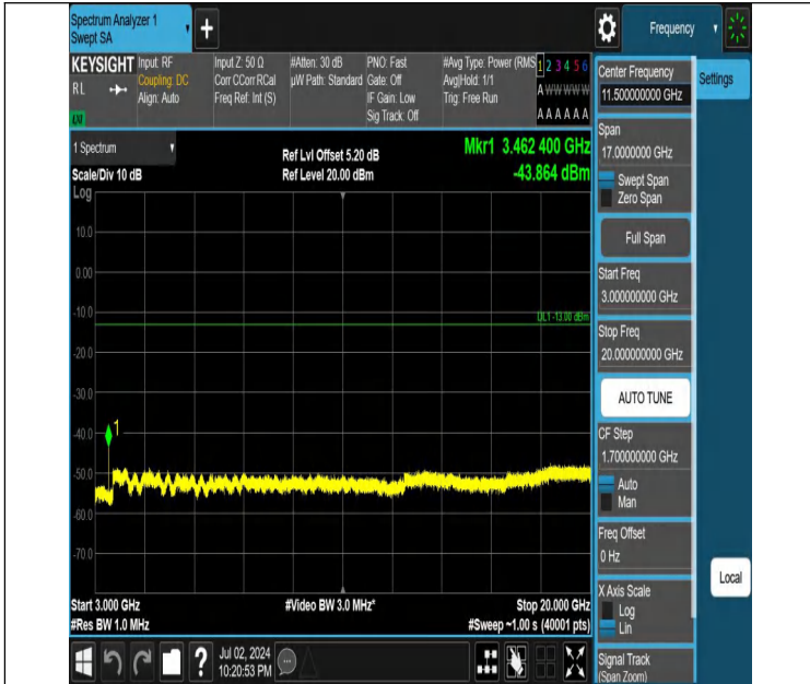
Band4-3MHz-QPSK-20175-1RB#0-3000~20000-PASS
