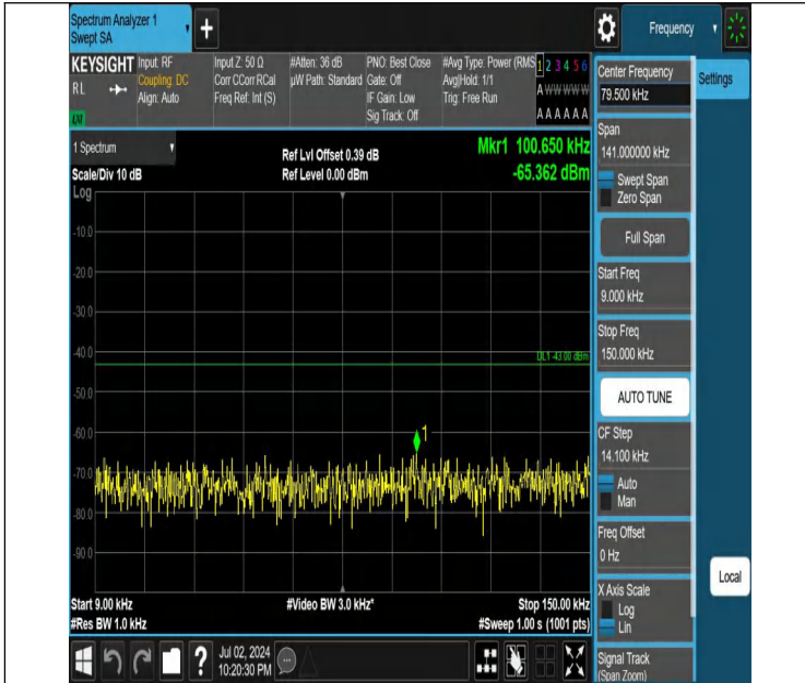
Band4-3MHz-QPSK-20175-1RB#0-0.009~0.15-PASS
