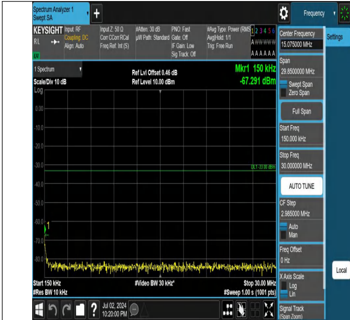
Band4-3MHz-QPSK-19965-1RB#14-0.15~30-PASS
