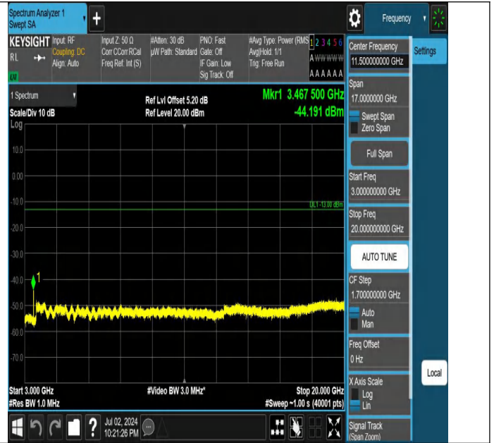
Band4-3MHz-QPSK-20175-1RB#14-3000~20000-PASS
