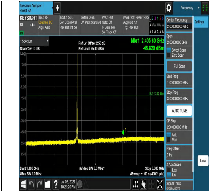
Band4-3MHz-QPSK-20175-1RB#14-1000~3000-PASS
