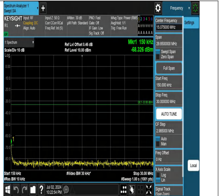
Band4-5MHz-QPSK-19975-1RB#0-0.15~30-PASS
