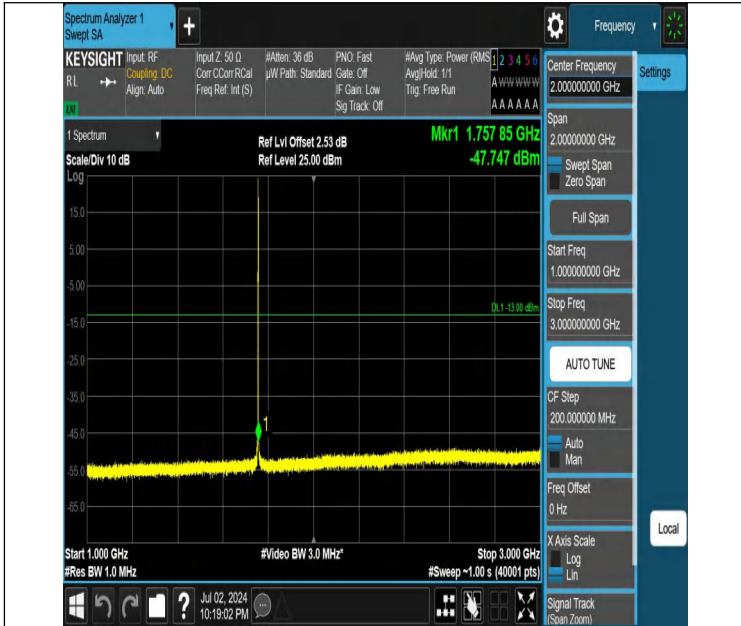
Band4-1.4MHz-QPSK-20393-1RB#5-1000~3000-PASS
