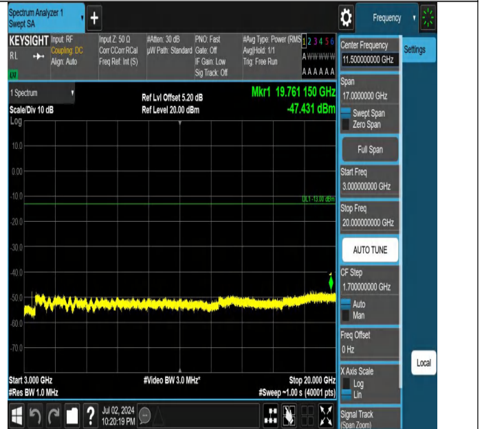
Band4-3MHz-QPSK-19965-1RB#14-3000~20000-PASS
