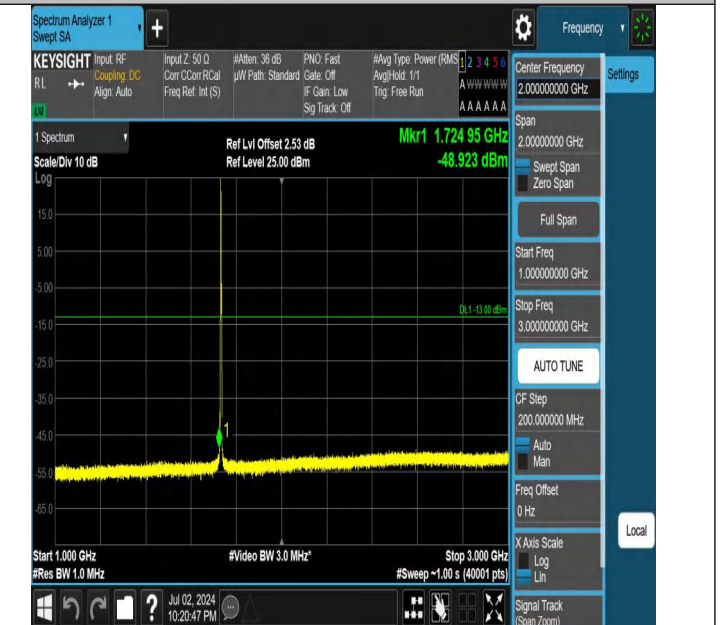
Band4-3MHz-QPSK-20175-1RB#0-1000~3000-PASS
