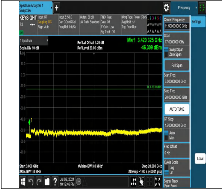
Band4-3MHz-QPSK-19965-1RB#0-3000~20000-PASS
