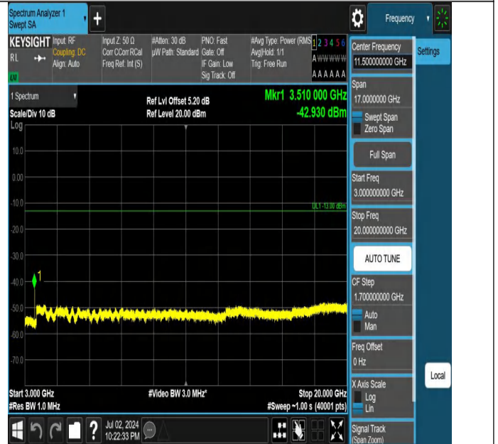
Band4-3MHz-QPSK-20385-1RB#14-3000~20000-PASS
