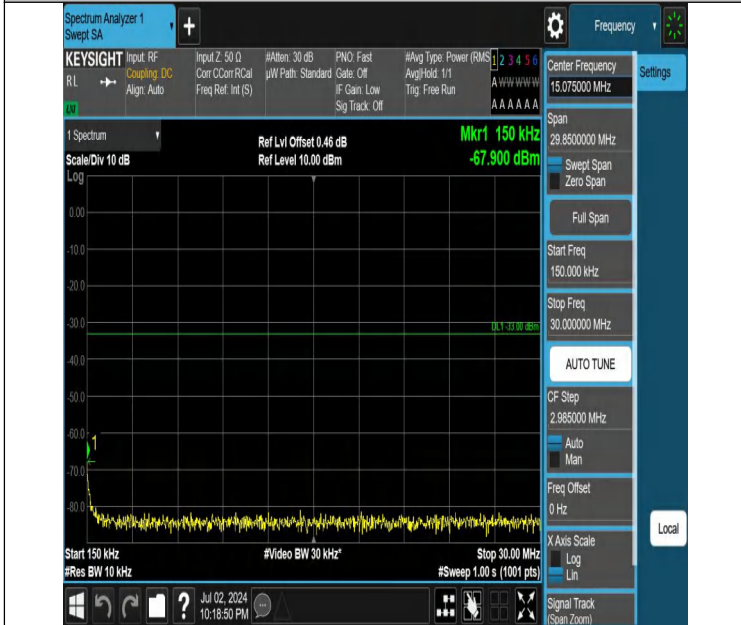
Band4-1.4MHz-QPSK-20393-1RB#5-0.15~30-PASS
