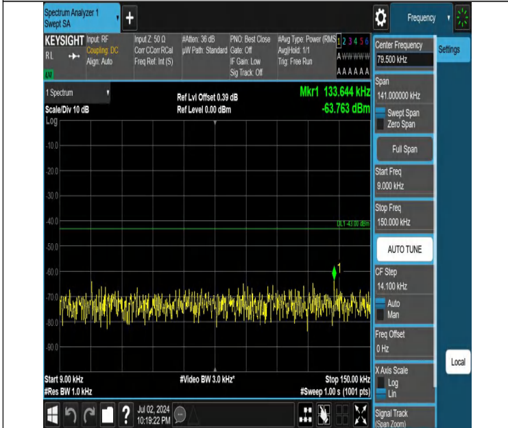
Band4-3MHz-QPSK-19965-1RB#0-0.009~0.15-PASS
