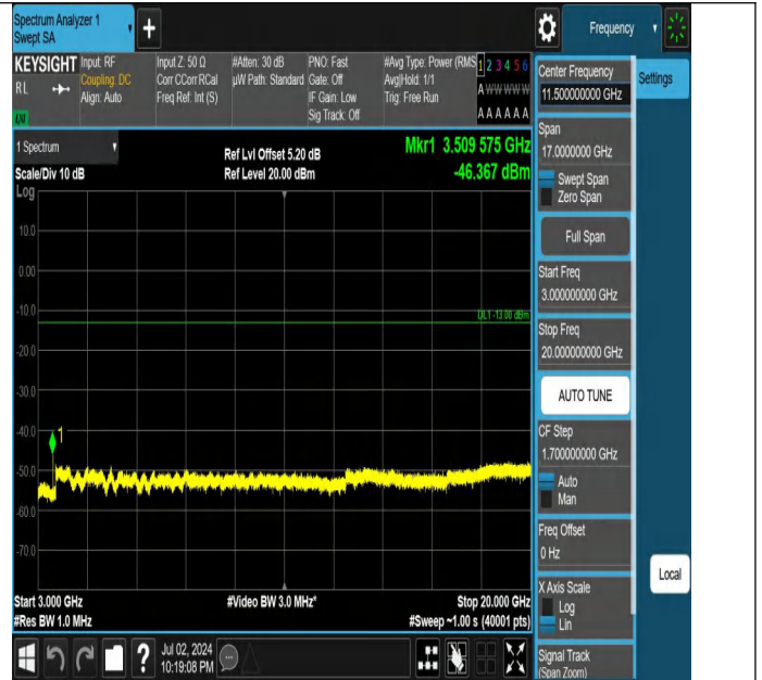
Band4-1.4MHz-QPSK-20393-1RB#5-3000~20000-PASS
