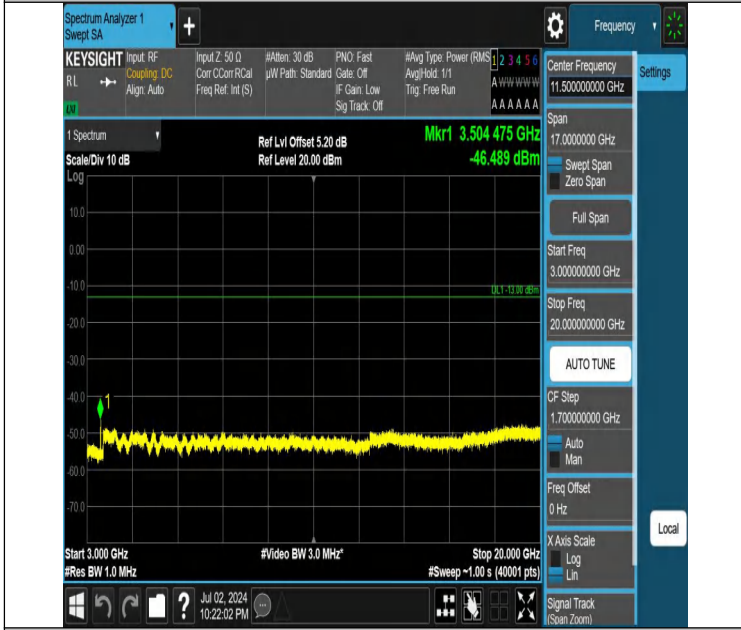
Band4-3MHz-QPSK-20385-1RB#0-3000~20000-PASS
