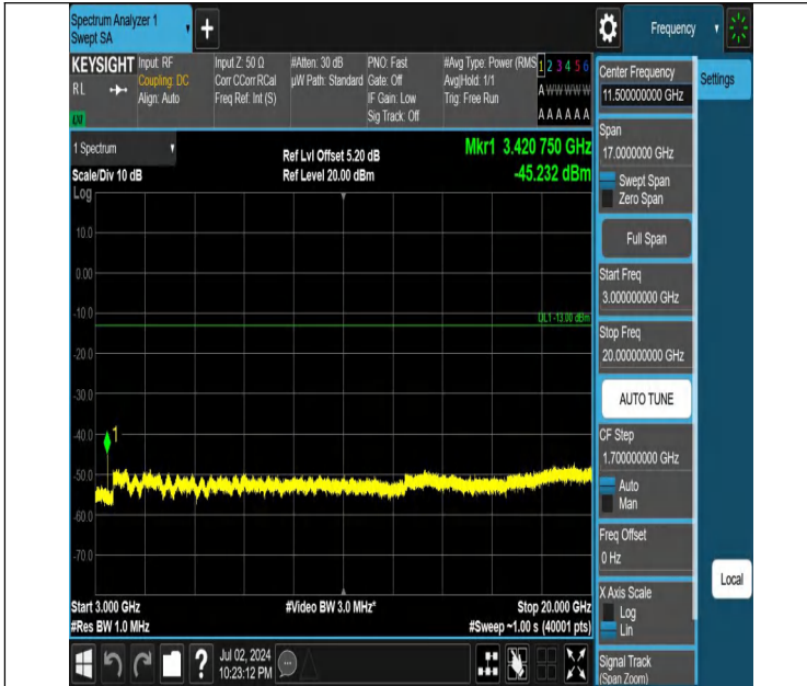
Band4-5MHz-QPSK-19975-1RB#0-3000~20000-PASS
