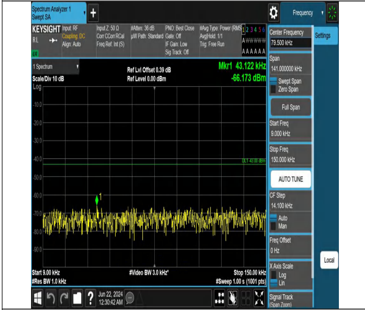
Band2_3MHz_QPSK_18900_1RB#14_0.009~0.15_0.009~0.15
