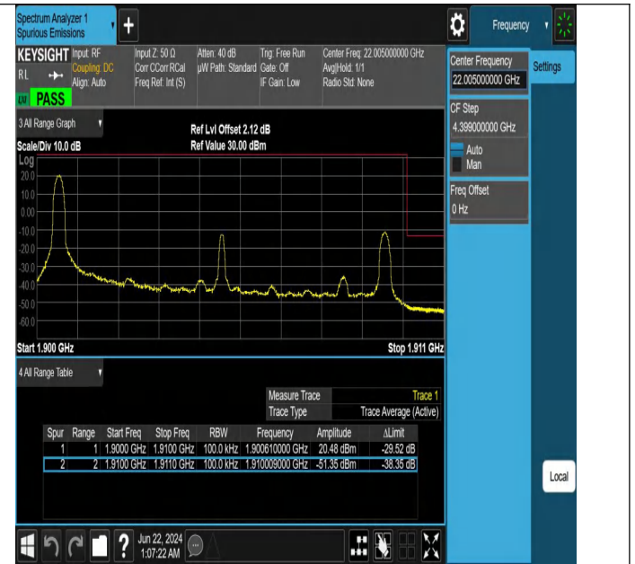
Band2_10MHz_QPSK_19150_1RB#0
