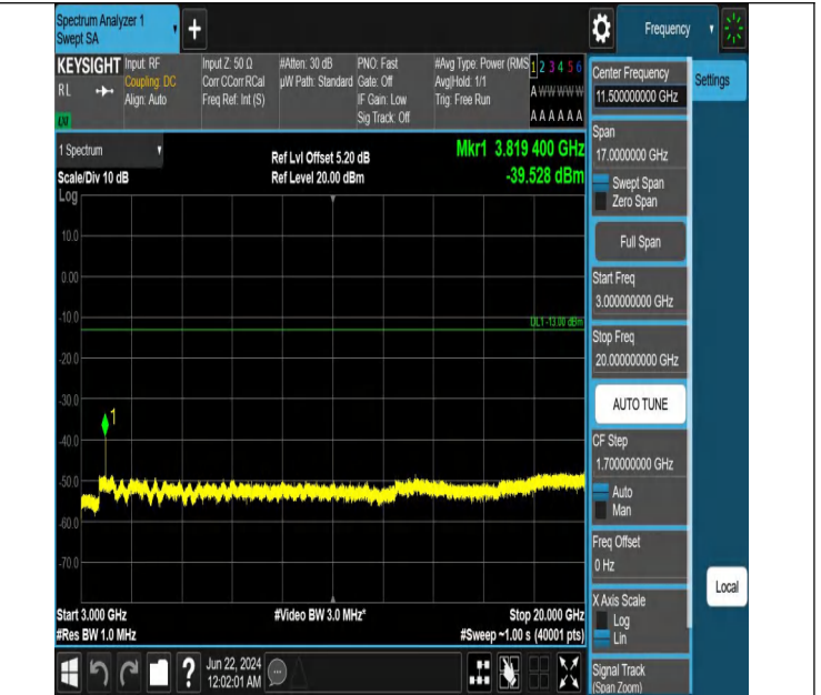
Band2_1.4MHz_QPSK_19193_1RB#5_3000~20000_3000~20000
