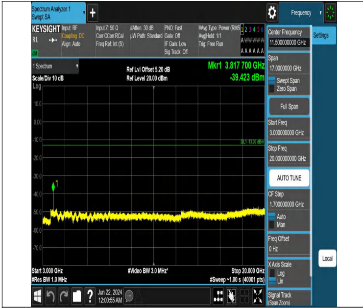
Band2_1.4MHz_QPSK_19193_1RB#0_3000~20000_3000~20000
