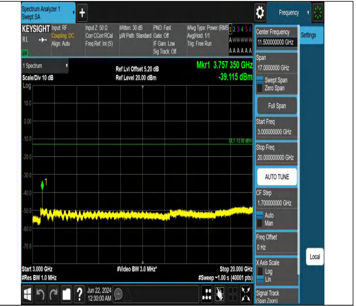
Band2_3MHz_QPSK_18900_1RB#0_3000~20000_3000~20000
