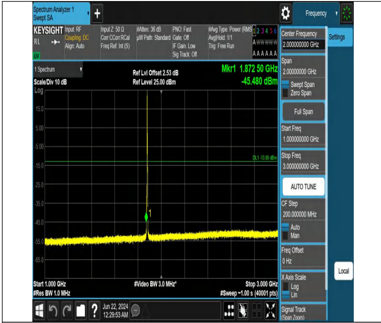
Band2_3MHz_QPSK_18900_1RB#0_1000~3000_1000~3000
