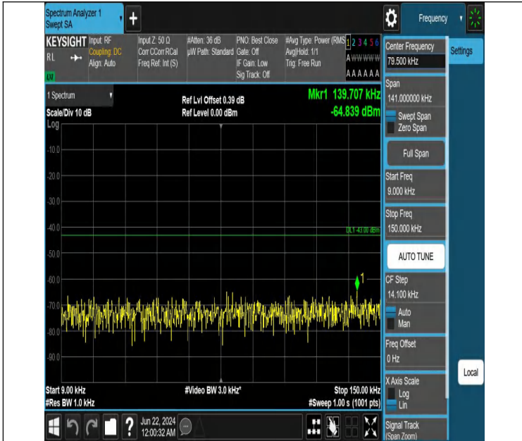
Band2_1.4MHz_QPSK_19193_1RB#0_0.009~0.15_0.009~0.15
