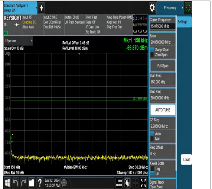
Band2_1.4MHz_QPSK_19193_1RB#0_0.15~30_0.15~30
