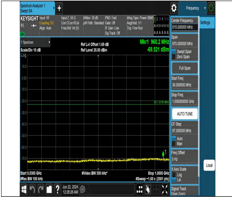
Band2_3MHz_QPSK_18615_1RB#0_30~1000_30~1000
