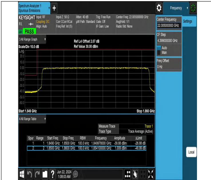
Band2_10MHz_QPSK_18650_50RB#0
