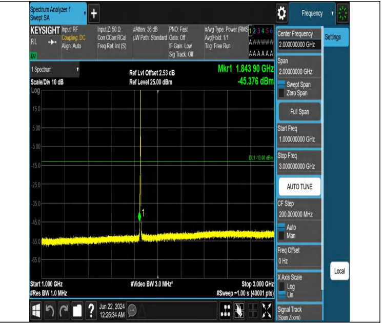
Band2_3MHz_QPSK_18615_1RB#0_1000~3000_1000~3000
