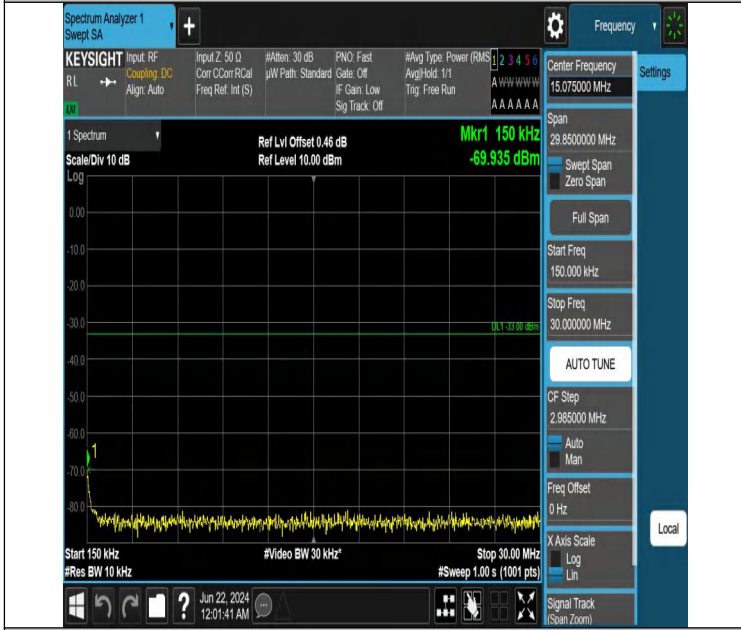
Band2_1.4MHz_QPSK_19193_1RB#5_0.15~30_0.15~30
