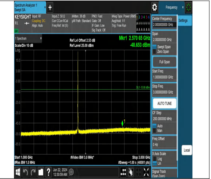
Band2_3MHz_QPSK_18900_1RB#14_1000~3000_1000~3000
