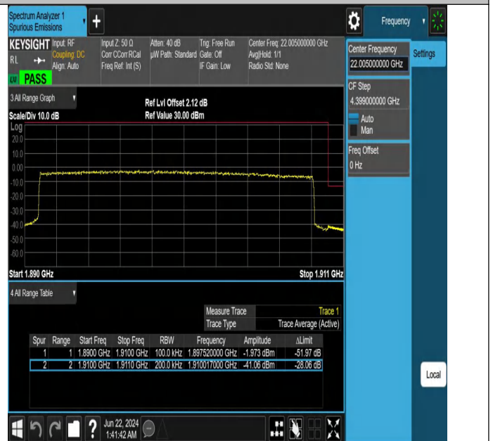
Band2_20MHz_QPSK_19100_100RB#0
