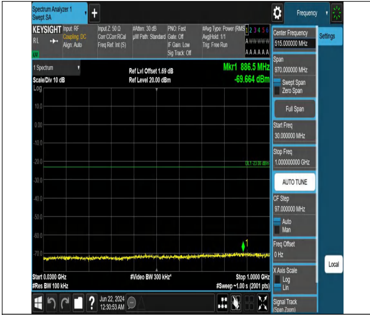
Band2_3MHz_QPSK_18900_1RB#14_30~1000_30~1000
