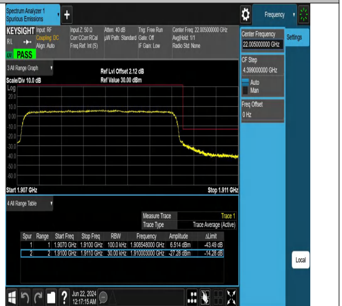
Band2_3MHz_QPSK_19185_15RB#0
