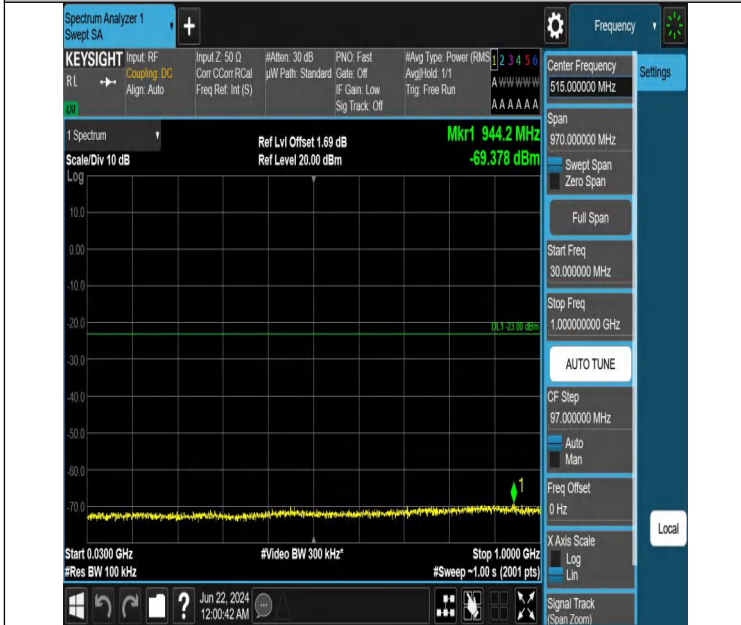
Band2_1.4MHz_QPSK_19193_1RB#0_30~1000_30~1000
