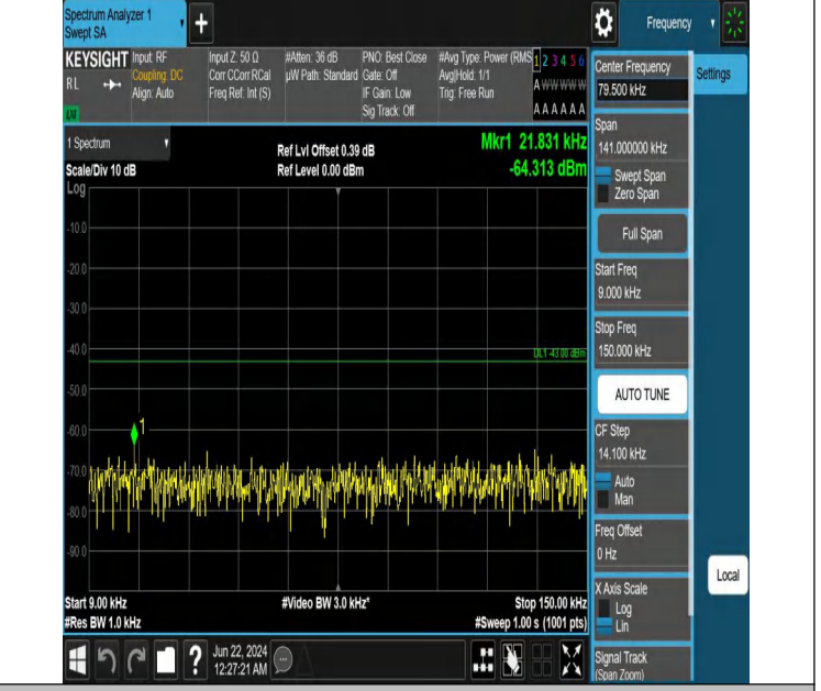
Band2_3MHz_QPSK_18615_1RB#14_0.009~0.15_0.009~0.15
