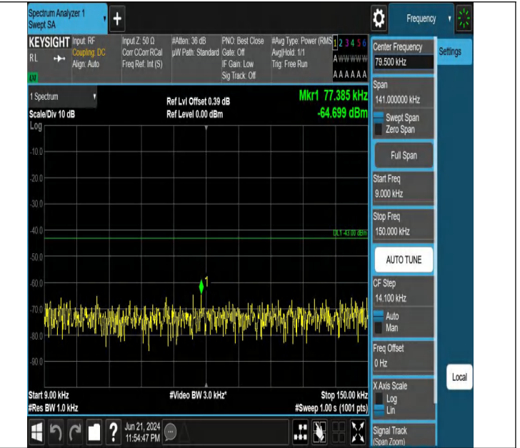
Band2_1.4MHz_QPSK_18607_1RB#5_0.009~0.15_0.009~0.15
