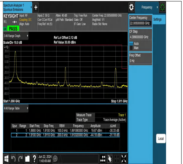
Band2_20MHz_QPSK_19100_1RB#0
