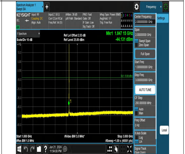
Band2_1.4MHz_QPSK_18607_1RB#0_1000~3000_1000~3000
