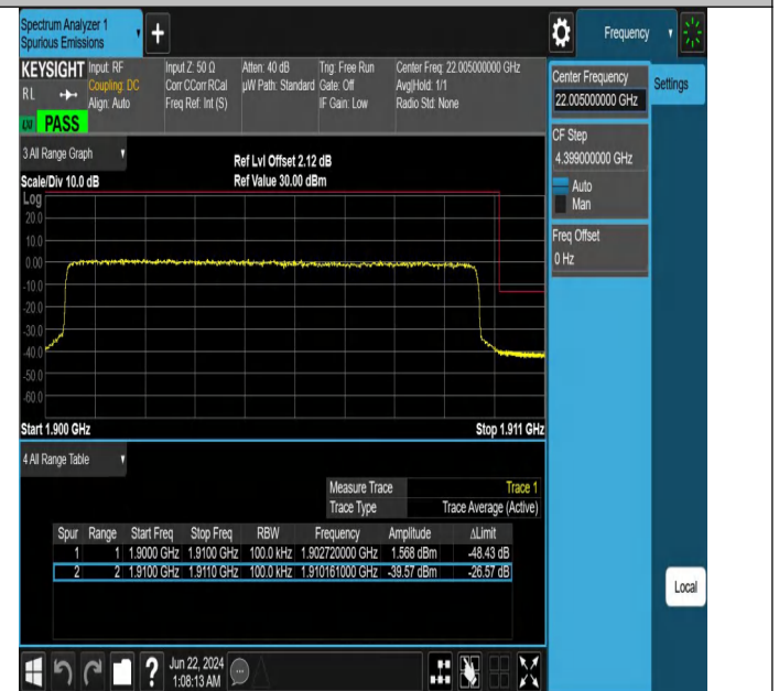
Band2_10MHz_QPSK_19150_50RB#0
