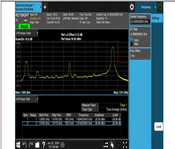
Band2_10MHz_QPSK_19150_1RB#49
