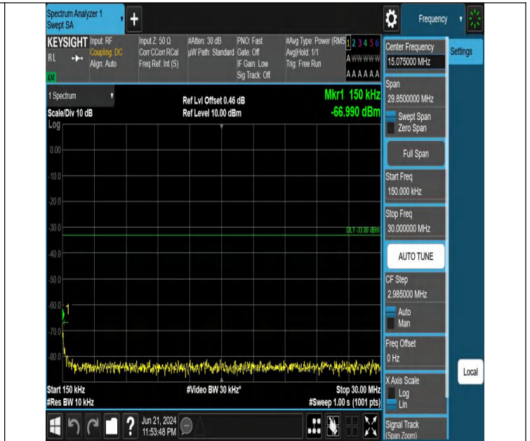
Band2_1.4MHz_QPSK_18607_1RB#0_0.15~30_0.15~30
