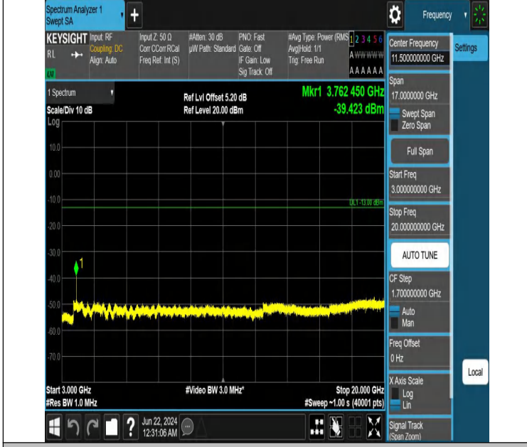
Band2_3MHz_QPSK_18900_1RB#14_3000~20000_3000~20000
