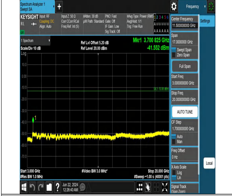
Band2_3MHz_QPSK_18615_1RB#0_3000~20000_3000~20000
