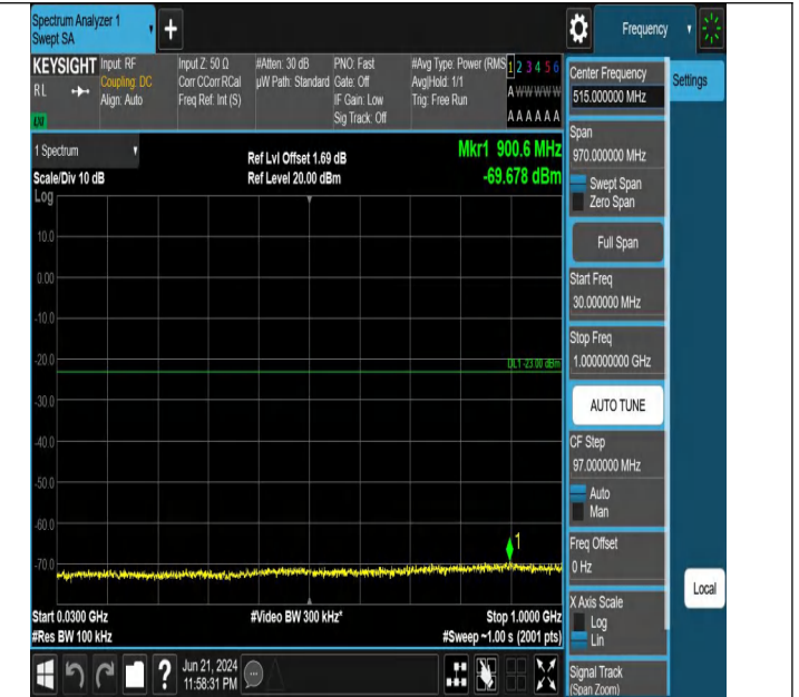
Band2_1.4MHz_QPSK_18900_1RB#5_30~1000_30~1000
