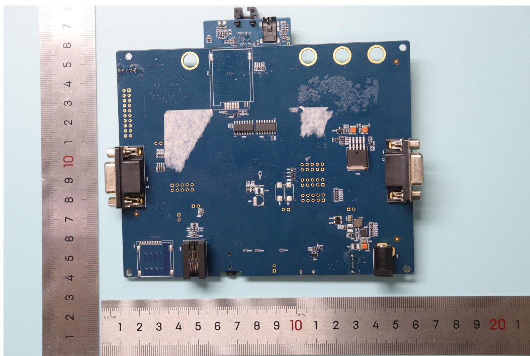
EC600U-LA + EVB_Bottom
