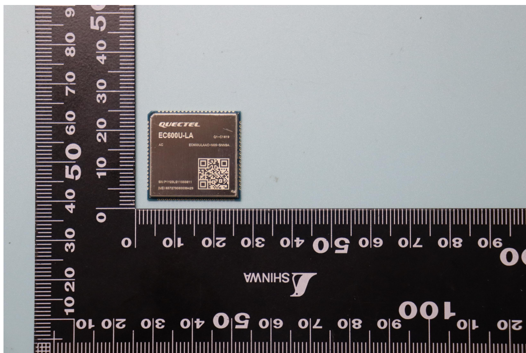
EC600U-LA_Top
