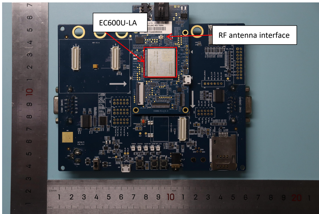
EC600U-LA + EVB_Top
