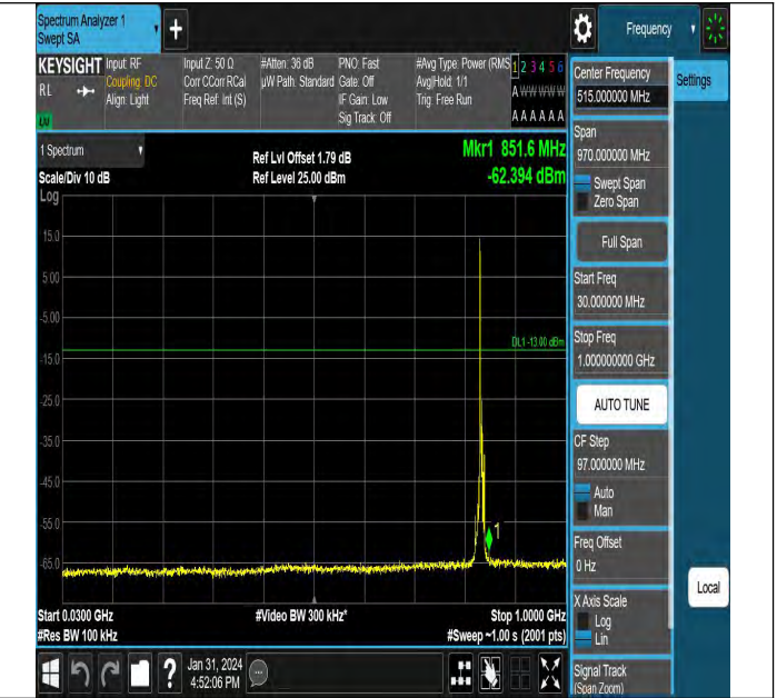
Band5_5MHz_QPSK_20525_1RB#0_30~1000_30~1000
