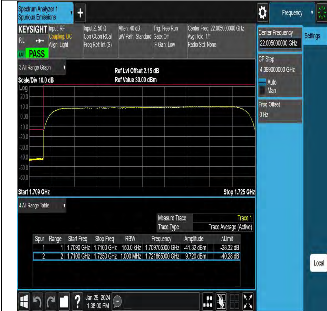
Band4_15MHz_QPSK_20025_75RB#0
