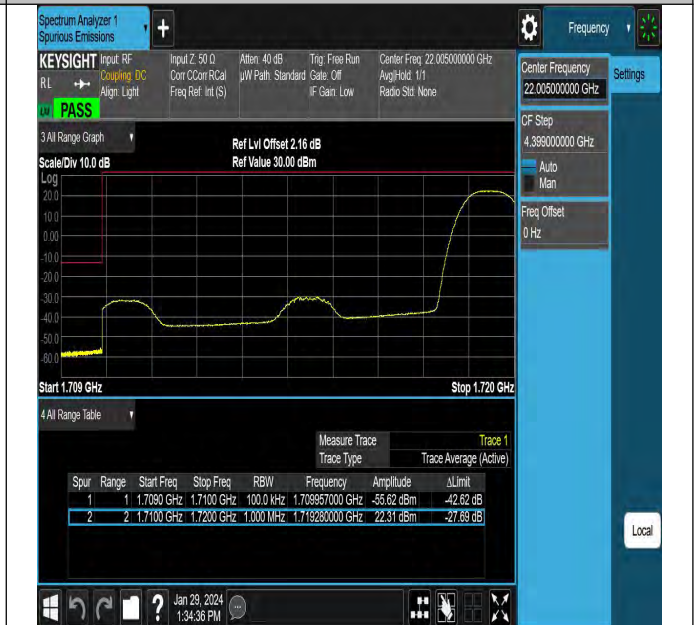
Band4_10MHz_QPSK_20000_1RB#49
