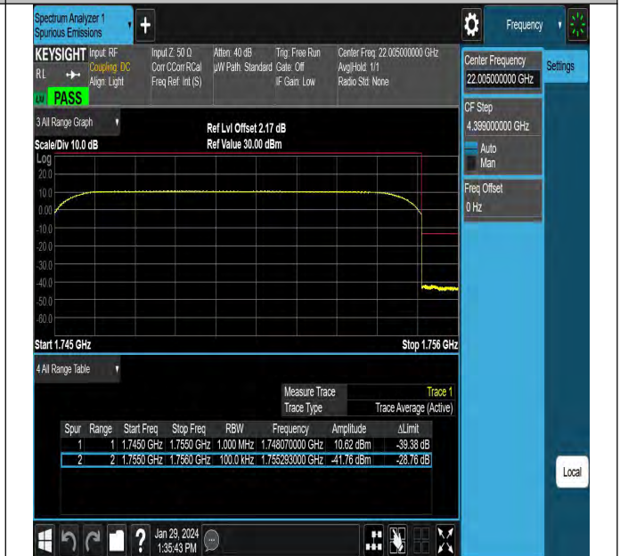
Band4_10MHz_QPSK_20350_50RB#0
