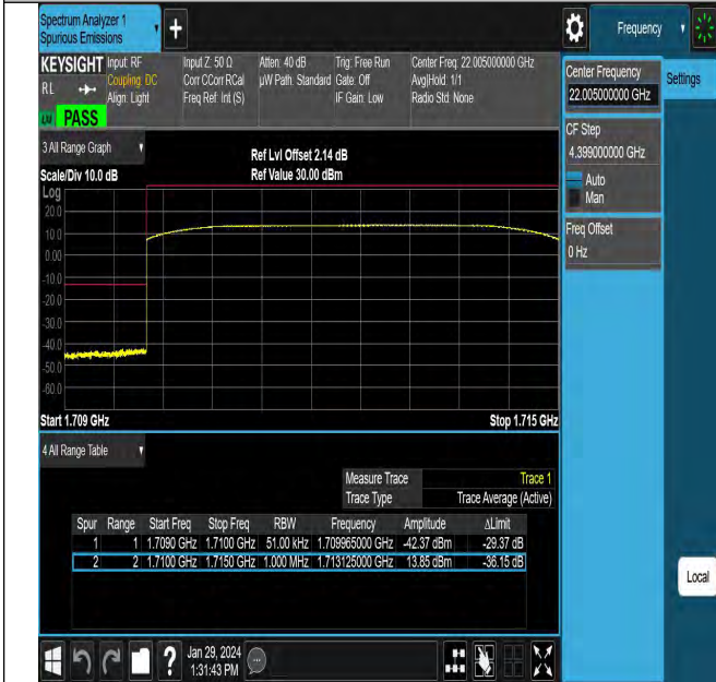
Band4_5MHz_QPSK_19975_25RB#0
