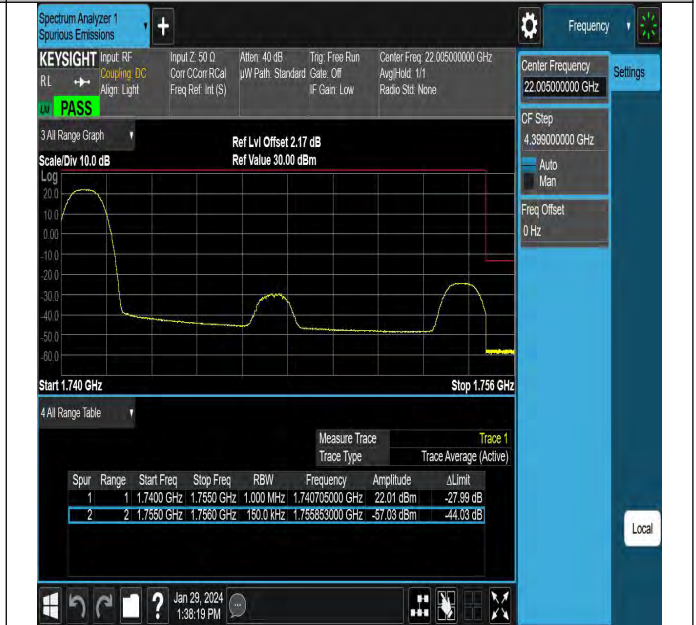
Band4_15MHz_QPSK_20325_1RB#0
