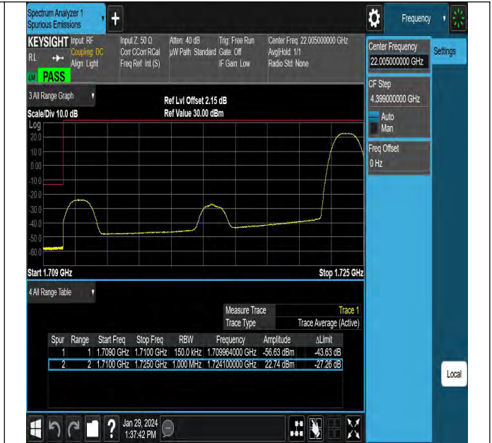
Band4_15MHz_QPSK_20025_1RB#74
