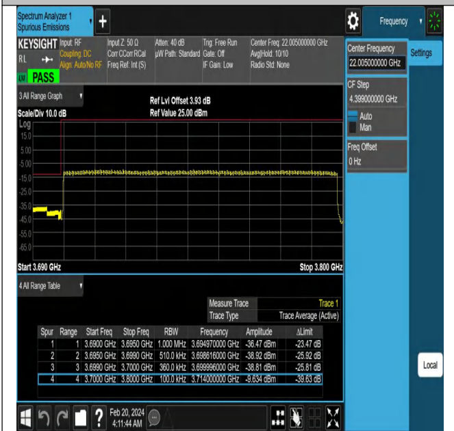
NTNV-N78-3700-3800-PC2-30-100-L-DFT-QPSK-Outer_FuII-Ant1-PASS
