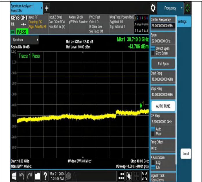
NTNV-N78-3700-3800-PC2-30-10-L-DFT-PI2BPSK-Edge_1R B_Left-Ant1-PASS
