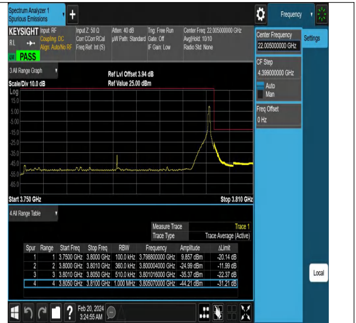
NTNV-N78-3700-3800-PC2-30-50-H-DFT-PI2BPSK-Edge_1RB_Right-Ant1-PASS
