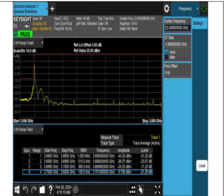
NTNV-N78-3700-3800-PC2-30-100-L-DFT-PI2BPSK-Edge_1RB_Left-Ant1-PASS
