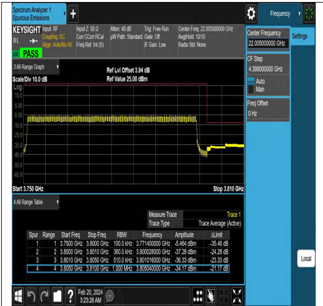
NTNV-N78-3700-3800-PC2-30-50-H-DFT-PI2BPSK-Outer_Full-Ant1-PASS
