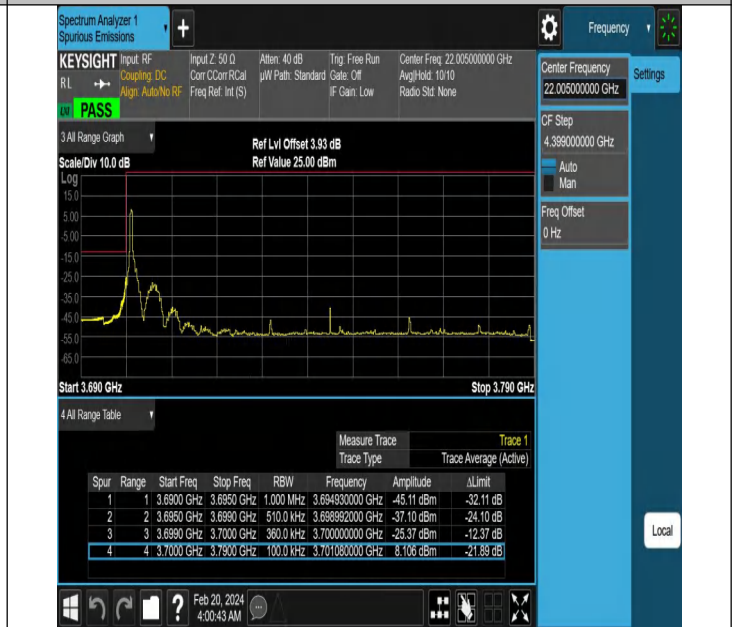
NTNV-N78-3700-3800-PC2-30-90-L-DFT-QPSK-Edge_1RB_Left-Ant1-PASS
