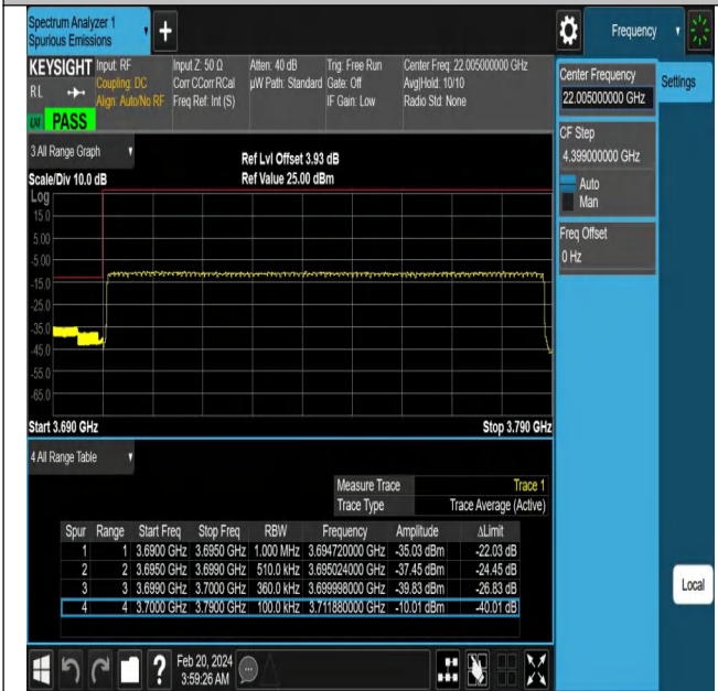
NTNV-N78-3700-3800-PC2-30-90-L-DFT-QPSK-Outer_Full-Ant1-PASS
