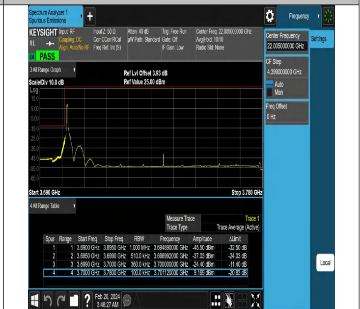
NTNV-N78-3700-3800-PC2-30-80-L-DFT-QPSK-Edge_1RB_Left-Ant1-PASS
