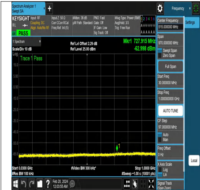
NTNV-N78-3700-3800-PC2-30-10-L-DFT-PI2BPSK-Edge_1R B_Right-Ant1-PASS
