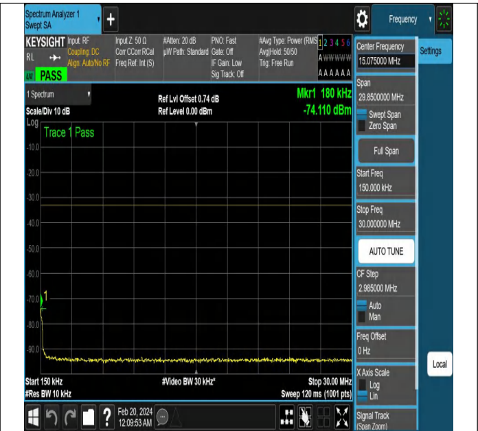
NTNV-N78-3700-3800-PC2-30-10-M-DFT-QPSK-Edge_1RB_ Left-Ant1-PASS
