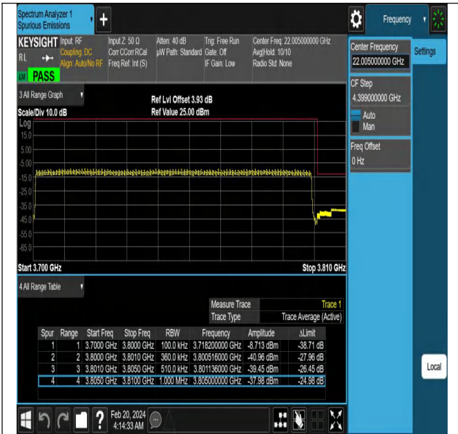
NTNV-N78-3700-3800-PC2-30-100-H-DFT-PI2BPSK-Outer_Full-Ant1-PASS
