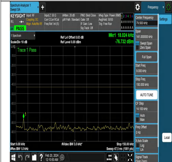
NTNV-N78-3700-3800-PC2-30-10-M-DFT-QPSK-Edge_1RB_
