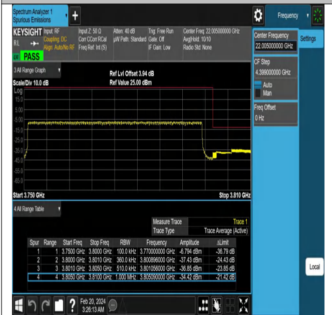
NTNV-N78-3700-3800-PC2-30-50-H-DFT-QPSK-Outer_Full-Ant1-PASS
