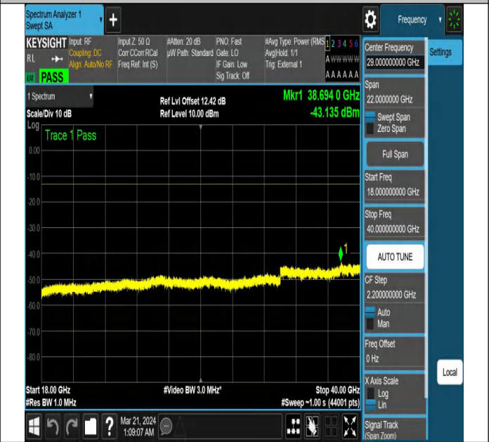
NTNV-N78-3700-3800-PC2-30-10-M-DFT-PI2BPSK-Edge_1R
