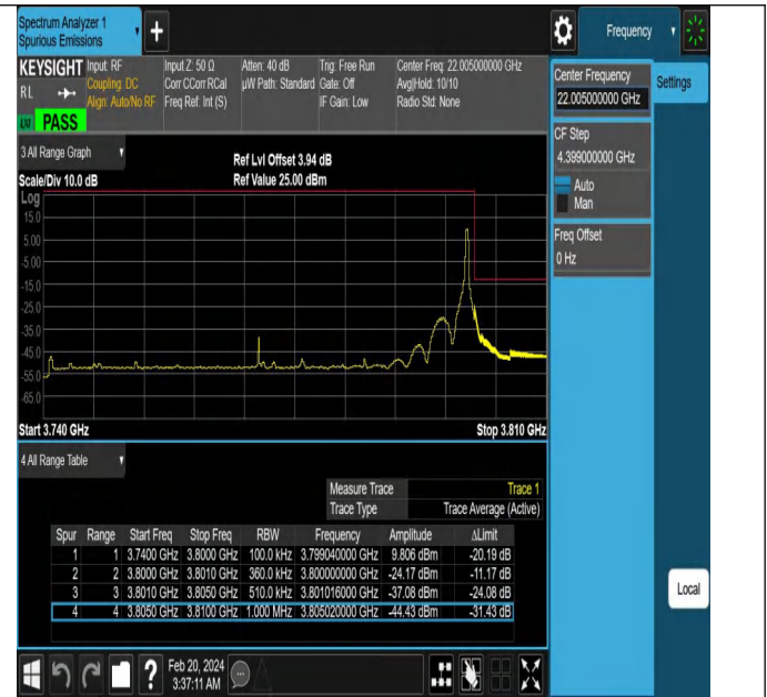
NTNV-N78-3700-3800-PC2-30-60-H-DFT-PI2BPSK-Edge_1RB_ Right-Ant1-PASS
