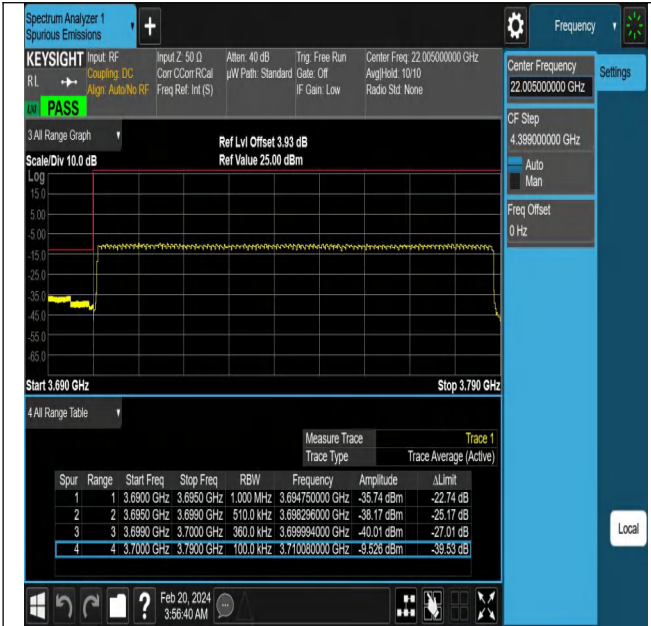
NTNV-N78-3700-3800-PC2-30-90-L-DFT-PI2BPSK-Outer_Full-Ant1-PASS
