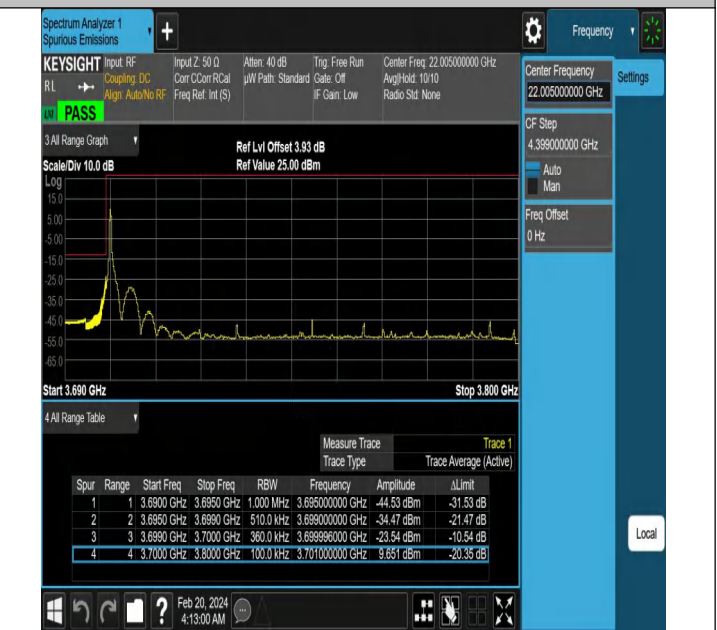
NTNV-N78-3700-3800-PC2-30-100-L-DFT-QPSK-Edge_1RB_Left-Ant1-PASS
