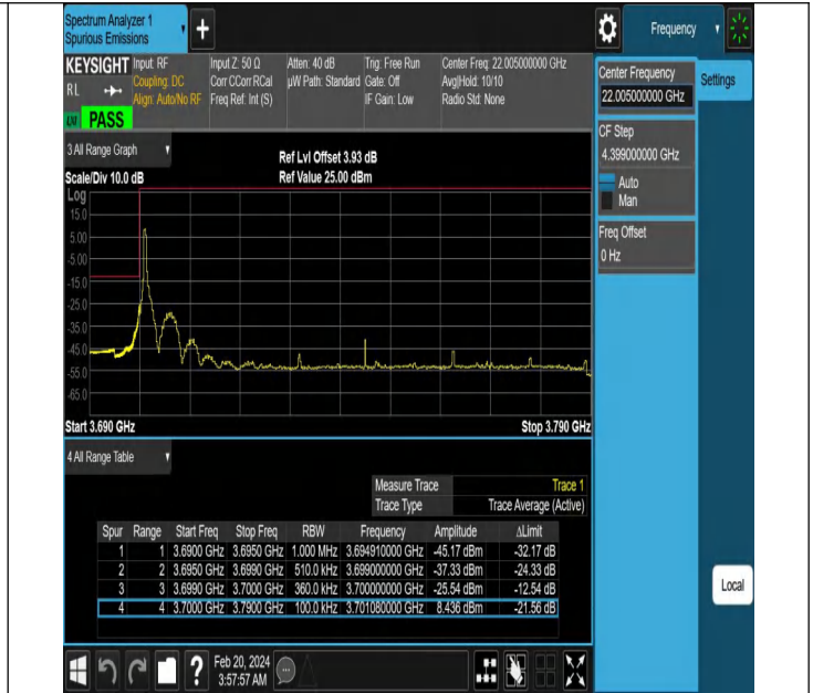
NTNV-N78-3700-3800-PC2-30-90-L-DFT-PI2BPSK-Edge_1RB_Left-Ant1-PASS
