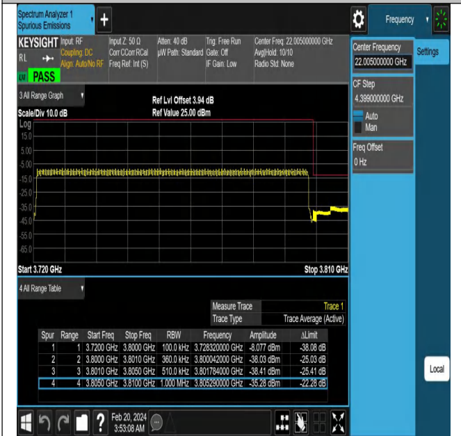
NTNV-N78-3700-3800-PC2-30-80-H-DFT-QPSK-Outer_Full-Ant1-PASS
