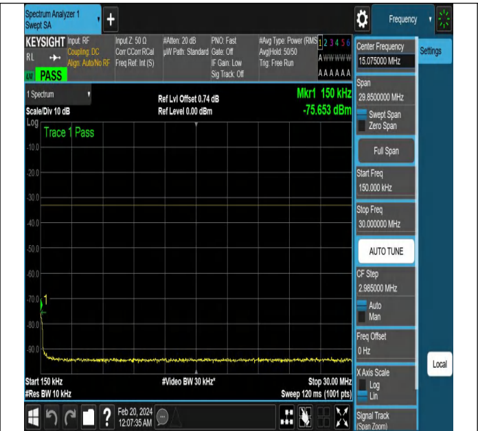
NTNV-N78-3700-3800-PC2-30-10-M-DFT-PI2BPSK-Edge_1R B_Left-Ant1-PASS
