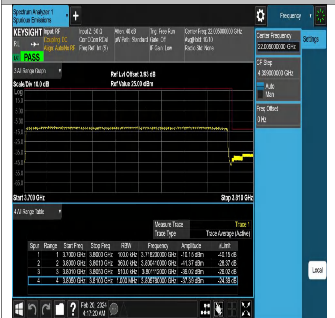
NTNV-N78-3700-3800-PC2-30-100-H-DFT-QPSK-Outer_Full-Ant1-PASS
