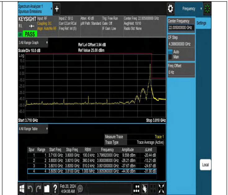
NTNV-N78-3700-3800-PC2-30-90-H-DFT-PI2BPSK-Edge_1RB_Right-Ant1-PASS
