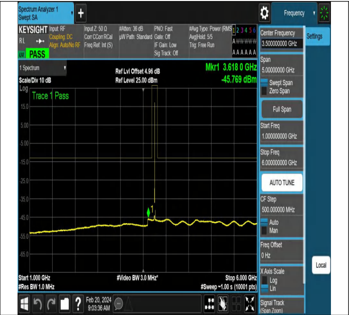
NTNV-N78-3700-3800-PC2-30-10-M-DFT-PI2BPSK-Edge_1R
