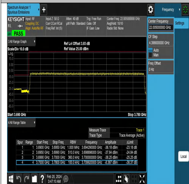
NTNV-N78-3700-3800-PC2-30-80-L-DFT-QPSK-Outer_Full-Ant1-PASS
