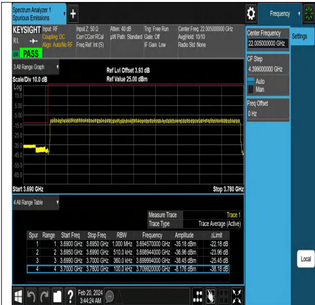
NTNV-N78-3700-3800-PC2-30-80-L-DFT-PI2BPSK-Outer_Full-Ant1-PASS
