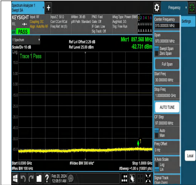
NTNV-N78-3700-3800-PC2-30-10-M-DFT-PI2BPSK-Edge_1R
