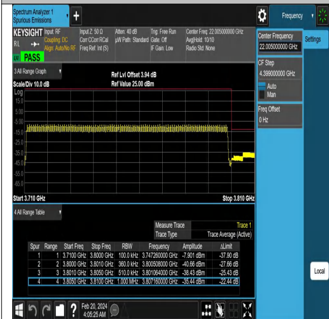
NTNV-N78-3700-3800-PC2-30-90-H-DFT-QPSK-Outer_Full-Ant1-PASS
