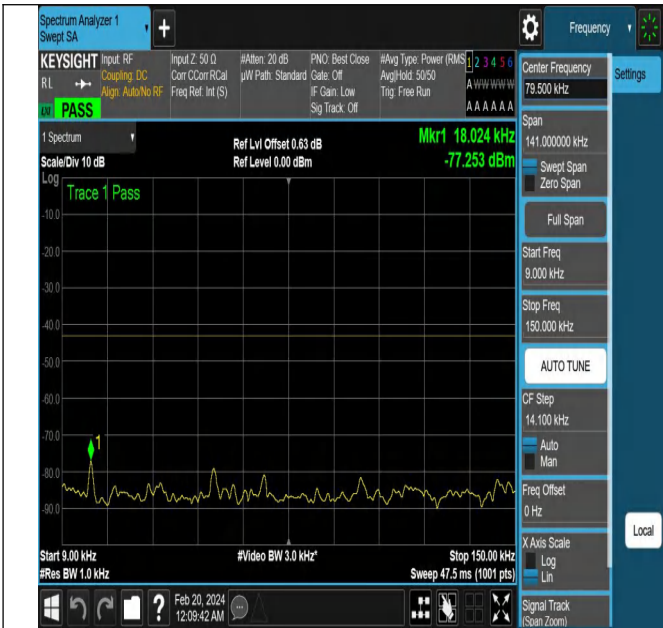
NTNV-N78-3700-3800-PC2-30-10-M-DFT-QPSK-Edge_1RB_ Left-Ant1-PASS
