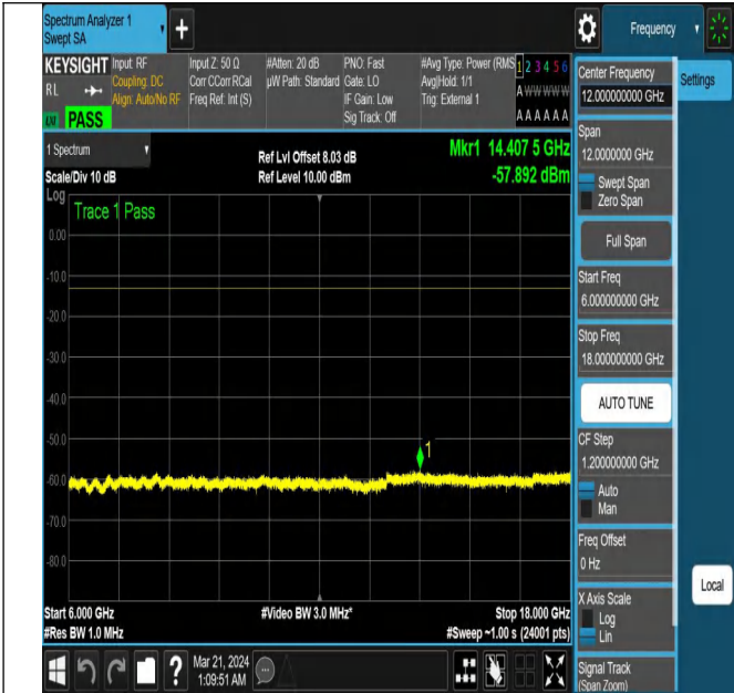
NTNV-N78-3700-3800-PC2-30-10-M-DFT-QPSK-Edge_1RB_
