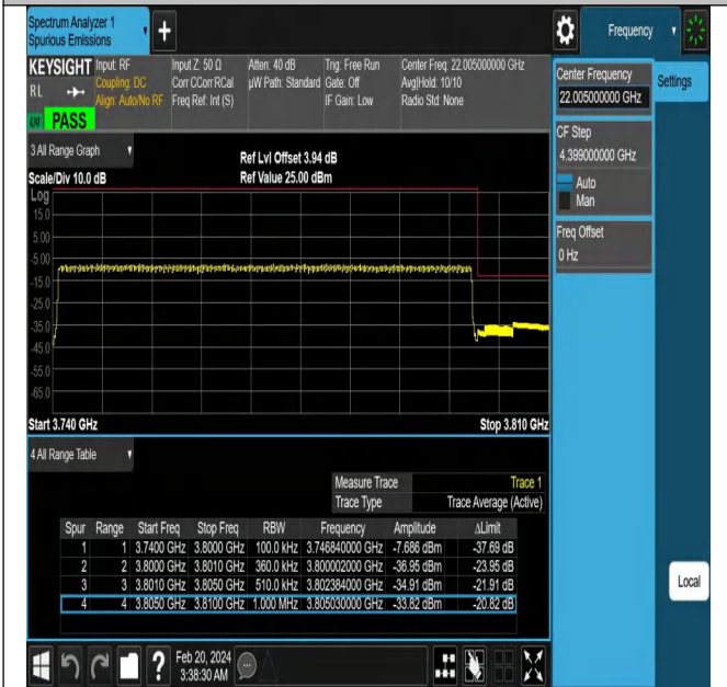
NTNV-N78-3700-3800-PC2-30-60-H-DFT-QPSK-Outer_Full -Ant1-PASS
