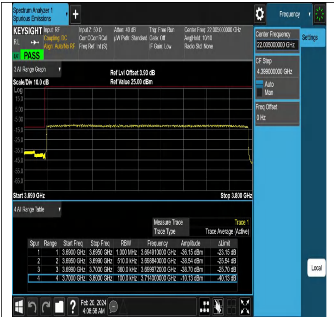
NTNV-N78-3700-3800-PC2-30-100-L-DFT-PI2BPSK-Outer_Full-Ant1-PASS
