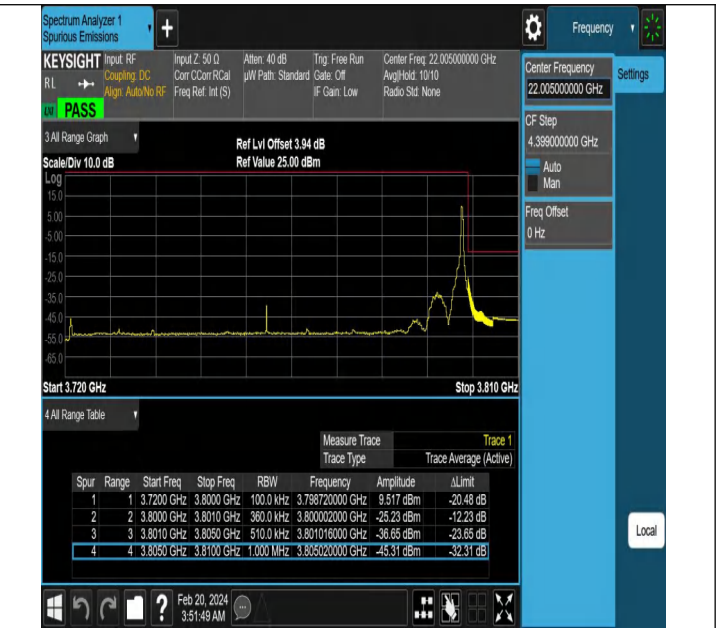
NTNV-N78-3700-3800-PC2-30-80-H-DFT-PI2BPSK-Edge_1RB_Right-Ant1-PASS
