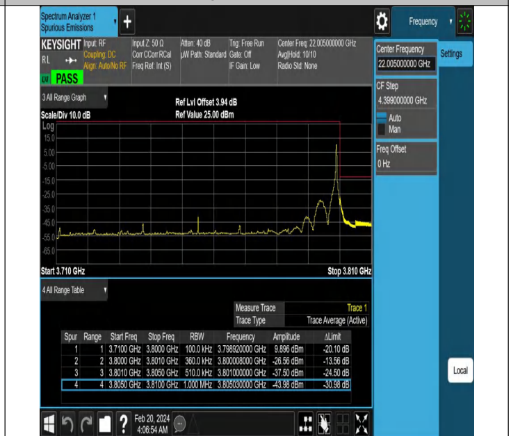
NTNV-N78-3700-3800-PC2-30-90-H-DFT-QPSK-Edge_1RB_Right-Ant1-PASS
