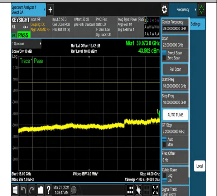
NTNV-N78-3700-3800-PC2-30-10-L-DFT-PI2BPSK-Edge_1R B_Right-Ant1-PASS
