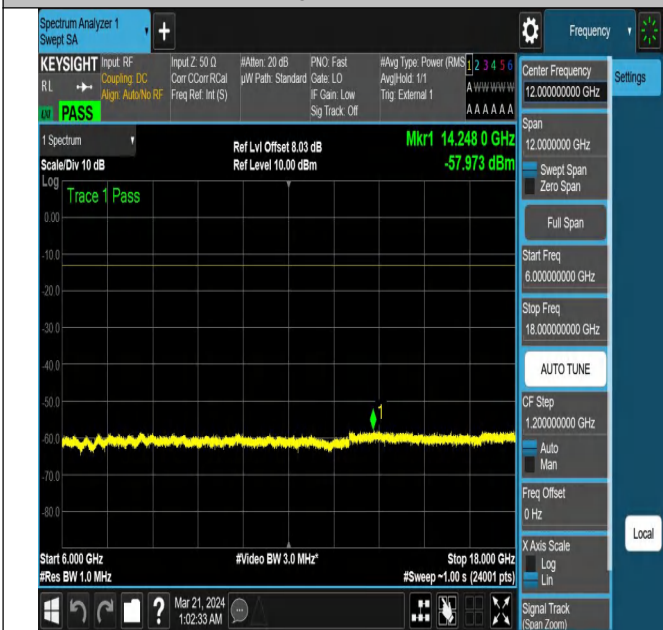
NTNV-N78-3700-3800-PC2-30-10-L-DFT-PI2BPSK-Edge_1R B_Right-Ant1-PASS
