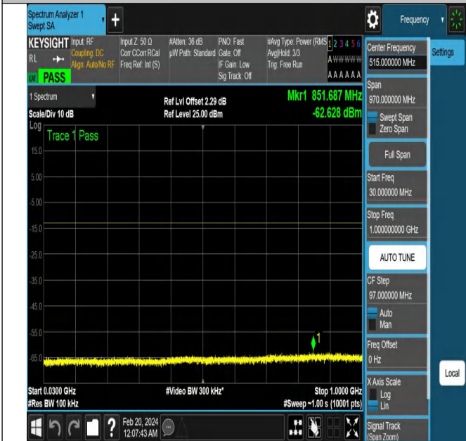
NTNV-N78-3700-3800-PC2-30-10-M-DFT-PI2BPSK-Edge_1R B_Left-Ant1-PASS
