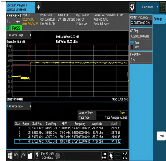
NTNV-N78-3700-3800-PC2-30-60-L-DFT-PI2BPSK-Outer_Full-Ant1-PASS
