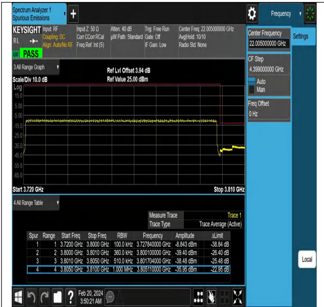
NTNV-N78-3700-3800-PC2-30-80-H-DFT-PI2BPSK-Outer_Full-Ant1-PASS
