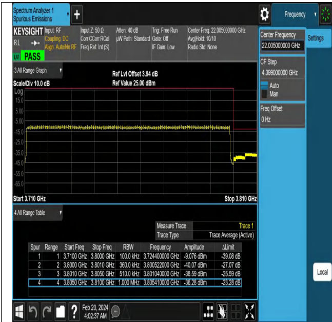
NTNV-N78-3700-3800-PC2-30-90-H-DFT-PI2BPSK-Outer_Full-Ant1-PASS
