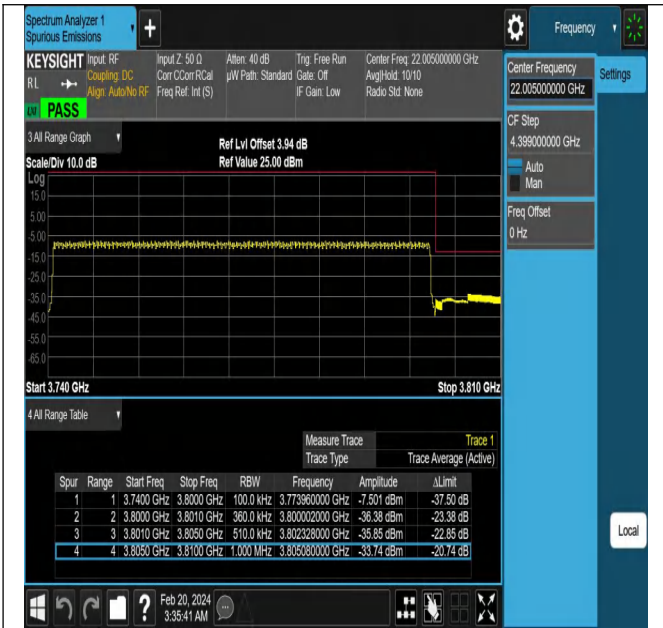
NTNV-N78-3700-3800-PC2-30-60-H-DFT-PI2BPSK-Outer_ Full-Ant1-PASS
