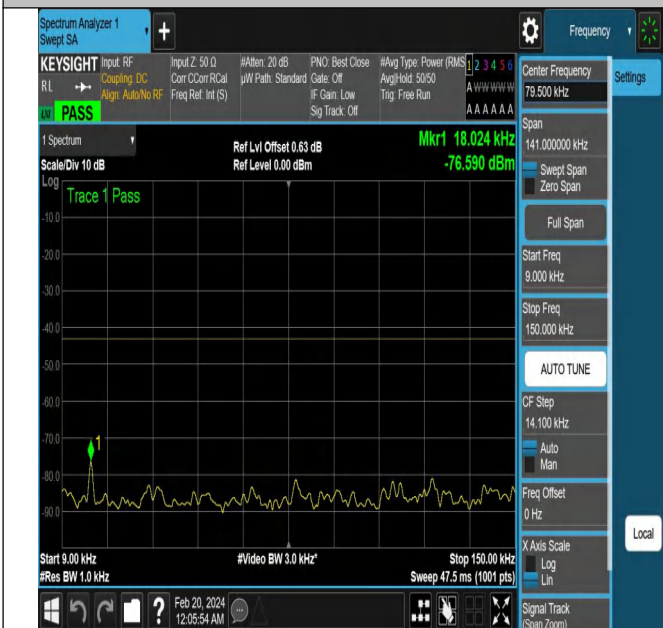
NTNV-N78-3700-3800-PC2-30-10-L-DFT-QPSK-Edge_1RB_ Right-Ant1-PASS
