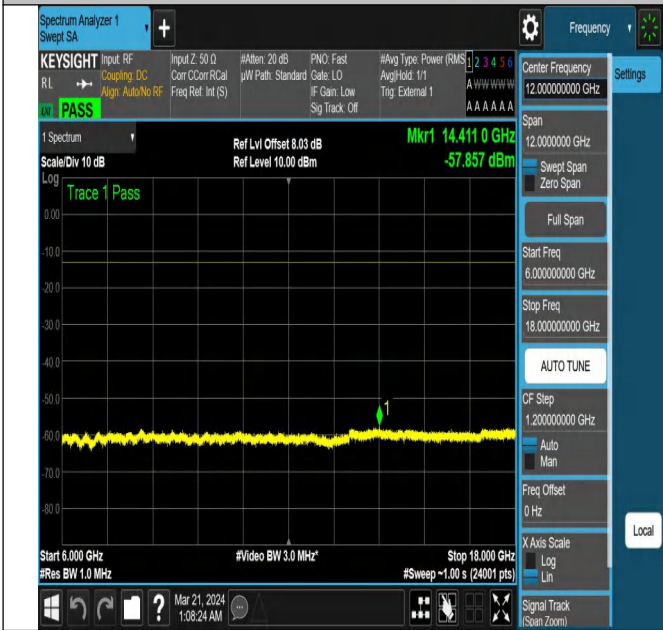
NTNV-N78-3700-3800-PC2-30-10-M-DFT-PI2BPSK-Edge_1R
