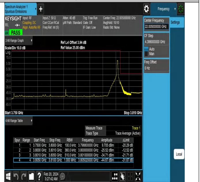
NTNV-N78-3700-3800-PC2-30-50-H-DFT-QPSK-Edge_1RB_Right-Ant1-PASS
