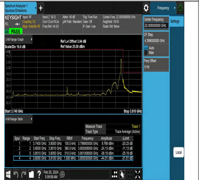
NTNV-N78-3700-3800-PC2-30-60-H-DFT-QPSK-Edge_1RB_Rig ht-Ant1-PASS
