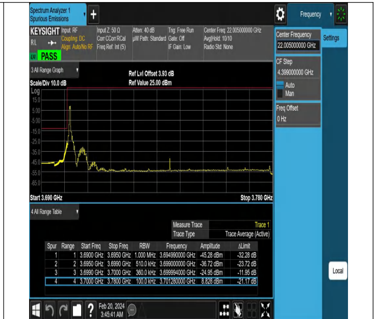
NTNV-N78-3700-3800-PC2-30-80-L-DFT-PI2BPSK-Edge_1RB_Left-Ant1-PASS
