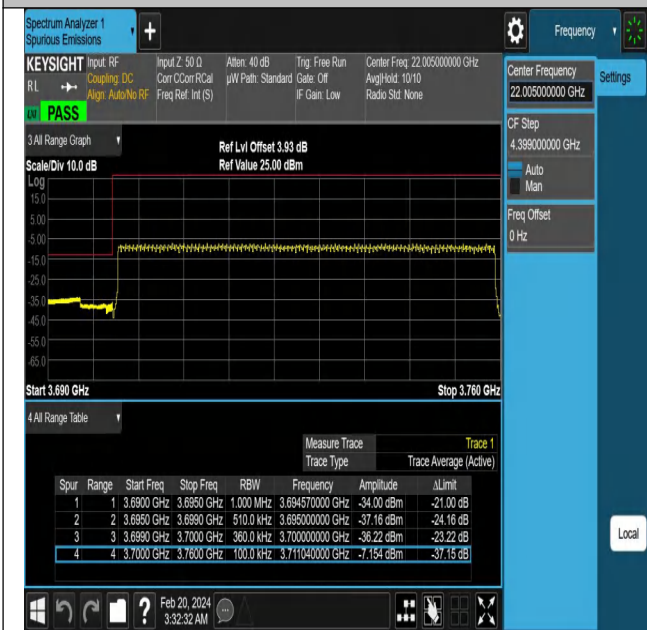
NTNV-N78-3700-3800-PC2-30-60-L-DFT-QPSK-Outer_Full-Ant1-PASS
