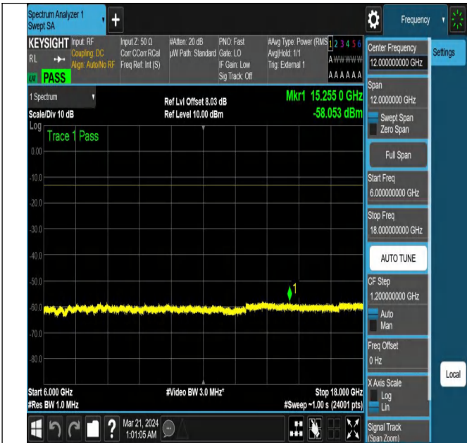
NTNV-N78-3700-3800-PC2-30-10-L-DFT-PI2BPSK-Edge_1R B_Left-Ant1-PASS
