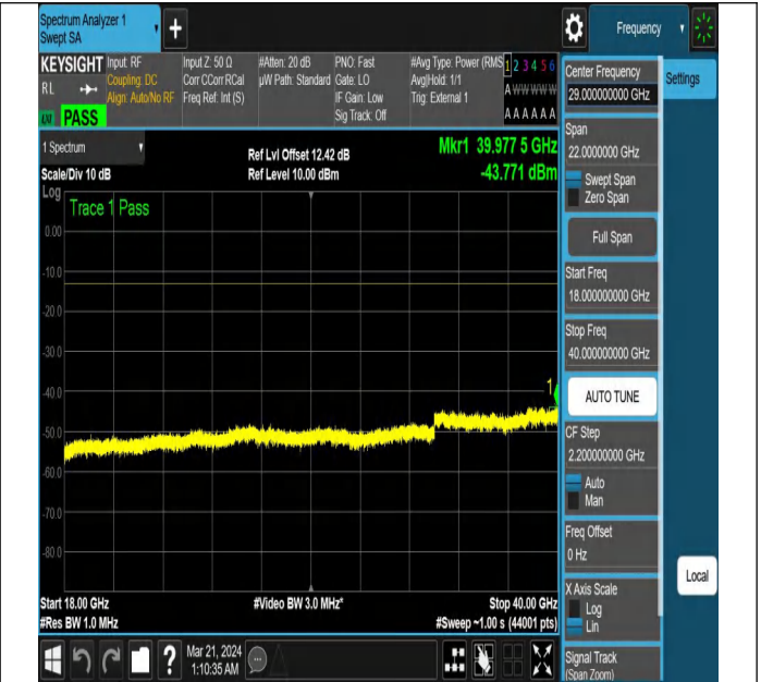
NTNV-N78-3700-3800-PC2-30-10-M-DFT-QPSK-Edge_1RB_
