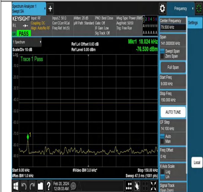
NTNV-N78-3700-3800-PC2-30-10-M-DFT-PI2BPSK-Edge_1R B_Right-Ant1-PASS
