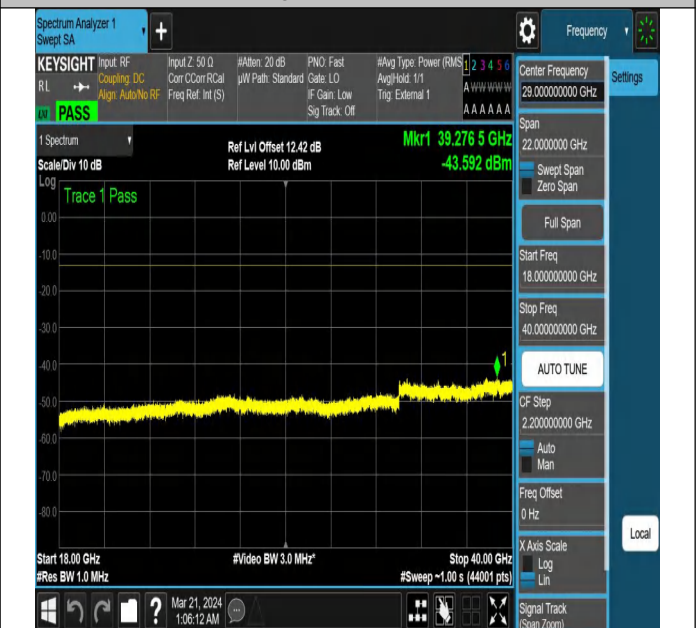
NTNV-N78-3700-3800-PC2-30-10-L-DFT-QPSK-Edge_1RB_
