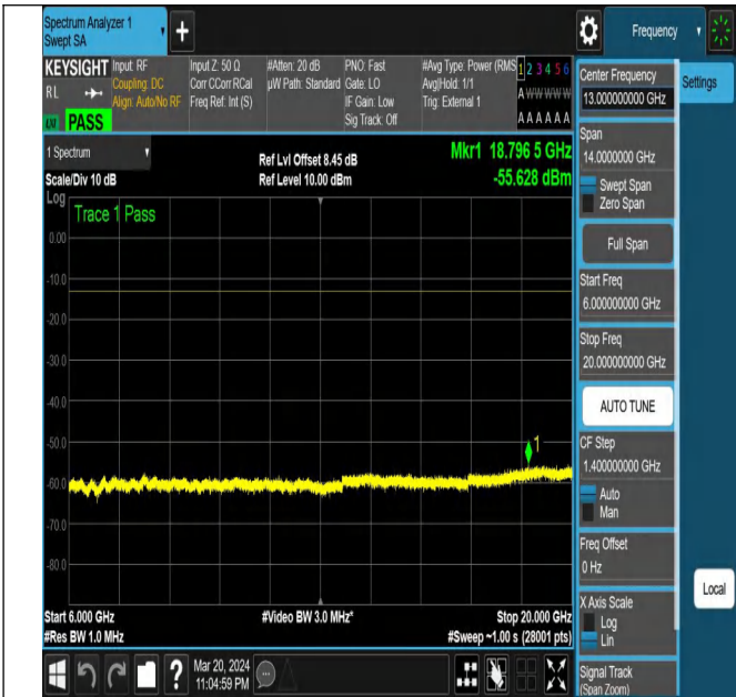
NTNV-N78-3450-3550-PC2-30-20-M-DFT-PI2BPSK-Edge_1R B_Right-Ant1-PASS
