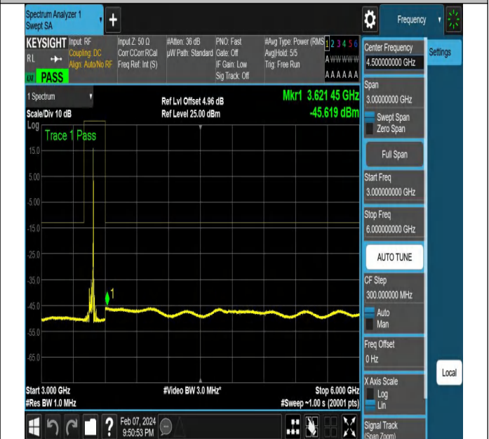
NTNV-N78-3450-3550-PC2-30-40-L-DFT-PI2BPSK-Edge_1R B_Right-Ant1-PASS
