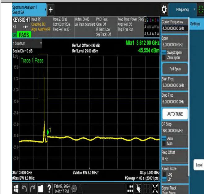
NTNV-N78-3450-3550-PC2-30-20-H-DFT-QPSK-Edge_1RB_ Left-Ant1-PASS
