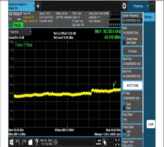
NTNV-N78-3450-3550-PC2-30-40-L-DFT-PI2BPSK-Edge_1R B_Right-Ant1-PASS
