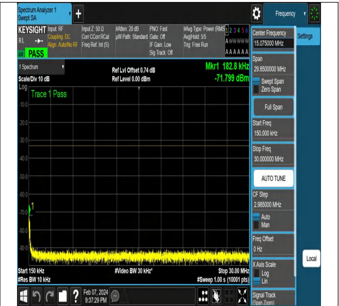
NTNV-N78-3450-3550-PC2-30-20-H-DFT-PI2BPSK-Edge_1R B_Left-Ant1-PASS
