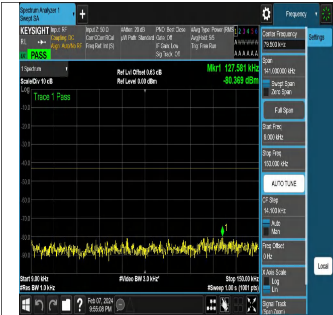
NTNV-N78-3450-3550-PC2-30-40-M-DFT-PI2BPSK-Edge_1R B_Left-Ant1-PASS
