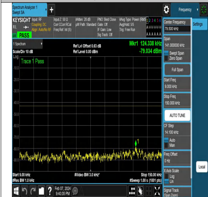
NTNV-N78-3450-3550-PC2-30-20-H-DFT-QPSK-Edge_1RB_ Left-Ant1-PASS
