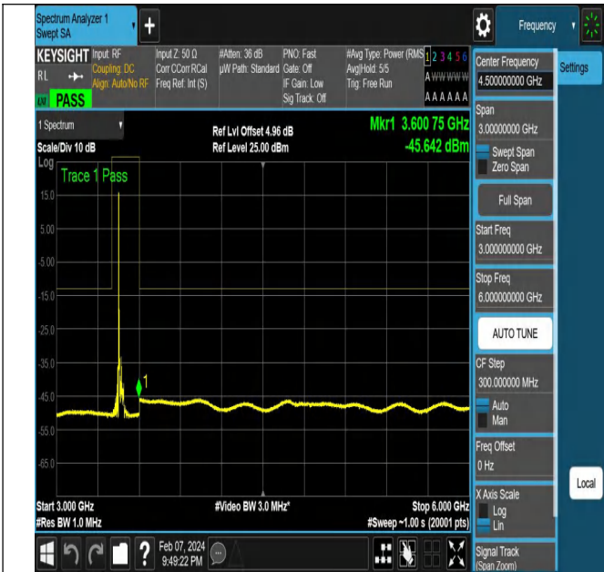
NTNV-N78-3450-3550-PC2-30-40-L-DFT-PI2BPSK-Edge_1R B_Left-Ant1-PASS
