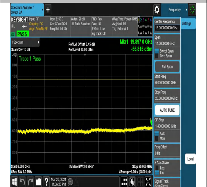
NTNV-N78-3450-3550-PC2-30-20-M-DFT-QPSK-Edge_1RB_ Left-Ant1-PASS
