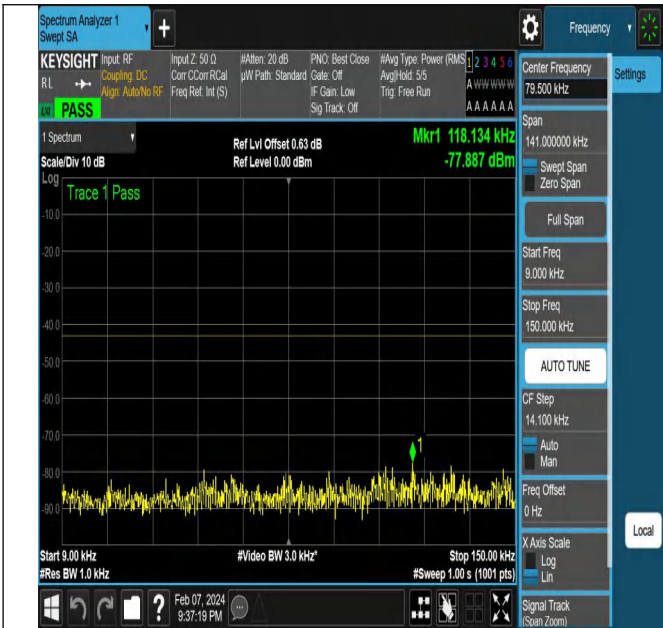
NTNV-N78-3450-3550-PC2-30-20-H-DFT-PI2BPSK-Edge_1R B_Left-Ant1-PASS
