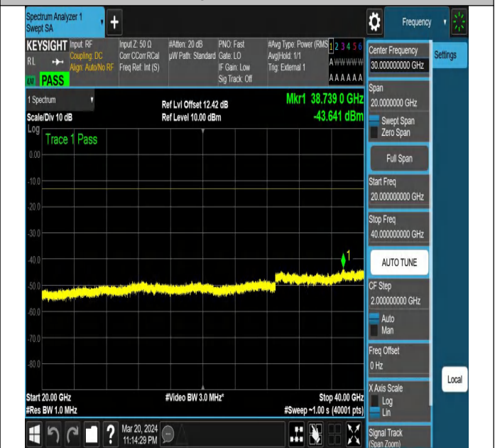
NTNV-N78-3450-3550-PC2-30-20-H-DFT-QPSK-Edge_1RB_ Right-Ant1-PASS
