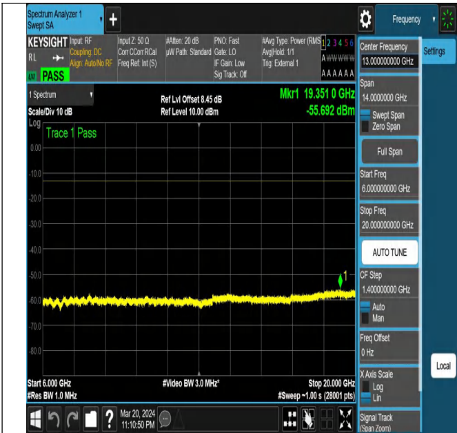
NTNV-N78-3450-3550-PC2-30-20-H-DFT-PI2BPSK-Edge_1R B_Right-Ant1-PASS
