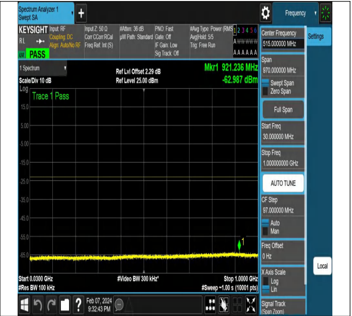
NTNV-N78-3450-3550-PC2-30-20-M-DFT-PI2BPSK-Edge_1R
