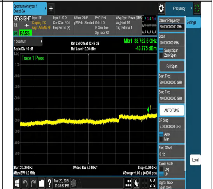
NTNV-N78-3450-3550-PC2-30-20-M-DFT-QPSK-Edge_1RB_ Right-Ant1-PASS
