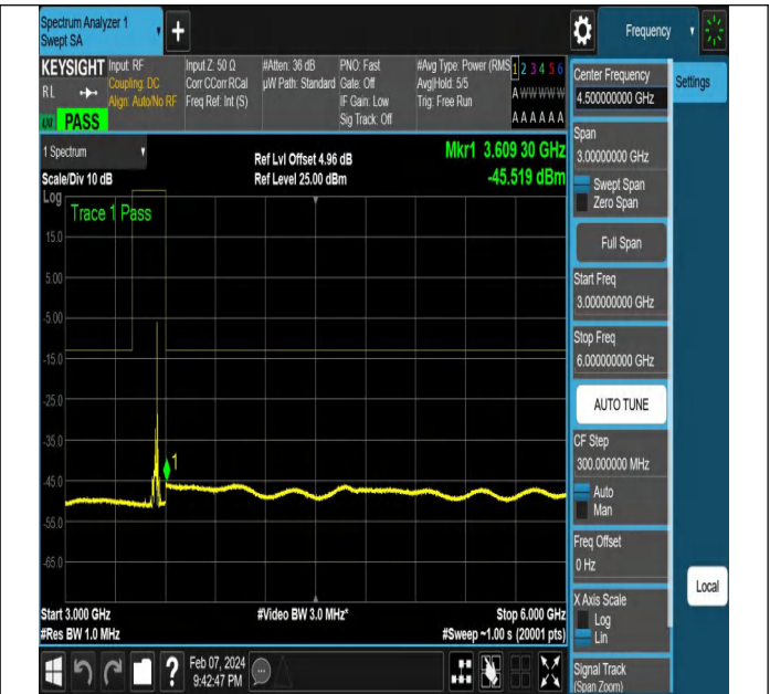
NTNV-N78-3450-3550-PC2-30-20-H-DFT-QPSK-Edge_1RB_ Right-Ant1-PASS
