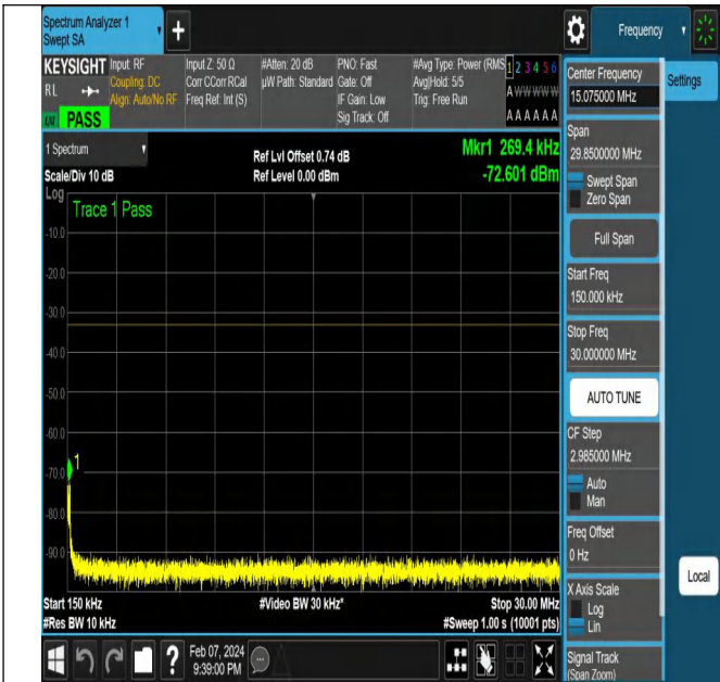
NTNV-N78-3450-3550-PC2-30-20-H-DFT-PI2BPSK-Edge_1R
