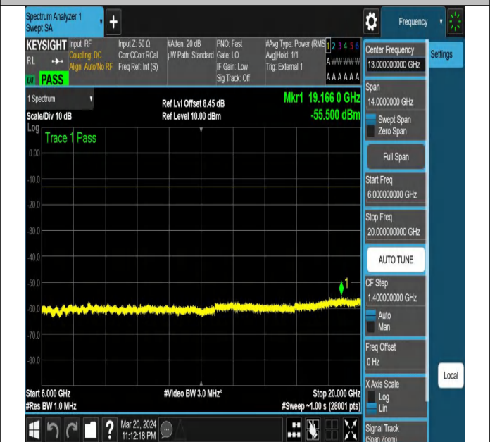
NTNV-N78-3450-3550-PC2-30-20-H-DFT-QPSK-Edge_1RB_ Left-Ant1-PASS
