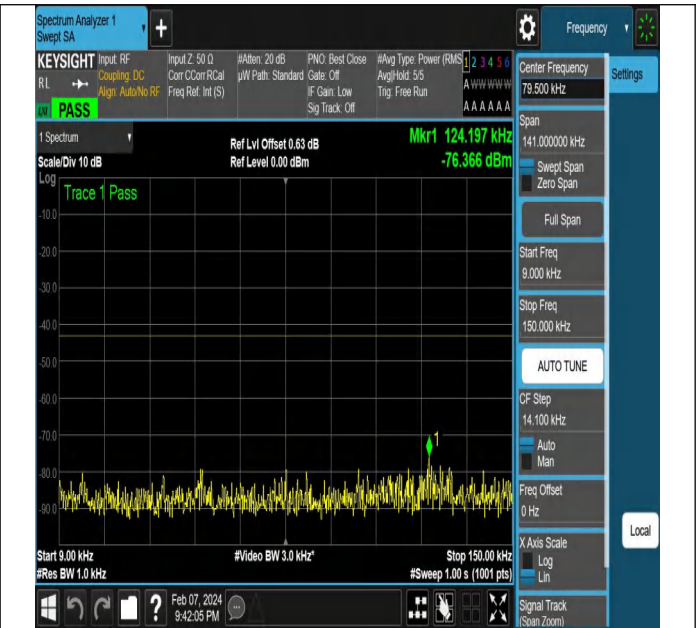
NTNV-N78-3450-3550-PC2-30-20-H-DFT-QPSK-Edge_1RB_
