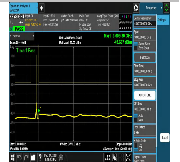
NTNV-N78-3450-3550-PC2-30-20-H-DFT-PI2BPSK-Edge_1R
