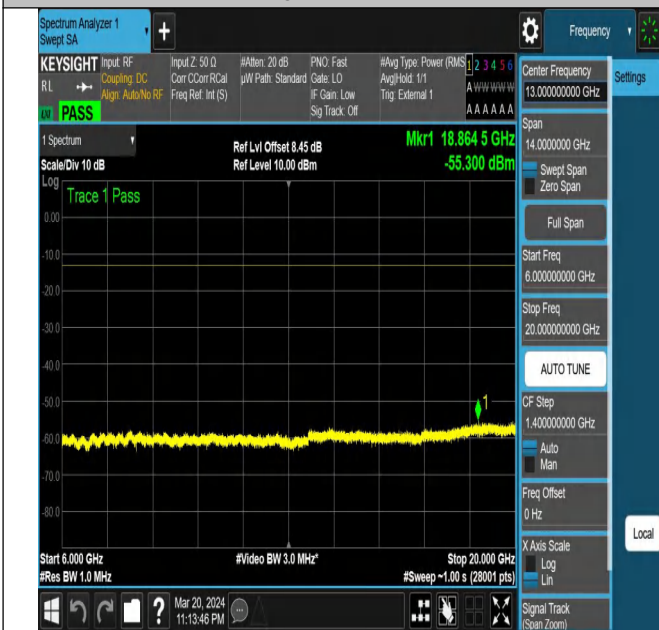
NTNV-N78-3450-3550-PC2-30-20-H-DFT-QPSK-Edge_1RB_ Right-Ant1-PASS
