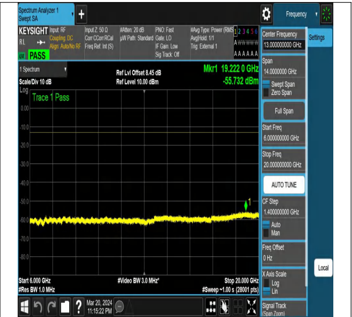
NTNV-N78-3450-3550-PC2-30-40-L-DFT-PI2BPSK-Edge_1R B_Left-Ant1-PASS
