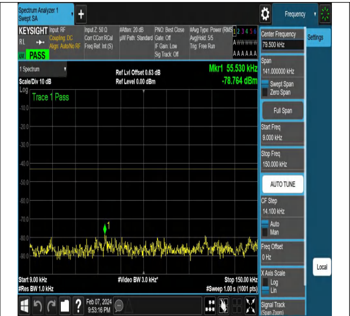
NTNV-N78-3450-3550-PC2-30-40-L-DFT-QPSK-Edge_1RB_ Right-Ant1-PASS
