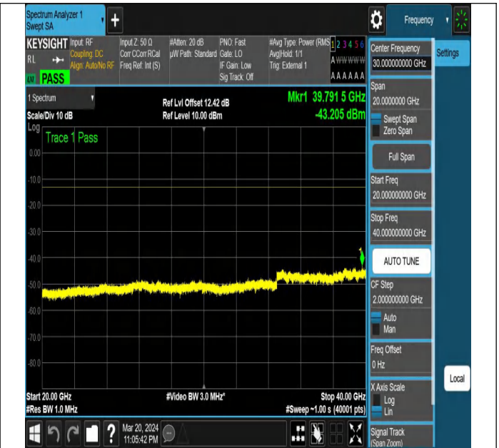
NTNV-N78-3450-3550-PC2-30-20-M-DFT-PI2BPSK-Edge_1R B_Right-Ant1-PASS
