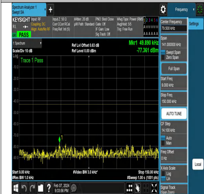
NTNV-N78-3450-3550-PC2-30-20-M-DFT-QPSK-Edge_1RB_ Left-Ant1-PASS
