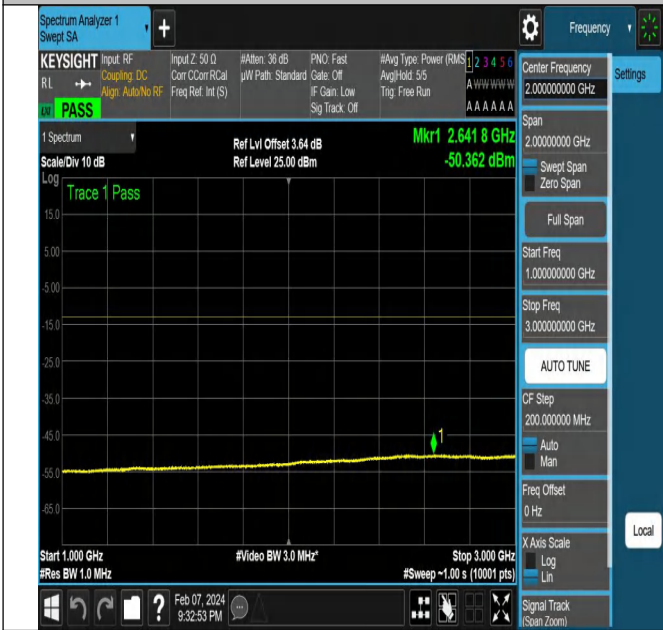
NTNV-N78-3450-3550-PC2-30-20-M-DFT-PI2BPSK-Edge_1R
