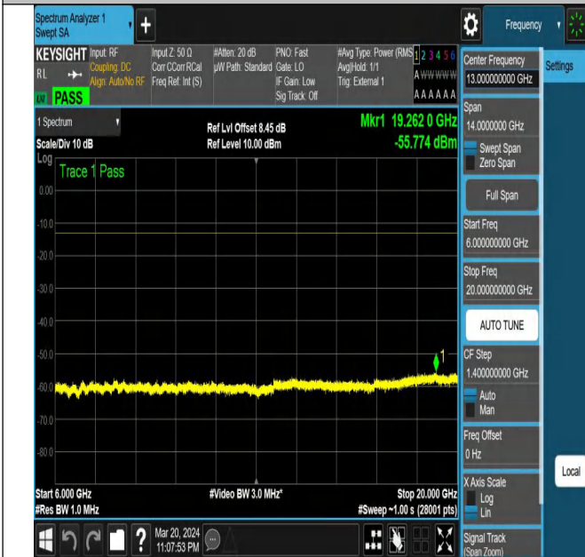
NTNV-N78-3450-3550-PC2-30-20-M-DFT-QPSK-Edge_1RB_ Right-Ant1-PASS
