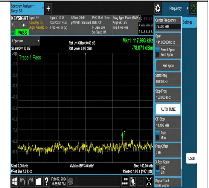
NTNV-N78-3450-3550-PC2-30-20-H-DFT-PI2BPSK-Edge_1R B_Right-Ant1-PASS
