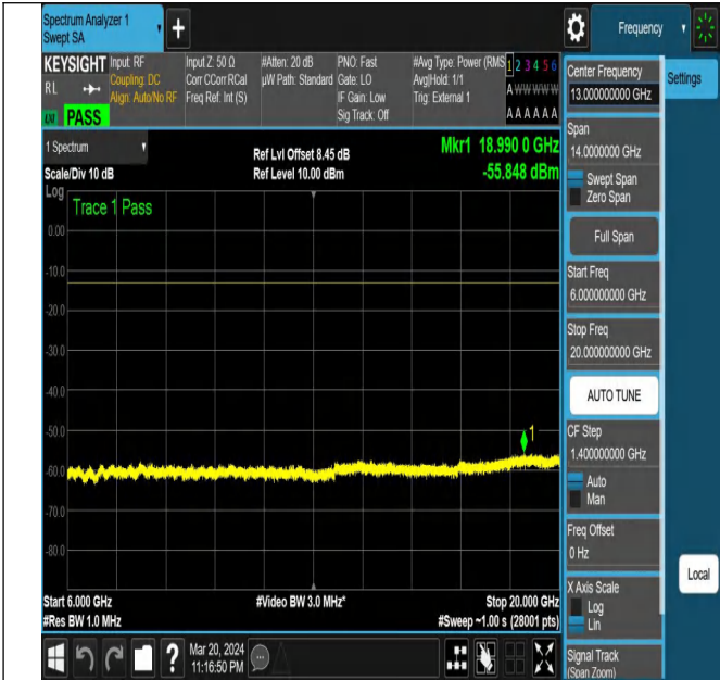
NTNV-N78-3450-3550-PC2-30-40-L-DFT-PI2BPSK-Edge_1R B_Right-Ant1-PASS
