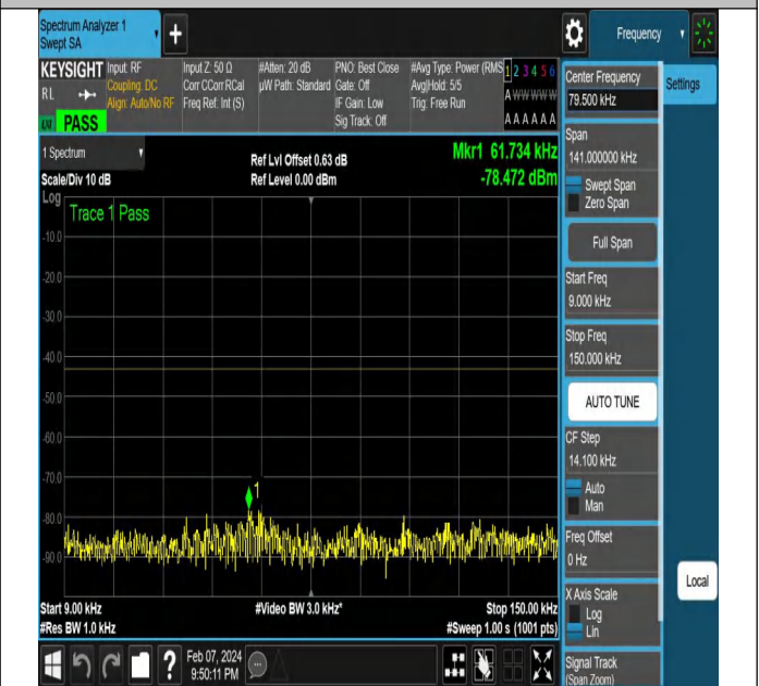
NTNV-N78-3450-3550-PC2-30-40-L-DFT-PI2BPSK-Edge_1R B_Right-Ant1-PASS
