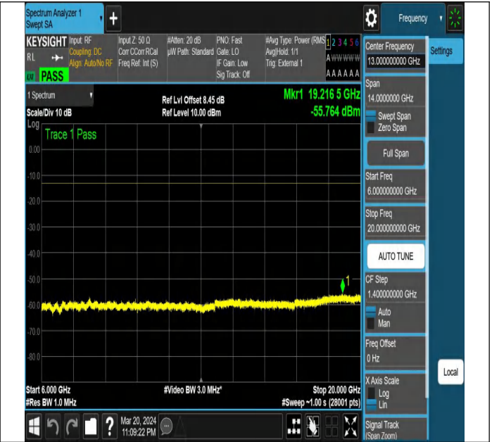
NTNV-N78-3450-3550-PC2-30-20-H-DFT-PI2BPSK-Edge_1R B_Left-Ant1-PASS
