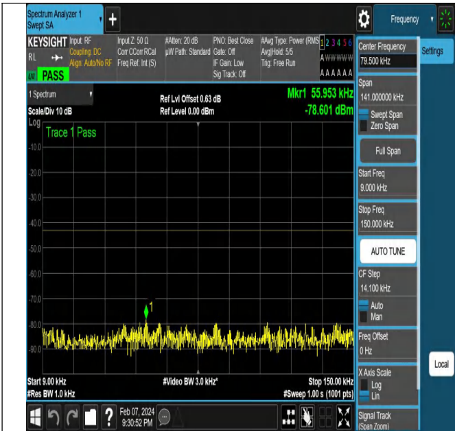
NTNV-N78-3450-3550-PC2-30-20-M-DFT-PI2BPSK-Edge_1R B_Left-Ant1-PASS
