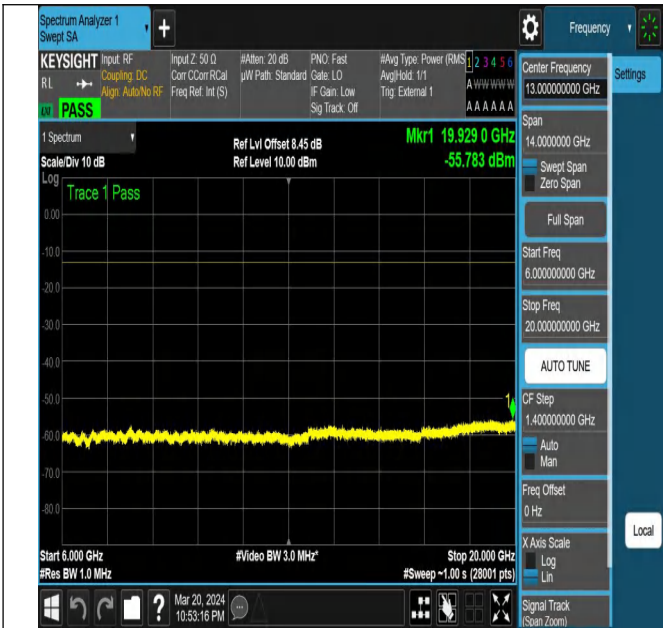
NTNV-N78-3450-3550-PC2-30-15-H-DFT-PI2BPSK-Edge_1R B_Right-Ant1-PASS
