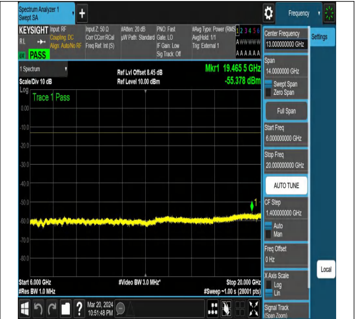
NTNV-N78-3450-3550-PC2-30-15-H-DFT-PI2BPSK-Edge_1R B_Left-Ant1-PASS
