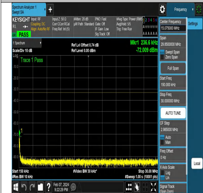
NTNV-N78-3450-3550-PC2-30-15-H-DFT-QPSK-Edge_1RB_ Right-Ant1-PASS
