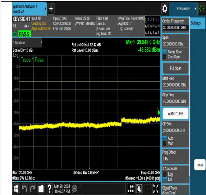
NTNV-N78-3450-3550-PC2-30-15-M-DFT-QPSK-Edge_1RB_ Left-Ant1-PASS
