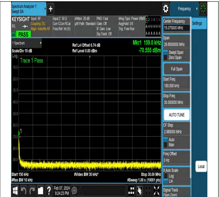
NTNV-N78-3450-3550-PC2-30-20-L-DFT-PI2BPSK-Edge_1R B_Left-Ant1-PASS
