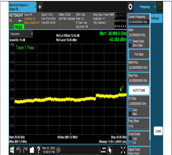
NTNV-N78-3450-3550-PC2-30-20-L-DFT-PI2BPSK-Edge_1R B_Right-Ant1-PASS
