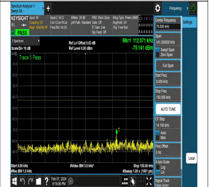
NTNV-N78-3450-3550-PC2-30-15-H-DFT-PI2BPSK-Edge_1R B_Right-Ant1-PASS
