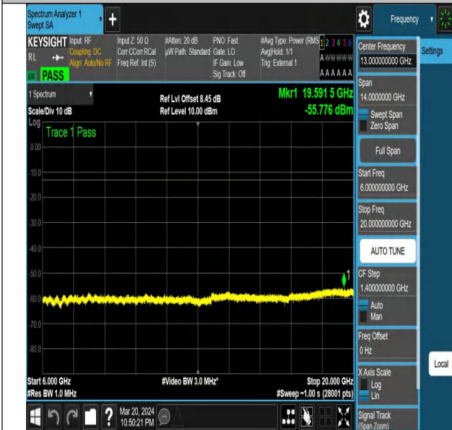
NTNV-N78-3450-3550-PC2-30-15-M-DFT-QPSK-Edge_1RB_ Right-Ant1-PASS
