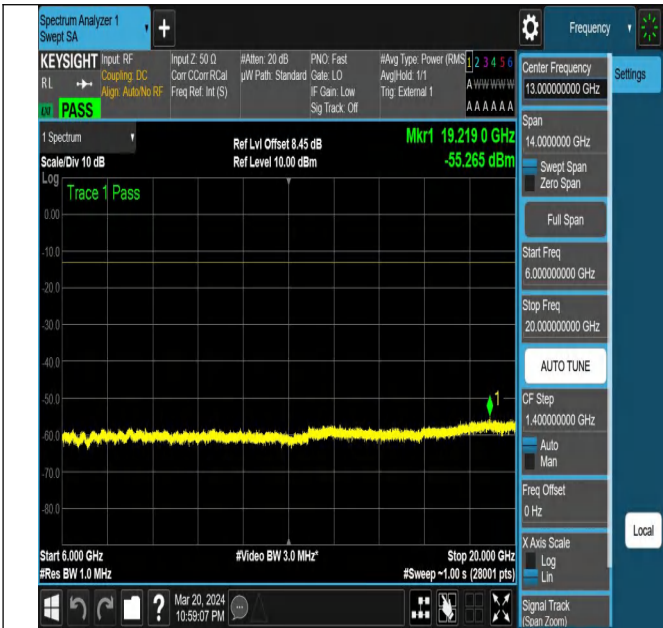
NTNV-N78-3450-3550-PC2-30-20-L-DFT-PI2BPSK-Edge_1R B_Right-Ant1-PASS
