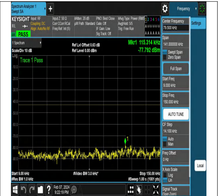
NTNV-N78-3450-3550-PC2-30-15-H-DFT-QPSK-Edge_1RB_ Right-Ant1-PASS
