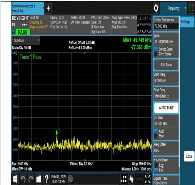
NTNV-N78-3450-3550-PC2-30-20-L-DFT-PI2BPSK-Edge_1R B_Left-Ant1-PASS
