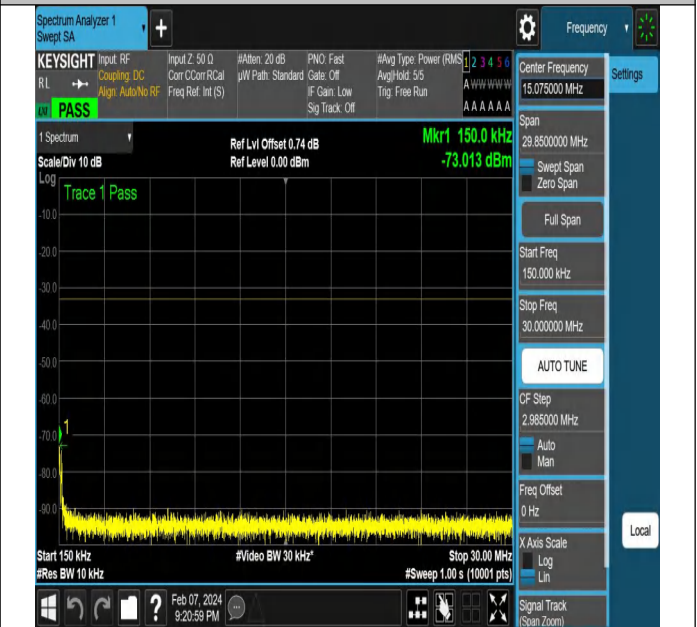
NTNV-N78-3450-3550-PC2-30-15-H-DFT-QPSK-Edge_1RB_ Left-Ant1-PASS
