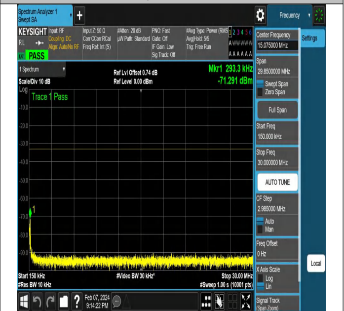
NTNV-N78-3450-3550-PC2-30-15-M-DFT-QPSK-Edge_1RB_ Left-Ant1-PASS
