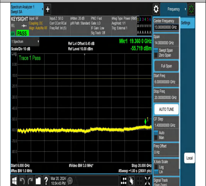
NTNV-N78-3450-3550-PC2-30-15-H-DFT-QPSK-Edge_1RB_
