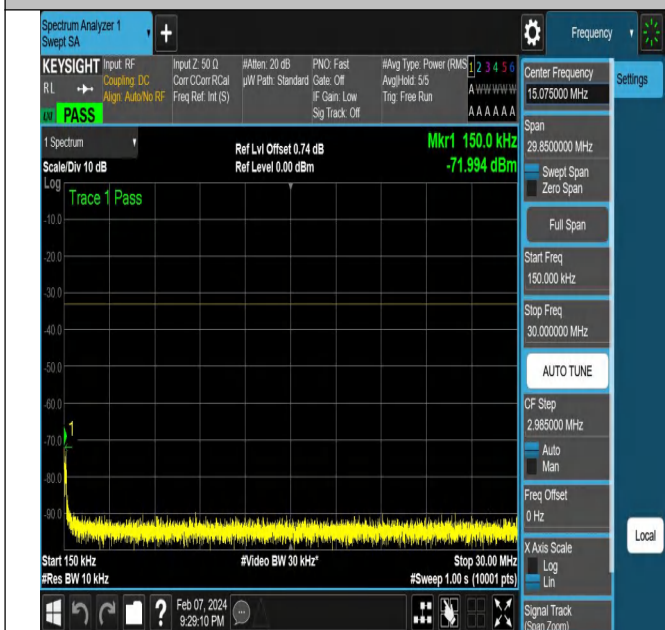
NTNV-N78-3450-3550-PC2-30-20-L-DFT-QPSK-Edge_1RB_ Right-Ant1-PASS
