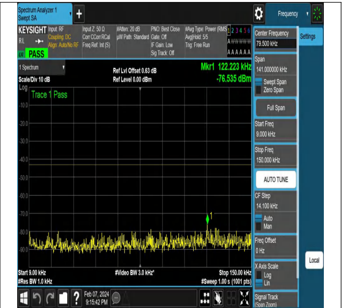
NTNV-N78-3450-3550-PC2-30-15-M-DFT-QPSK-Edge_1RB_ Right-Ant1-PASS
