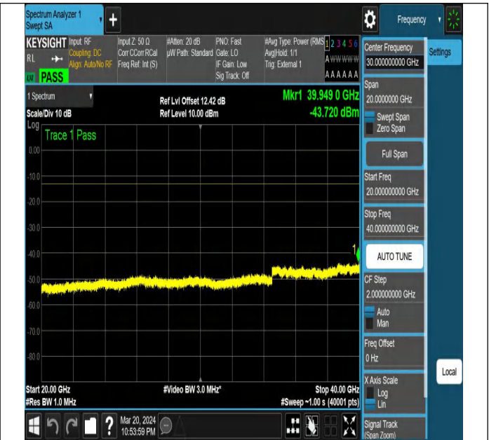
NTNV-N78-3450-3550-PC2-30-15-H-DFT-PI2BPSK-Edge_1R B_Right-Ant1-PASS
