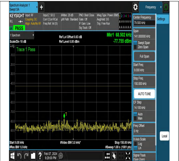
NTNV-N78-3450-3550-PC2-30-20-L-DFT-QPSK-Edge_1RB_ Right-Ant1-PASS
