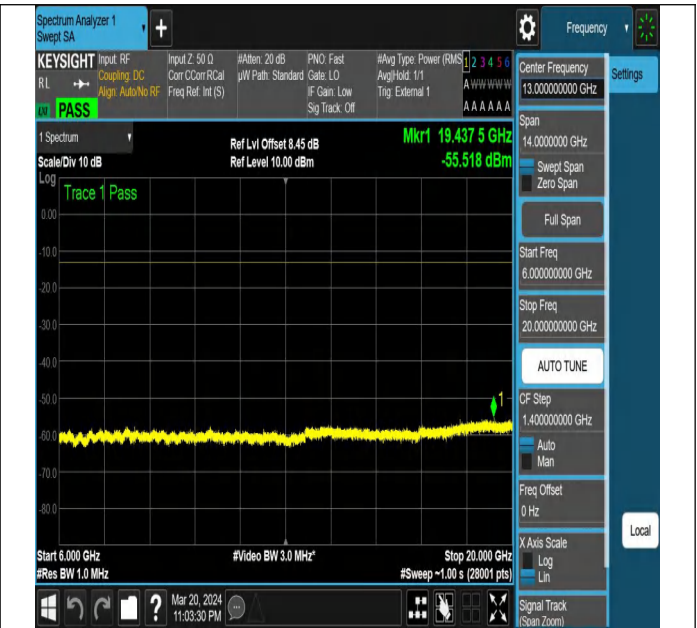
NTNV-N78-3450-3550-PC2-30-20-M-DFT-PI2BPSK-Edge_1R B_Left-Ant1-PASS
