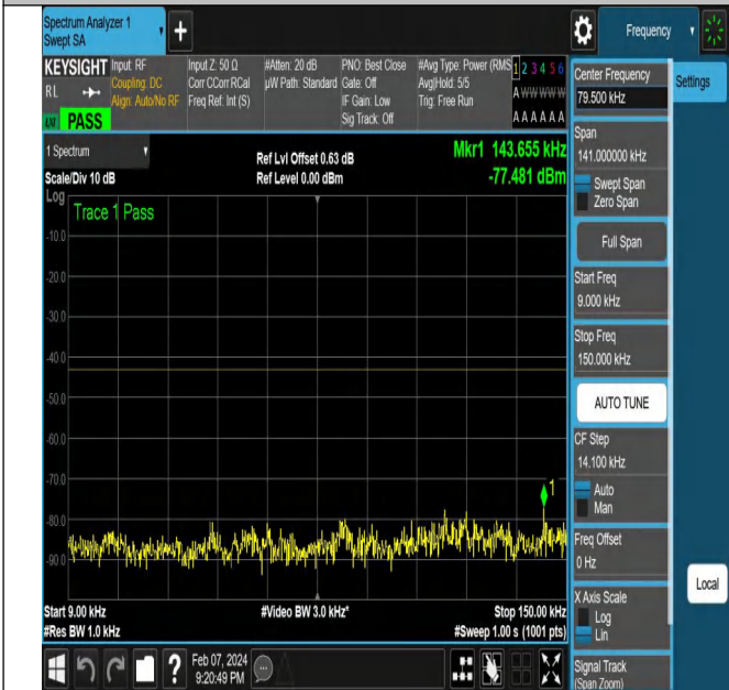
NTNV-N78-3450-3550-PC2-30-15-H-DFT-QPSK-Edge_1RB_ Left-Ant1-PASS
