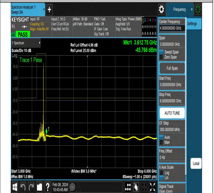
NTNV-N78-3450-3550-PC2-30-90-H-DFT-PI2BPSK-Edge_1R B_Right-Ant1-PASS
