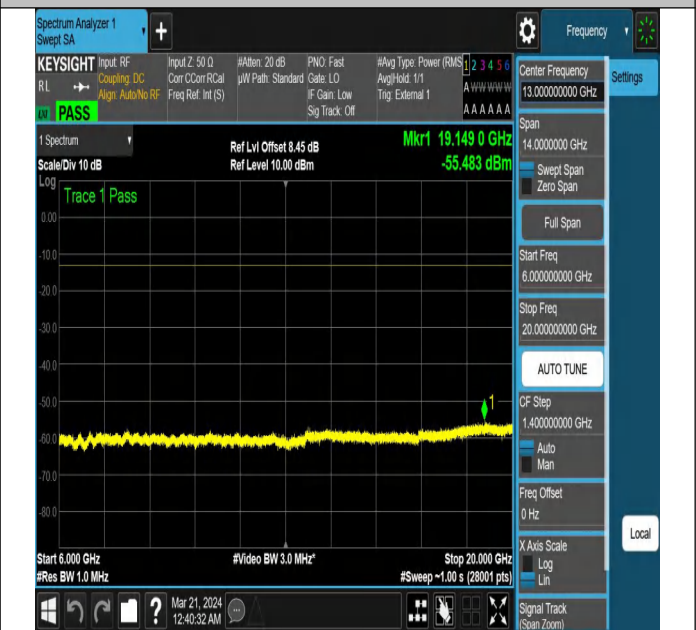
NTNV-N78-3450-3550-PC2-30-90-H-DFT-QPSK-Edge_1RB_
