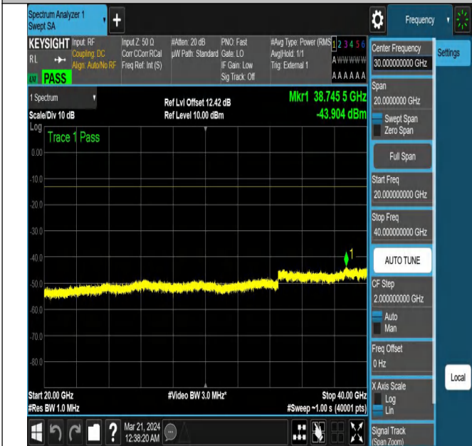
NTNV-N78-3450-3550-PC2-30-90-H-DFT-PI2BPSK-Edge_1R B_Left-Ant1-PASS
