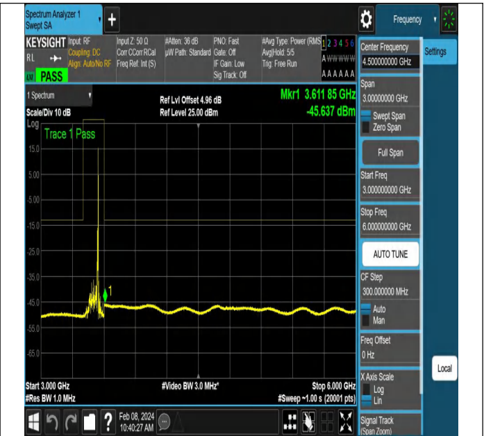
NTNV-N78-3450-3550-PC2-30-90-M-DFT-QPSK-Edge_1RB_ Right-Ant1-PASS
