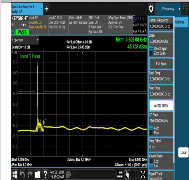
NTNV-N78-3450-3550-PC2-30-90-H-DFT-QPSK-Edge_1RB_
