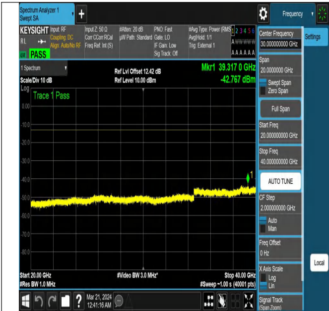
NTNV-N78-3450-3550-PC2-30-90-H-DFT-QPSK-Edge_1RB_ Left-Ant1-PASS
