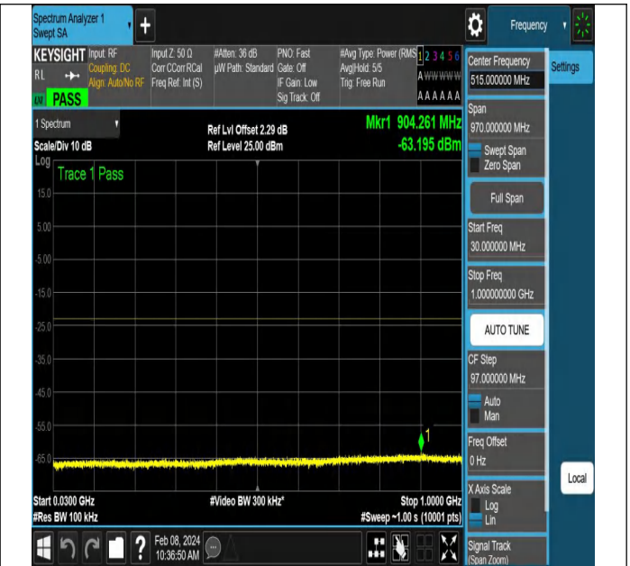
NTNV-N78-3450-3550-PC2-30-90-M-DFT-PI2BPSK-Edge_1R B_Right-Ant1-PASS
