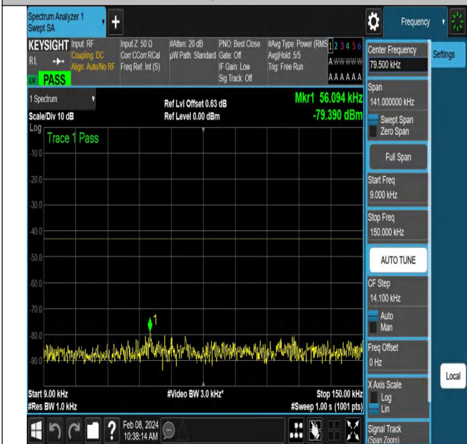
NTNV-N78-3450-3550-PC2-30-90-M-DFT-QPSK-Edge_1RB_ Left-Ant1-PASS
