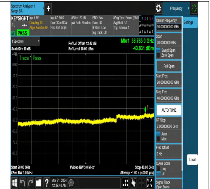
NTNV-N78-3450-3550-PC2-30-90-H-DFT-PI2BPSK-Edge_1R B_Right-Ant1-PASS
