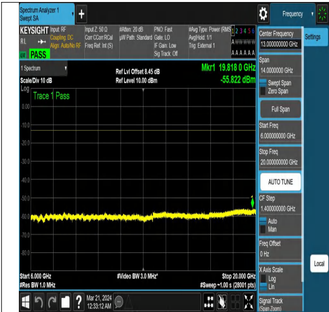
NTNV-N78-3450-3550-PC2-30-90-M-DFT-PI2BPSK-Edge_1R B_Right-Ant1-PASS
