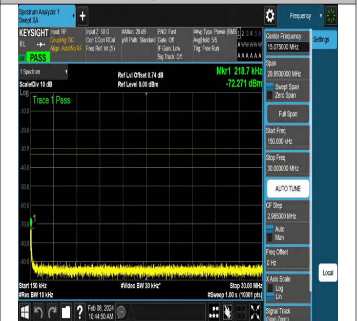
NTNV-N78-3450-3550-PC2-30-90-H-DFT-QPSK-Edge_1RB_ Left-Ant1-PASS
