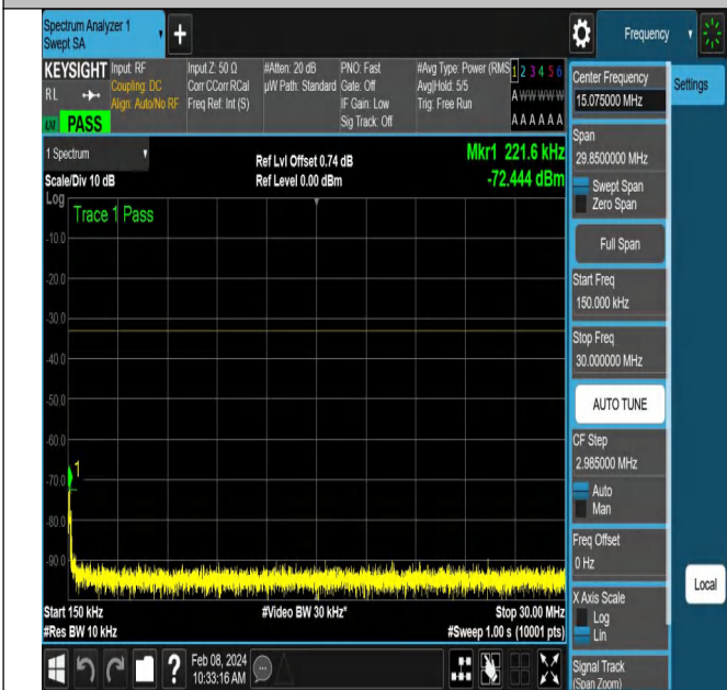
NTNV-N78-3450-3550-PC2-30-90-L-DFT-QPSK-Edge_1RB_ Right-Ant1-PASS
