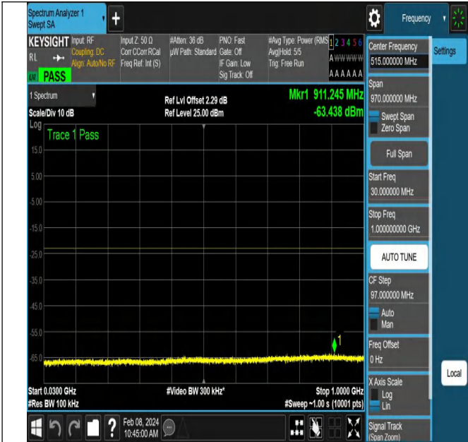
NTNV-N78-3450-3550-PC2-30-90-H-DFT-QPSK-Edge_1RB_
