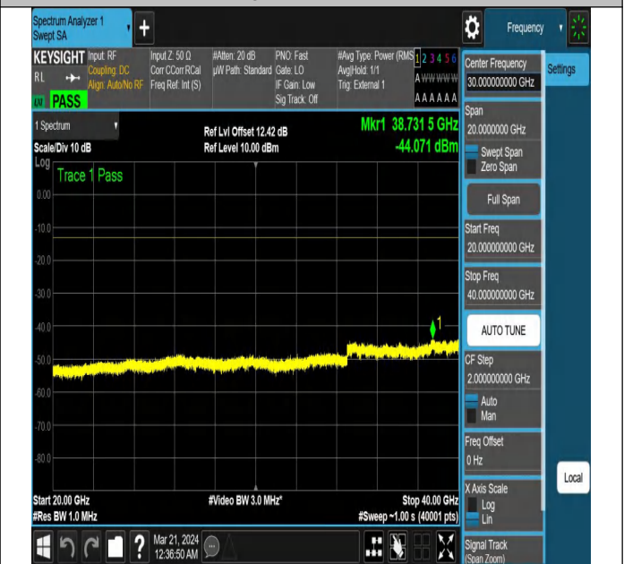
NTNV-N78-3450-3550-PC2-30-90-M-DFT-QPSK-Edge_1RB_ Right-Ant1-PASS
