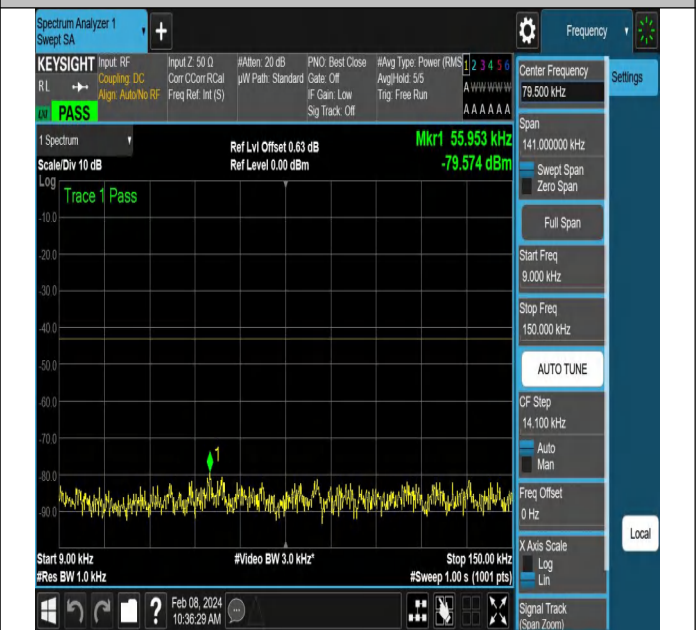
NTNV-N78-3450-3550-PC2-30-90-M-DFT-PI2BPSK-Edge_1R B_Right-Ant1-PASS
