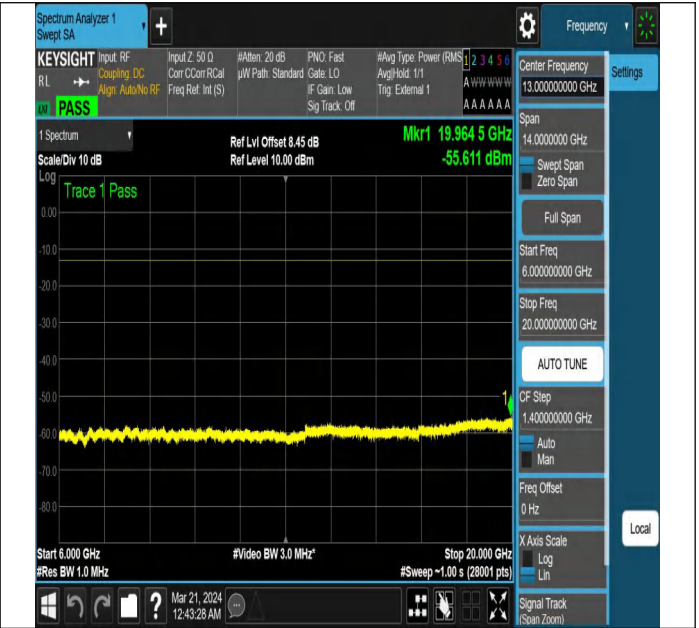
NTNV-N78-3450-3550-PC2-30-100-L-DFT-PI2BPSK-Edge_1
