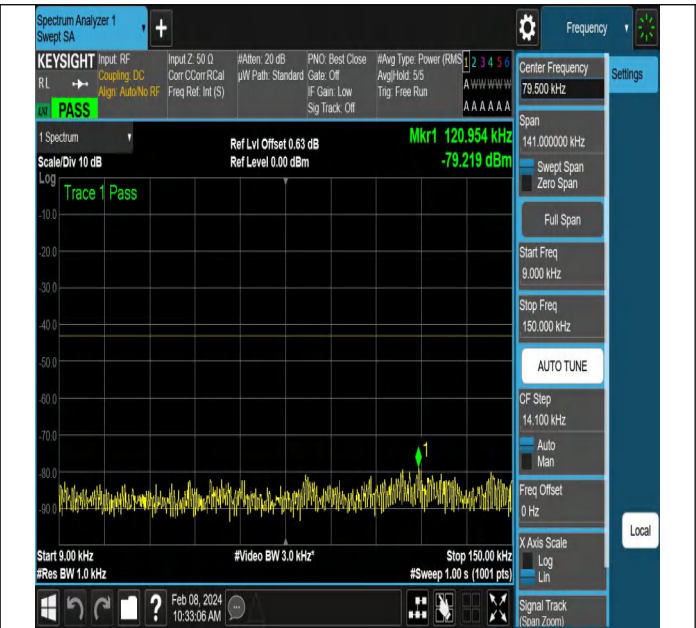
NTNV-N78-3450-3550-PC2-30-90-L-DFT-QPSK-Edge_1RB_ Right-Ant1-PASS
