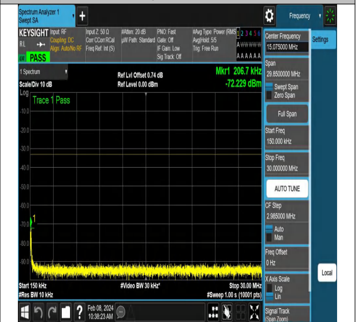
NTNV-N78-3450-3550-PC2-30-90-M-DFT-QPSK-Edge_1RB_ Left-Ant1-PASS
