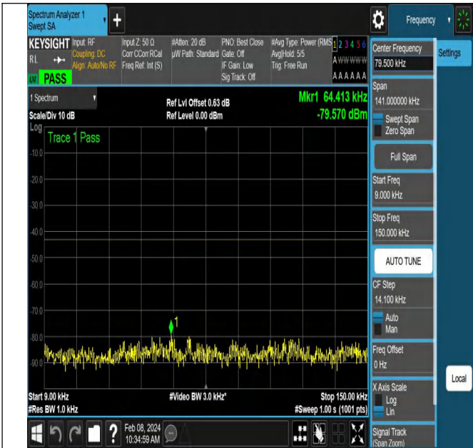
NTNV-N78-3450-3550-PC2-30-90-M-DFT-PI2BPSK-Edge_1R B_Left-Ant1-PASS
