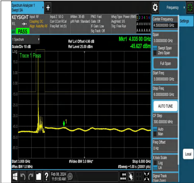
NTNV-N78-3450-3550-PC2-30-100-L-DFT-PI2BPSK-Edge_1
