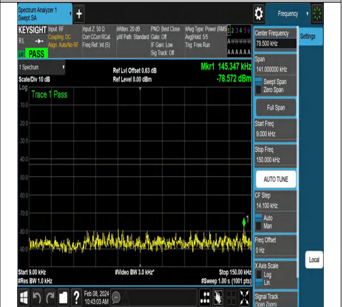
NTNV-N78-3450-3550-PC2-30-90-H-DFT-PI2BPSK-Edge_1R B_Right-Ant1-PASS
