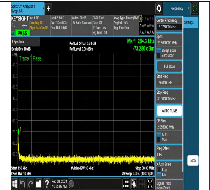
NTNV-N78-3450-3550-PC2-30-90-M-DFT-PI2BPSK-Edge_1R B_Left-Ant1-PASS
