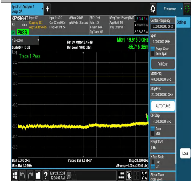
NTNV-N78-3450-3550-PC2-30-90-M-DFT-QPSK-Edge_1RB_ Right-Ant1-PASS
