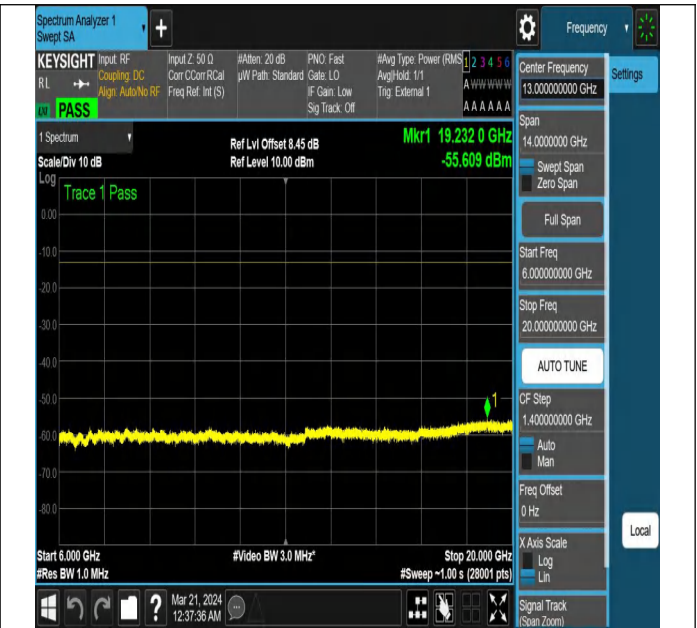
NTNV-N78-3450-3550-PC2-30-90-H-DFT-PI2BPSK-Edge_1R B_Left-Ant1-PASS
