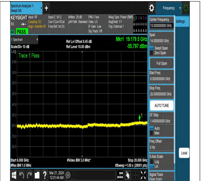
NTNV-N78-3450-3550-PC2-30-90-M-DFT-PI2BPSK-Edge_1R B_Left-Ant1-PASS
