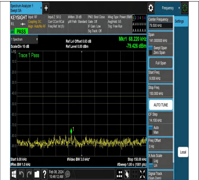
NTNV-N78-3450-3550-PC2-30-90-H-DFT-QPSK-Edge_1RB_ Right-Ant1-PASS
