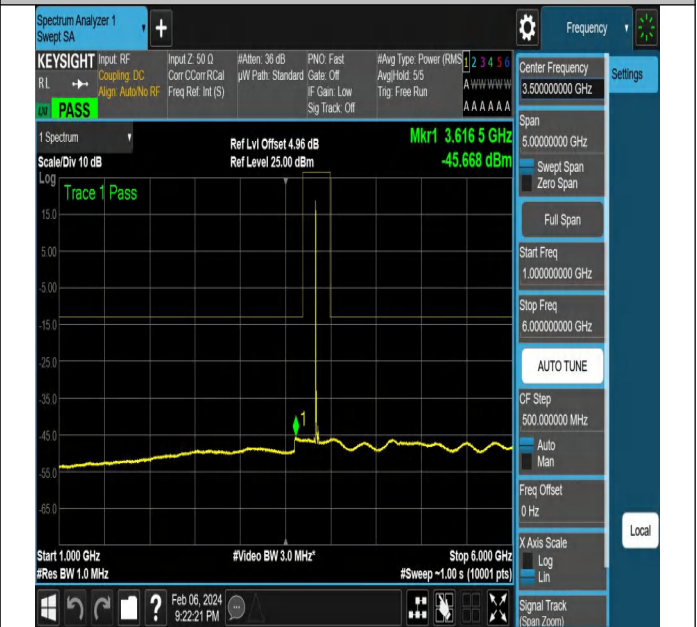
NTNV-N77-3700-3980-PC2-30-20-M-DFT-PI2BPSK-Edge_1R B_Left-Ant1-PASS
