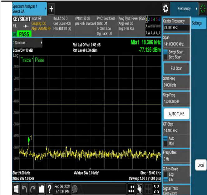
NTNV-N77-3700-3980-PC2-30-15-H-DFT-PI2BPSK-Edge_1R B_Right-Ant1-PASS
