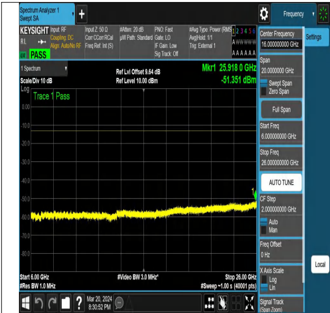
NTNV-N77-3700-3980-PC2-30-20-H-DFT-PI2BPSK-Edge_1R B_Left-Ant1-PASS
