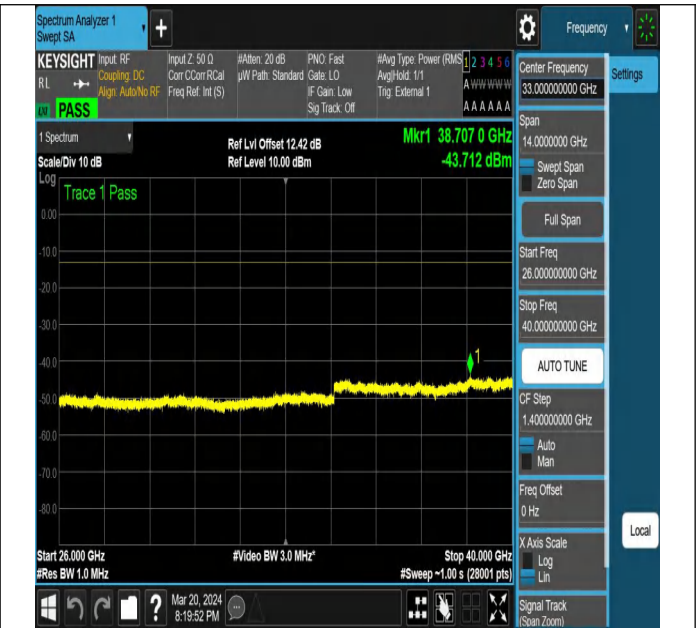
NTNV-N77-3700-3980-PC2-30-20-L-DFT-PI2BPSK-Edge_1R B_Left-Ant1-PASS
