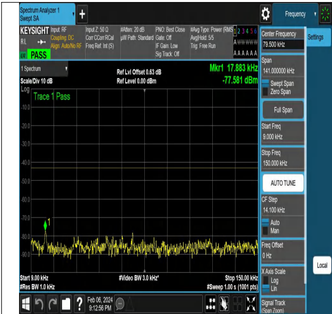
NTNV-N77-3700-3980-PC2-30-15-H-DFT-QPSK-Edge_1RB_
