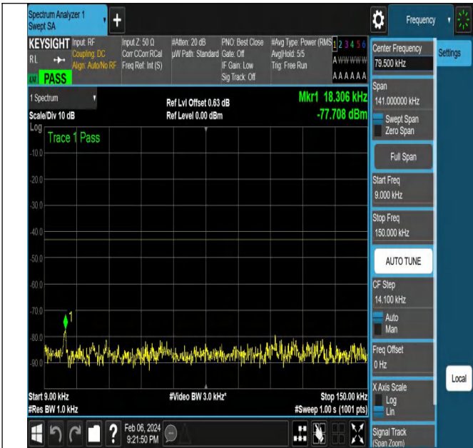
NTNV-N77-3700-3980-PC2-30-20-M-DFT-PI2BPSK-Edge_1R B_Left-Ant1-PASS
