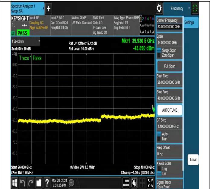
NTNV-N77-3700-3980-PC2-30-20-H-DFT-PI2BPSK-Edge_1R B_Left-Ant1-PASS
