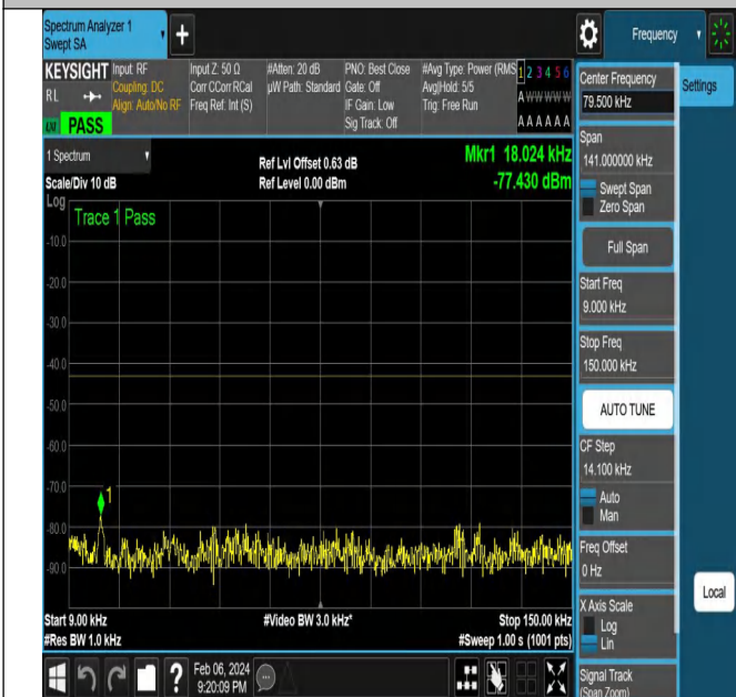
NTNV-N77-3700-3980-PC2-30-20-L-DFT-QPSK-Edge_1RB_ Right-Ant1-PASS
