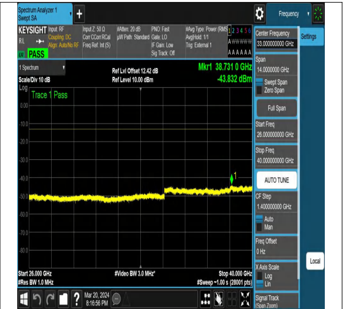
NTNV-N77-3700-3980-PC2-30-15-H-DFT-QPSK-Edge_1RB_
