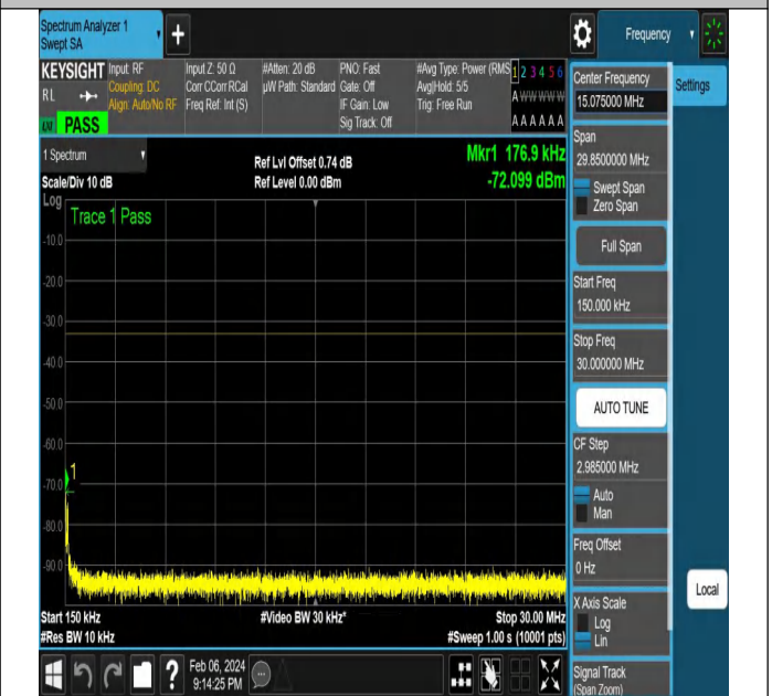
NTNV-N77-3700-3980-PC2-30-15-H-DFT-QPSK-Edge_1RB_
