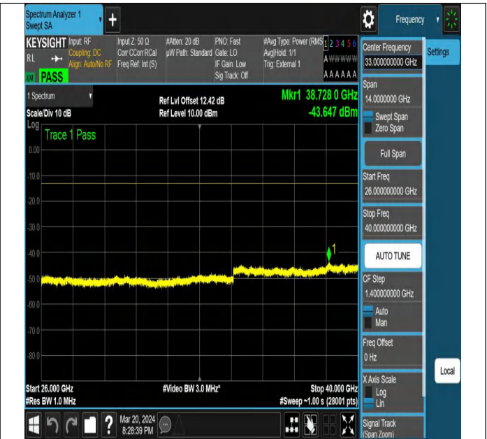
NTNV-N77-3700-3980-PC2-30-20-M-DFT-QPSK-Edge_1RB_ Left-Ant1-PASS
