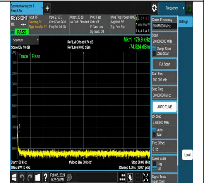
NTNV-N77-3700-3980-PC2-30-20-M-DFT-QPSK-Edge_1RB_ Right-Ant1-PASS
