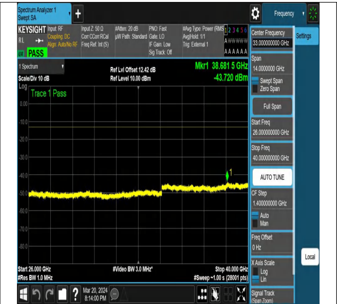
NTNV-N77-3700-3980-PC2-30-15-H-DFT-PI2BPSK-Edge_1R B_Left-Ant1-PASS
