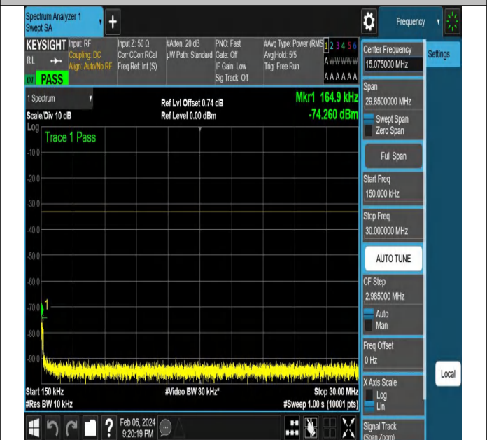
NTNV-N77-3700-3980-PC2-30-20-L-DFT-QPSK-Edge_1RB_ Right-Ant1-PASS
