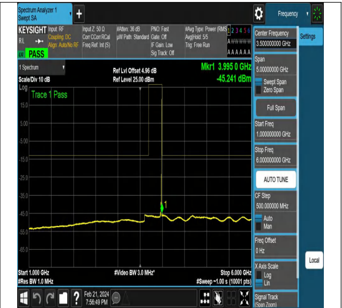
NTNV-N77-3700-3980-PC2-30-15-H-DFT-PI2BPSK-Edge_1R B_Right-Ant1-PASS
