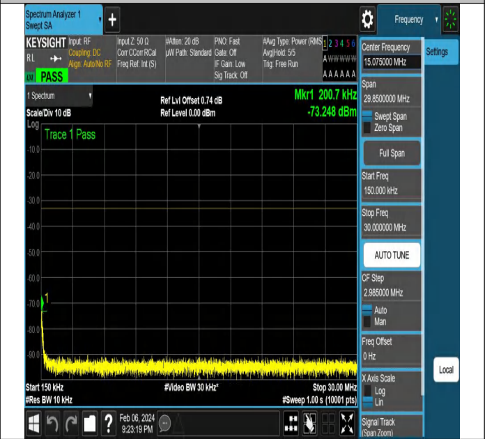
NTNV-N77-3700-3980-PC2-30-20-M-DFT-PI2BPSK-Edge_1R B_Right-Ant1-PASS
