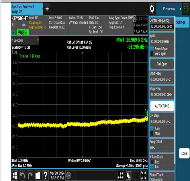
NTNV-N77-3700-3980-PC2-30-20-H-DFT-PI2BPSK-Edge_1R B_Right-Ant1-PASS
