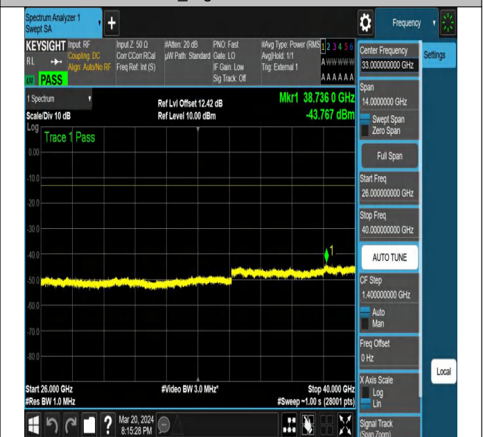
NTNV-N77-3700-3980-PC2-30-15-H-DFT-PI2BPSK-Edge_1R B_Right-Ant1-PASS
