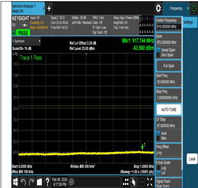
NTNV-N77-3700-3980-PC2-30-20-L-DFT-PI2BPSK-Edge_1R B_Right-Ant1-PASS
