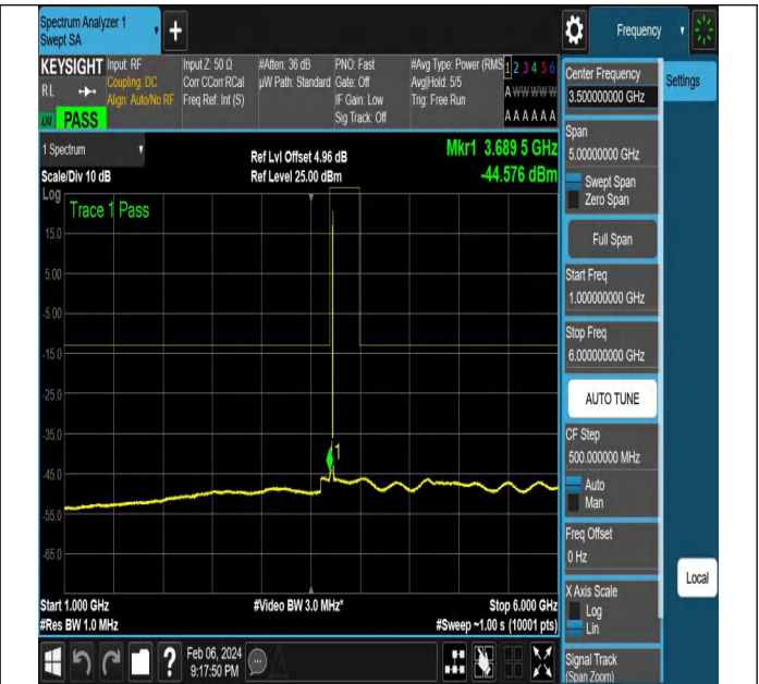
NTNV-N77-3700-3980-PC2-30-20-L-DFT-PI2BPSK-Edge_1R B_Right-Ant1-PASS
