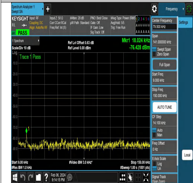
NTNV-N77-3700-3980-PC2-30-15-H-DFT-QPSK-Edge_1RB_
