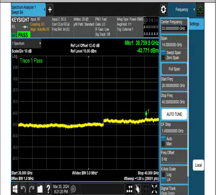
NTNV-N77-3700-3980-PC2-30-20-L-DFT-PI2BPSK-Edge_1R B_Right-Ant1-PASS
