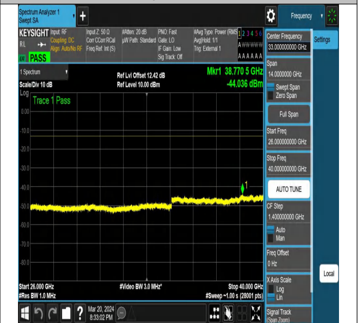
NTNV-N77-3700-3980-PC2-30-20-H-DFT-PI2BPSK-Edge_1R B_Right-Ant1-PASS
