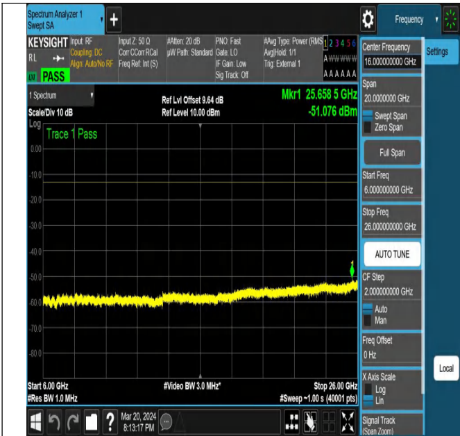
NTNV-N77-3700-3980-PC2-30-15-H-DFT-PI2BPSK-Edge_1R B_Left-Ant1-PASS
