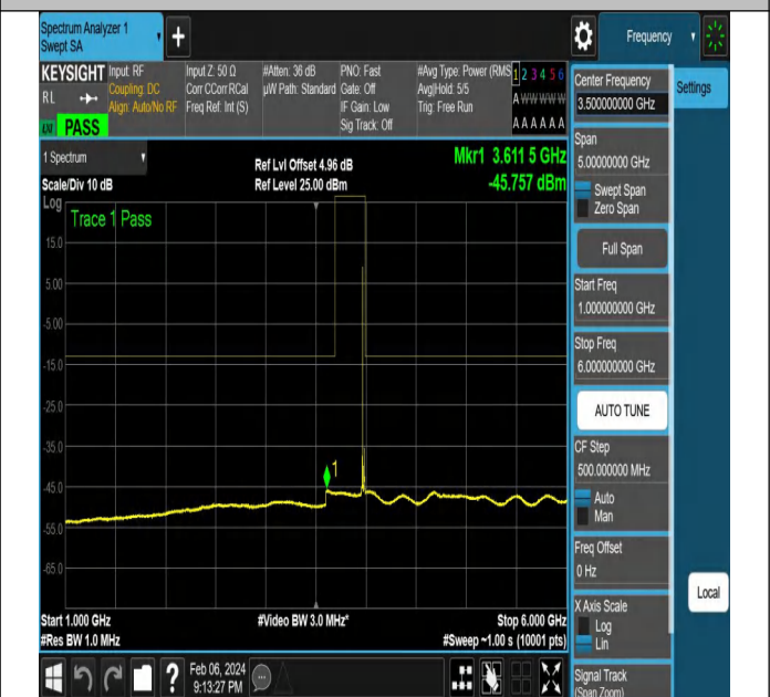
NTNV-N77-3700-3980-PC2-30-15-H-DFT-QPSK-Edge_1RB_
