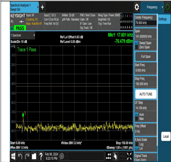
NTNV-N77-3700-3980-PC2-30-20-M-DFT-PI2BPSK-Edge_1R B_Right-Ant1-PASS
