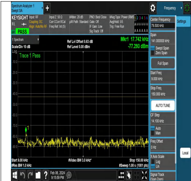
NTNV-N77-3700-3980-PC2-30-20-L-DFT-PI2BPSK-Edge_1R
