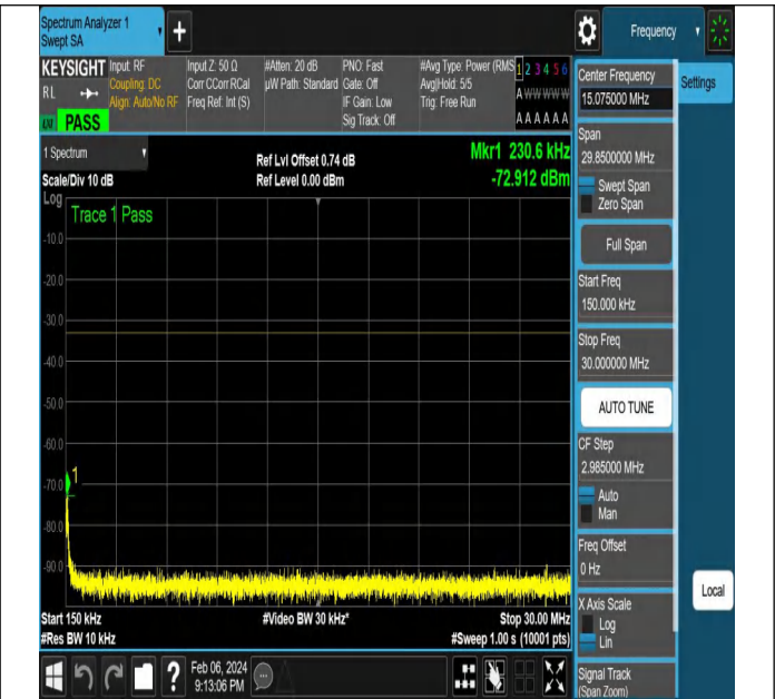
NTNV-N77-3700-3980-PC2-30-15-H-DFT-QPSK-Edge_1RB_
