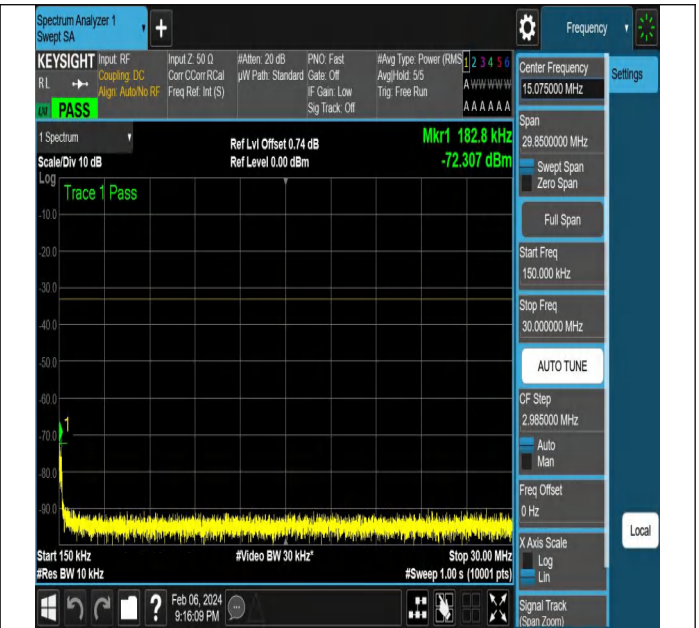
NTNV-N77-3700-3980-PC2-30-20-L-DFT-PI2BPSK-Edge_1R
