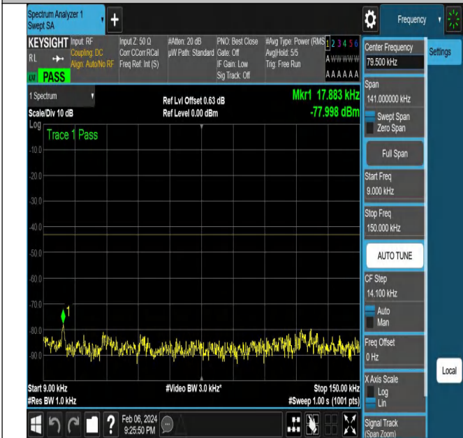
NTNV-N77-3700-3980-PC2-30-20-M-DFT-QPSK-Edge_1RB_ Right-Ant1-PASS
