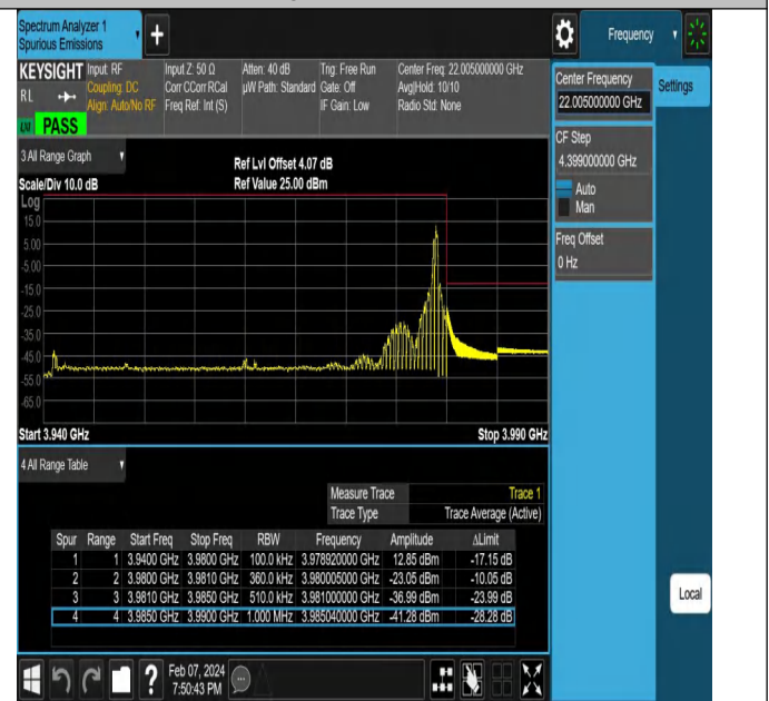
NTNV-N77-3700-3980-PC2-30-40-H-DFT-QPSK-Edge_1RB_Rig ht-Ant1-PASS
