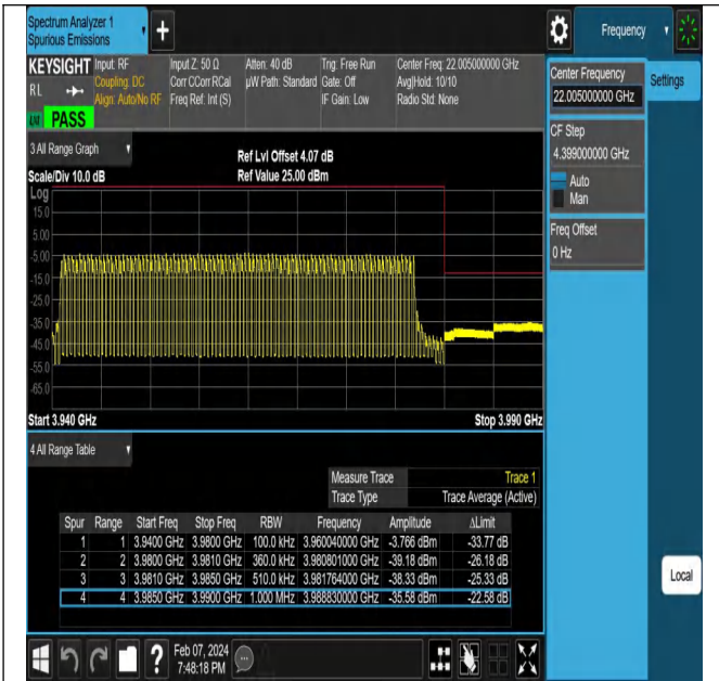
NTNV-N77-3700-3980-PC2-30-40-H-DFT-PI2BPSK-Outer_ Full-Ant1-PASS
