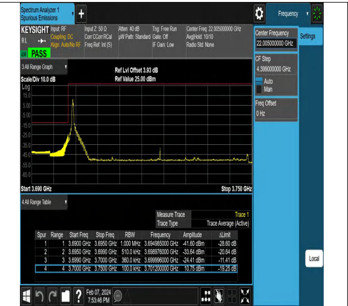
NTNV-N77-3700-3980-PC2-30-50-L-DFT-PI2BPSK-Edge_1RB_Left-Ant1-PASS
