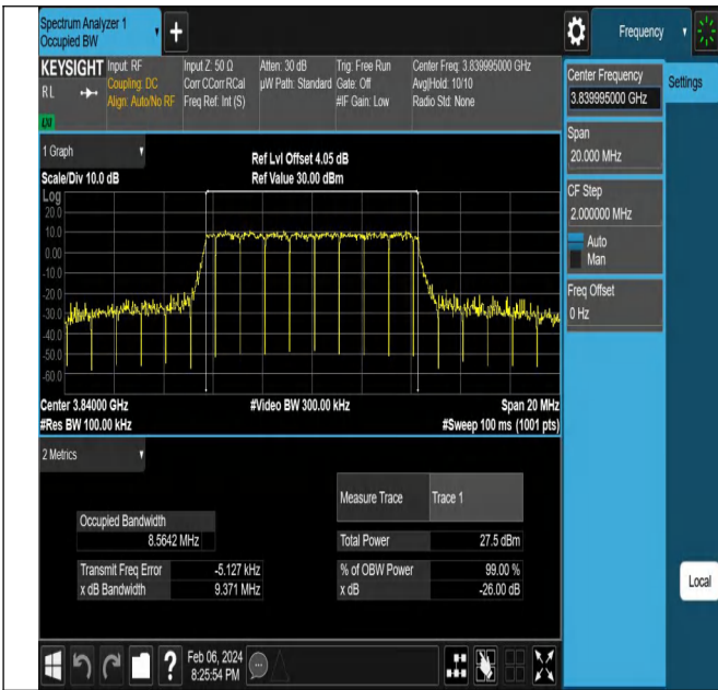
NTNV-N77-3700-3980-PC2-30-10-M-CP-QPSK-Outer_Full-A nt1-PASS
