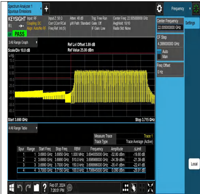
NTNV-N77-3700-3980-PC2-30-15-L-DFT-PI2BPSK-Outer_Full-Ant1-PASS
