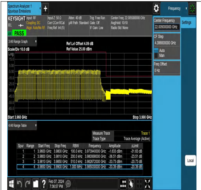
NTNV-N77-3700-3980-PC2-30-20-H-DFT-PI2BPSK-Outer_ Full-Ant1-PASS
