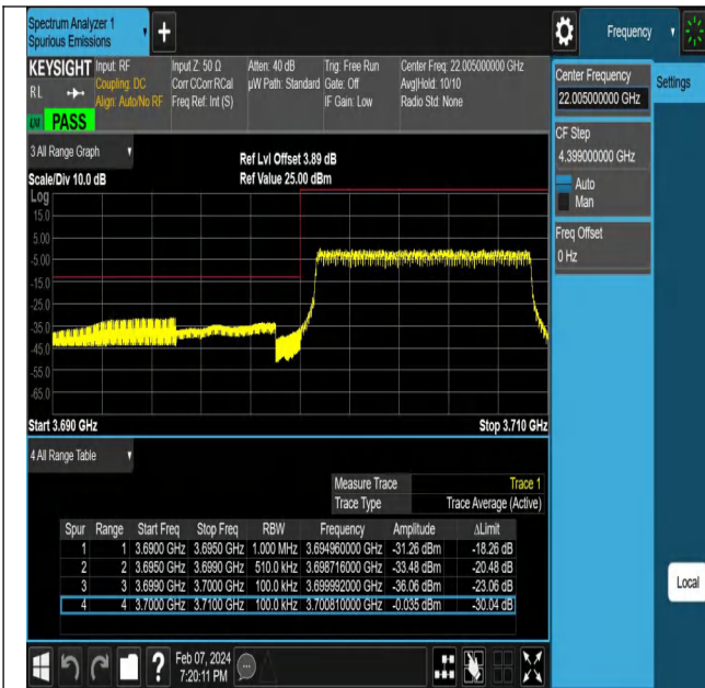
NTNV-N77-3700-3980-PC2-30-10-L-DFT-PI2BPSK-Outter_Full-Ant1-PASS
