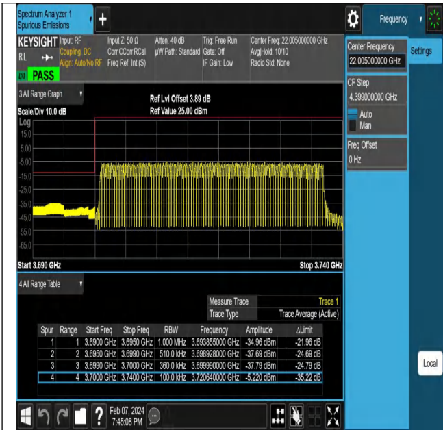
NTNV-N77-3700-3980-PC2-30-40-L-DFT-PI2BPSK-Outer_Full-Ant1-PASS
