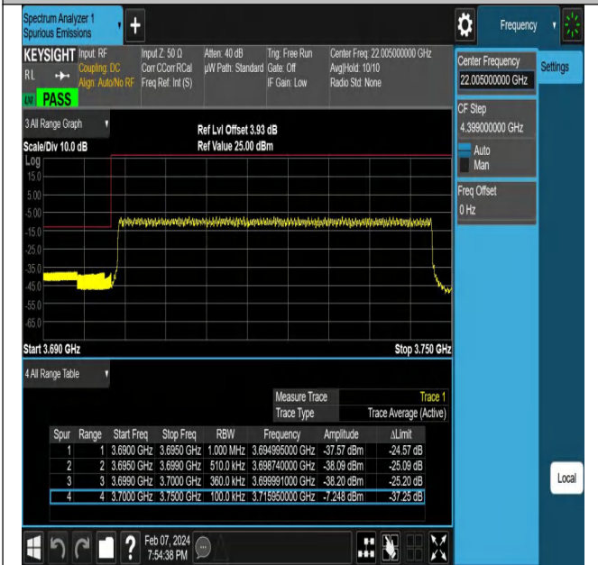
NTNV-N77-3700-3980-PC2-30-50-L-DFT-QPSK-Outer_Full-Ant1-PASS
