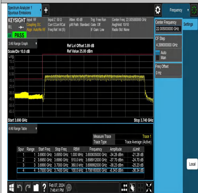
NTNV-N77-3700-3980-PC2-30-40-L-DFT-QPSK-Outer_Full-Ant1-PASS
