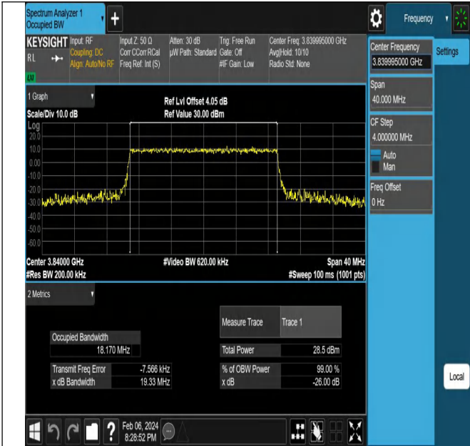
NTNV-N77-3700-3980-PC2-30-20-M-CP-QPSK-Outer_Full-A
