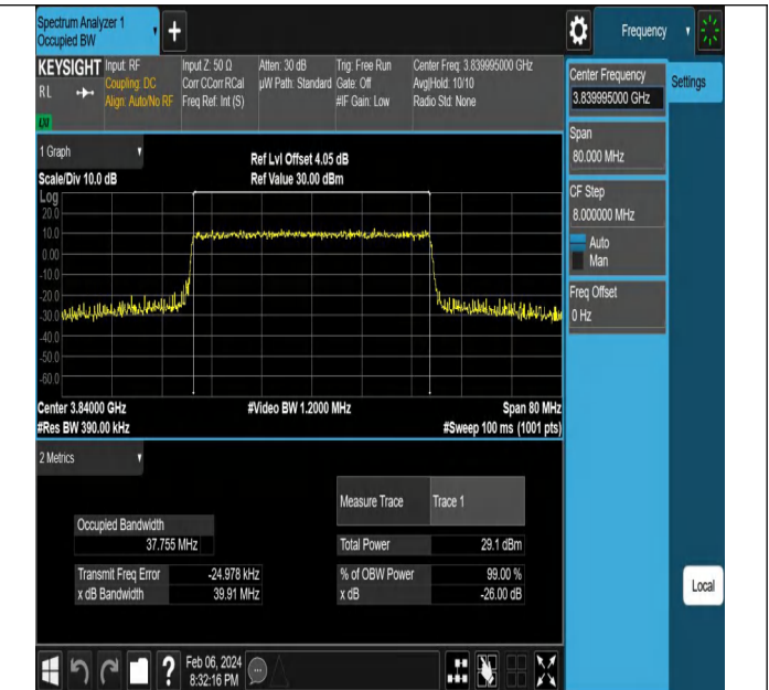
NTNV-N77-3700-3980-PC2-30-40-M-CP-16QAM-Outer_Full-A nt1-PASS
