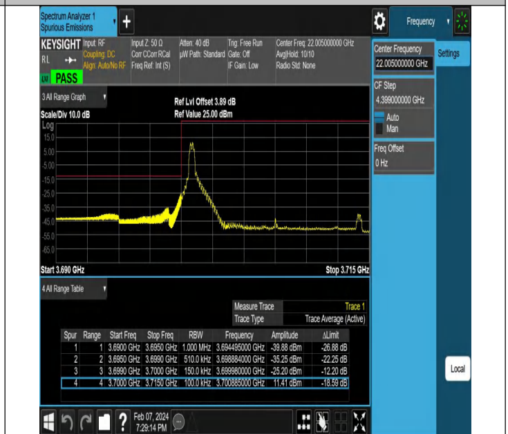
NTNV-N77-3700-3980-PC2-30-15-L-DFT-QPSK-Edge_1RB_Left-Ant1-PASS
