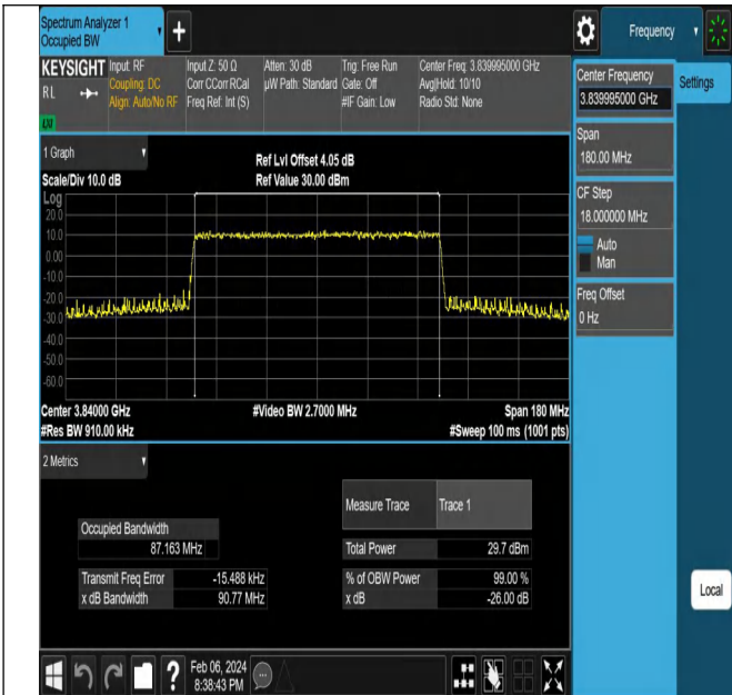
NTNV-N77-3700-3980-PC2-30-90-M-CP-QPSK-Outer_Full-A nt1-PASS
