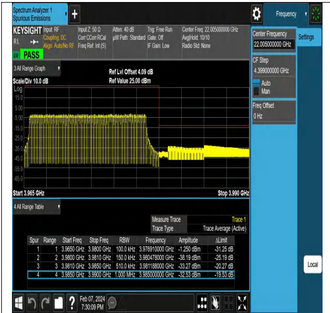
NTNV-N77-3700-3980-PC2-30-15-H-DFT-PI2BPSK-Outer_ Full-Ant1-PASS
