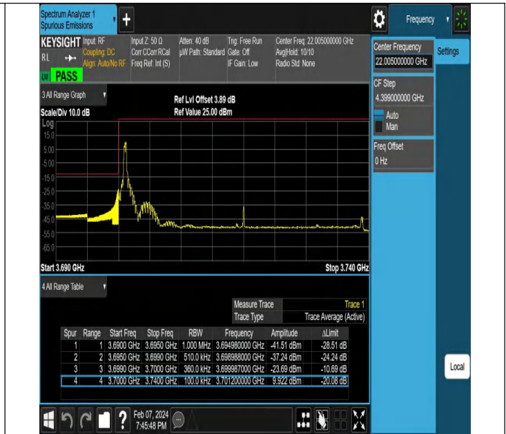
NTNV-N77-3700-3980-PC2-30-40-L-DFT-PI2BPSK-Edge_1RB_Left-Ant1-PASS
