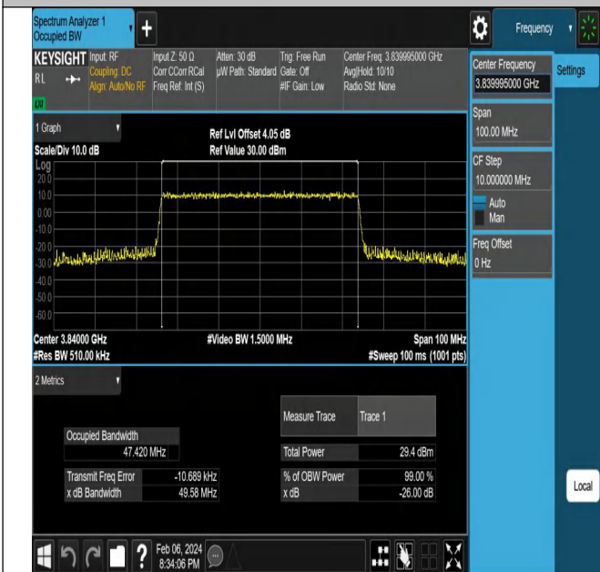
NTNV-N77-3700-3980-PC2-30-50-M-CP-64QAM-Outer_Full-A
