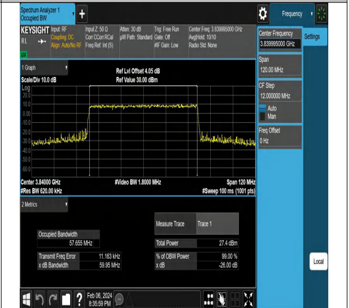
NTNV-N77-3700-3980-PC2-30-60-M-CP-256QAM-Outer_Full- Ant1-PASS
