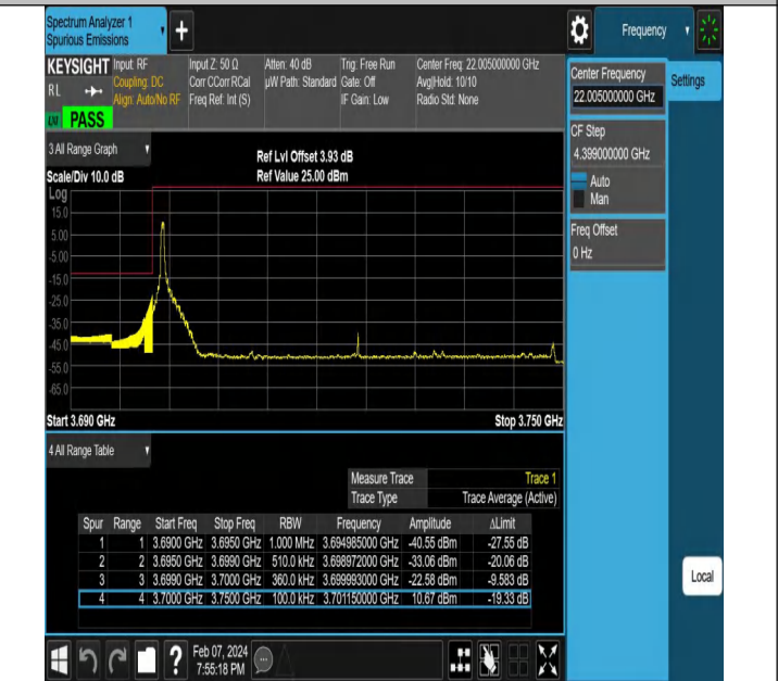
NTNV-N77-3700-3980-PC2-30-50-L-DFT-QPSK-Edge_1RB_Left-Ant1-PASS
