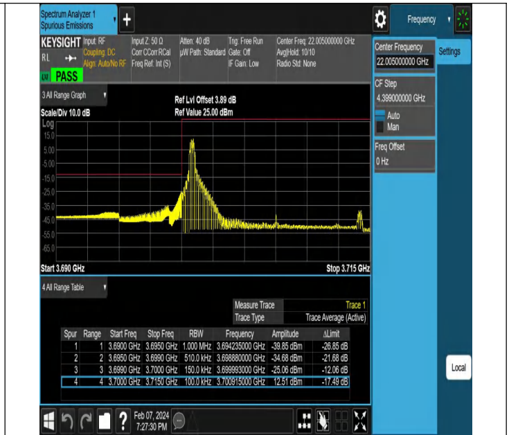
NTNV-N77-3700-3980-PC2-30-15-L-DFT-PI2BPSK-Edge_1RB_Left-Ant1-PASS
