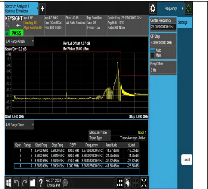
NTNV-N77-3700-3980-PC2-30-40-H-DFT-PI2BPSK-Edge_1RB_ Right-Ant1-PASS
