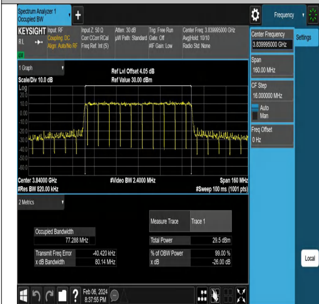
NTNV-N77-3700-3980-PC2-30-80-M-CP-64QAM-Outer_Full-Ant1-PASS
