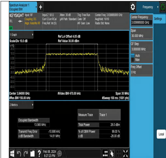
NTNV-N77-3700-3980-PC2-30-15-M-CP-QPSK-Outer_Full-A
