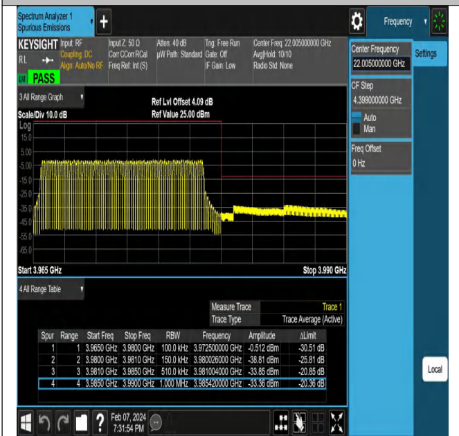
NTNV-N77-3700-3980-PC2-30-15-H-DFT-QPSK-Outer_Full -Ant1-PASS
