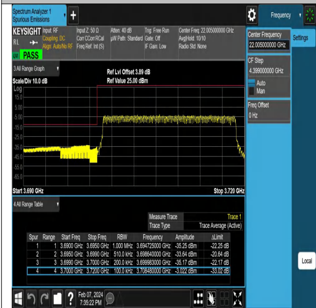
NTNV-N77-3700-3980-PC2-30-20-L-DFT-QPSK-Outer_Full-Ant1-PASS
