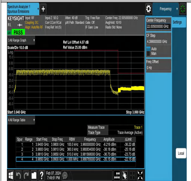
NTNV-N77-3700-3980-PC2-30-40-H-DFT-QPSK-Outer_Full -Ant1-PASS
