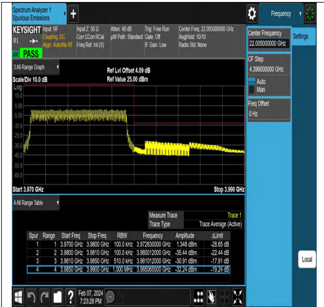
NTNV-N77-3700-3980-PC2-30-10-H-DFT-PI2BPSK-Outer_ Full-Ant1-PASS
