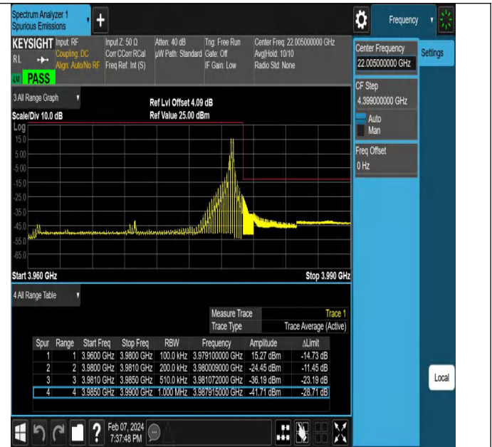
NTNV-N77-3700-3980-PC2-30-20-H-DFT-PI2BPSK-Edge_1RB_ Right-Ant1-PASS
