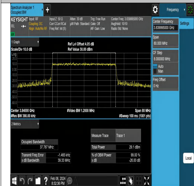
NTNV-N77-3700-3980-PC2-30-40-M-CP-64QAM-Outer_Full-A Ant1-PASS
