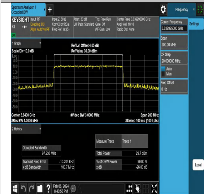
NTNV-N77-3700-3980-PC2-30-100-M-CP-64QAM-Outer_Full -Ant1-PASS
