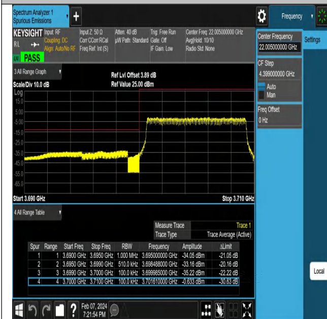
NTNV-N77-3700-3980-PC2-30-10-L-DFT-QPSK-Outter_Full-Ant1-PASS
