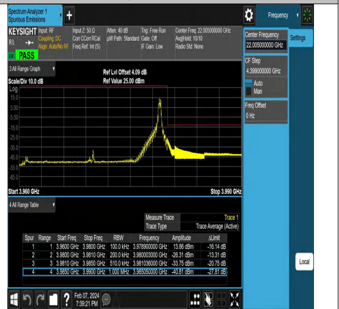
NTNV-N77-3700-3980-PC2-30-20-H-DFT-QPSK-Edge_1RB_Rig ht-Ant1-PASS
