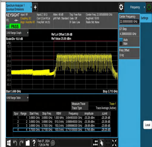
NTNV-N77-3700-3980-PC2-30-15-L-DFT-QPSK-Outer_Full-Ant1-PASS
