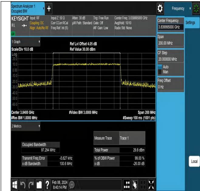
NTNV-N77-3700-3980-PC2-30-100-M-CP-QPSK-Outer_Full -Ant1-PASS
