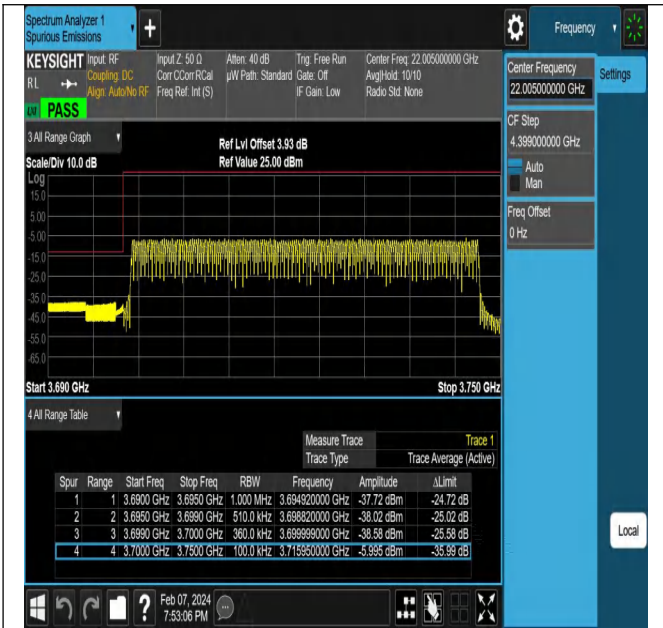
NTNV-N77-3700-3980-PC2-30-50-L-DFT-PI2BPSK-Outer_Full-Ant1-PASS
