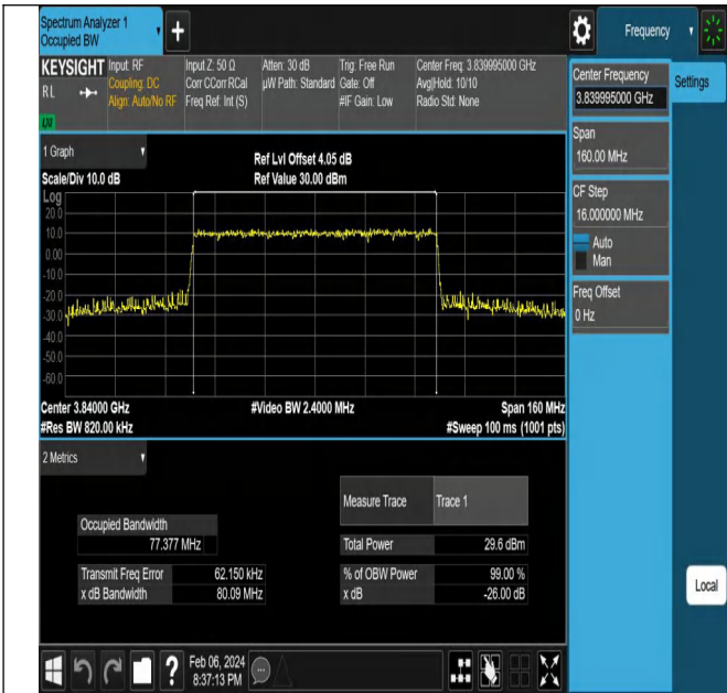
NTNV-N77-3700-3980-PC2-30-80-M-CP-QPSK-Outer_Full-A
