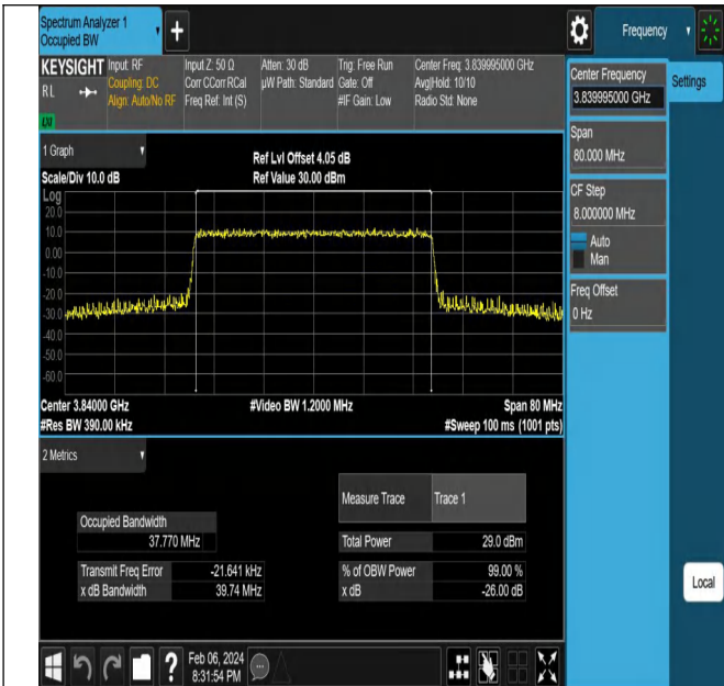
NTNV-N77-3700-3980-PC2-30-40-M-CP-QPSK-Outer_Full-A nt1-PASS
