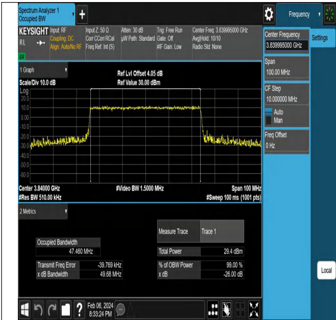
NTNV-N77-3700-3980-PC2-30-50-M-CP-QPSK-Outer_Full-A
