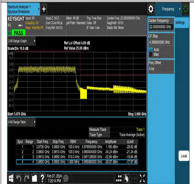
NTNV-N77-3700-3980-PC2-30-10-H-DFT-QPSK-Outer_Full -Ant1-PASS
