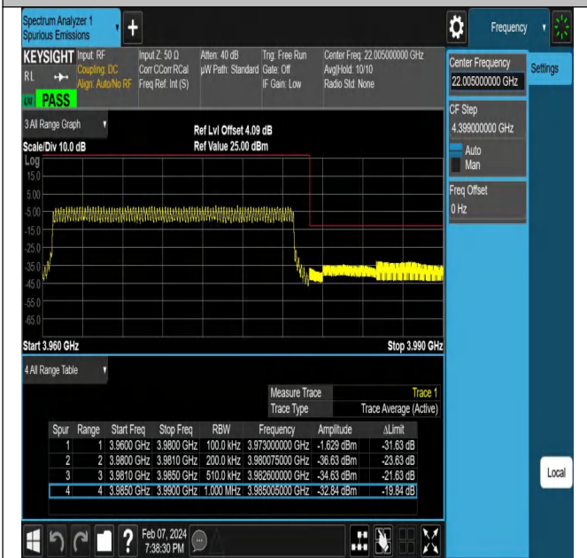
NTNV-N77-3700-3980-PC2-30-20-H-DFT-QPSK-Outer_Full -Ant1-PASS
