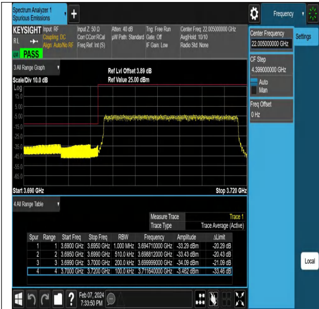
NTNV-N77-3700-3980-PC2-30-20-L-DFT-PI2BPSK-Outer_Full-Ant1-PASS
