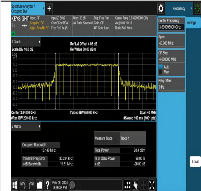
NTNV-N77-3700-3980-PC2-30-20-M-CP-64QAM-Outer_Full-A
