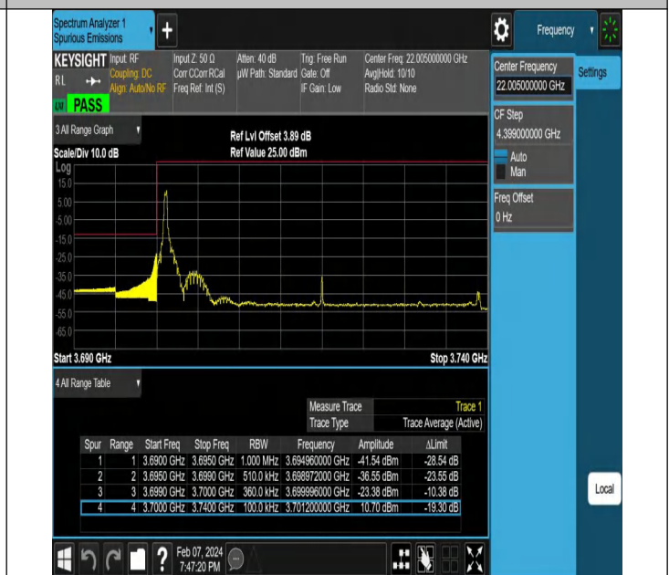
NTNV-N77-3700-3980-PC2-30-40-L-DFT-QPSK-Edge_1RB_Left-Ant1-PASS
