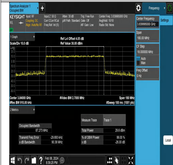
NTNV-N77-3700-3980-PC2-30-90-M-CP-64QAM-Outer_Full-A Ant1-PASS
