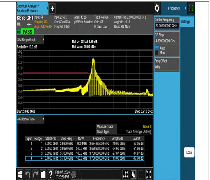
NTNV-N77-3700-3980-PC2-30-10-L-DFT-PI2BPSK-Edge_1RB_Left-Ant1-PASS
