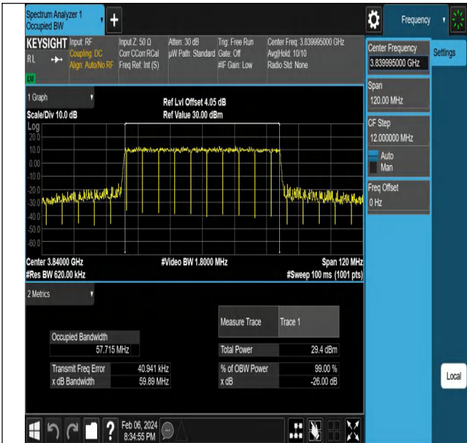
NTNV-N77-3700-3980-PC2-30-60-M-CP-QPSK-Outer_Full-A nt1-PASS
