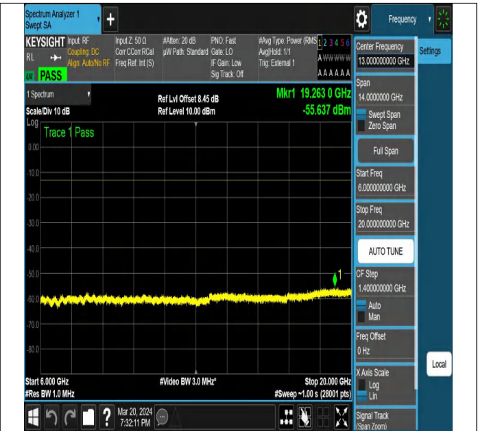
NTNV-N77-3450-3550-PC2-30-90-M-DFT-QPSK-Edge_1RB_
