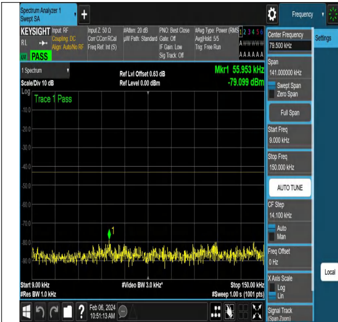
NTNV-N77-3450-3550-PC2-30-90-L-DFT-QPSK-Edge_1RB_
