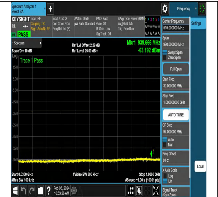
NTNV-N77-3450-3550-PC2-30-90-M-DFT-PI2BPSK-Edge_1R B_Left-Ant1-PASS
