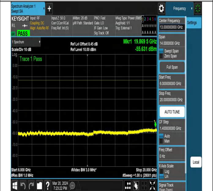
NTNV-N77-3450-3550-PC2-30-90-L-DFT-PI2BPSK-Edge_1R
