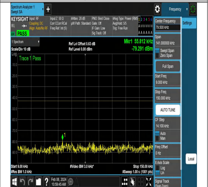
NTNV-N77-3450-3550-PC2-30-90-H-DFT-PI2BPSK-Edge_1RB_
