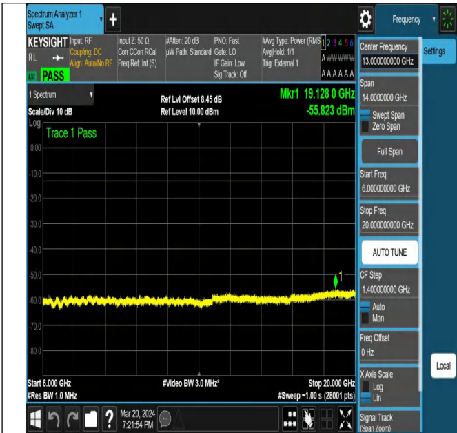
NTNV-N77-3450-3550-PC2-30-90-L-DFT-PI2BPSK-Edge_1R B_Left-Ant1-PASS
