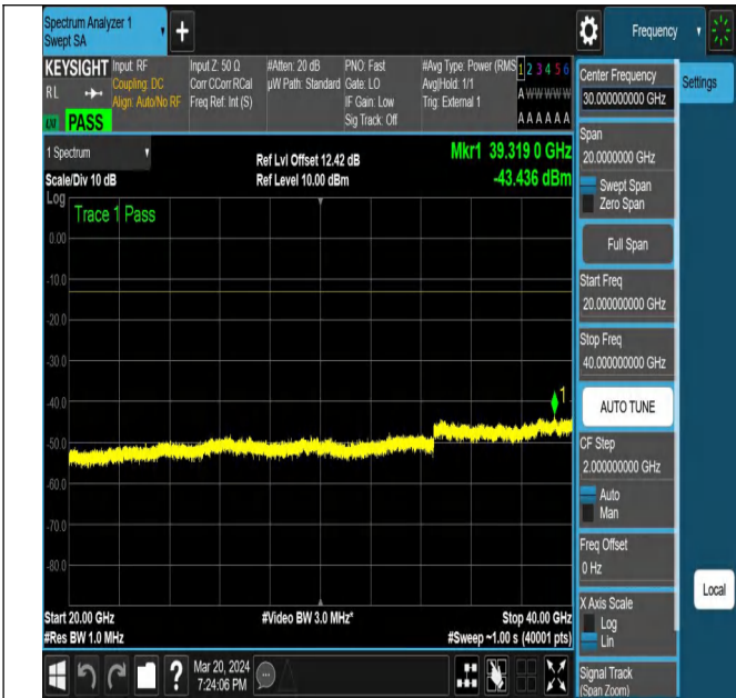
NTNV-N77-3450-3550-PC2-30-90-L-DFT-PI2BPSK-Edge_1R_B_Right-Ant1-PASS
