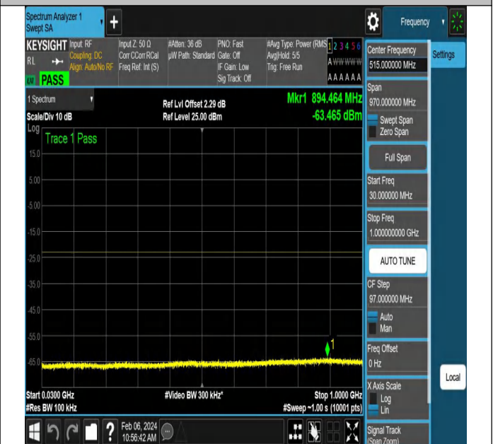
NTNV-N77-3450-3550-PC2-30-90-M-DFT-QPSK-Edge_1RB_Left-Ant1-PASS
