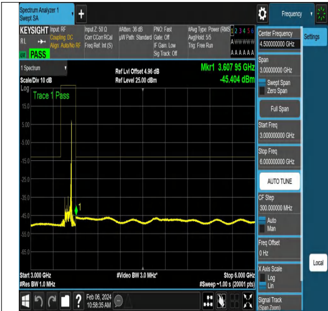
NTNV-N77-3450-3550-PC2-30-90-M-DFT-QPSK-Edge_1RB_
