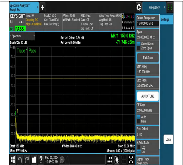
NTNV-N77-3450-3550-PC2-30-90-M-DFT-QPSK-Edge_1RB_ Right-Ant1-PASS
