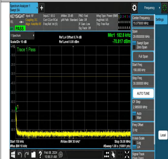
NTNV-N77-3450-3550-PC2-30-90-M-DFT-QPSK-Edge_1RB_Left-Ant1-PASS
