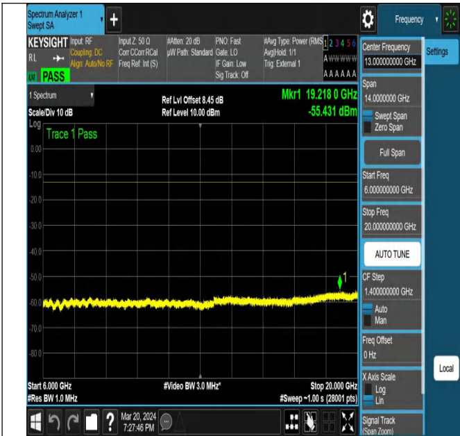
NTNV-N77-3450-3550-PC2-30-90-M-DFT-PI2BPSK-Edge_1R B_Left-Ant1-PASS
