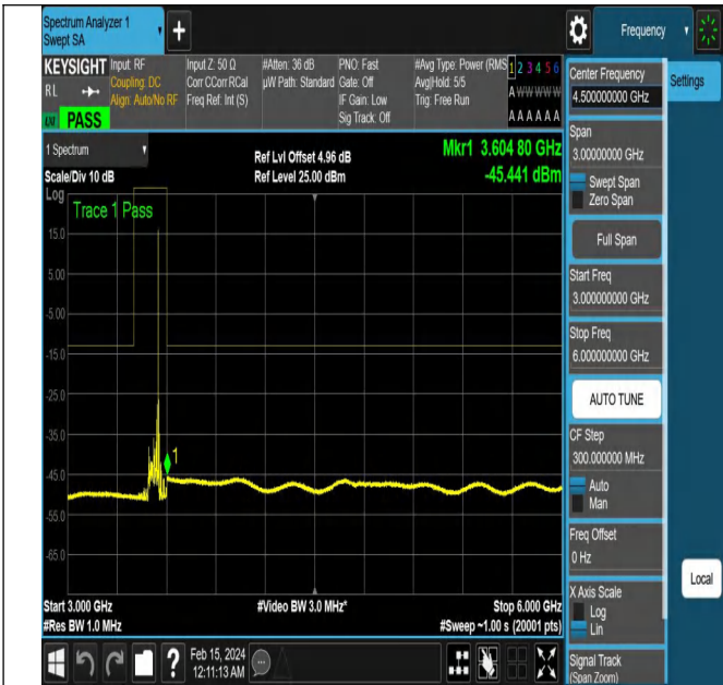
NTNV-N77-3450-3550-PC2-30-60-H-DFT-QPSK-Edge_1RB_
