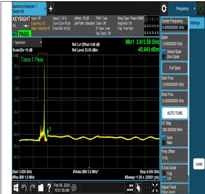
NTNV-N77-3450-3550-PC2-30-90-L-DFT-QPSK-Edge_1RB_ Right-Ant1-PASS
