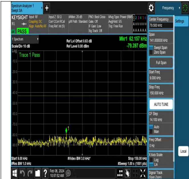
NTNV-N77-3450-3550-PC2-30-90-M-DFT-QPSK-Edge_1RB_ Right-Ant1-PASS
