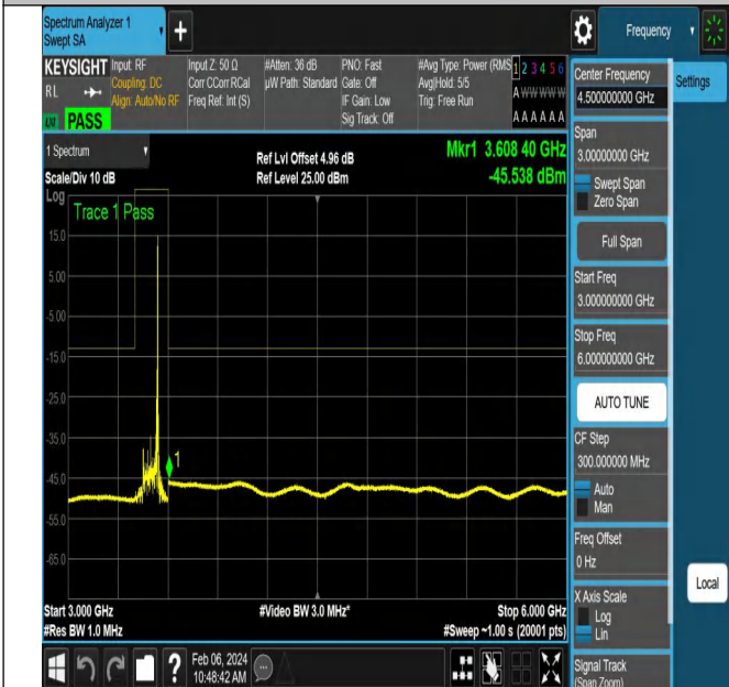
NTNV-N77-3450-3550-PC2-30-90-L-DFT-PI2BPSK-Edge_1R
