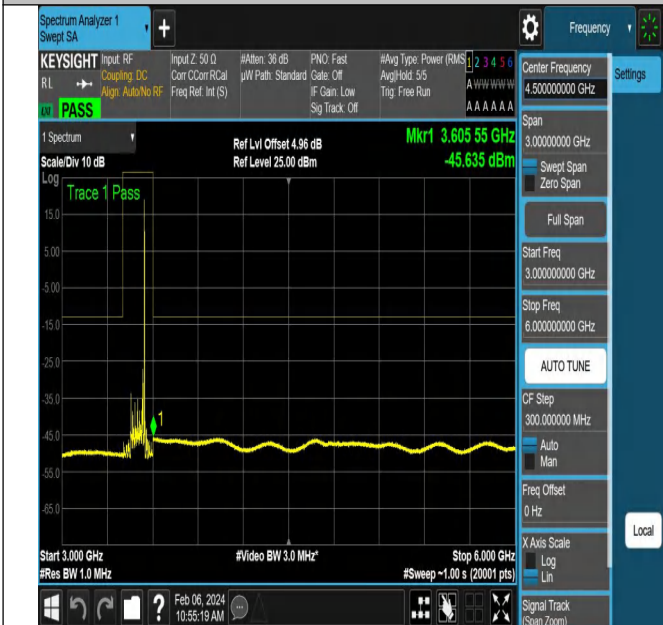
NTNV-N77-3450-3550-PC2-30-90-M-DFT-PI2BPSK-Edge_1R B_Right-Ant1-PASS
