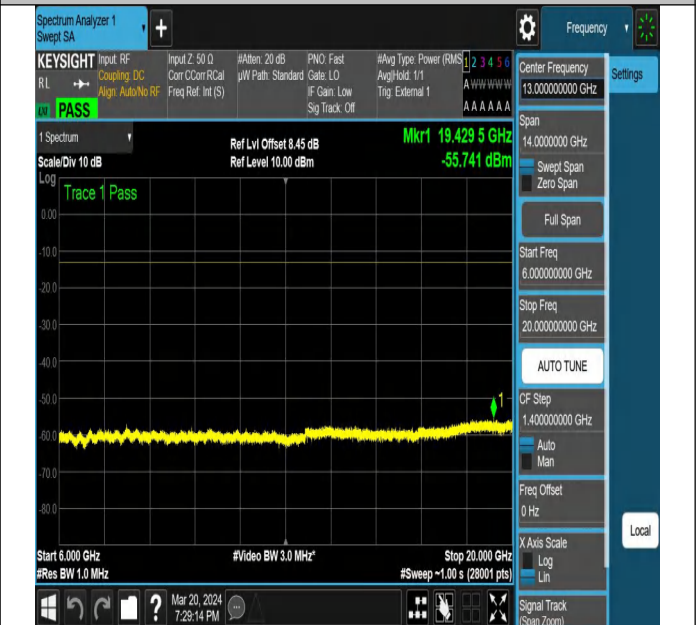
NTNV-N77-3450-3550-PC2-30-90-M-DFT-PI2BPSK-Edge_1R B_Right-Ant1-PASS
