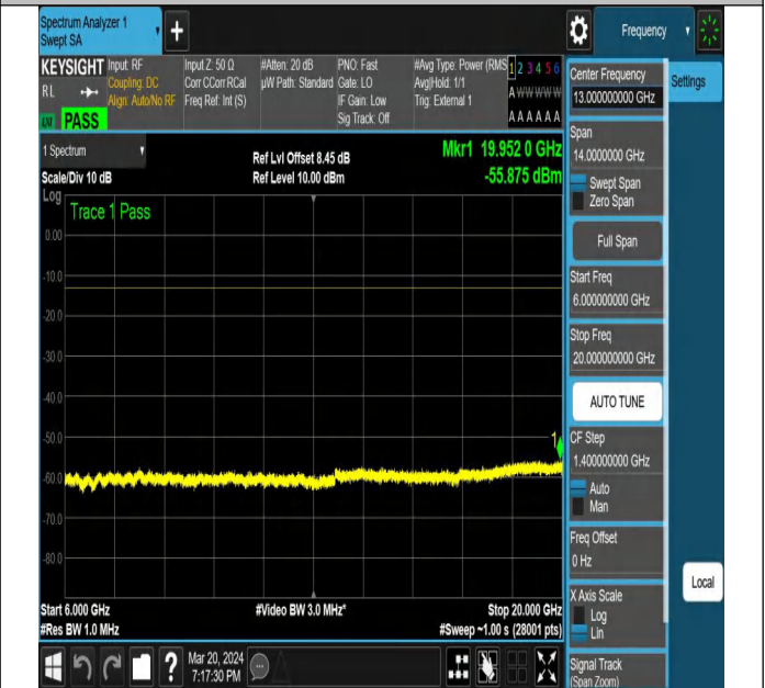
NTNV-N77-3450-3550-PC2-30-60-H-DFT-PI2BPSK-Edge_1R B_Right-Ant1-PASS
