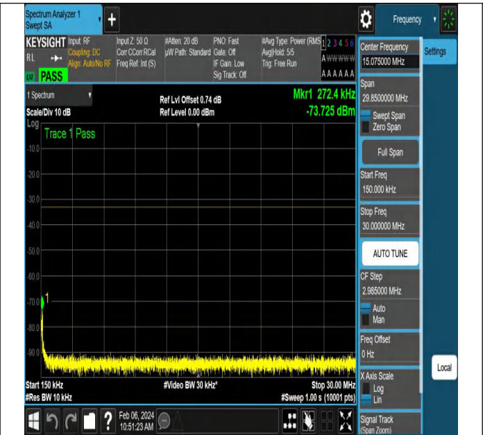
NTNV-N77-3450-3550-PC2-30-90-L-DFT-QPSK-Edge_1RB_
