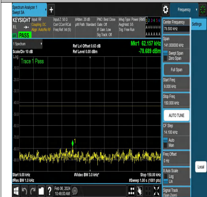
NTNV-N77-3450-3550-PC2-30-90-L-DFT-PI2BPSK-Edge_1R B_Right-Ant1-PASS
