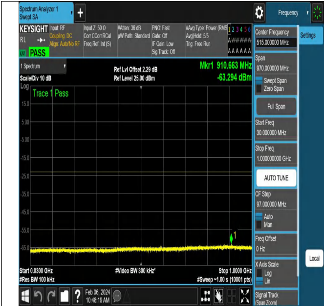
NTNV-N77-3450-3550-PC2-30-90-L-DFT-PI2BPSK-Edge_1R
