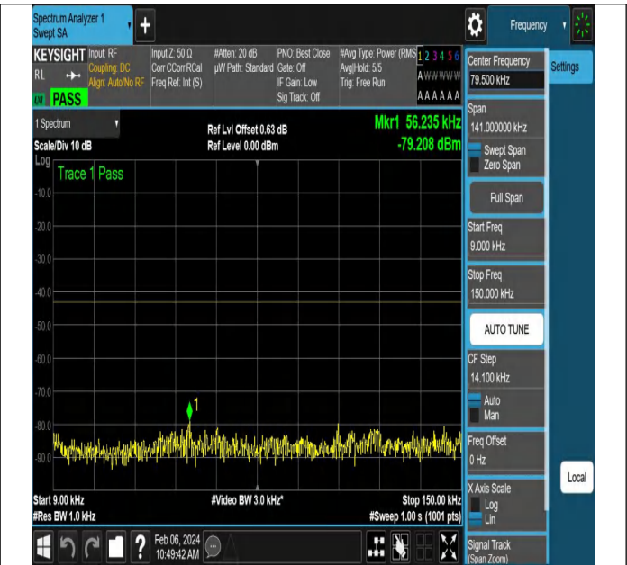
NTNV-N77-3450-3550-PC2-30-90-L-DFT-QPSK-Edge_1RB_L_eft-Ant1-PASS
