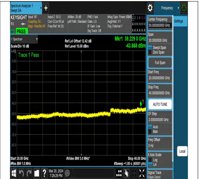
NTNV-N77-3450-3550-PC2-30-90-M-DFT-PI2BPSK-Edge_1R B_Left-Ant1-PASS
