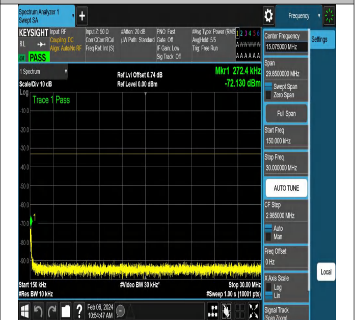
NTNV-N77-3450-3550-PC2-30-90-M-DFT-PI2BPSK-Edge_1R B_Right-Ant1-PASS
