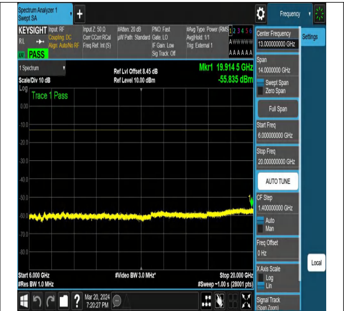
NTNV-N77-3450-3550-PC2-30-60-H-DFT-QPSK-Edge_1RB_
