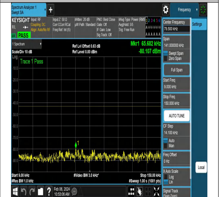
NTNV-N77-3450-3550-PC2-30-90-M-DFT-PI2BPSK-Edge_1RB_ B_Left-Ant1-PASS
