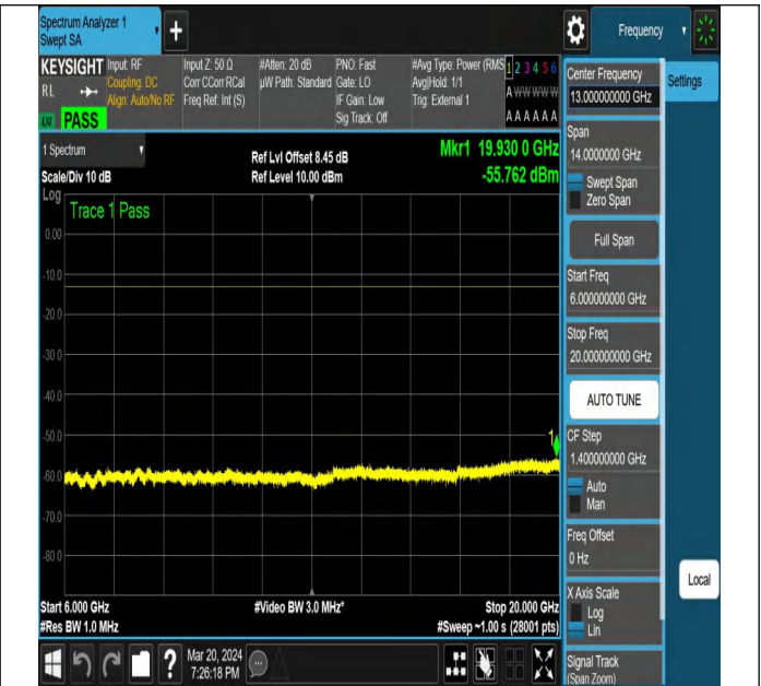
NTNV-N77-3450-3550-PC2-30-90-L-DFT-QPSK-Edge_1RB_ Right-Ant1-PASS
