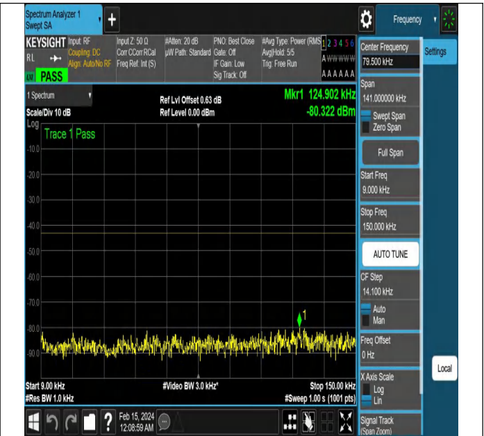
NTNV-N77-3450-3550-PC2-30-60-H-DFT-QPSK-Edge_1RB_Left-Ant1-PASS
