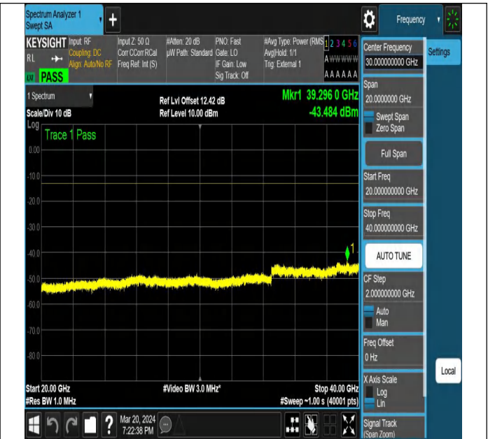
NTNV-N77-3450-3550-PC2-30-90-L-DFT-PI2BPSK-Edge_1R B_Left-Ant1-PASS
