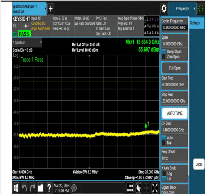
NTNV-N77-3450-3550-PC2-30-60-M-DFT-QPSK-Edge_1RB_ Left-Ant1-PASS
