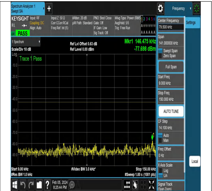
NTNV-N77-3450-3550-PC2-30-80-H-DFT-QPSK-Edge_1RB_Left-Ant1-PASS
