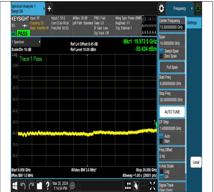
NTNV-N77-3450-3550-PC2-30-60-M-DFT-QPSK-Edge_1RB_ Right-Ant1-PASS
