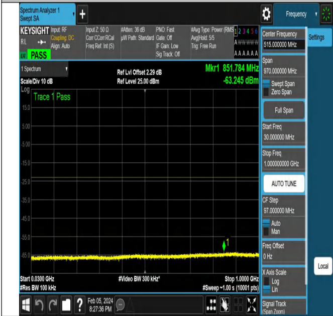
NTNV-N77-3450-3550-PC2-30-80-H-DFT-QPSK-Edge_1RB_ Right-Ant1-PASS
