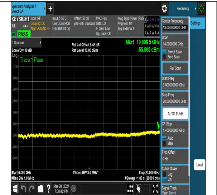
NTVN-N77-3450-3550-PC2-30-60-L-DFT-QPSK-Edge_1RB_ Right-Ant1-PASS
