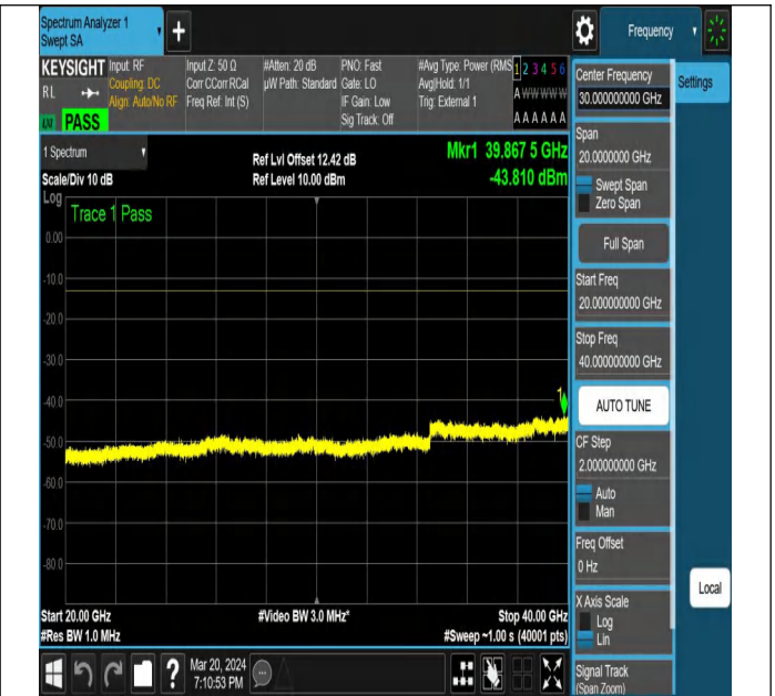
NTNV-N77-3450-3550-PC2-30-60-M-DFT-PI2BPSK-Edge_1R B_Left-Ant1-PASS
