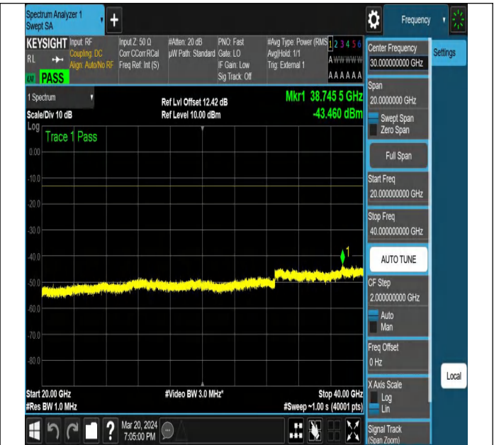
NTNV-N77-3450-3550-PC2-30-60-L-DFT-PI2BPSK-Edge_1R B_Left-Ant1-PASS
