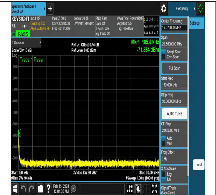
NTNV-N77-3450-3550-PC2-30-60-M-DFT-QPSK-Edge_1RB_ Right-Ant1-PASS
