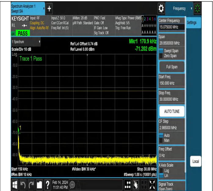
NTNV-N77-3450-3550-PC2-30-60-L-DFT-QPSK-Edge_1RB_
