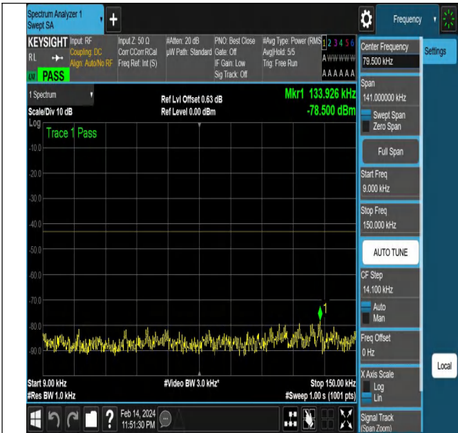
NTNV-N77-3450-3550-PC2-30-60-L-DFT-QPSK-Edge_1RB_
