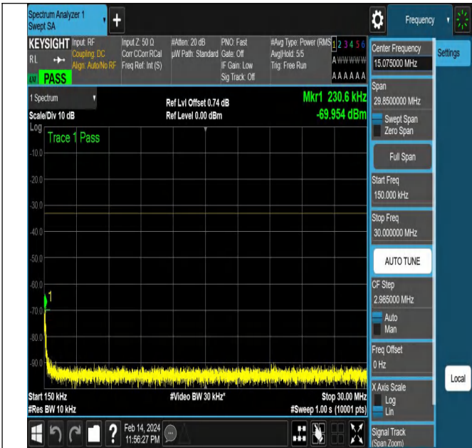
NTNV-N77-3450-3550-PC2-30-60-M-DFT-PI2BPSK-Edge_1R B_Left-Ant1-PASS
