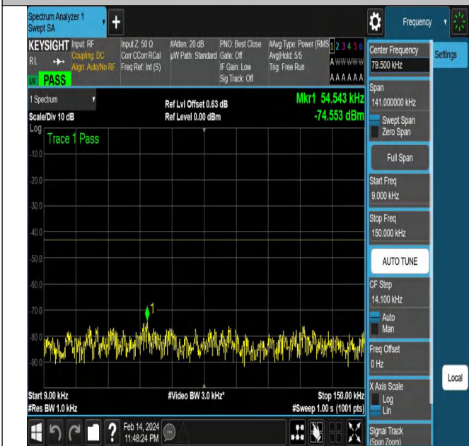
NTNV-N77-3450-3550-PC2-30-60-L-DFT-PI2BPSK-Edge_1R B_Right-Ant1-PASS
