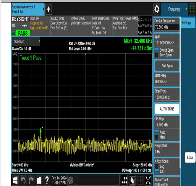
NTNV-N77-3450-3550-PC2-30-60-M-DFT-PI2BPSK-Edge_1R B_Right-Ant1-PASS
