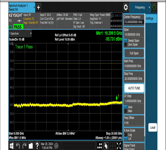
NTNV-N77-3450-3550-PC2-30-60-L-DFT-PI2BPSK-Edge_1R B_Right-Ant1-PASS
