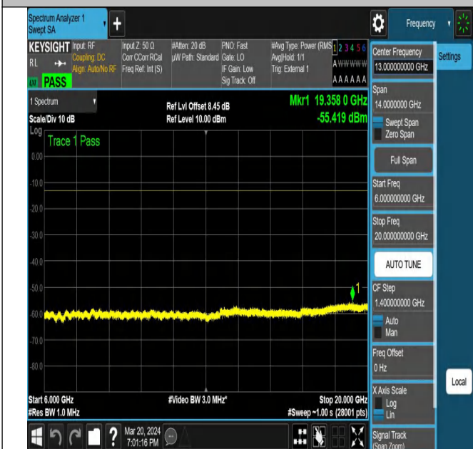
NTNV-N77-3450-3550-PC2-30-80-H-DFT-QPSK-Edge_1RB_
