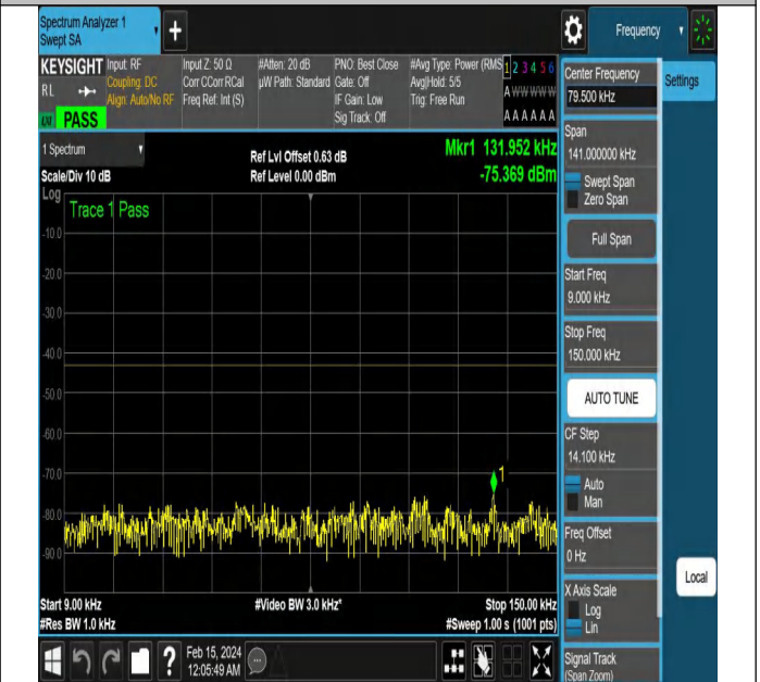
NTNV-N77-3450-3550-PC2-30-60-H-DFT-PI2BPSK-Edge_1RB_ B_Left-Ant1-PASS
