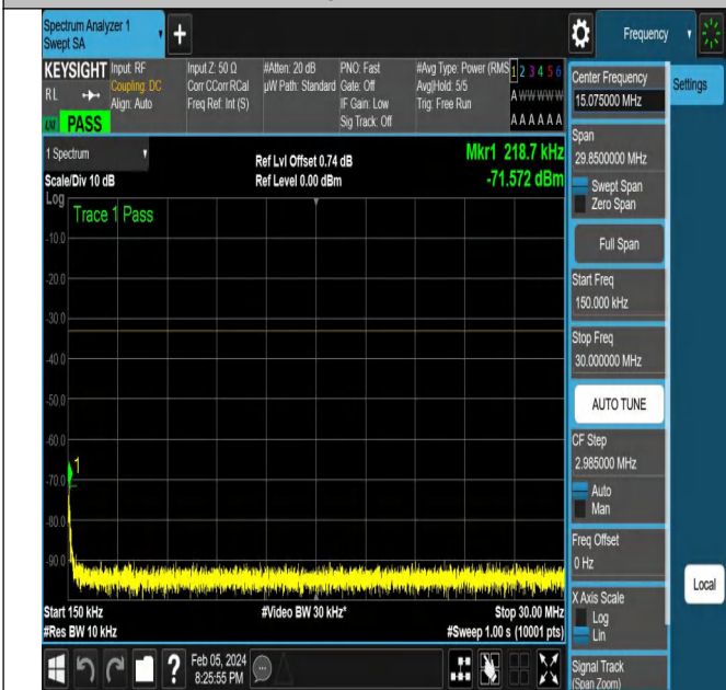
NTNV-N77-3450-3550-PC2-30-80-H-DFT-QPSK-Edge_1RB_Left-Ant1-PASS
