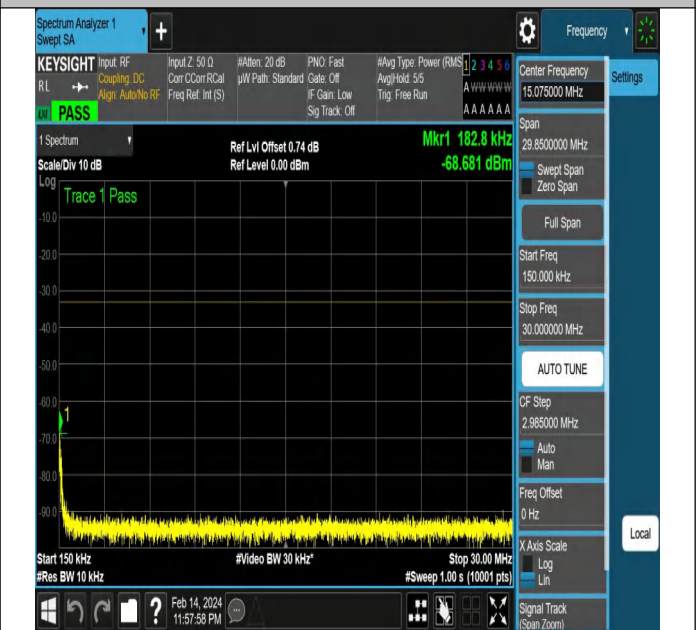
NTNV-N77-3450-3550-PC2-30-60-M-DFT-PI2BPSK-Edge_1R B_Right-Ant1-PASS
