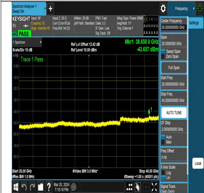
NTNV-N77-3450-3550-PC2-30-60-M-DFT-QPSK-Edge_1RB_ Right-Ant1-PASS
