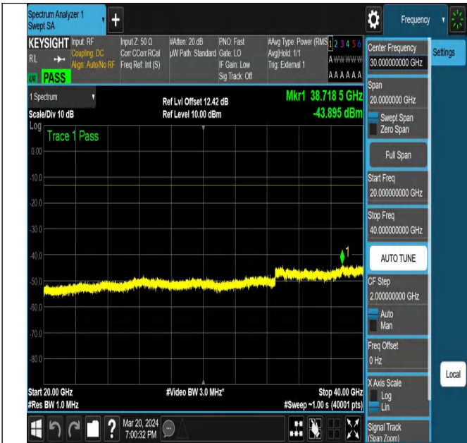
NTNV-N77-3450-3550-PC2-30-80-H-DFT-PI2BPSK-Edge_1R_B_Right-Ant1-PASS
