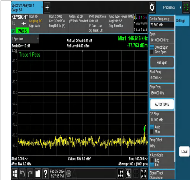
NTNV-N77-3450-3550-PC2-30-80-H-DFT-QPSK-Edge_1RB_ Right-Ant1-PASS
