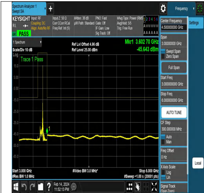
NTVN-N77-3450-3550-PC2-30-60-L-DFT-QPSK-Edge_1RB_ Right-Ant1-PASS
