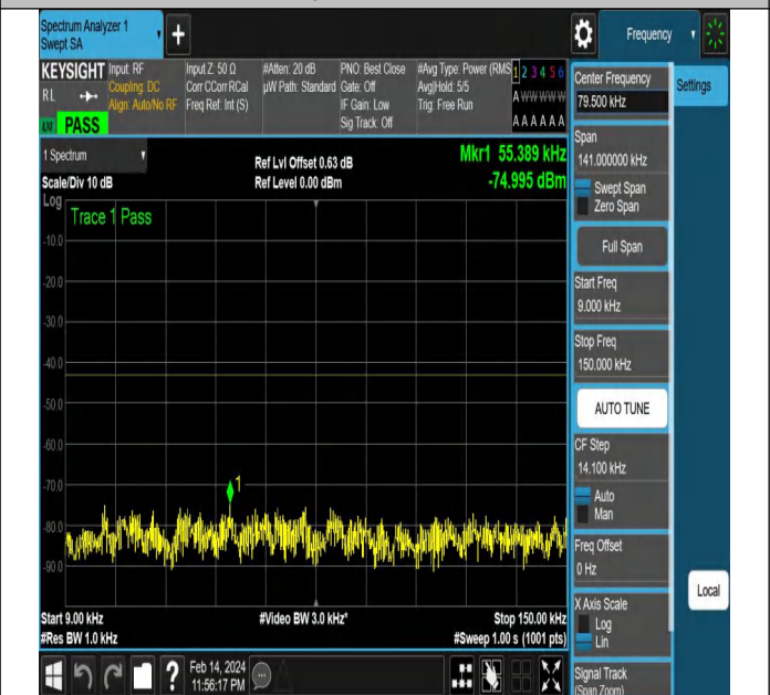
NTVN-N77-3450-3550-PC2-30-60-M-DFT-PI2BPSK-Edge_1RB_ B_Left-Ant1-PASS
