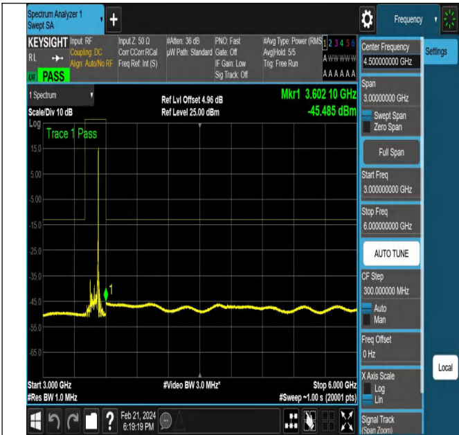
NTVN-N77-3450-3550-PC2-30-80-L-DFT-QPSK-Edge_1RB_ Right-Ant1-PASS
