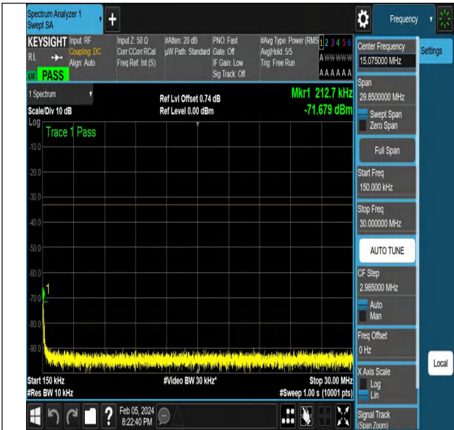
NTNV-N77-3450-3550-PC2-30-80-H-DFT-PI2BPSK-Edge_1R B_Left-Ant1-PASS
