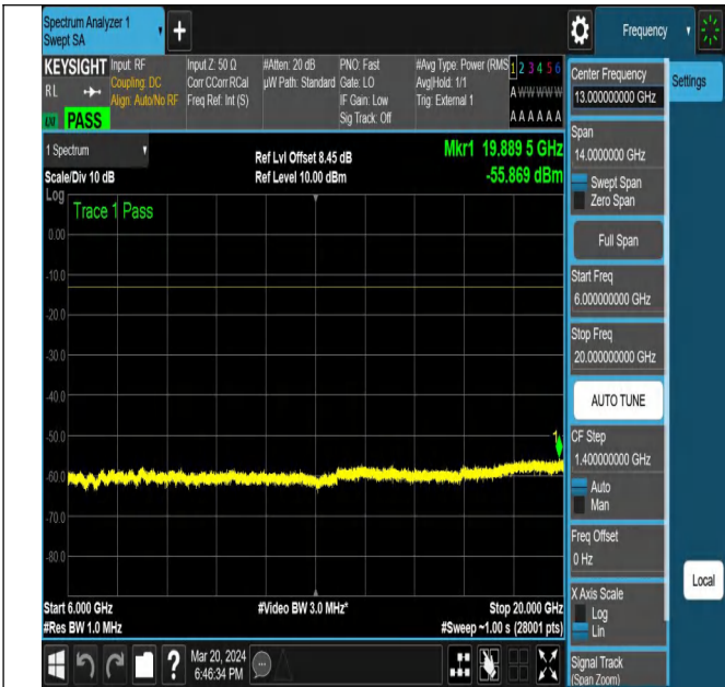
NTNV-N77-3450-3550-PC2-30-80-L-DFT-PI2BPSK-Edge_1R B_Left-Ant1-PASS
