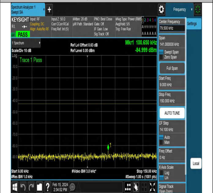
NTNV-N77-3450-3550-PC2-30-80-L-DFT-PI2BPSK-Edge_1R
