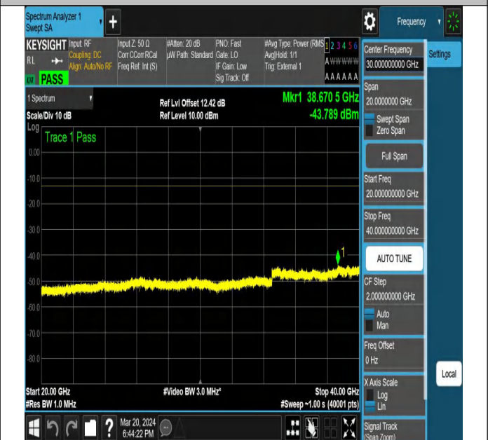
NTNV-N77-3450-3550-PC2-30-50-H-DFT-QPSK-Edge_1RB_
