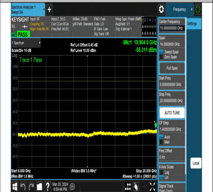
NTNV-N77-3450-3550-PC2-30-80-H-DFT-PI2BPSK-Edge_1R B_Right-Ant1-PASS
