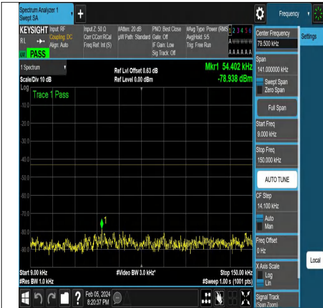
NTNV-N77-3450-3550-PC2-30-80-M-DFT-QPSK-Edge_1RB_ Right-Ant1-PASS
