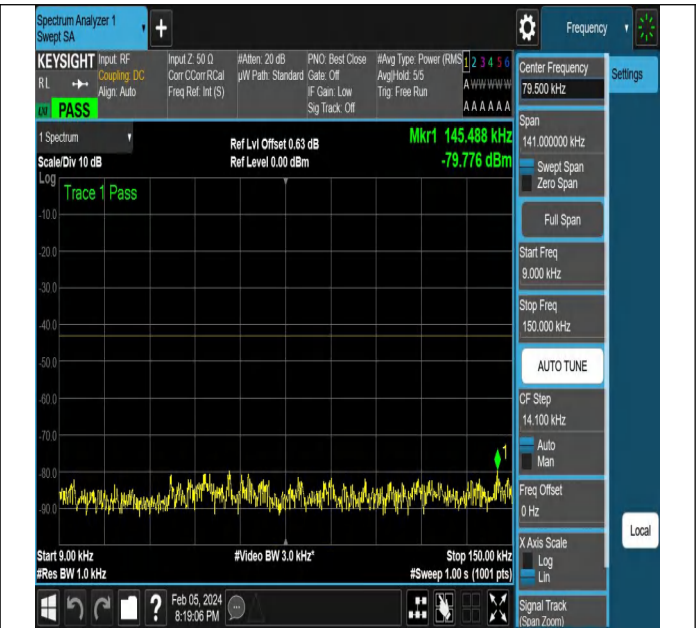
NTNV-N77-3450-3550-PC2-30-80-M-DFT-QPSK-Edge_1RB_Left-Ant1-PASS
