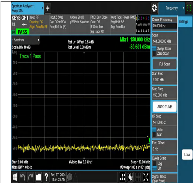
NTNV-N77-3450-3550-PC2-30-80-L-DFT-QPSK-Edge_1RB_ Right-Ant1-PASS
