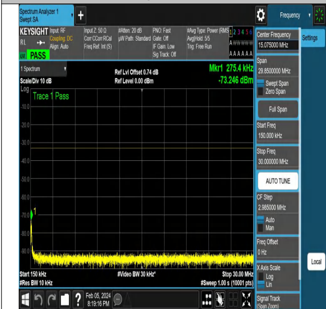
NTNV-N77-3450-3550-PC2-30-80-M-DFT-QPSK-Edge_1RB_Left-Ant1-PASS
