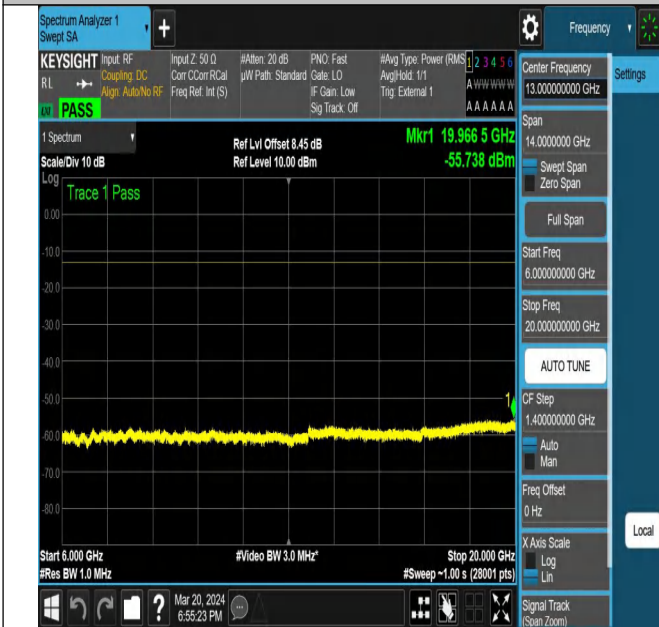
NTNV-N77-3450-3550-PC2-30-80-M-DFT-QPSK-Edge_1RB_ Left-Ant1-PASS
