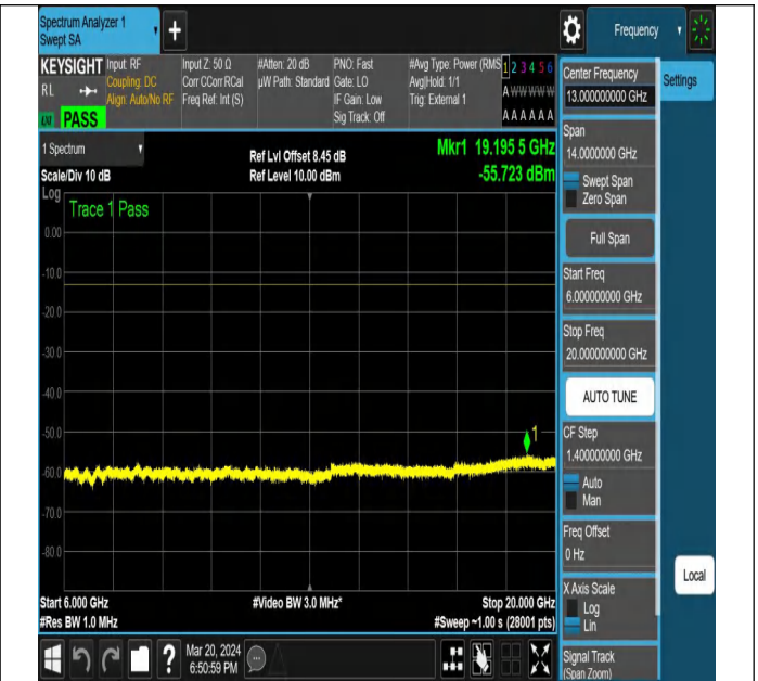
NTVN-N77-3450-3550-PC2-30-80-L-DFT-QPSK-Edge_1RB_ Right-Ant1-PASS
