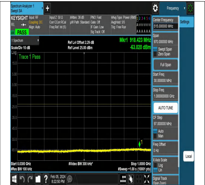
NTNV-N77-3450-3550-PC2-30-80-H-DFT-PI2BPSK-Edge_1R B_Left-Ant1-PASS
