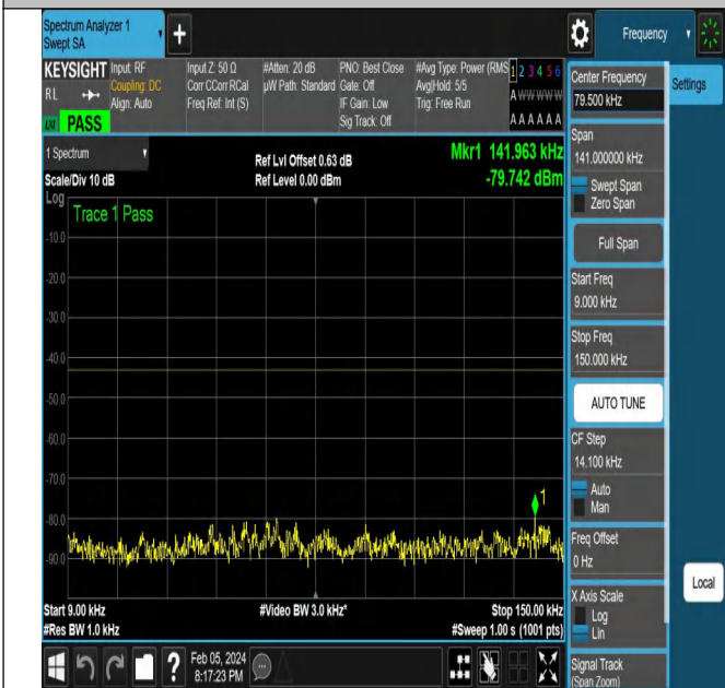
NTNV-N77-3450-3550-PC2-30-80-M-DFT-PI2BPSK-Edge_1R B_Right-Ant1-PASS
