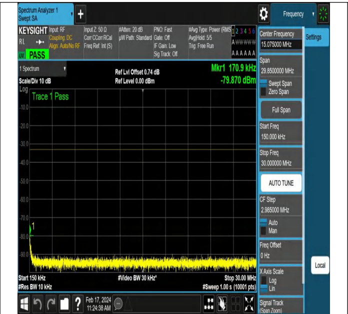
NTNV-N77-3450-3550-PC2-30-80-L-DFT-QPSK-Edge_1RB_ Right-Ant1-PASS
