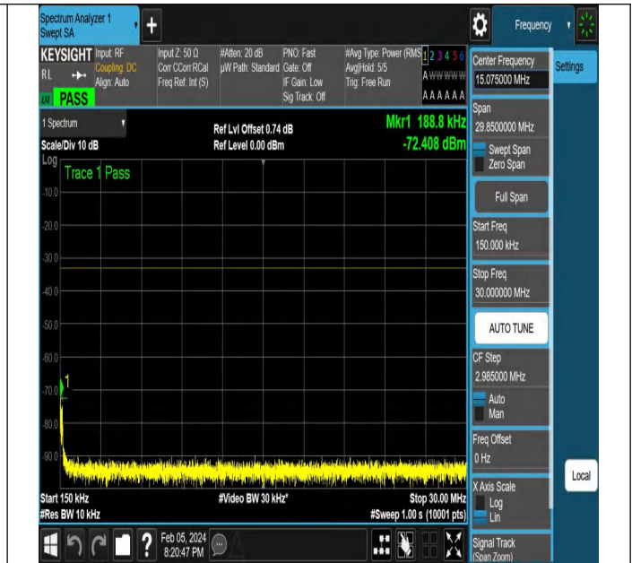
NTNV-N77-3450-3550-PC2-30-80-M-DFT-QPSK-Edge_1RB_ Right-Ant1-PASS
