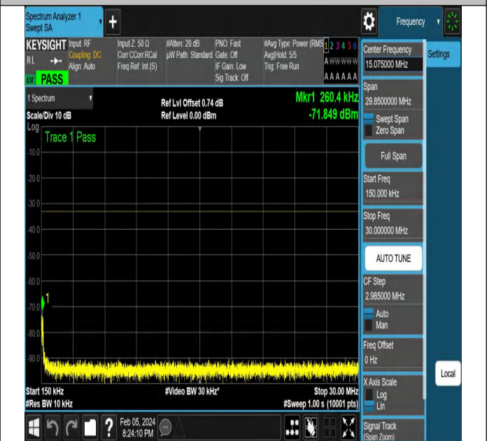
NTNV-N77-3450-3550-PC2-30-80-H-DFT-PI2BPSK-Edge_1R B_Right-Ant1-PASS
