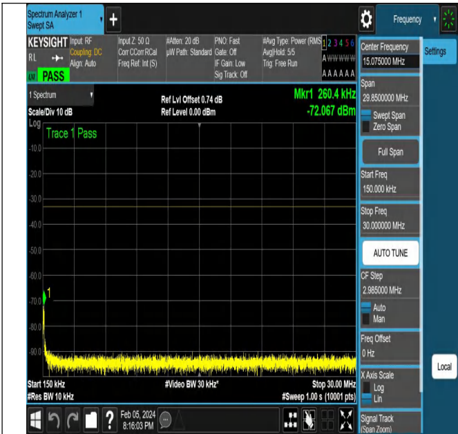
NTNV-N77-3450-3550-PC2-30-80-M-DFT-PI2BPSK-Edge_1R B_Left-Ant1-PASS
