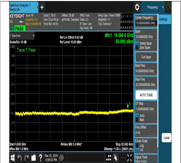
NTNV-N77-3450-3550-PC2-30-80-M-DFT-QPSK-Edge_1RB_ Right-Ant1-PASS
