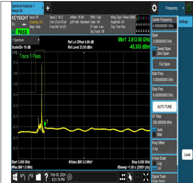
NTNV-N77-3450-3550-PC2-30-80-M-DFT-QPSK-Edge_1RB_ Right-Ant1-PASS
