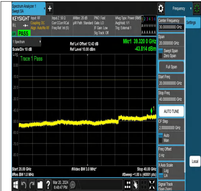
NTNV-N77-3450-3550-PC2-30-80-L-DFT-PI2BPSK-Edge_1R_B_Right-Ant1-PASS
