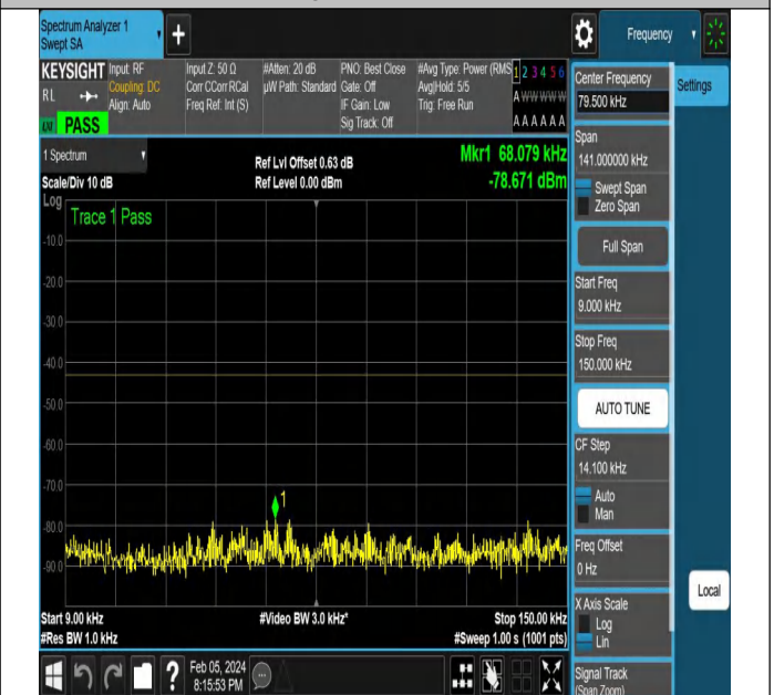
NTVN-N77-3450-3550-PC2-30-80-M-DFT-PI2BPSK-Edge_1RB_ B_Left-Ant1-PASS
