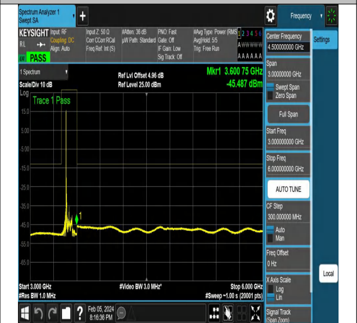
NTNV-N77-3450-3550-PC2-30-80-M-DFT-PI2BPSK-Edge_1R B_Left-Ant1-PASS
