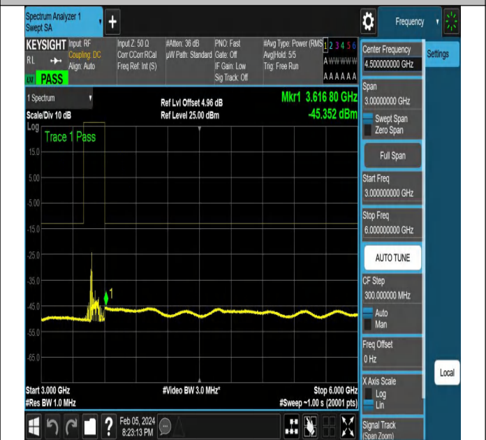
NTNV-N77-3450-3550-PC2-30-80-H-DFT-PI2BPSK-Edge_1R B_Left-Ant1-PASS
