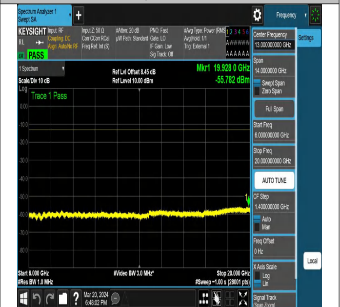
NTNV-N77-3450-3550-PC2-30-80-L-DFT-PI2BPSK-Edge_1R B_Right-Ant1-PASS
