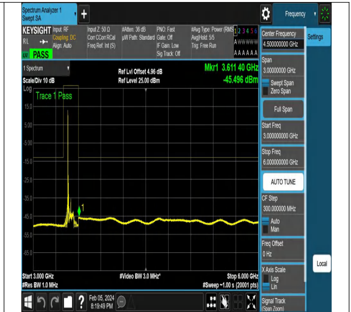
NTNV-N77-3450-3550-PC2-30-80-M-DFT-QPSK-Edge_1RB_ Left-Ant1-PASS
