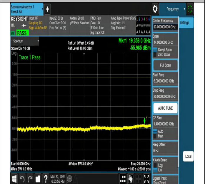
NTNV-N77-3450-3550-PC2-30-80-M-DFT-PI2BPSK-Edge_1R B_Right-Ant1-PASS
