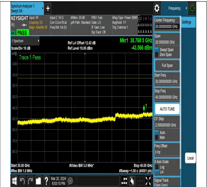
NTNV-N77-3450-3550-PC2-30-80-M-DFT-PI2BPSK-Edge_1R B_Left-Ant1-PASS
