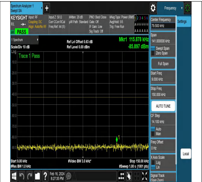
NTNV-N77-3450-3550-PC2-30-80-L-DFT-QPSK-Edge_1RB_L_eft-Ant1-PASS
