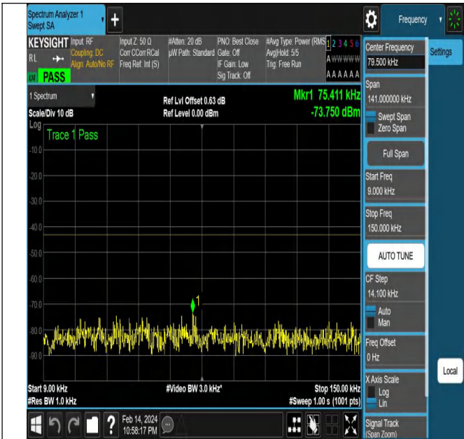
NTNV-N77-3450-3550-PC2-30-40-M-DFT-PI2BPSK-Edge_1R B_Left-Ant1-PASS
