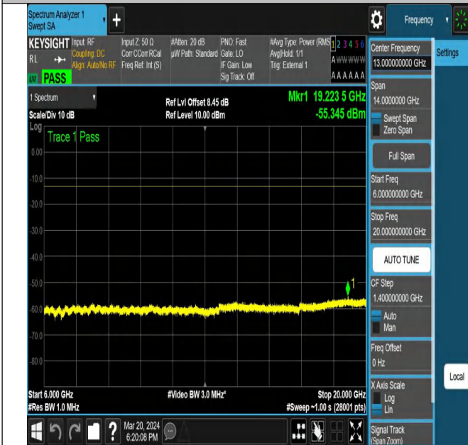
NTNV-N77-3450-3550-PC2-30-40-M-DFT-QPSK-Edge_1RB_ Right-Ant1-PASS
