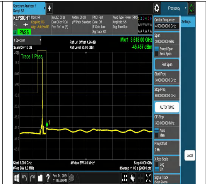
NTNV-N77-3450-3550-PC2-30-40-M-DFT-QPSK-Edge_1RB_ Right-Ant1-PASS
