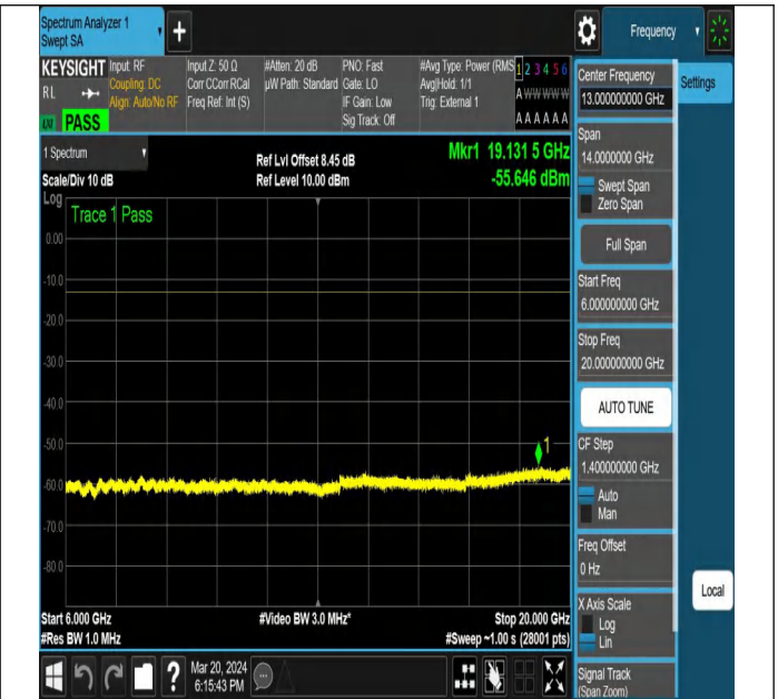
NTNV-N77-3450-3550-PC2-30-40-M-DFT-PI2BPSK-Edge_1R B_Left-Ant1-PASS
