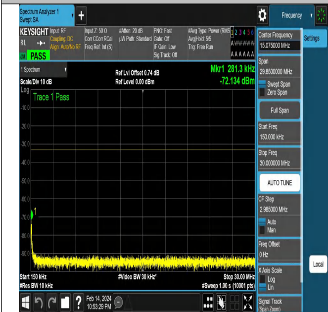
NTNV-N77-3450-3550-PC2-30-40-L-DFT-QPSK-Edge_1RB_ Right-Ant1-PASS
