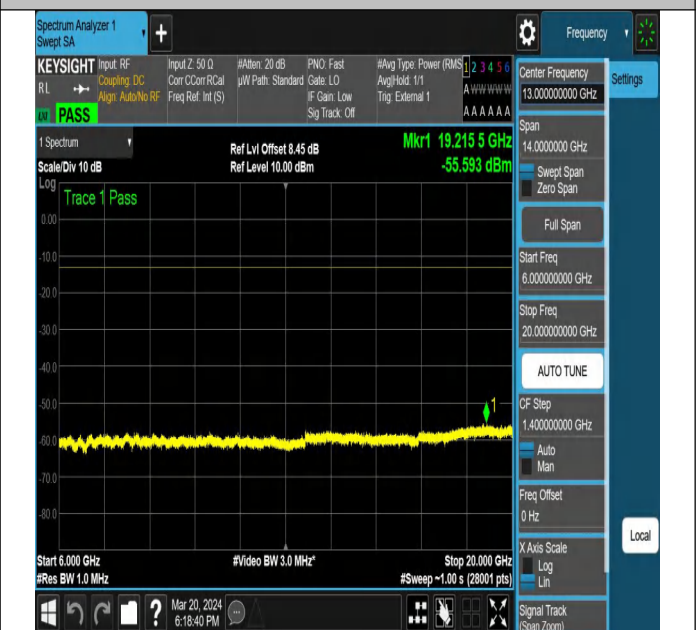
NTNV-N77-3450-3550-PC2-30-40-M-DFT-QPSK-Edge_1RB_ Left-Ant1-PASS
