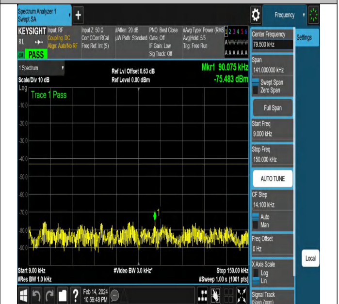
NTNV-N77-3450-3550-PC2-30-40-M-DFT-PI2BPSK-Edge_1R B_Right-Ant1-PASS
