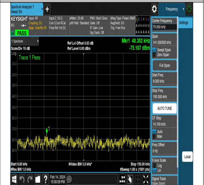
NTNV-N77-3450-3550-PC2-30-40-L-DFT-PI2BPSK-Edge_1R B_Right-Ant1-PASS
