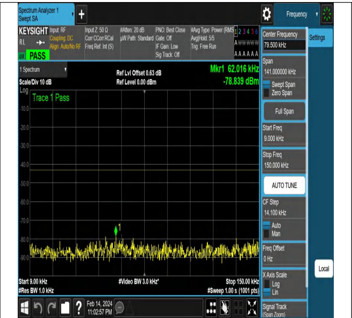
NTNV-N77-3450-3550-PC2-30-40-M-DFT-QPSK-Edge_1RB_ Right-Ant1-PASS
