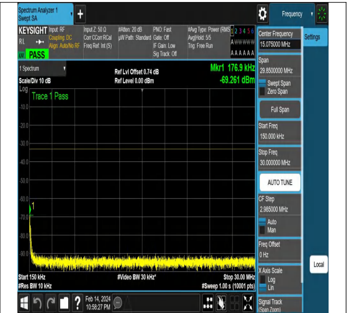
NTNV-N77-3450-3550-PC2-30-40-M-DFT-PI2BPSK-Edge_1R B_Left-Ant1-PASS
