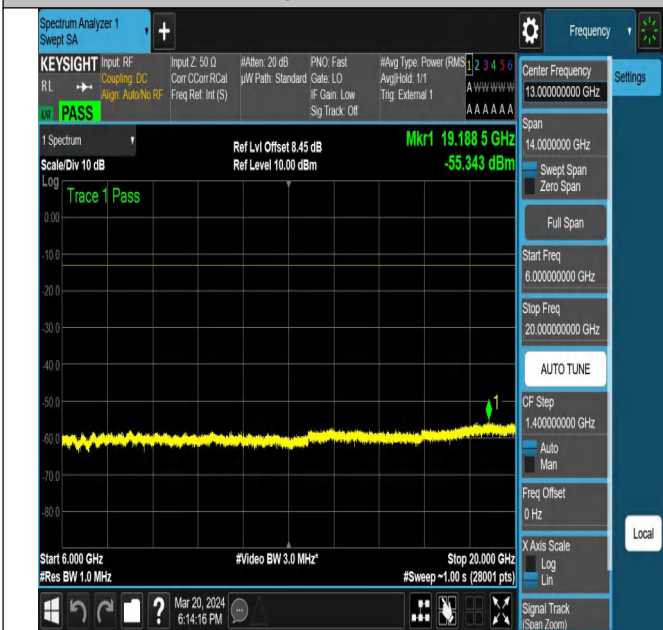
NTNV-N77-3450-3550-PC2-30-40-L-DFT-QPSK-Edge_1RB_
