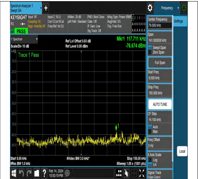
NTNV-N77-3450-3550-PC2-30-40-L-DFT-QPSK-Edge_1RB_ Right-Ant1-PASS
