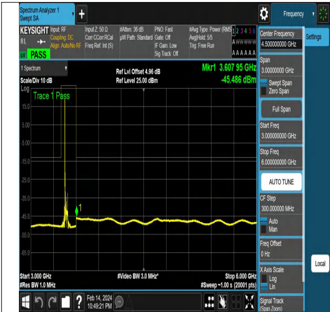
NTNV-N77-3450-3550-PC2-30-40-L-DFT-PI2BPSK-Edge_1R B_Left-Ant1-PASS
