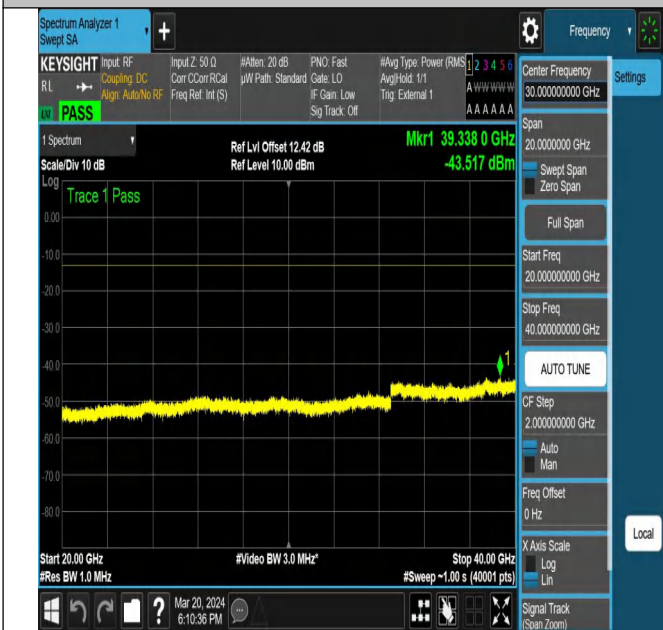
NTNV-N77-3450-3550-PC2-30-40-L-DFT-PI2BPSK-Edge_1R B_Left-Ant1-PASS
