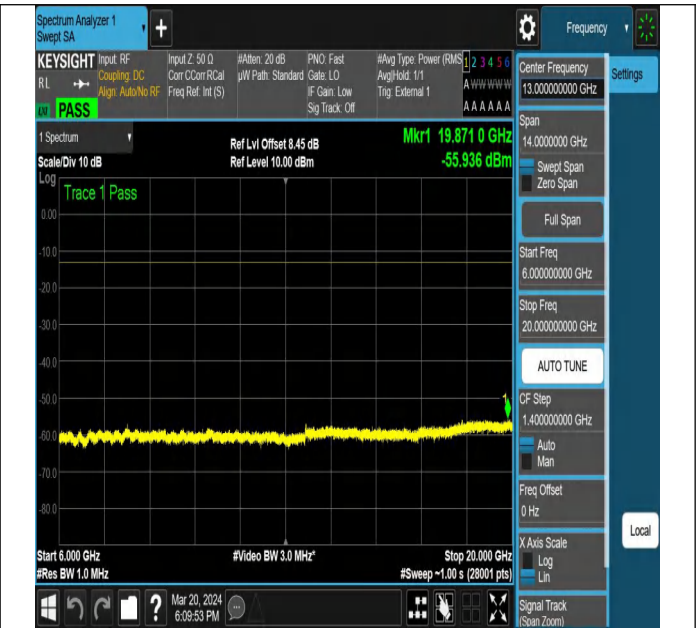
NTNV-N77-3450-3550-PC2-30-40-L-DFT-PI2BPSK-Edge_1R B_Left-Ant1-PASS
