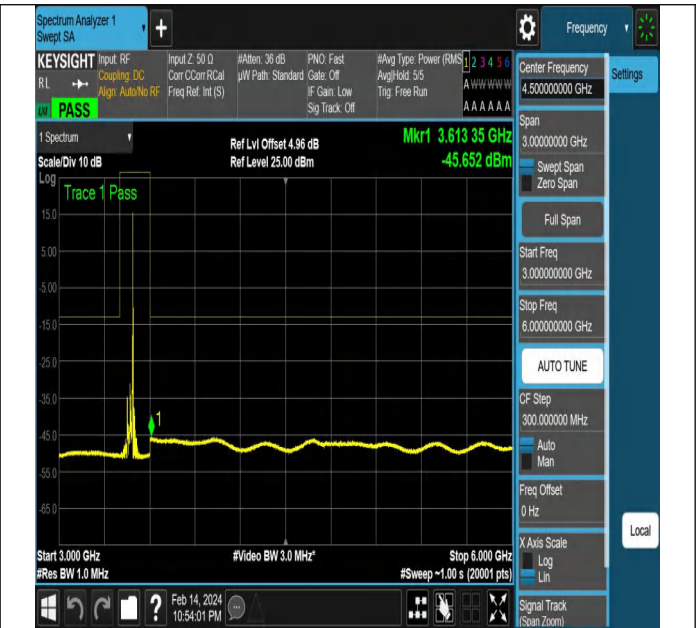
NTNV-N77-3450-3550-PC2-30-40-L-DFT-QPSK-Edge_1RB_
