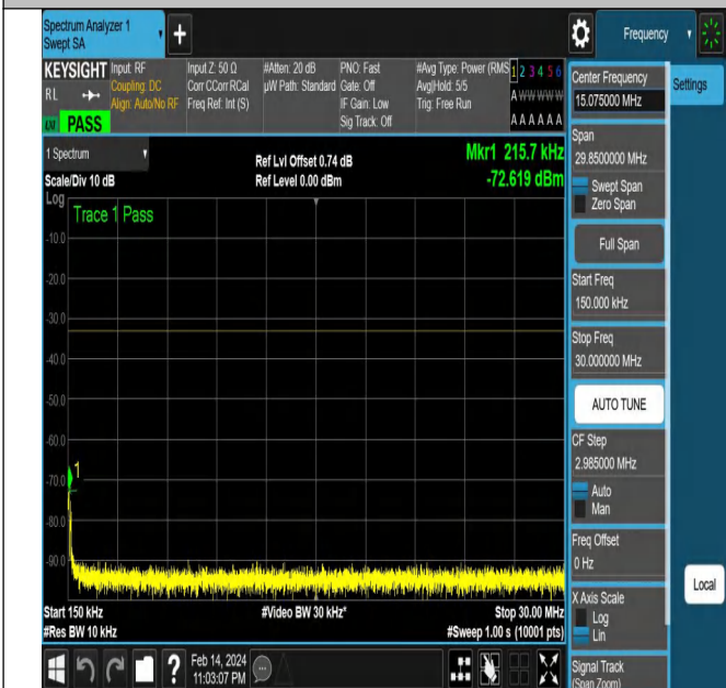
NTNV-N77-3450-3550-PC2-30-40-M-DFT-QPSK-Edge_1RB_ Right-Ant1-PASS
