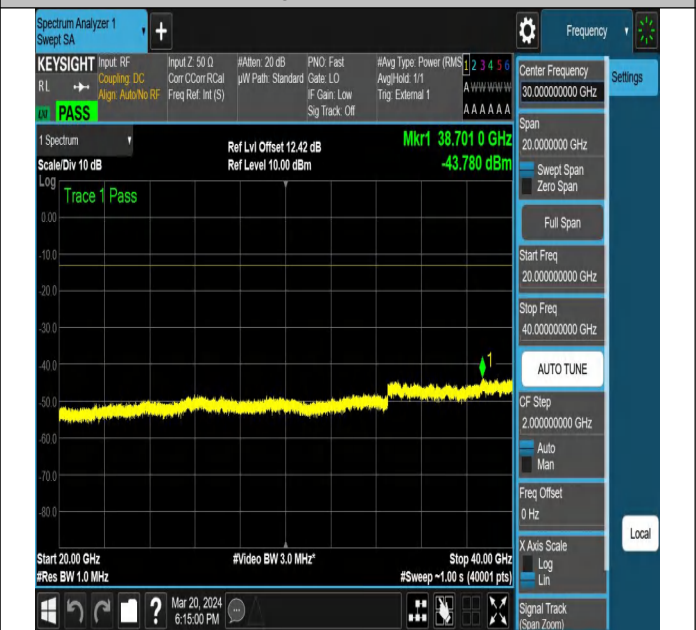
NTNV-N77-3450-3550-PC2-30-40-L-DFT-QPSK-Edge_1RB_
