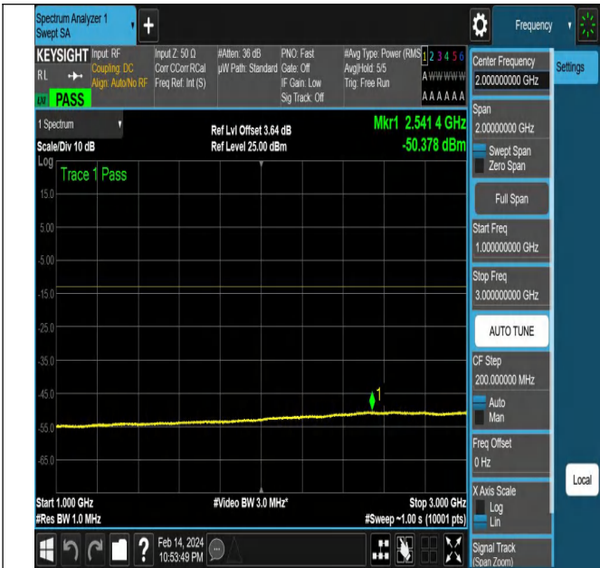
NTNV-N77-3450-3550-PC2-30-40-L-DFT-QPSK-Edge_1RB_
