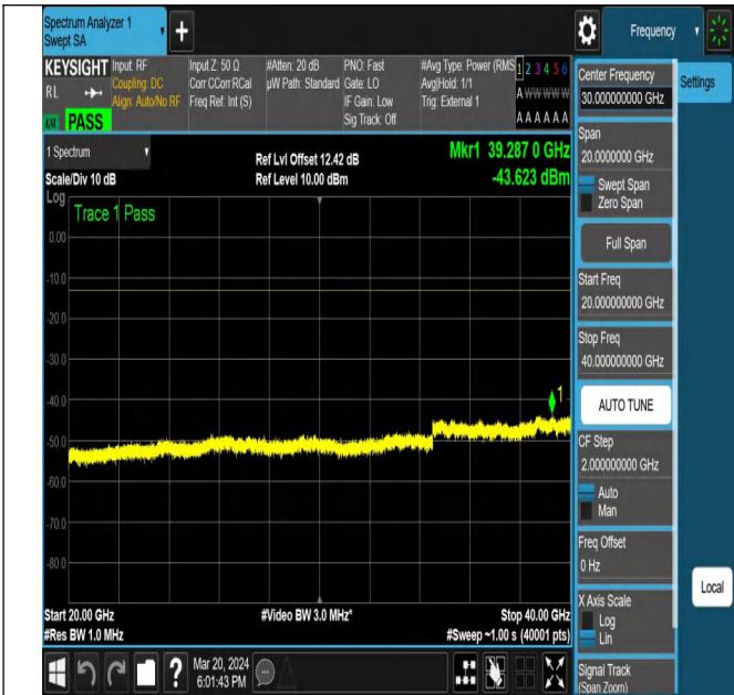
NTNV-N77-3450-3550-PC2-30-20-M-DFT-QPSK-Edge_1RB_
