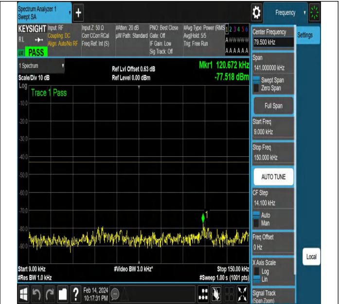
NTNV-N77-3450-3550-PC2-30-20-L-DFT-QPSK-Edge_1RB_ Right-Ant1-PASS
