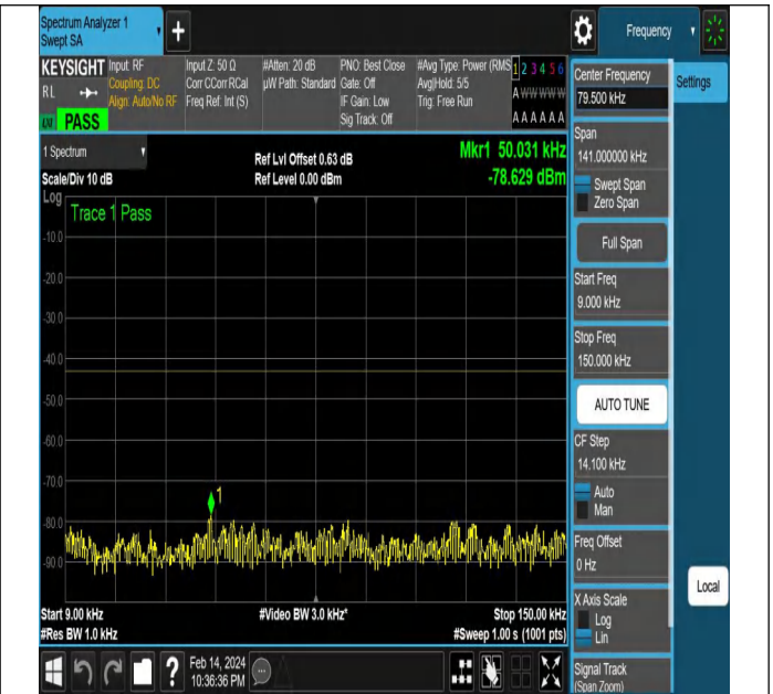
NTNV-N77-3450-3550-PC2-30-20-H-DFT-QPSK-Edge_1RB_ Right-Ant1-PASS
