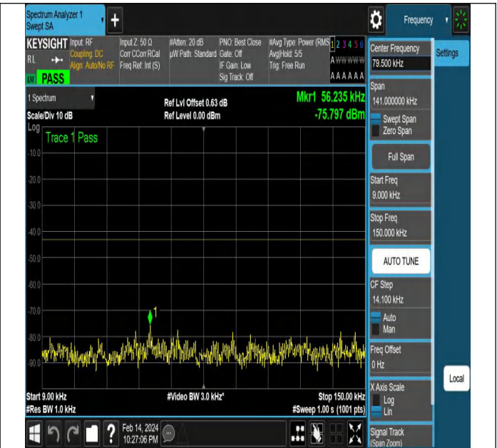
NTNV-N77-3450-3550-PC2-30-20-M-DFT-QPSK-Edge_1RB_
