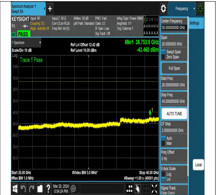
NTNV-N77-3450-3550-PC2-30-20-L-DFT-PI2BPSK-Edge_1R B_Right-Ant1-PASS
