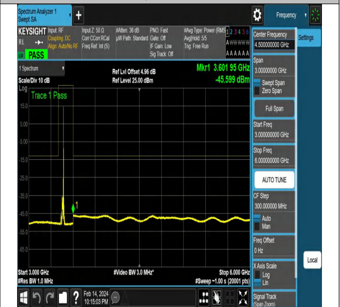
NTNV-N77-3450-3550-PC2-30-20-L-DFT-PI2BPSK-Edge_1R B_Right-Ant1-PASS
