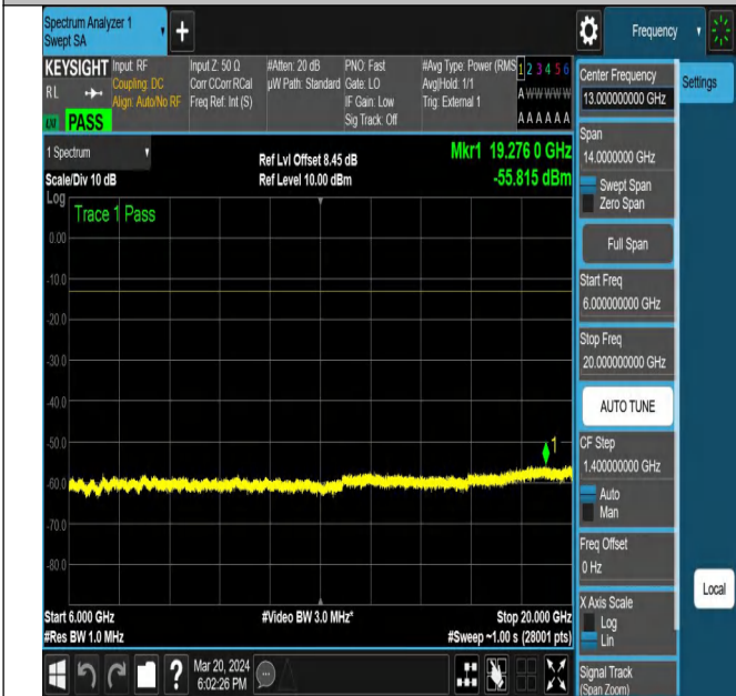
NTNV-N77-3450-3550-PC2-30-20-M-DFT-QPSK-Edge_1RB_ Right-Ant1-PASS
