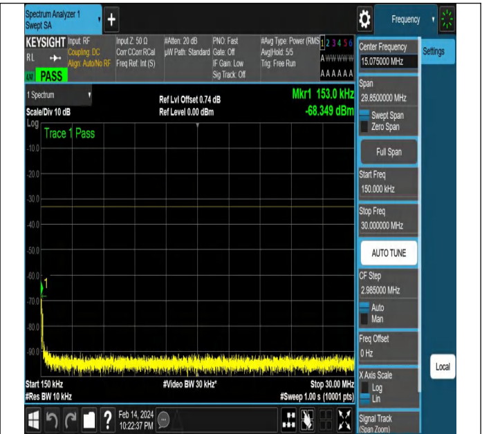
NTNV-N77-3450-3550-PC2-30-20-M-DFT-PI2BPSK-Edge_1R B_Left-Ant1-PASS
