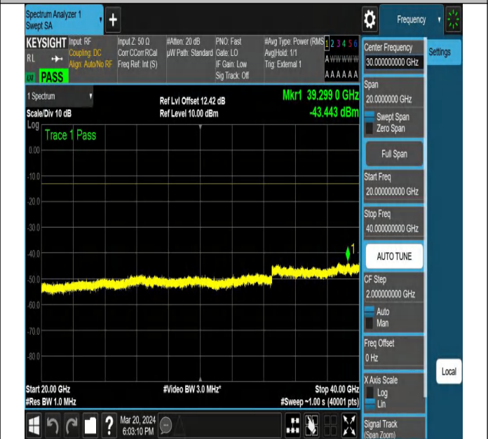
NTNV-N77-3450-3550-PC2-30-20-M-DFT-QPSK-Edge_1RB_ Right-Ant1-PASS
