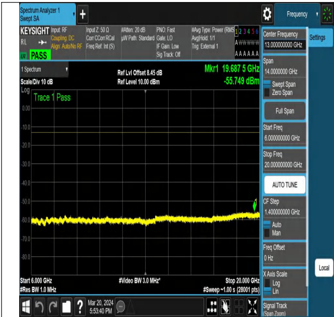
NTNV-N77-3450-3550-PC2-30-20-L-DFT-PI2BPSK-Edge_1R B_Right-Ant1-PASS
