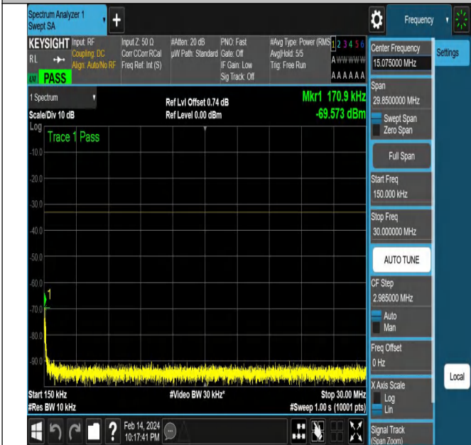
NTNV-N77-3450-3550-PC2-30-20-L-DFT-QPSK-Edge_1RB_ Right-Ant1-PASS
