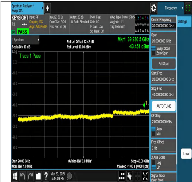
NTNV-N77-3450-3550-PC2-30-15-M-DFT-QPSK-Edge_1RB_ Left-Ant1-PASS
