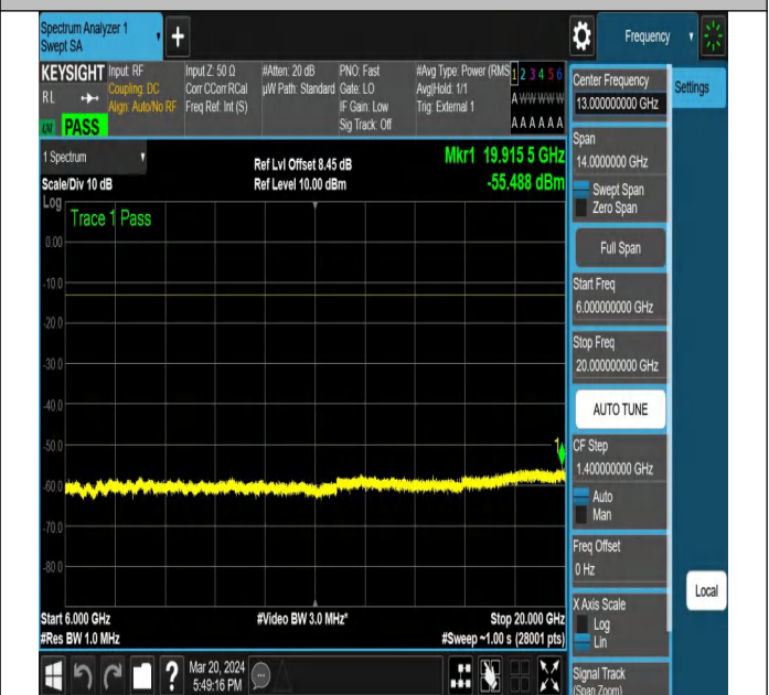
NTNV-N77-3450-3550-PC2-30-15-H-DFT-QPSK-Edge_1RB_ Left-Ant1-PASS
