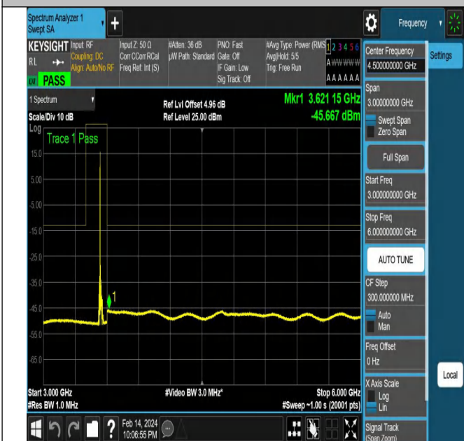
NTNV-N77-3450-3550-PC2-30-15-H-DFT-QPSK-Edge_1RB_ Left-Ant1-PASS
