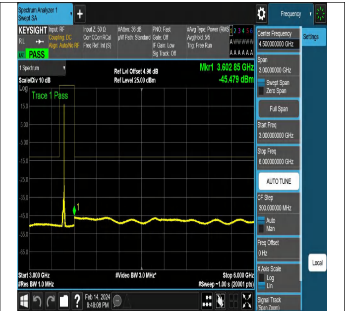
NTNV-N77-3450-3550-PC2-30-15-L-DFT-QPSK-Edge_1RB_
