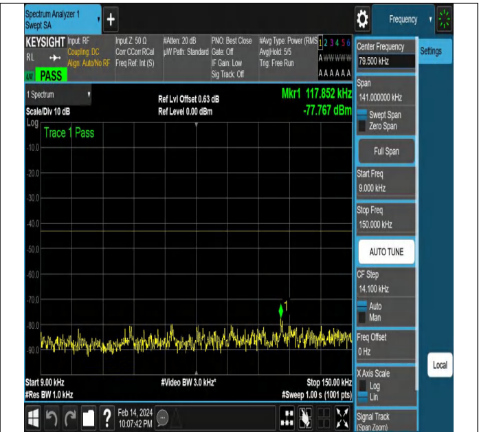
NTNV-N77-3450-3550-PC2-30-15-H-DFT-QPSK-Edge_1RB_ Right-Ant1-PASS
