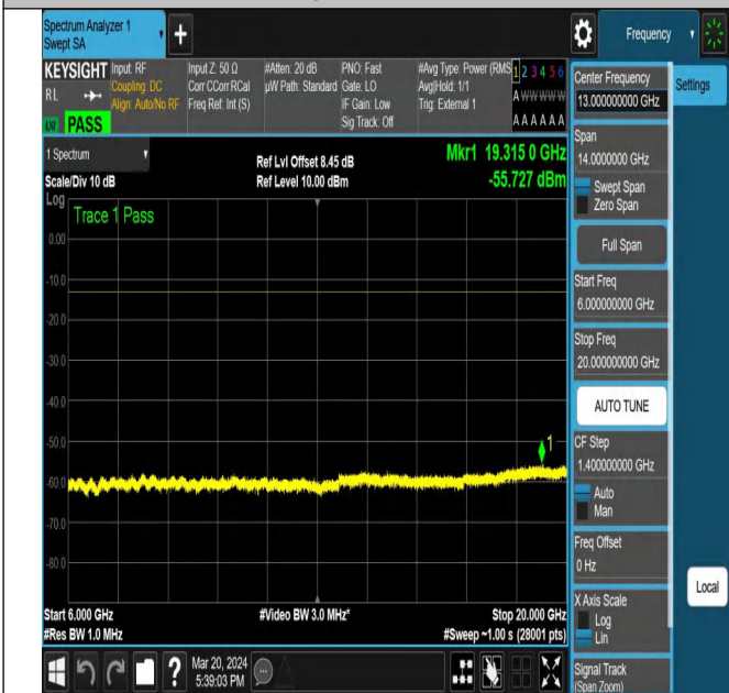
NTNV-N77-3450-3550-PC2-30-15-L-DFT-QPSK-Edge_1RB_
