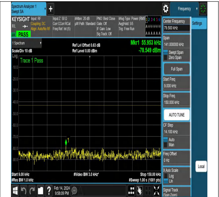
NTNV-N77-3450-3550-PC2-30-15-M-DFT-QPSK-Edge_1RB_ Right-Ant1-PASS
