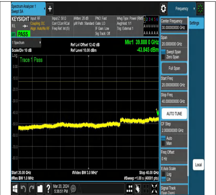
NTNV-N77-3450-3550-PC2-30-15-L-DFT-PI2BPSK-Edge_1R B_Right-Ant1-PASS
