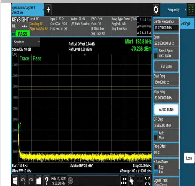
NTNV-N77-3450-3550-PC2-30-15-M-DFT-QPSK-Edge_1RB_ Right-Ant1-PASS
