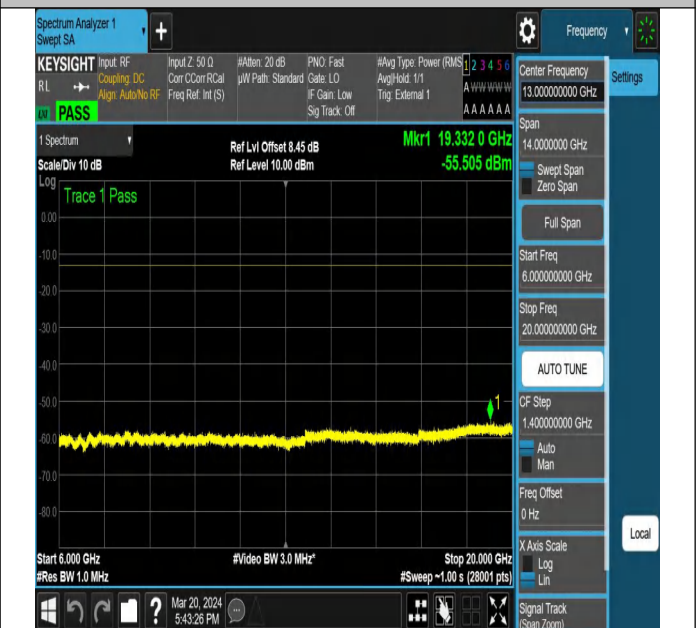
NTNV-N77-3450-3550-PC2-30-15-M-DFT-QPSK-Edge_1RB_ Left-Ant1-PASS
