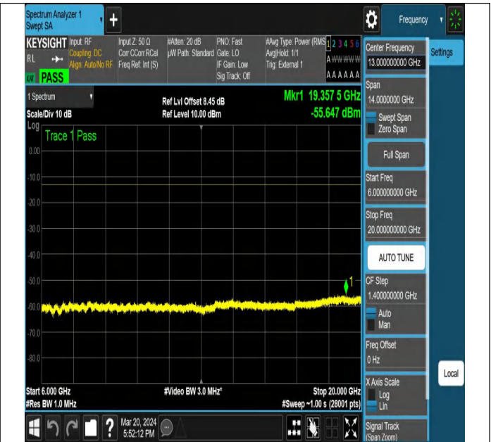
NTNV-N77-3450-3550-PC2-30-20-L-DFT-PI2BPSK-Edge_1R B_Left-Ant1-PASS
