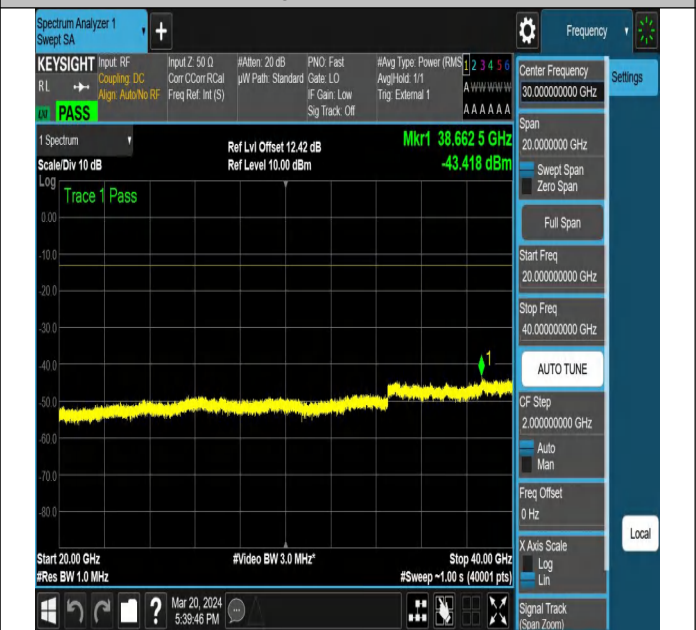
NTNV-N77-3450-3550-PC2-30-15-L-DFT-QPSK-Edge_1RB_
