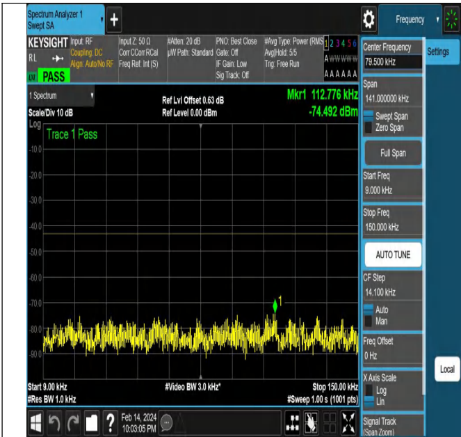
NTNV-N77-3450-3550-PC2-30-15-H-DFT-PI2BPSK-Edge_1R B_Left-Ant1-PASS
