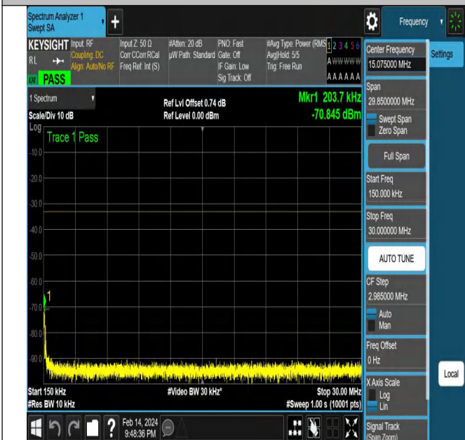
NTNV-N77-3450-3550-PC2-30-15-L-DFT-QPSK-Edge_1RB_ Right-Ant1-PASS
