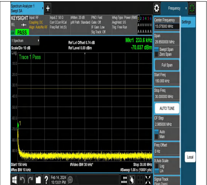
NTNV-N77-3450-3550-PC2-30-20-L-DFT-PI2BPSK-Edge_1R B_Left-Ant1-PASS
