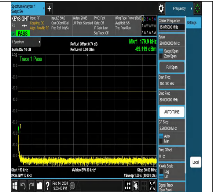
NTNV-N77-3450-3550-PC2-30-15-M-DFT-PI2BPSK-Edge_1R B_Left-Ant1-PASS
