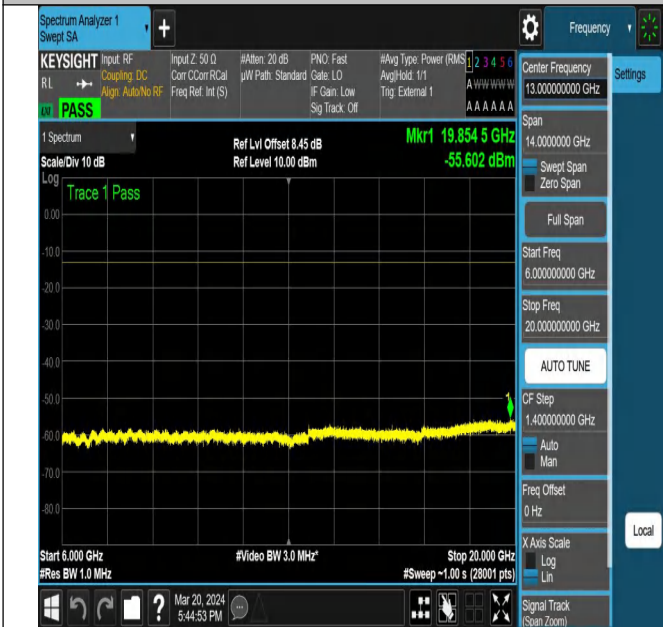
NTNV-N77-3450-3550-PC2-30-15-M-DFT-QPSK-Edge_1RB_ Right-Ant1-PASS
