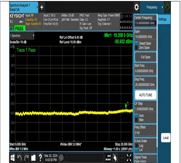
NTNV-N77-3450-3550-PC2-30-15-M-DFT-PI2BPSK-Edge_1R B_Left-Ant1-PASS
