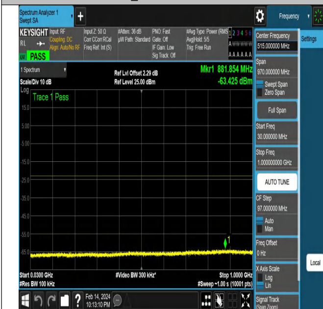
NTNV-N77-3450-3550-PC2-30-20-L-DFT-PI2BPSK-Edge_1R B_Left-Ant1-PASS
