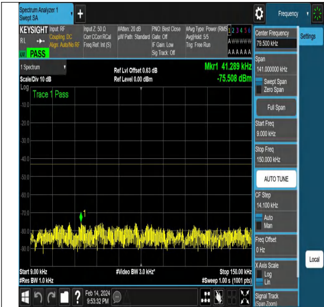
NTNV-N77-3450-3550-PC2-30-15-M-DFT-PI2BPSK-Edge_1R B_Left-Ant1-PASS
