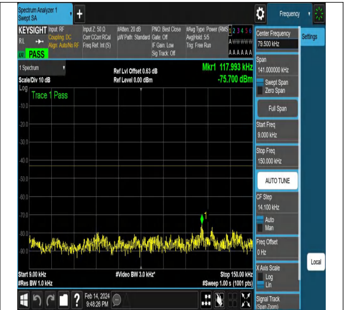
NTNV-N77-3450-3550-PC2-30-15-L-DFT-QPSK-Edge_1RB_ Right-Ant1-PASS
