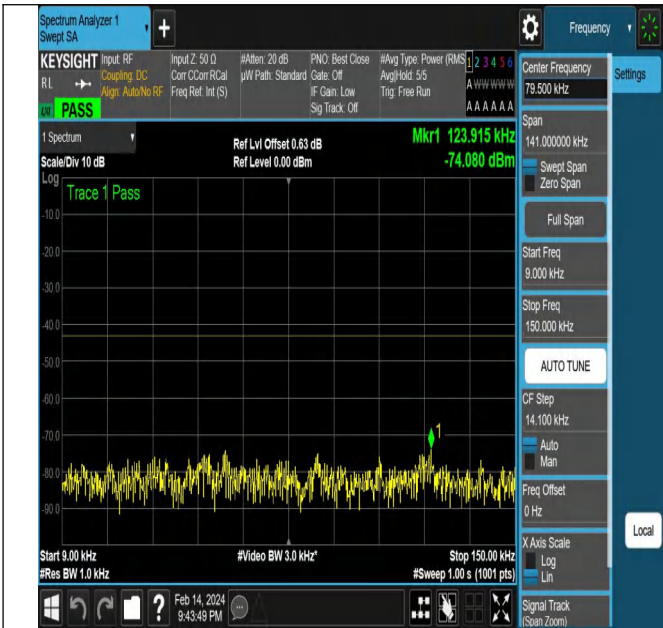
NTNV-N77-3450-3550-PC2-30-15-L-DFT-PI2BPSK-Edge_1R B_Left-Ant1-PASS
