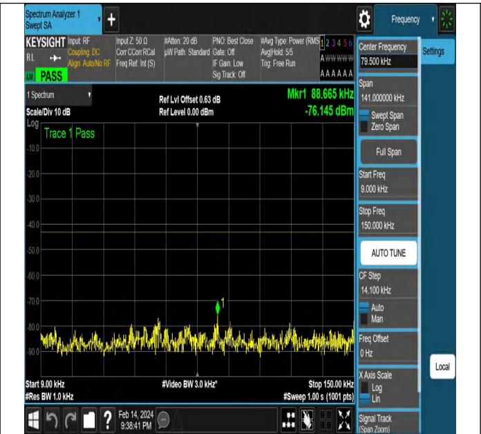
NTNV-N77-3450-3550-PC2-30-10-H-DFT-QPSK-Edge_1RB_ Right-Ant1-PASS
