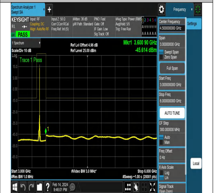
NTNV-N77-3450-3550-PC2-30-15-L-DFT-PI2BPSK-Edge_1R B_Right-Ant1-PASS
