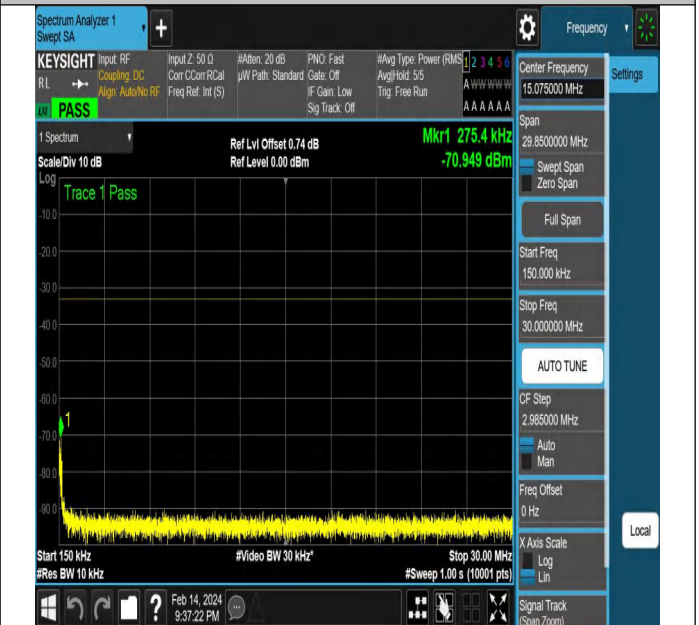
NTNV-N77-3450-3550-PC2-30-10-H-DFT-QPSK-Edge_1RB_ Left-Ant1-PASS
