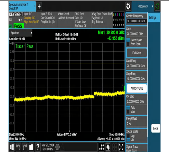
NTNV-N77-3450-3550-PC2-30-10-H-DFT-PI2BPSK-Edge_1R B_Right-Ant1-PASS
