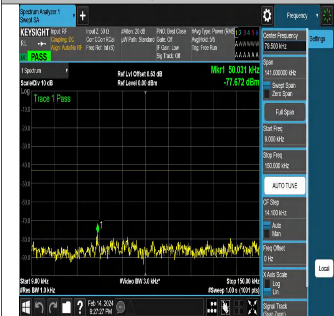
NTNV-N77-3450-3550-PC2-30-10-M-DFT-QPSK-Edge_1RB_ Left-Ant1-PASS
