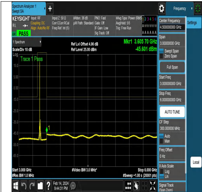
NTNV-N77-3450-3550-PC2-30-15-L-DFT-PI2BPSK-Edge_1R
