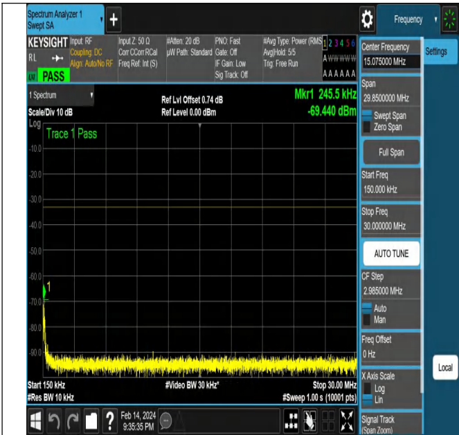
NTNV-N77-3450-3550-PC2-30-10-H-DFT-PI2BPSK-Edge_1R B_Right-Ant1-PASS
