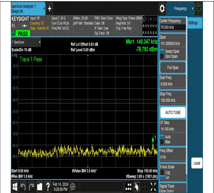
NTNV-N77-3450-3550-PC2-30-10-M-DFT-QPSK-Edge_1RB_
