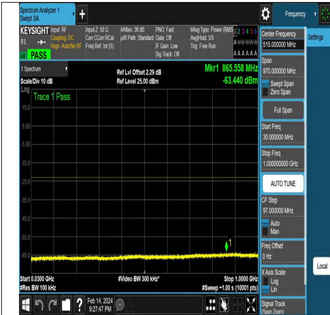
NTNV-N77-3450-3550-PC2-30-10-M-DFT-QPSK-Edge_1RB_ Left-Ant1-PASS
