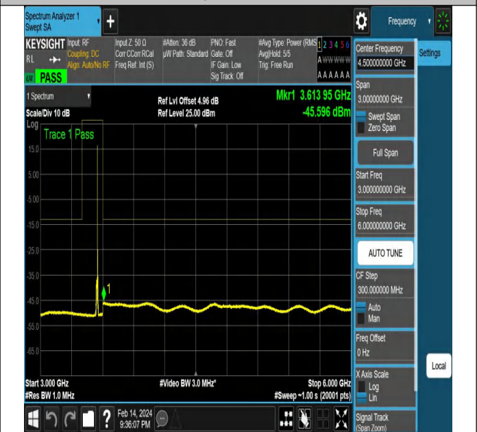
NTNV-N77-3450-3550-PC2-30-10-H-DFT-PI2BPSK-Edge_1R B_Right-Ant1-PASS
