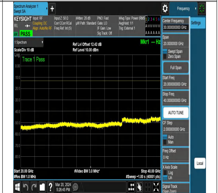
NTNV-N77-3450-3550-PC2-30-10-M-DFT-QPSK-Edge_1RB_ Right-Ant1-PASS
