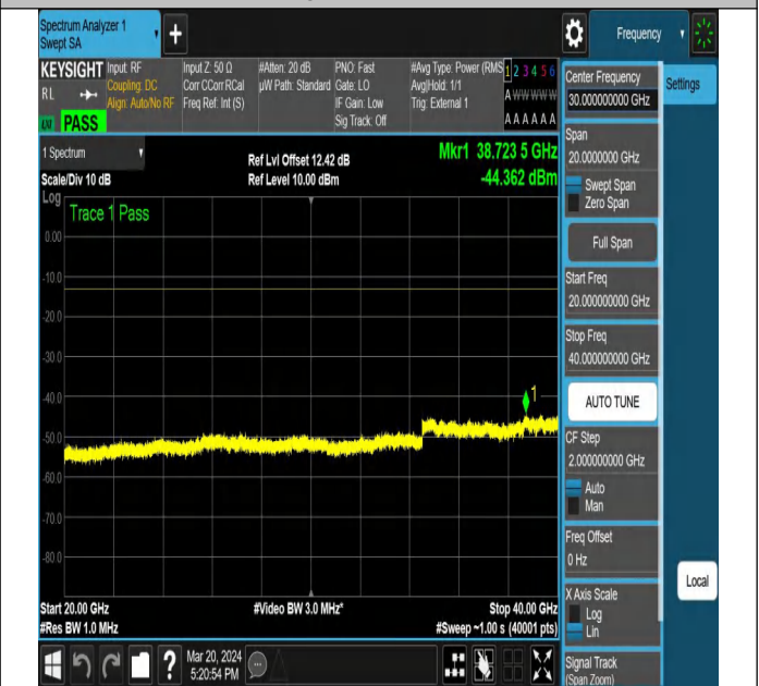
NTNV-N77-3450-3550-PC2-30-10-L-DFT-QPSK-Edge_1RB_
