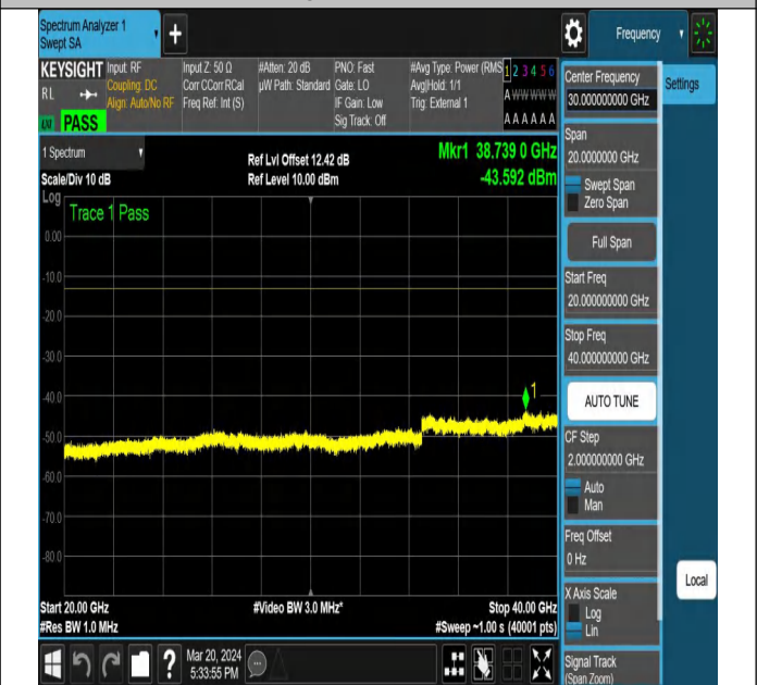
NTNV-N77-3450-3550-PC2-30-10-H-DFT-QPSK-Edge_1RB_ Right-Ant1-PASS
