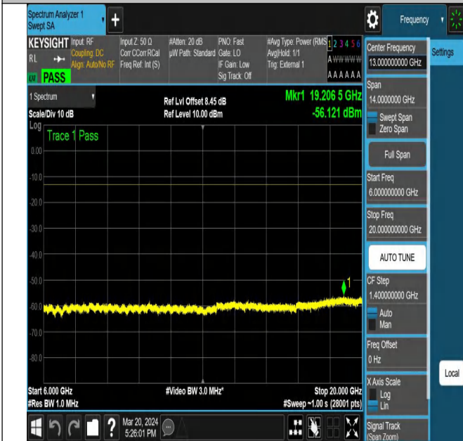
NTNV-N77-3450-3550-PC2-30-10-M-DFT-QPSK-Edge_1RB_ Right-Ant1-PASS
