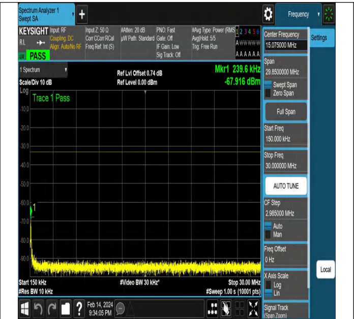
NTNV-N77-3450-3550-PC2-30-10-H-DFT-PI2BPSK-Edge_1R B_Left-Ant1-PASS
