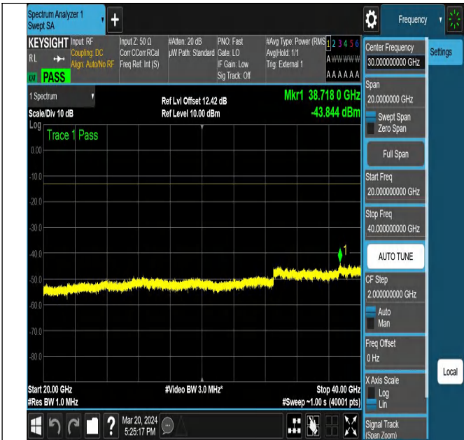
NTNV-N77-3450-3550-PC2-30-10-M-DFT-QPSK-Edge_1RB_
