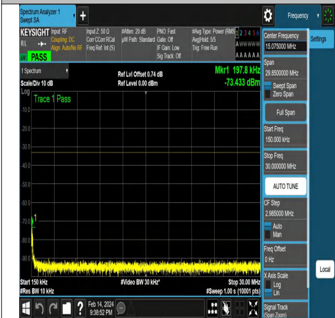
NTNV-N77-3450-3550-PC2-30-10-H-DFT-QPSK-Edge_1RB_ Right-Ant1-PASS
