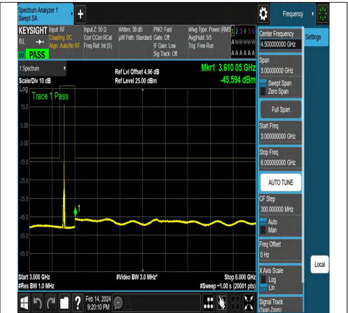
NTNV-N77-3450-3550-PC2-30-10-L-DFT-QPSK-Edge_1RB_
