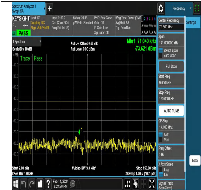
NTNV-N77-3450-3550-PC2-30-10-M-DFT-PI2BPSK-Edge_1R B_Left-Ant1-PASS
