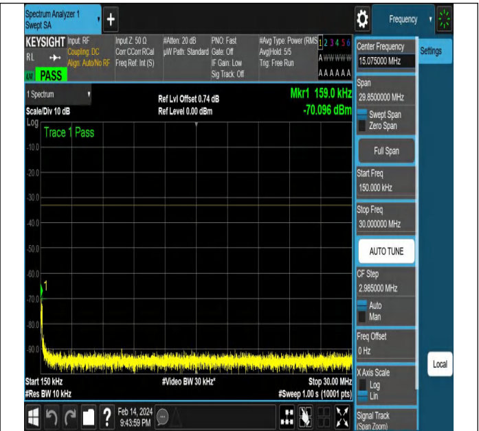
NTNV-N77-3450-3550-PC2-30-15-L-DFT-PI2BPSK-Edge_1R B_Left-Ant1-PASS
