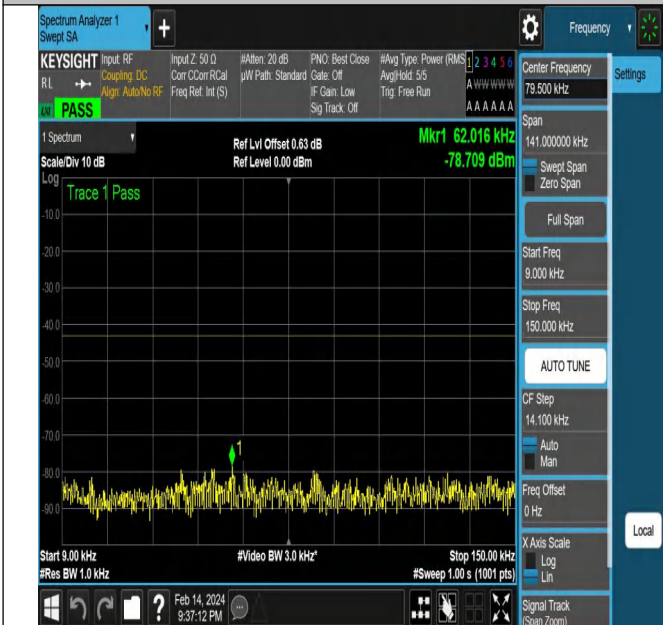
NTNV-N77-3450-3550-PC2-30-10-H-DFT-QPSK-Edge_1RB_ Left-Ant1-PASS
