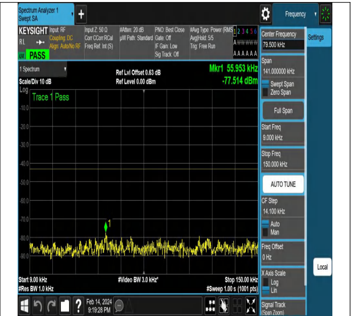
NTNV-N77-3450-3550-PC2-30-10-L-DFT-QPSK-Edge_1RB_ Right-Ant1-PASS
