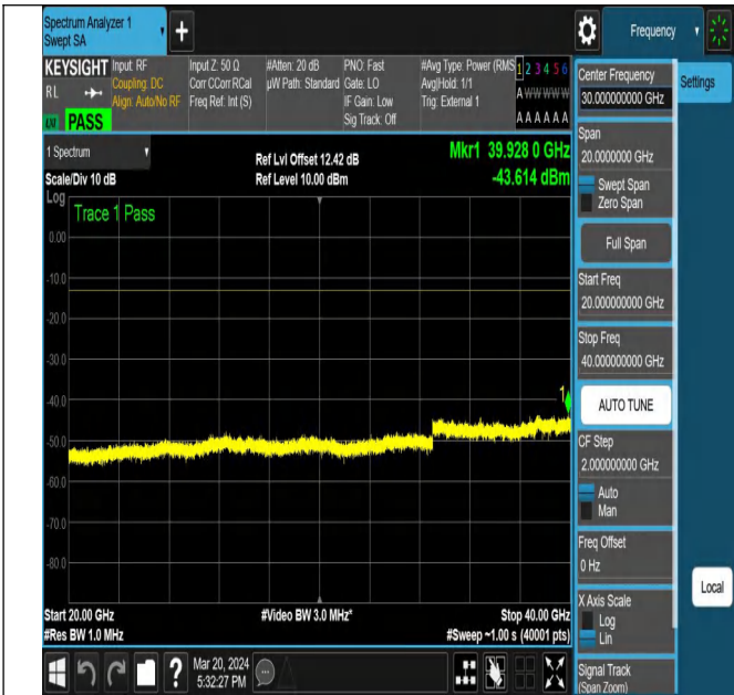
NTNV-N77-3450-3550-PC2-30-10-H-DFT-QPSK-Edge_1RB_ Left-Ant1-PASS
