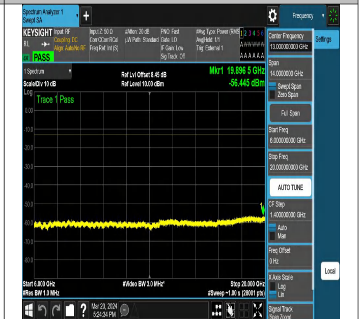
NTNV-N77-3450-3550-PC2-30-10-M-DFT-QPSK-Edge_1RB_ Left-Ant1-PASS
