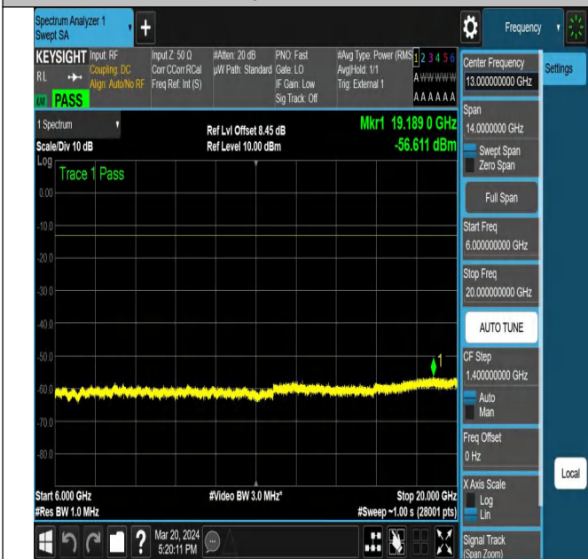
NTNV-N77-3450-3550-PC2-30-10-L-DFT-QPSK-Edge_1RB_
