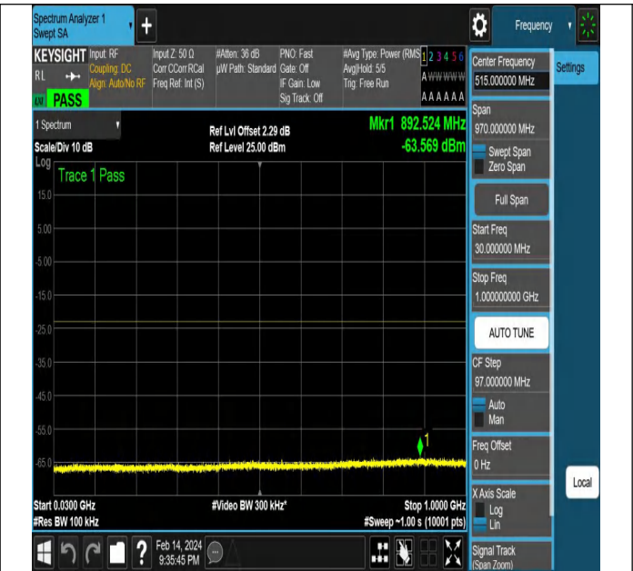
NTNV-N77-3450-3550-PC2-30-10-H-DFT-PI2BPSK-Edge_1R B_Right-Ant1-PASS
