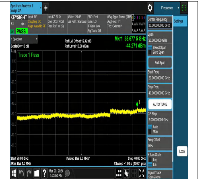
NTNV-N77-3450-3550-PC2-30-10-M-DFT-PI2BPSK-Edge_1R B_Right-Ant1-PASS
