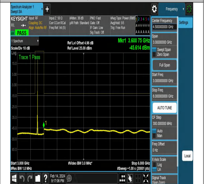
NTNV-N77-3450-3550-PC2-30-10-L-DFT-PI2BPSK-Edge_1R B_Right-Ant1-PASS
