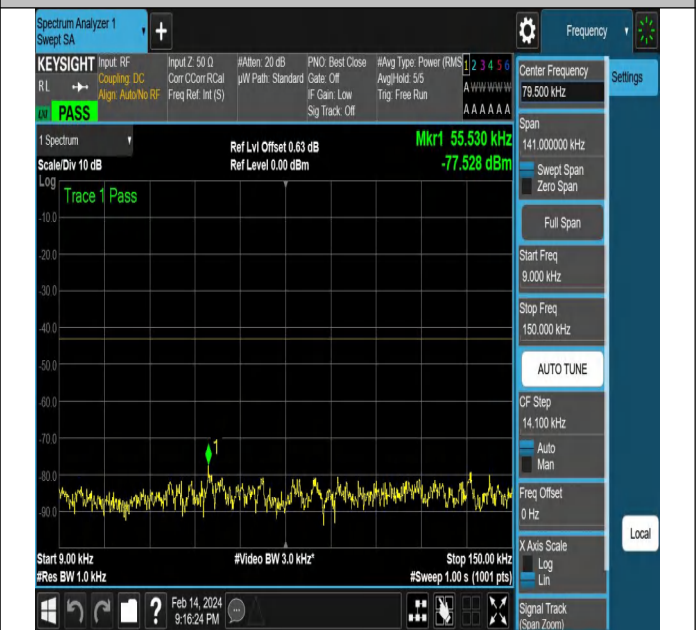
NTNV-N77-3450-3550-PC2-30-10-L-DFT-PI2BPSK-Edge_1R B_Right-Ant1-PASS
