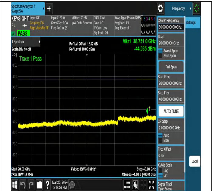
NTNV-N77-3450-3550-PC2-30-10-L-DFT-PI2BPSK-Edge_1R B_Right-Ant1-PASS
