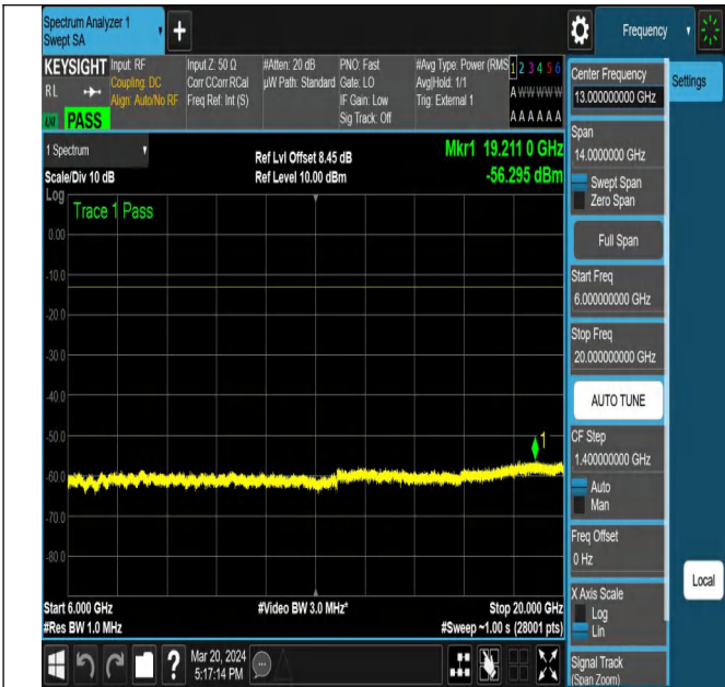
NTNV-N77-3450-3550-PC2-30-10-L-DFT-PI2BPSK-Edge_1R B_Right-Ant1-PASS
