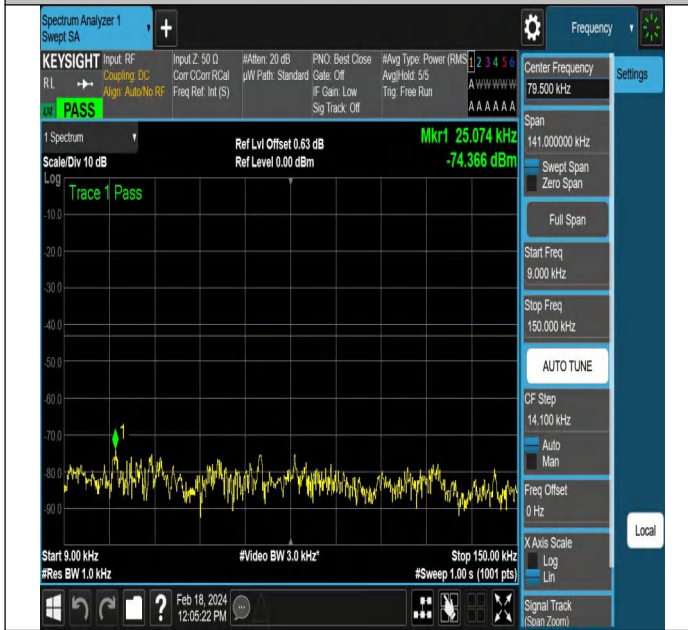
NTNV-DC_5A_n66A-PC3-15-5+40-M+L-QPSK-DFT-PI2BPSK -Edge_1RB_Right-PASS
