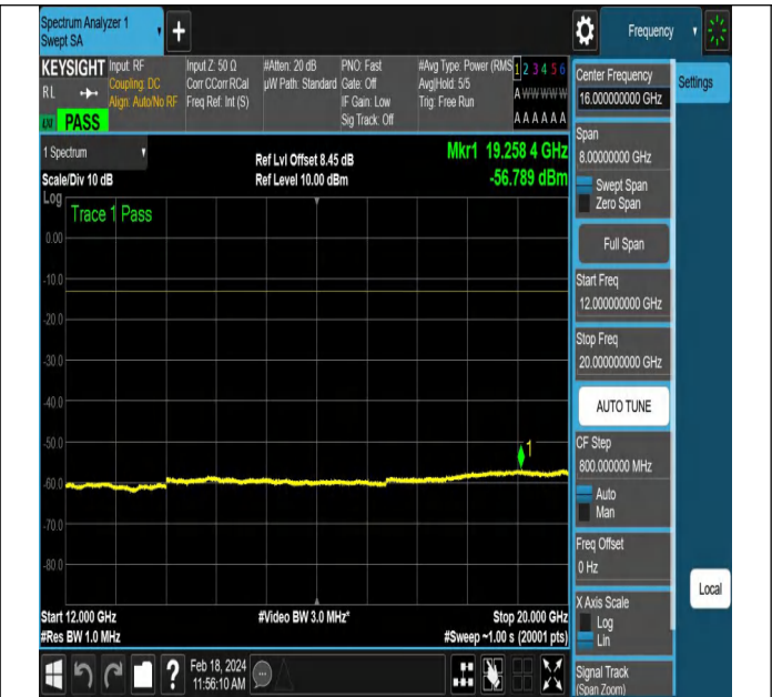
NTNV-DC_5A_n66A-PC3-15-5+20-M+H-QPSK-DFT-QPSK-E dge_1RB_Left-PASS
