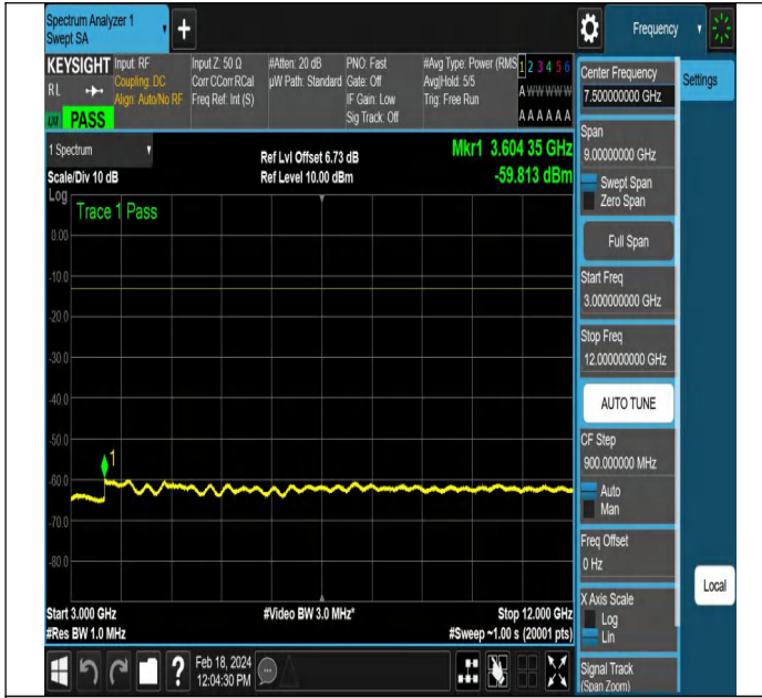
NTNV-DC_5A_n66A-PC3-15-5+40-M+L-QPSK-DFT-PI2BPSK -Edge_1RB_Left-PASS
