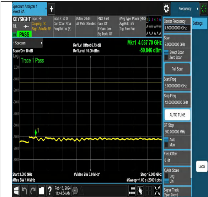
NTNV-DC_5A_n66A-PC3-15-5+20-M+M-QPSK-DFT-QPSK-E dge_1RB_Left-PASS
