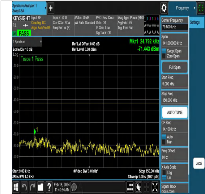
NTNV-DC_5A_n66A-PC3-15-5+20-M+M-QPSK-DFT-PI2BPS K-Edge_1RB_Left-PASS
