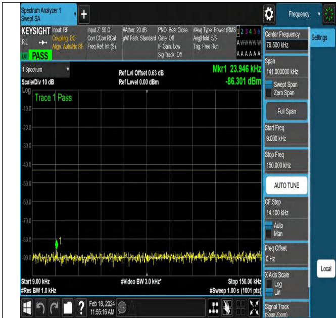
NTNV-DC_5A_n66A-PC3-15-5+20-M+H-QPSK-DFT-QPSK-E dge_1RB_Left-PASS
