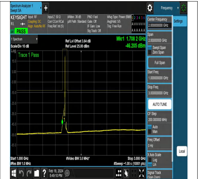
NTNV-DC_5A_n66A-PC3-15-5+40-M+L-QPSK-DFT-PI2BPSK -Edge_1RB_Right-PASS
