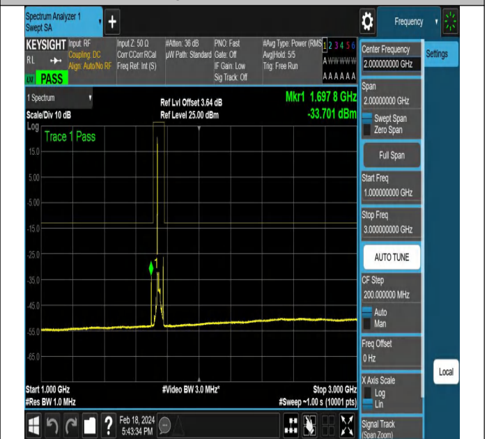
NTNV-DC_5A_n66A-PC3-15-5+20-M+M-QPSK-DFT-QPSK-E dge_1RB_Left-PASS
