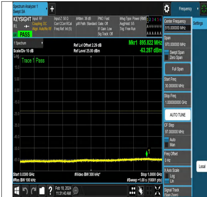
NTNV-DC_5A_n66A-PC3-15-5+20-M+L-QPSK-DFT-PI2BPSK -Edge_1RB_Right-PASS
