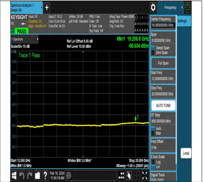
NTNV-DC_5A_n66A-PC3-15-5+20-M+L-QPSK-DFT-QPSK-Ed ge_1RB_Left-PASS
