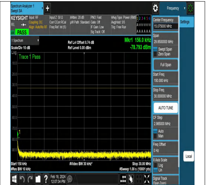
NTNV-DC_5A_n66A-PC3-15-5+40-M+L-QPSK-DFT-QPSK-Ed ge_1RB_Left-PASS
