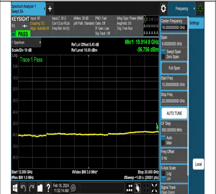
NTNV-DC_5A_n66A-PC3-15-5+20-M+L-QPSK-DFT-PI2BPSK -Edge_1RB_Right-PASS
