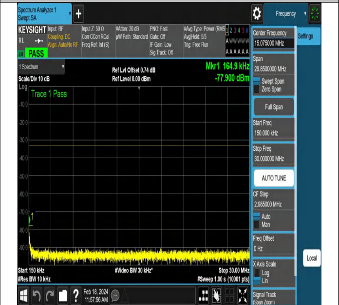
NTNV-DC_5A_n66A-PC3-15-5+20-M+H-QPSK-DFT-QPSK-E dge_1RB_Right-PASS
