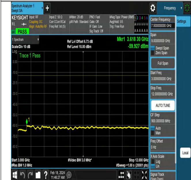
NTNV-DC_5A_n66A-PC3-15-5+20-M+M-QPSK-DFT-QPSK-E dge_1RB_Right-PASS
