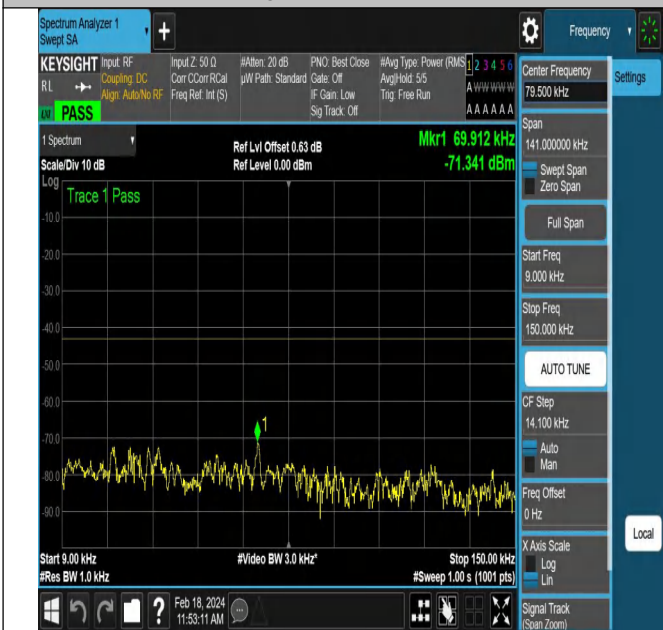
NTNV-DC_5A_n66A-PC3-15-5+20-M+H-QPSK-DFT-PI2BPSK -Edge_1RB_Right-PASS
