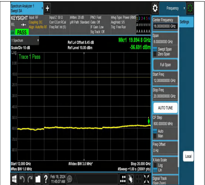
NTNV-DC_5A_n66A-PC3-15-5+20-M+M-QPSK-DFT-QPSK-E dge_1RB_Left-PASS
