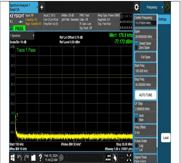
NTNV-DC_5A_n66A-PC3-15-5+20-M+M-QPSK-DFT-QPSK-E dge_1RB_Left-PASS
