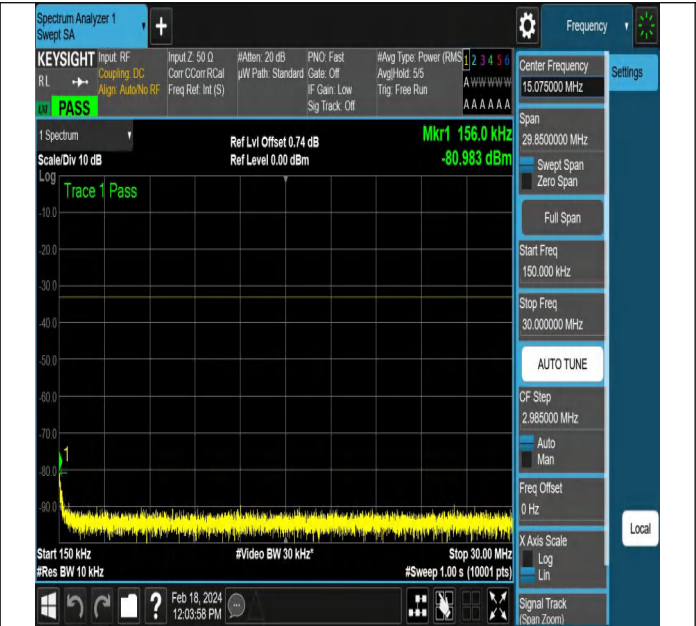
NTNV-DC_5A_n66A-PC3-15-5+40-M+L-QPSK-DFT-PI2BPSK -Edge_1RB_Left-PASS
