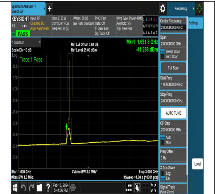
NTNV-DC_5A_n66A-PC3-15-5+20-M+L-QPSK-DFT-QPSK-Ed ge_1RB_Right-PASS
