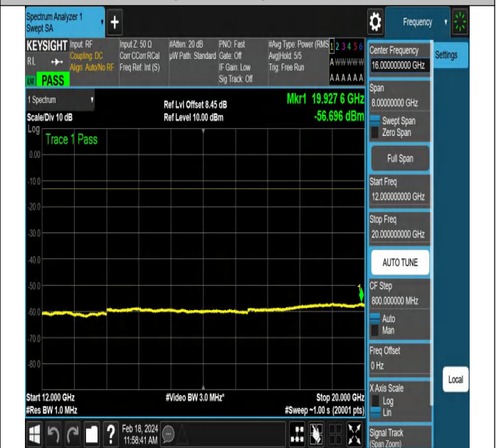
NTNV-DC_5A_n66A-PC3-15-5+20-M+H-QPSK-DFT-QPSK-E dge_1RB_Right-PASS
