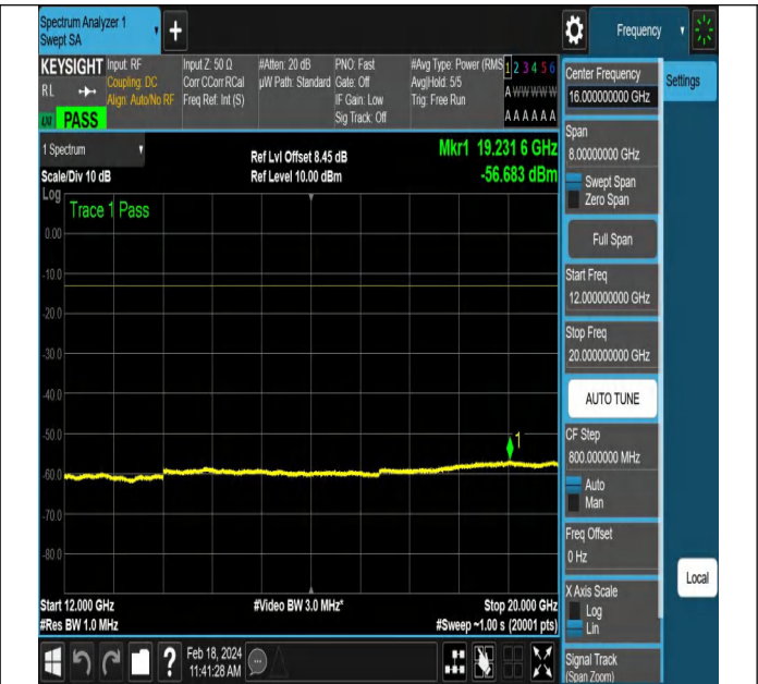
NTNV-DC_5A_n66A-PC3-15-5+20-M+M-QPSK-DFT-PI2BPS K-Edge_1RB_Left-PASS
