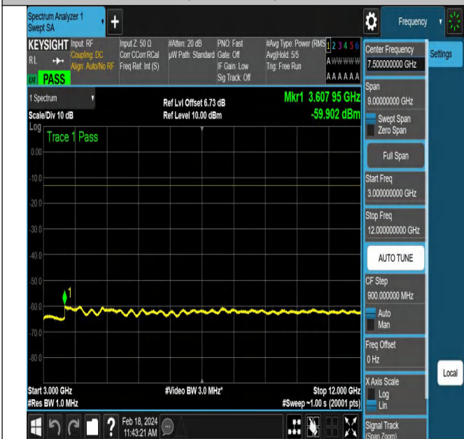
NTNV-DC_5A_n66A-PC3-15-5+20-M+M-QPSK-DFT-PI2BPS
