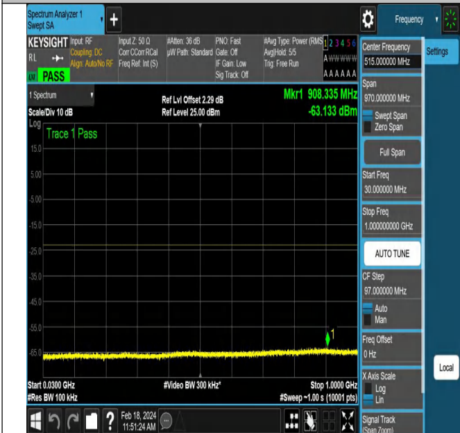
NTNV-DC_5A_n66A-PC3-15-5+20-M+H-QPSK-DFT-PI2BPSK -Edge_1RB_Left-PASS
