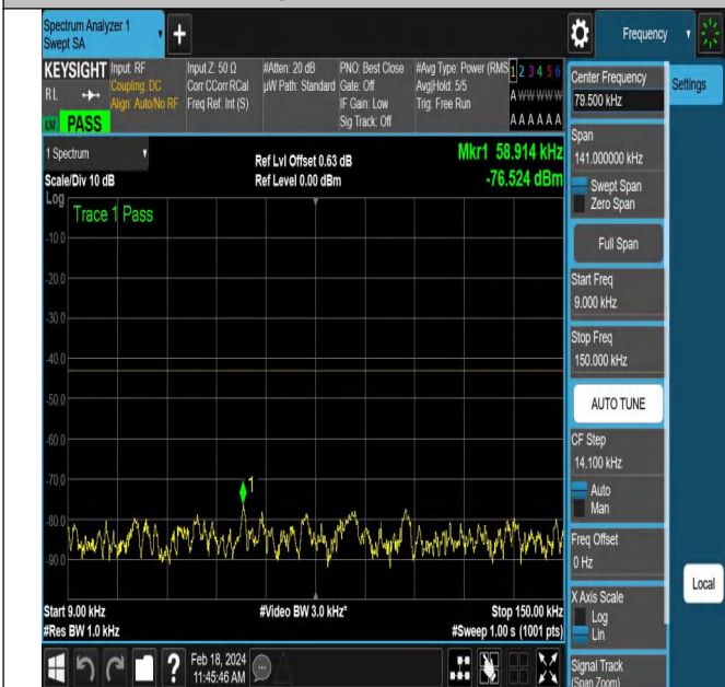
NTNV-DC_5A_n66A-PC3-15-5+20-M+M-QPSK-DFT-QPSK-E dge_1RB_Right-PASS
