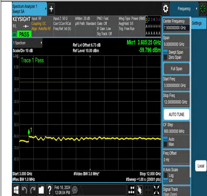
NTNV-DC_5A_n66A-PC3-15-5+40-M+L-QPSK-DFT-PI2BPSK -Edge_1RB_Right-PASS
