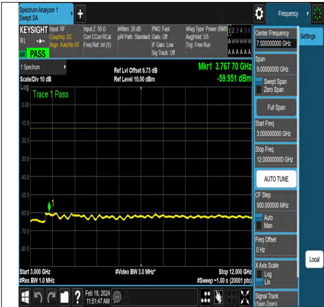
NTNV-DC_5A_n66A-PC3-15-5+20-M+H-QPSK-DFT-PI2BPSK -Edge_1RB_Left-PASS
