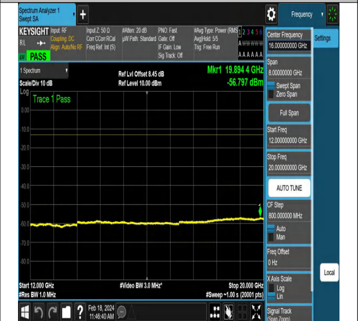
NTNV-DC_5A_n66A-PC3-15-5+20-M+M-QPSK-DFT-QPSK-E dge_1RB_Right-PASS
