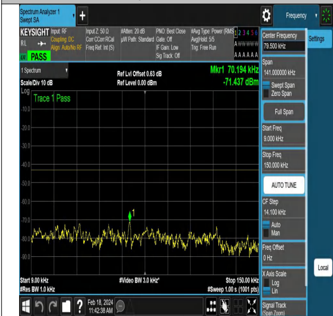
NTNV-DC_5A_n66A-PC3-15-5+20-M+M-QPSK-DFT-PI2BPS K-Edge_1RB_Right-PASS
