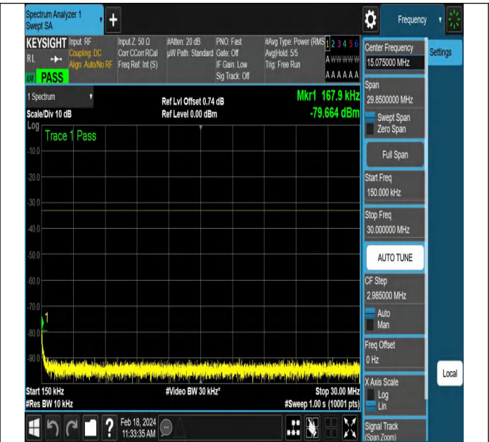
NTNV-DC_5A_n66A-PC3-15-5+20-M+L-QPSK-DFT-QPSK-Ed ge_1RB_Left-PASS
