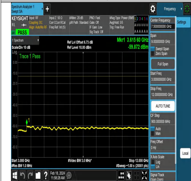
NTNV-DC_5A_n66A-PC3-15-5+20-M+H-QPSK-DFT-QPSK-E dge_1RB_Right-PASS
