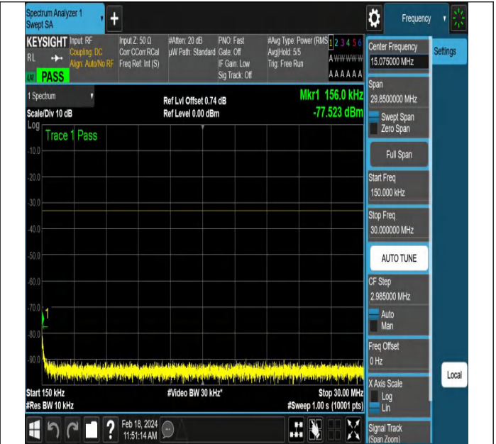
NTNV-DC_5A_n66A-PC3-15-5+20-M+H-QPSK-DFT-PI2BPSK -Edge_1RB_Left-PASS
