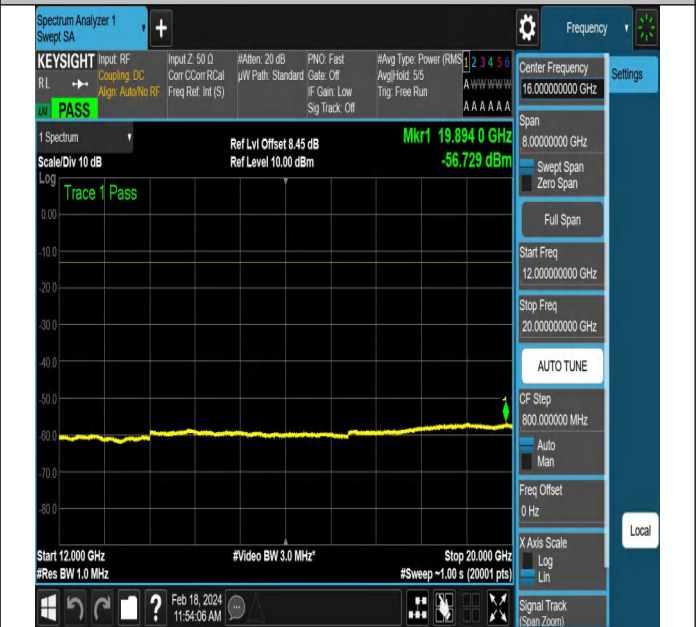
NTNV-DC_5A_n66A-PC3-15-5+20-M+H-QPSK-DFT-PI2BPSK -Edge_1RB_Right-PASS
