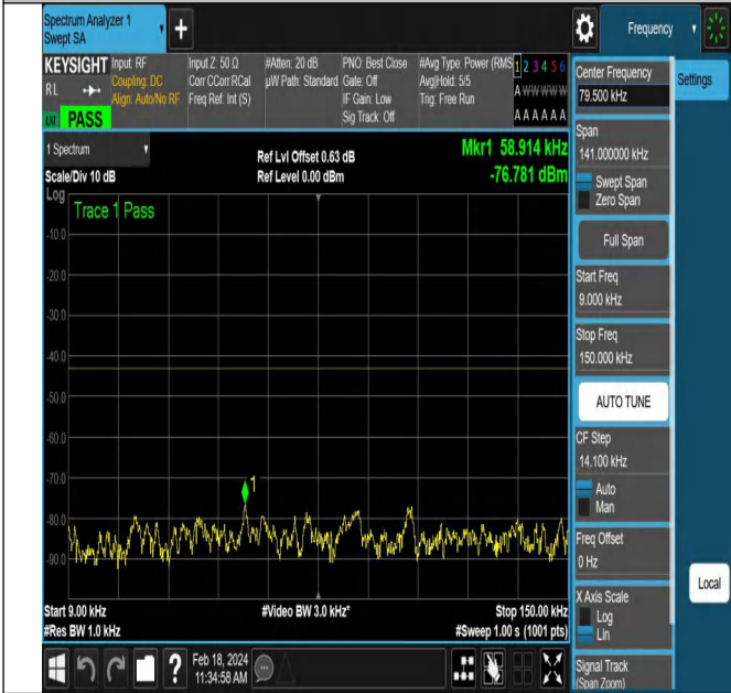
NTNV-DC_5A_n66A-PC3-15-5+20-M+L-QPSK-DFT-QPSK-Ed ge_1RB_Right-PASS
