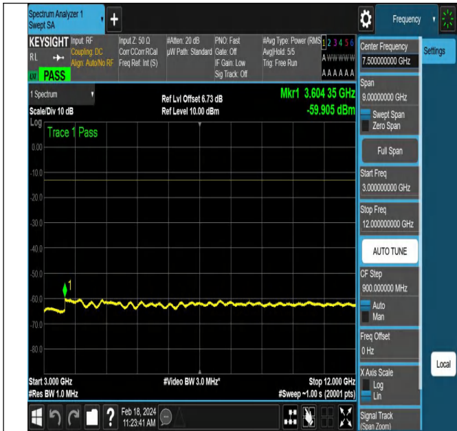
NTNV-DC_5A_n66A-PC3-15-5+15-M+H-QPSK-DFT-QPSK-E dge_1RB_Left-PASS
