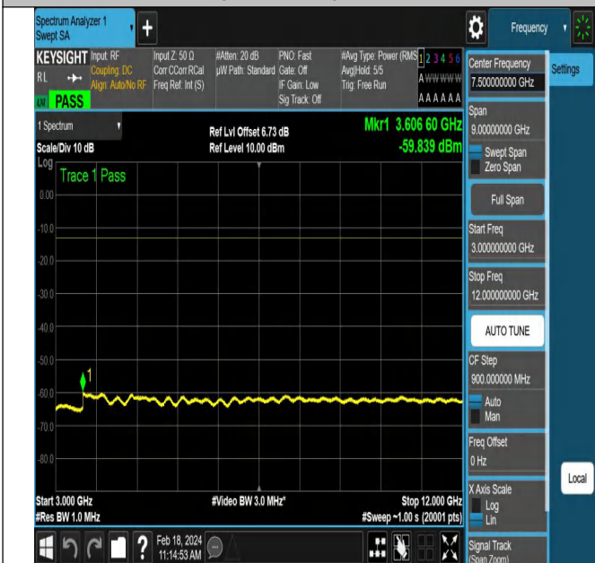
NTNV-DC_5A_n66A-PC3-15-5+15-M+M-QPSK-DFT-QPSK-E dge_1RB_Right-PASS
