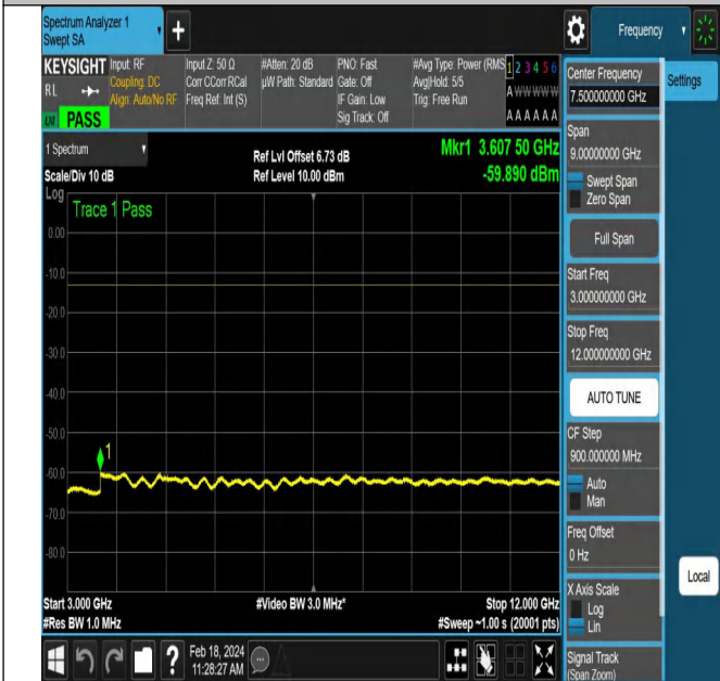
NTNV-DC_5A_n66A-PC3-15-5+15-M+H-QPSK-CP-QPSK-Ed ge_1RB_Right-PASS
