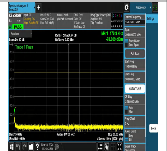
NTNV-DC_5A_n66A-PC3-15-5+15-M+H-QPSK-DFT-QPSK-E dge_1RB_Right-PASS
