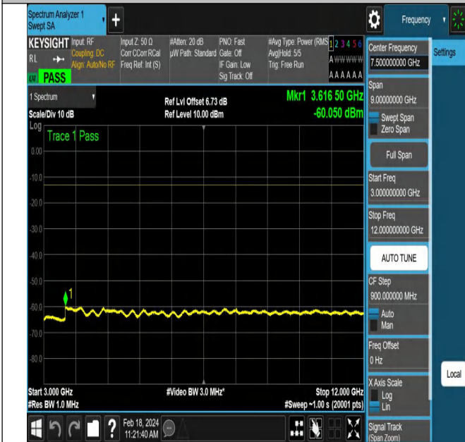
NTNV-DC_5A_n66A-PC3-15-5+15-M+H-QPSK-DFT-PI2BPSK -Edge_1RB_Right-PASS
