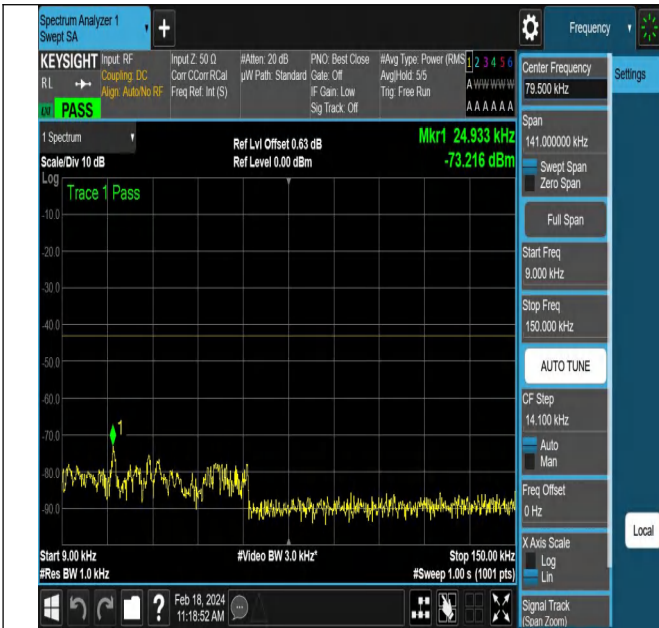
NTNV-DC_5A_n66A-PC3-15-5+15-M+H-QPSK-DFT-PI2BPSK -Edge_1RB_Left-PASS
