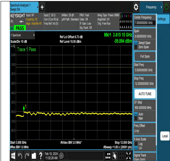
NTNV-DC_5A_n66A-PC3-15-5+15-M+L-QPSK-DFT-QPSK-Ed ge_1RB_Left-PASS
