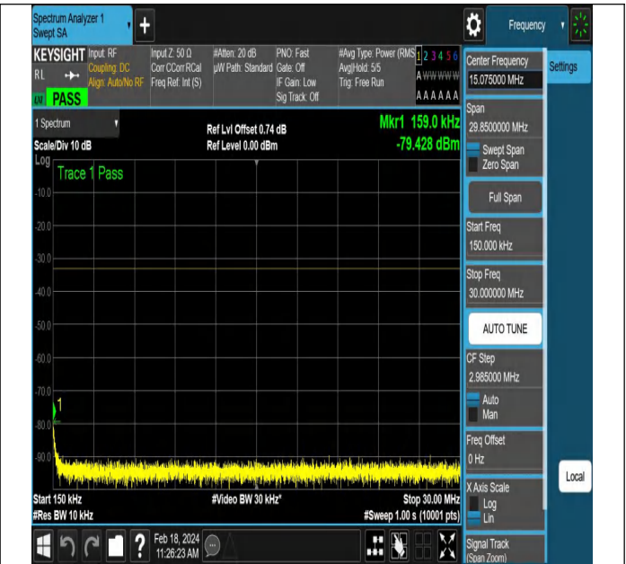
NTNV-DC_5A_n66A-PC3-15-5+15-M+H-QPSK-CP-QPSK-Ed ge_1RB_Left-PASS
