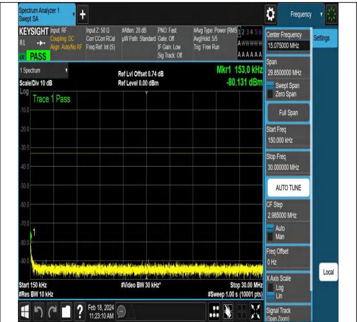
NTNV-DC_5A_n66A-PC3-15-5+15-M+H-QPSK-DFT-QPSK-E dge_1RB_Left-PASS
