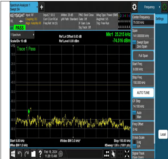
NTNV-DC_5A_n66A-PC3-15-5+15-M+H-QPSK-CP-QPSK-Ed ge_1RB_Left-PASS
