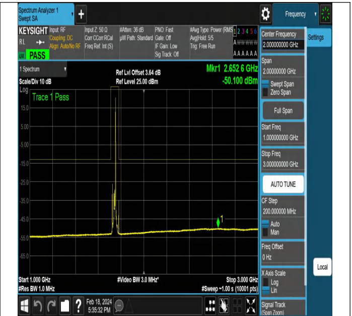
NTNV-DC_5A_n66A-PC3-15-5+15-M+M-QPSK-DFT-QPSK-E dge_1RB_Right-PASS
