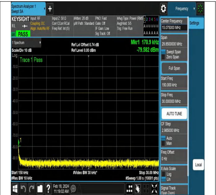
NTNV-DC_5A_n66A-PC3-15-5+15-M+H-QPSK-DFT-PI2BPSK -Edge_1RB_Left-PASS
