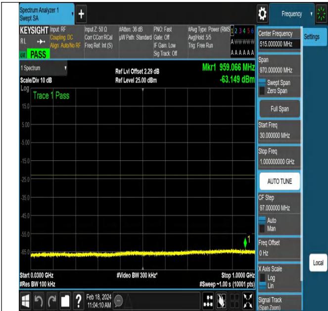
NTNV-DC_5A_n66A-PC3-15-5+15-M+L-QPSK-DFT-QPSK-Ed ge_1RB_Right-PASS
