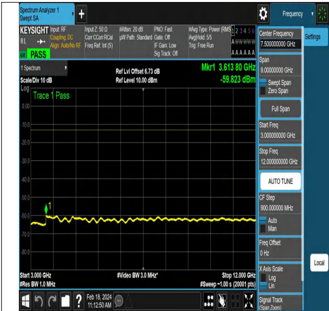
NTNV-DC_5A_n66A-PC3-15-5+15-M+M-QPSK-DFT-QPSK-E dge_1RB_Left-PASS
