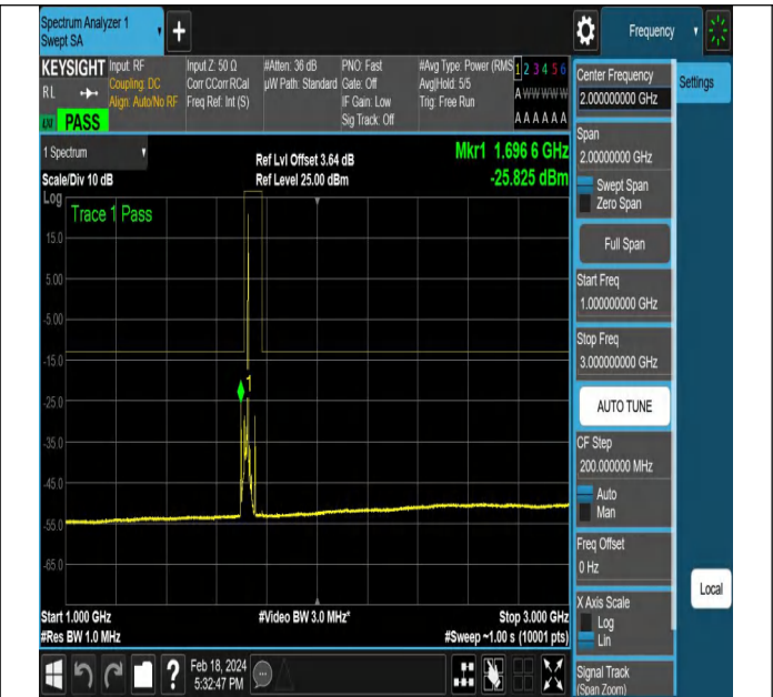
NTNV-DC_5A_n66A-PC3-15-5+15-M+L-QPSK-DFT-QPSK-Ed ge_1RB_Right-PASS
