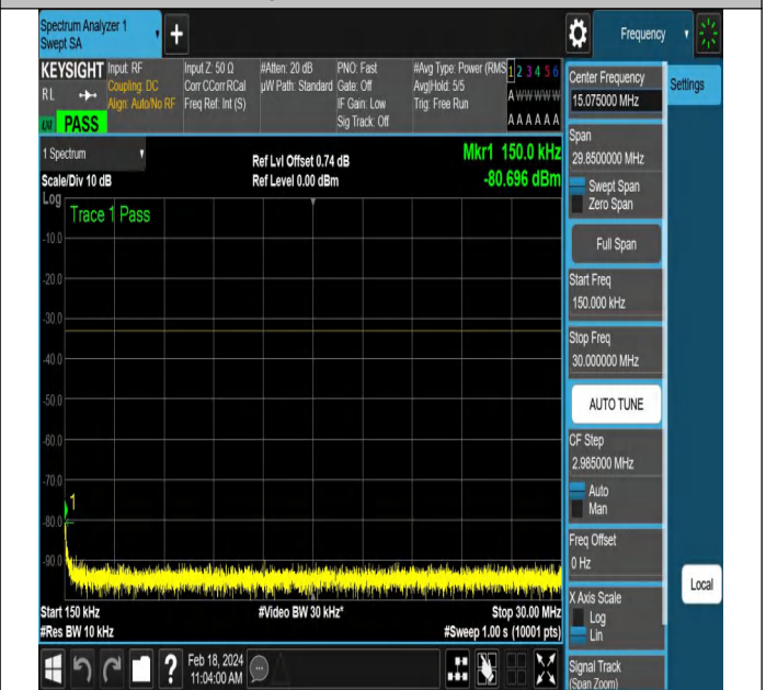
NTNV-DC_5A_n66A-PC3-15-5+15-M+L-QPSK-DFT-QPSK-Ed ge_1RB_Right-PASS
