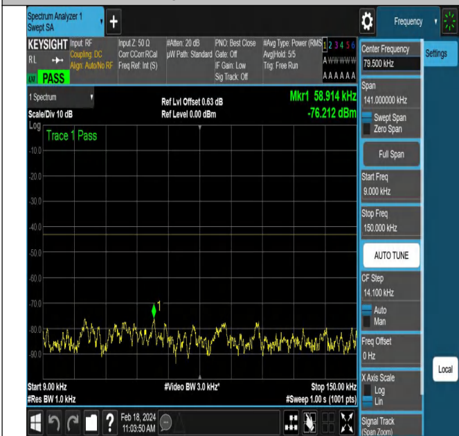
NTNV-DC_5A_n66A-PC3-15-5+15-M+L-QPSK-DFT-QPSK-Ed ge_1RB_Right-PASS
