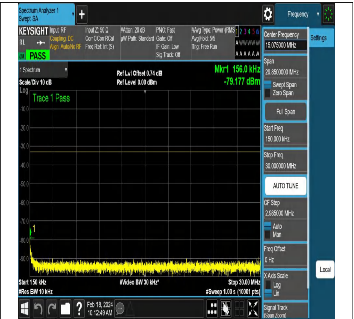
NTNV-DC_5A_n66A-PC3-15-5+5-M+M-QPSK-CP-QPSK-Edge e_1RB_Left-PASS
