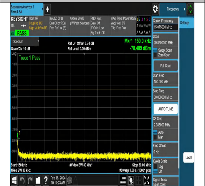
NTNV-DC_5A_n66A-PC3-15-5+5-M+M-QPSK-CP-QPSK-Edge e_1RB_Right-PASS
