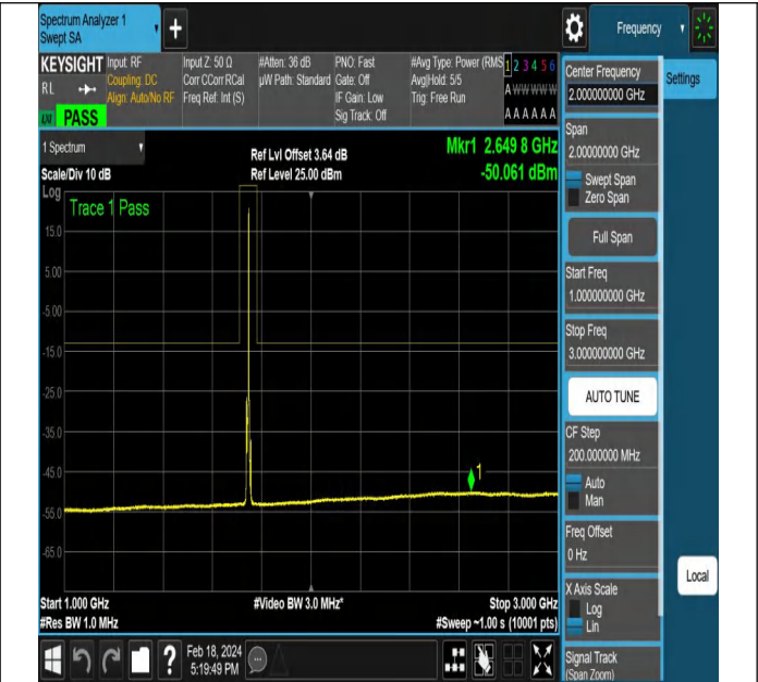
NTNV-DC_5A_n66A-PC3-15-5+5-M+M-QPSK-CP-QPSK-Edg e_1RB_Right-PASS
