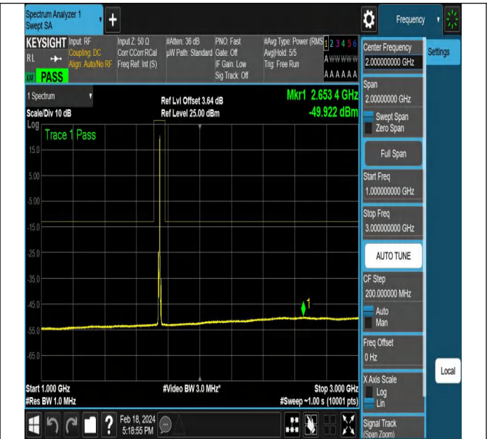
NTNV-DC_5A_n66A-PC3-15-5+5-M+M-QPSK-DFT-QPSK-Ed ge_1RB_Right-PASS
