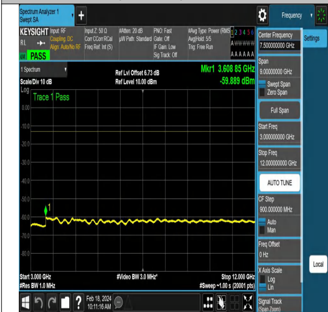
NTNV-DC_5A_n66A-PC3-15-5+5-M+M-QPSK-DFT-QPSK-Ed ge_1RB_Right-PASS
