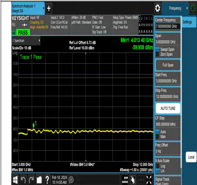
NTNV-DC_5A_n66A-PC3-15-5+5-M+M-QPSK-CP-QPSK-Edg e_1RB_Right-PASS
