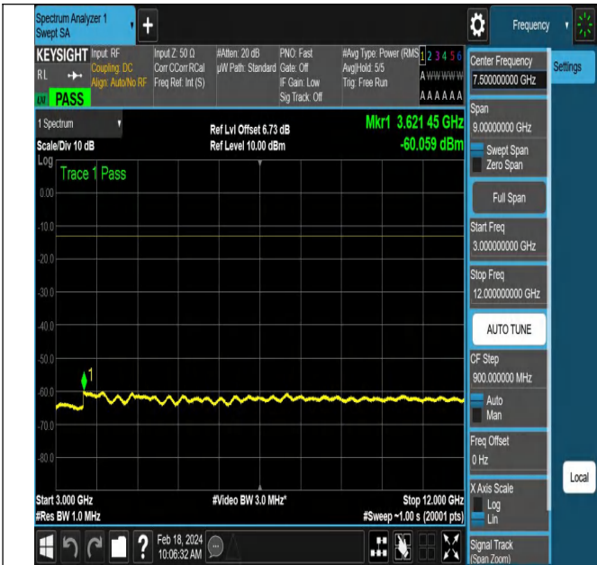
NTNV-DC_5A_n66A-PC3-15-5+5-M+M-QPSK-DFT-PI2BPSK- Edge_1RB_Left-PASS
