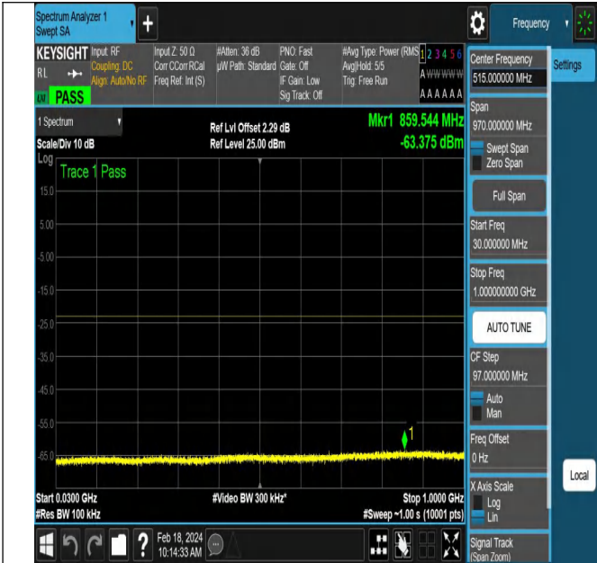
NTNV-DC_5A_n66A-PC3-15-5+5-M+M-QPSK-CP-QPSK-Edg e_1RB_Right-PASS
