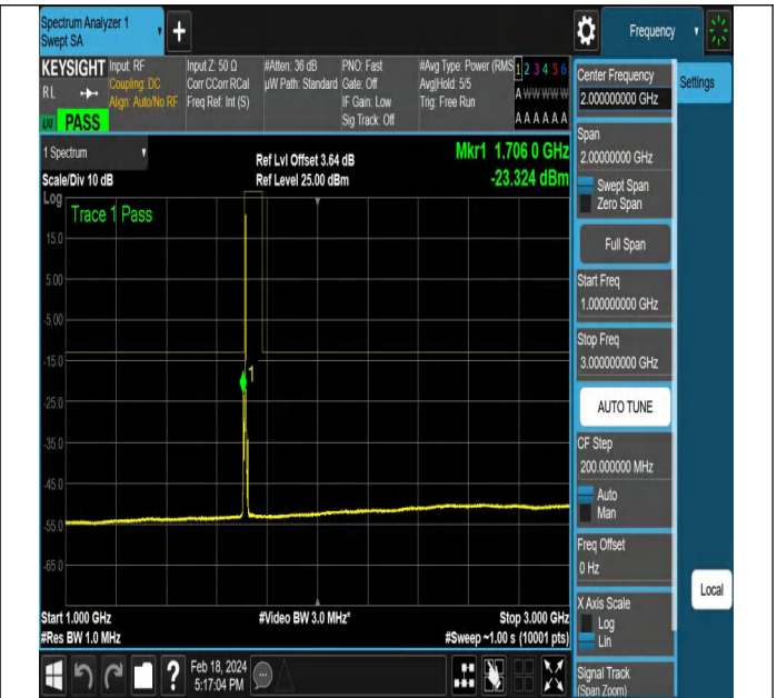
NTNV-DC_5A_n66A-PC3-15-5+5-M+L-QPSK-CP-QPSK-Edge_e_1RB_Right-PASS
