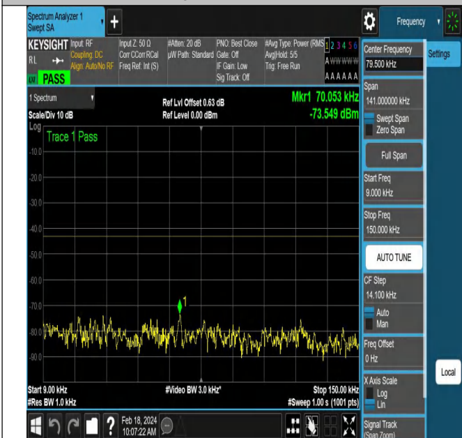
NTNV-DC_5A_n66A-PC3-15-5+5-M+M-QPSK-DFT-PI2BPSK- Edge_1RB_Right-PASS
