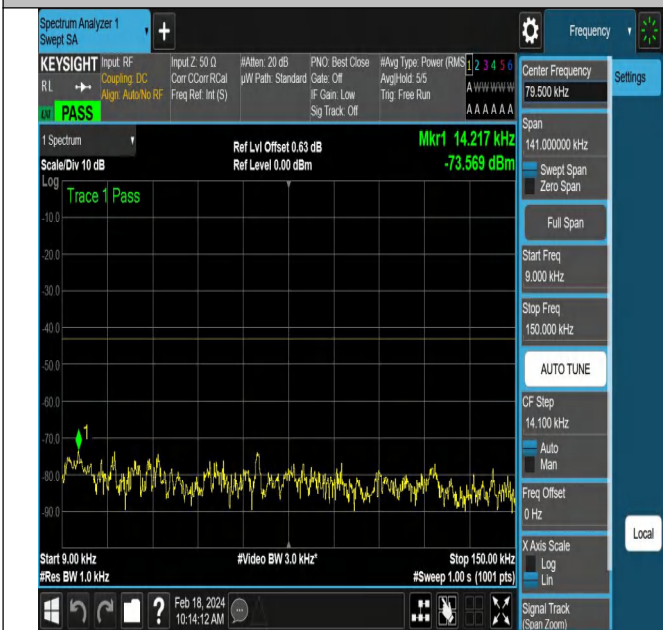
NTNV-DC_5A_n66A-PC3-15-5+5-M+M-QPSK-CP-QPSK-Edge e_1RB_Right-PASS
