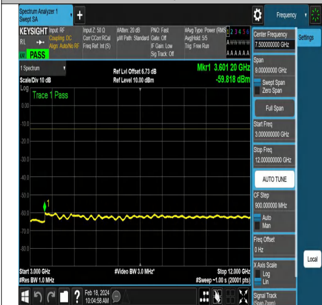
NTNV-DC_5A_n66A-PC3-15-5+5-M+L-QPSK-CP-QPSK-Edge_e_1RB_Right-PASS
