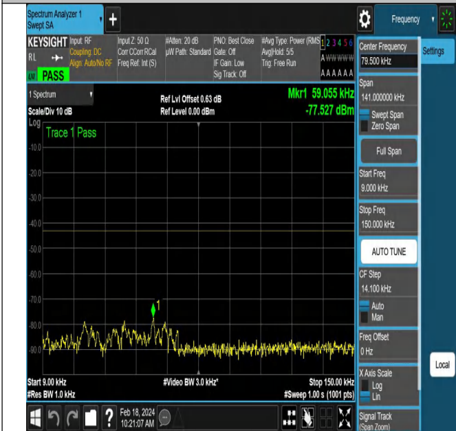
NTNV-DC_5A_n66A-PC3-15-5+5-M+H-QPSK-DFT-QPSK-Ed ge_1RB_Right-PASS
