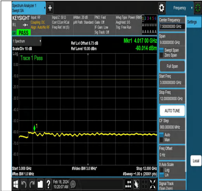
NTNV-DC_5A_n66A-PC3-15-5+5-M+H-QPSK-DFT-QPSK-Ed ge_1RB_Left-PASS
