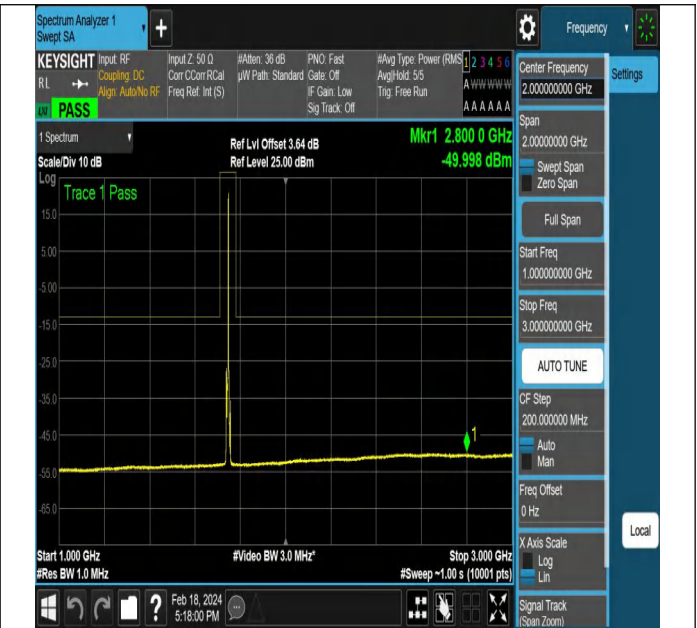
NTNV-DC_5A_n66A-PC3-15-5+5-M+M-QPSK-DFT-PI2BPSK-Edge_1RB_Right-PASS
