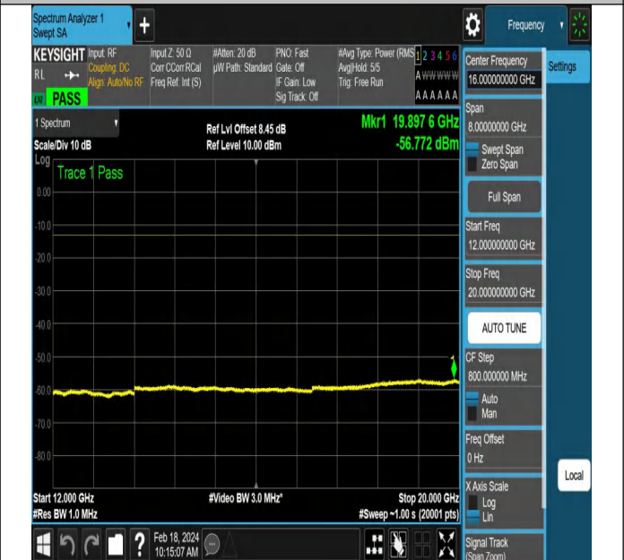
NTNV-DC_5A_n66A-PC3-15-5+5-M+M-QPSK-CP-QPSK-Edg e_1RB_Right-PASS
