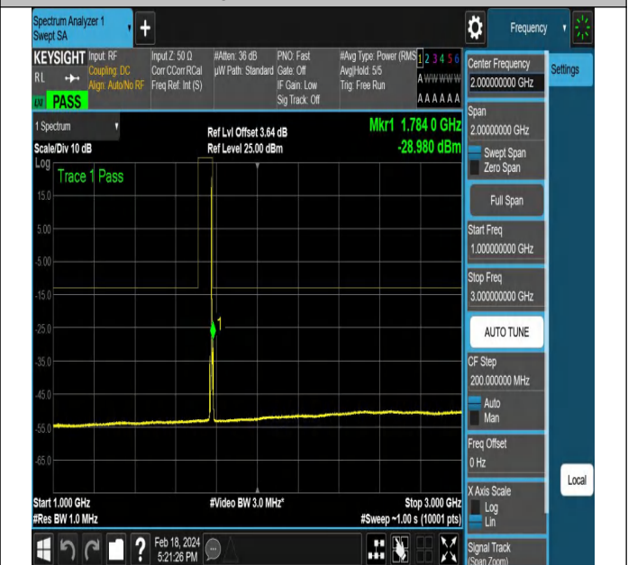
NTNV-DC_5A_n66A-PC3-15-5+5-M+H-QPSK-DFT-QPSK-Edge_1RB_Left-PASS
