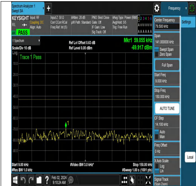
NTNV-N66-PC3-15-20-H-DFT-QPSK-Edge_1RB_Left-Ant1-P
