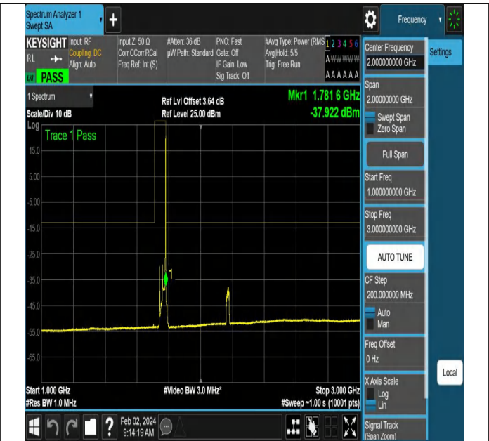
NTNV-N66-PC3-15-20-H-CP-QPSK-Edge_1RB_Right-Ant1-P
