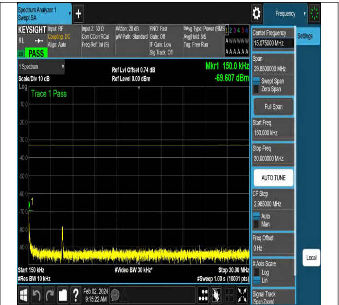
NTNV-N66-PC3-15-40-L-DFT-PI2BPSK-Edge_1RB_Left-Ant1- PASS
