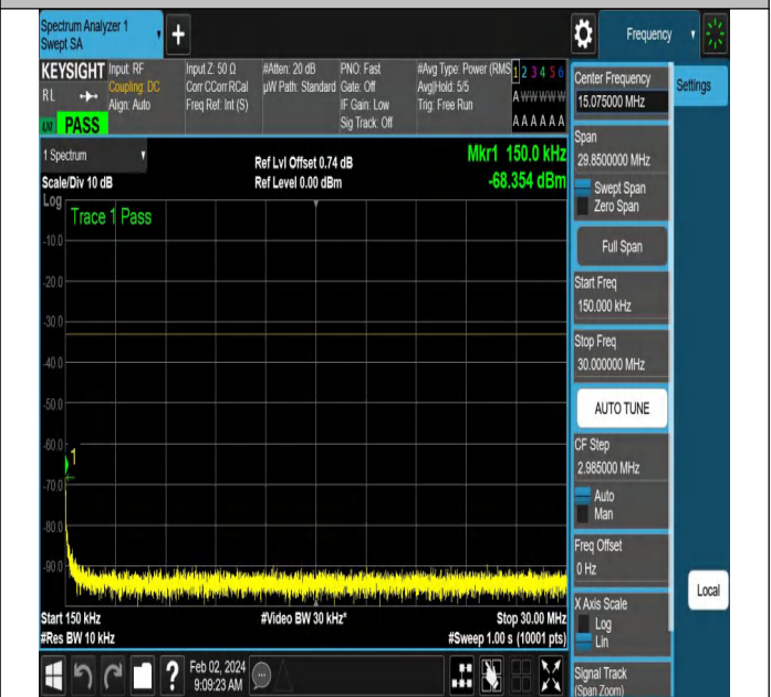
NTNV-N66-PC3-15-20-H-DFT-PI2BPSK-Edge_1RB_Right-Ant 1-PASS
