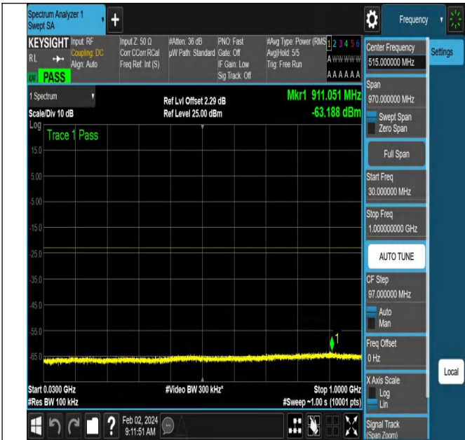
NTNV-N66-PC3-15-20-H-DFT-QPSK-Edge_1RB_Right-Ant1-
