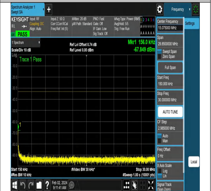
NTNV-N66-PC3-15-20-H-DFT-QPSK-Edge_1RB_Right-Ant1-P PASS
