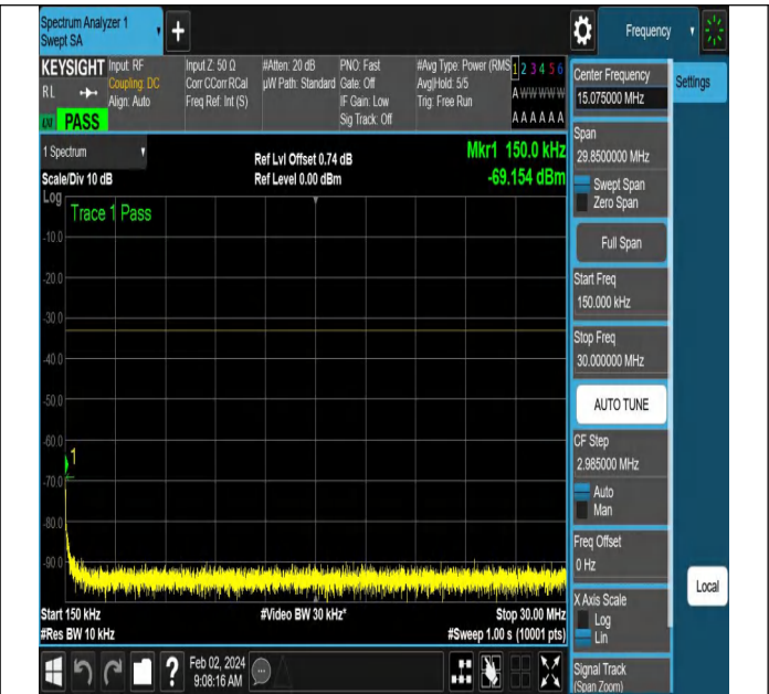
NTNV-N66-PC3-15-20-H-DFT-PI2BPSK-Edge_1RB_Left-Ant1
