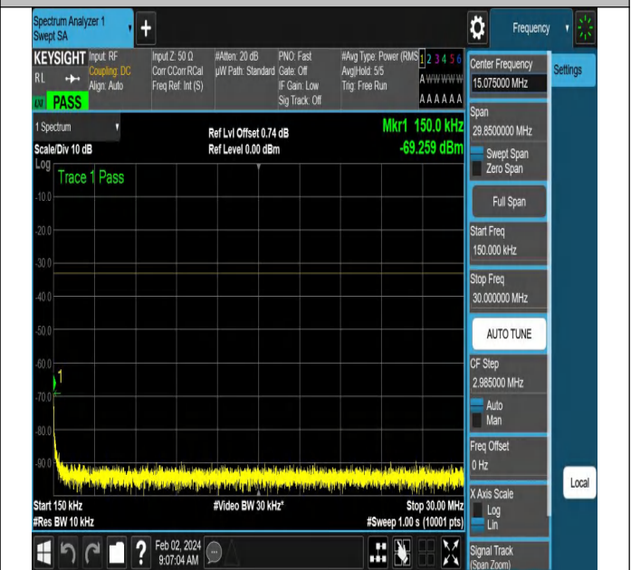
NTNV-N66-PC3-15-20-M-CP-QPSK-Edge_1RB_Right-Ant1-P
