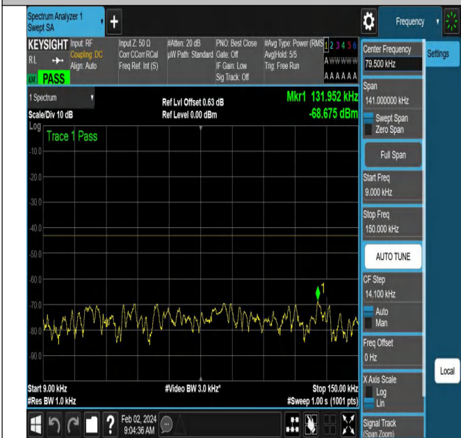
NTNV-N66-PC3-15-20-M-DFT-QPSK-Edge_1RB_Right-Ant1-P
