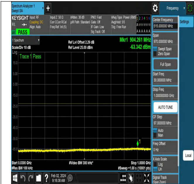
NTNV-N66-PC3-15-40-L-DFT-PI2BPSK-Edge_1RB_Right-Ant
