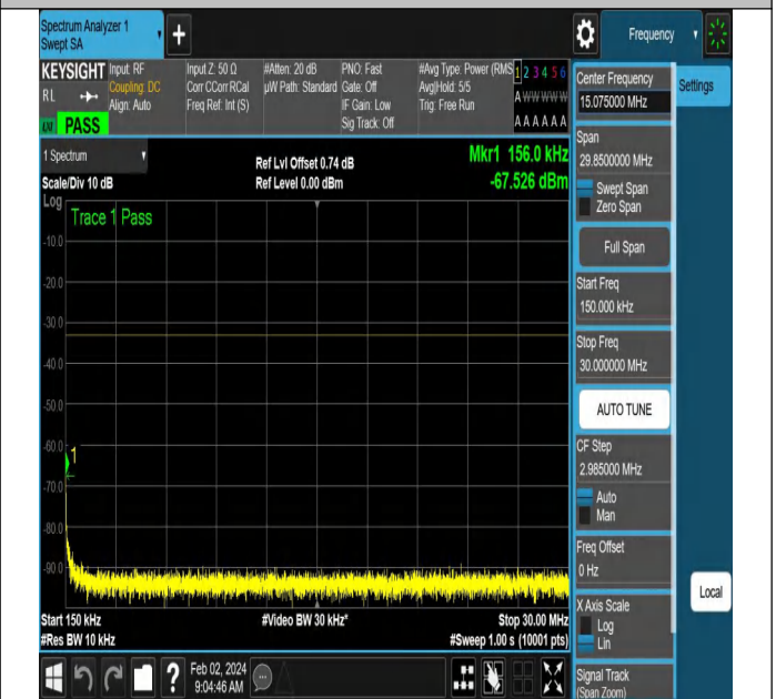
NTNV-N66-PC3-15-20-M-DFT-QPSK-Edge_1RB_Right-Ant1-P
