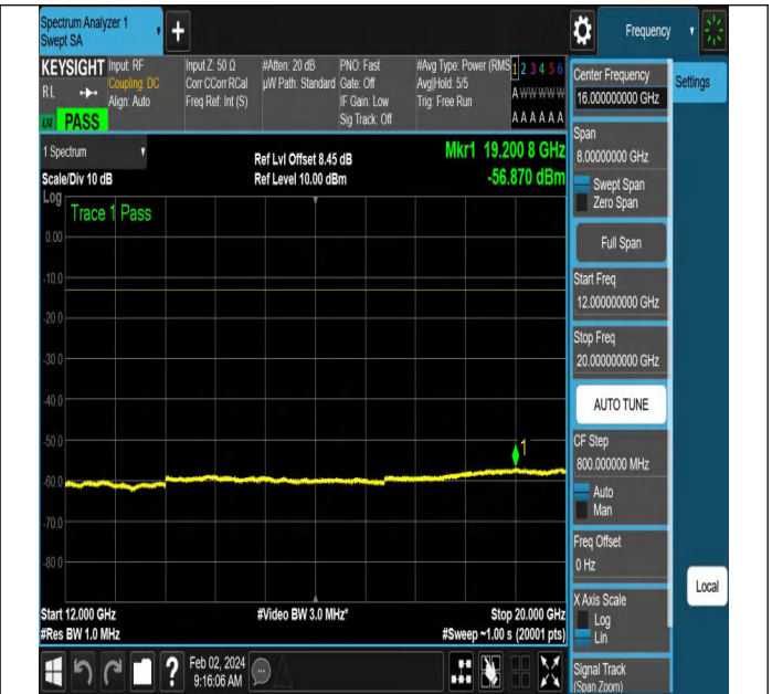
NTNV-N66-PC3-15-40-L-DFT-PI2BPSK-Edge_1RB_Left-Ant1-1 PASS
