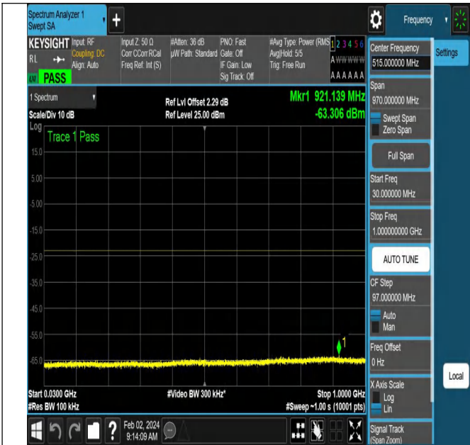
NTNV-N66-PC3-15-20-H-CP-QPSK-Edge_1RB_Right-Ant1-P
