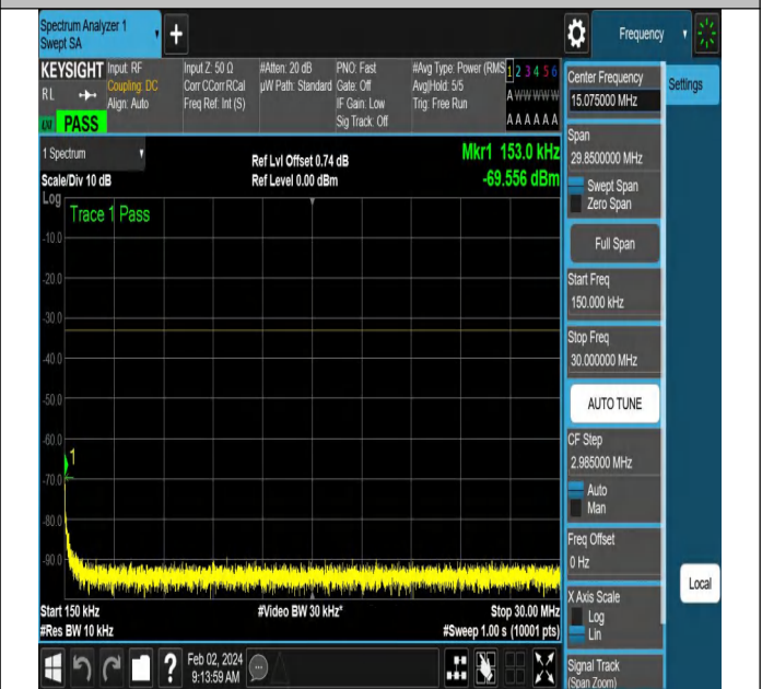
NTNV-N66-PC3-15-20-H-CP-QPSK-Edge_1RB_Right-Ant1-P
