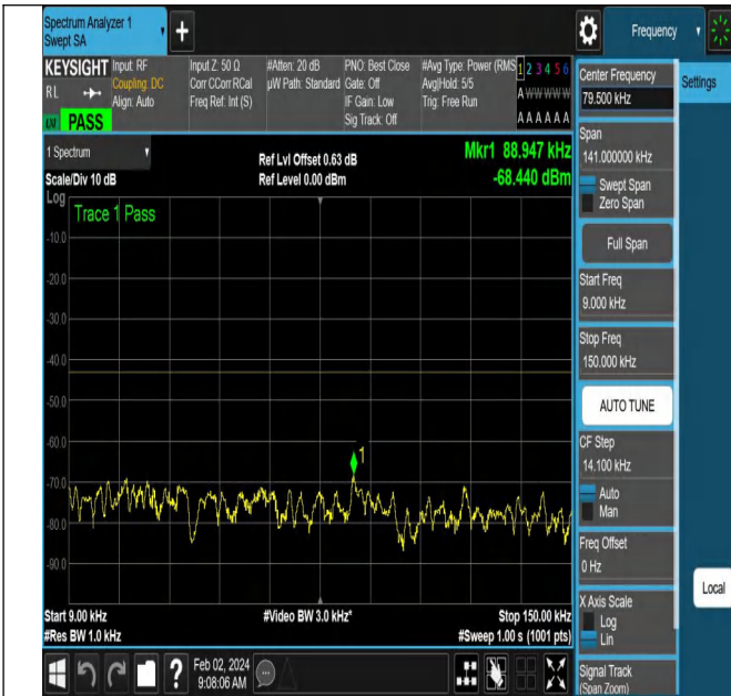
NTNV-N66-PC3-15-20-H-DFT-PI2BPSK-Edge_1RB_Left-Ant1
