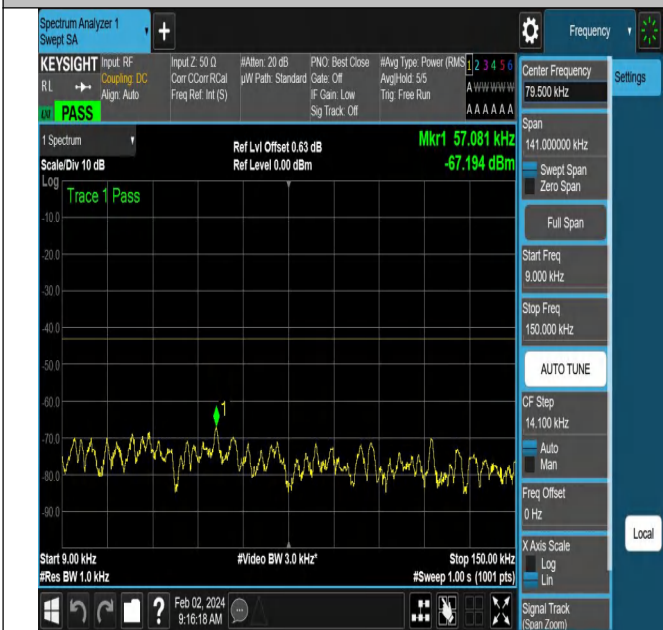
NTNV-N66-PC3-15-40-L-DFT-PI2BPSK-Edge_1RB_Right-Ant 1 1-PASS
