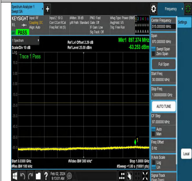
NTNV-N66-PC3-15-20-H-CP-QPSK-Edge_1RB_Left-Ant1-PA
