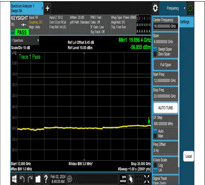
NTNV-N66-PC3-15-15-H-DFT-QPSK-Edge_1RB_Left-Ant1-P ASS
