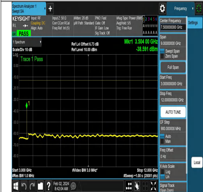
NTNV-N66-PC3-15-15-M-DFT-QPSK-Edge_1RB_Right-Ant1-
