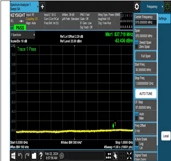
NTNV-N66-PC3-15-20-L-DFT-QPSK-Edge_1RB_Right-Ant1-P
