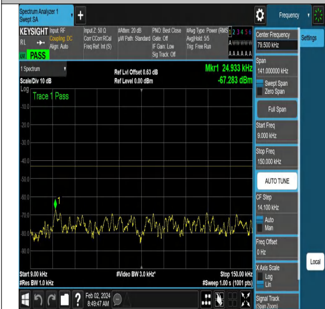
NTNV-N66-PC3-15-15-H-DFT-QPSK-Edge_1RB_Right-Ant1-P PASS
