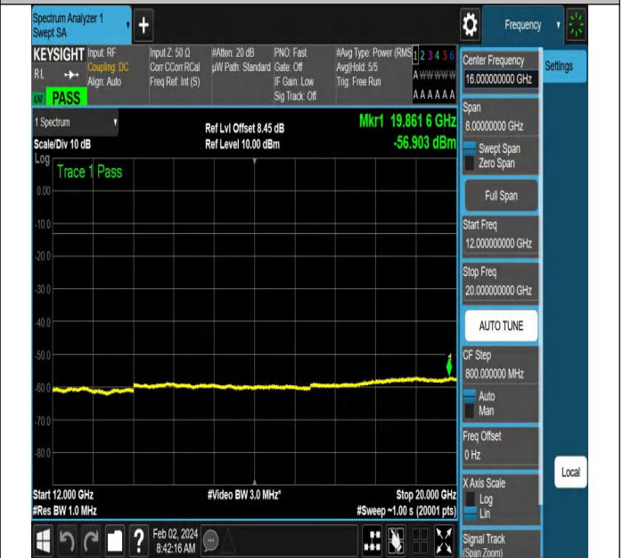
NTNV-N66-PC3-15-15-M-DFT-QPSK-Edge_1RB_Right-Ant1-
