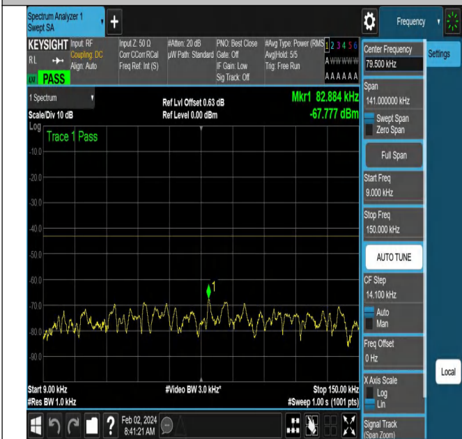
NTNV-N66-PC3-15-15-M-DFT-QPSK-Edge_1RB_Right-Ant1-P
