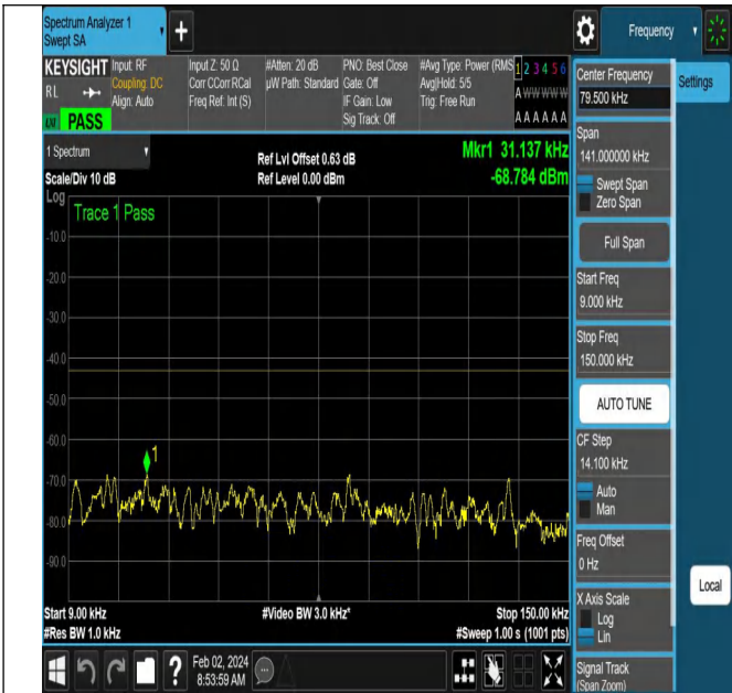
NTNV-N66-PC3-15-20-L-DFT-PI2BPSK-Edge_1RB_Left-Ant1- PASS
