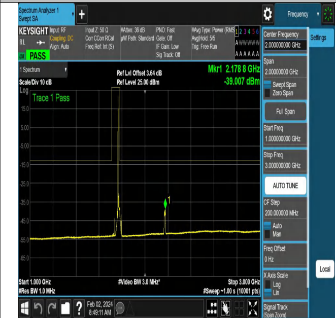
NTNV-N66-PC3-15-15-H-DFT-QPSK-Edge_1RB_Left-Ant1-P
