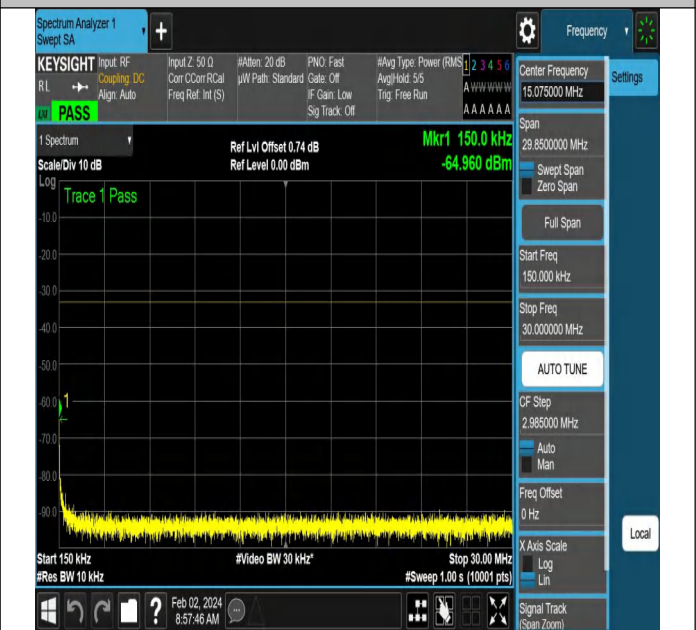
NTNV-N66-PC3-15-20-L-DFT-QPSK-Edge_1RB_Right-Ant1-P
