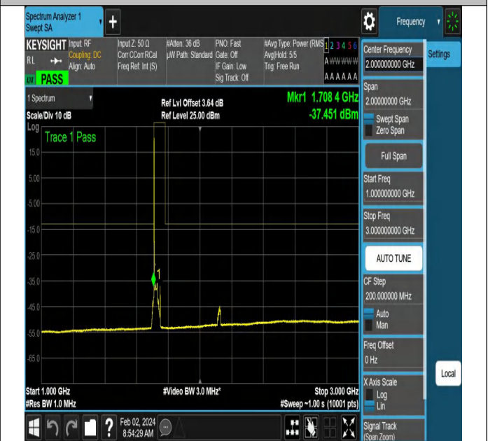
NTNV-N66-PC3-15-20-L-DFT-PI2BPSK-Edge_1RB_Left-Ant1- PASS
