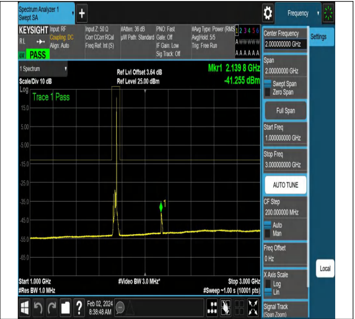
NTNV-N66-PC3-15-15-M-DFT-PI2BPSK-Edge_1RB_Right-An t1-PASS
