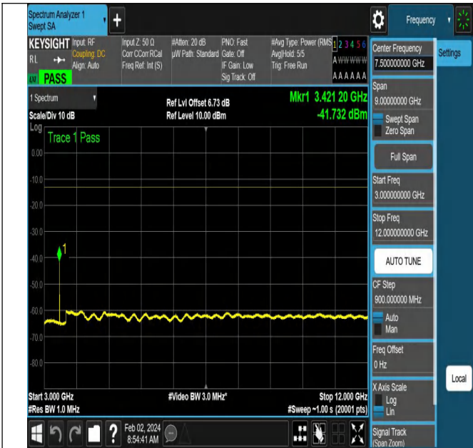
NTNV-N66-PC3-15-20-L-DFT-PI2BPSK-Edge_1RB_Left-Ant1-
