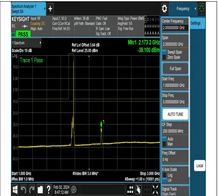
NTNV-N66-PC3-15-15-H-DFT-PI2BPSK-Edge_1RB_Right-Ant 1-PASS
