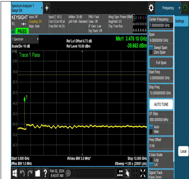
NTNV-N66-PC3-15-15-M-DFT-QPSK-Edge_1RB_Left-Ant1-P
