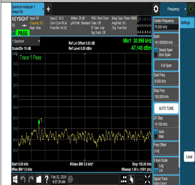
NTNV-N66-PC3-15-20-L-DFT-QPSK-Edge_1RB_Right-Ant1-P
