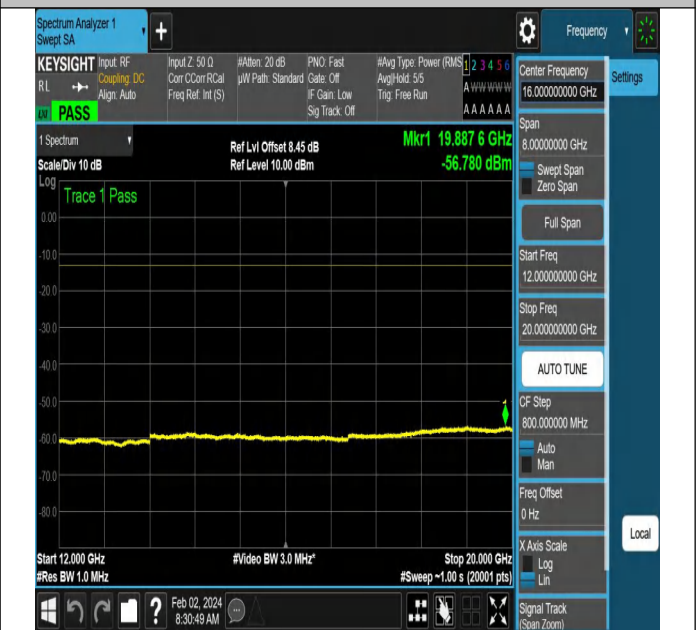
NTNV-N66-PC3-15-15-L-DFT-PI2BPSK-Edge_1RB_Right-Ant 1-PASS
