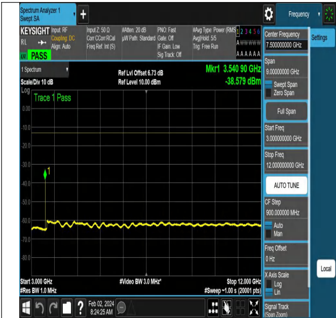
NTNV-N66-PC3-15-10-H-DFT-QPSK-Edge_1RB_Left-Ant1-P
