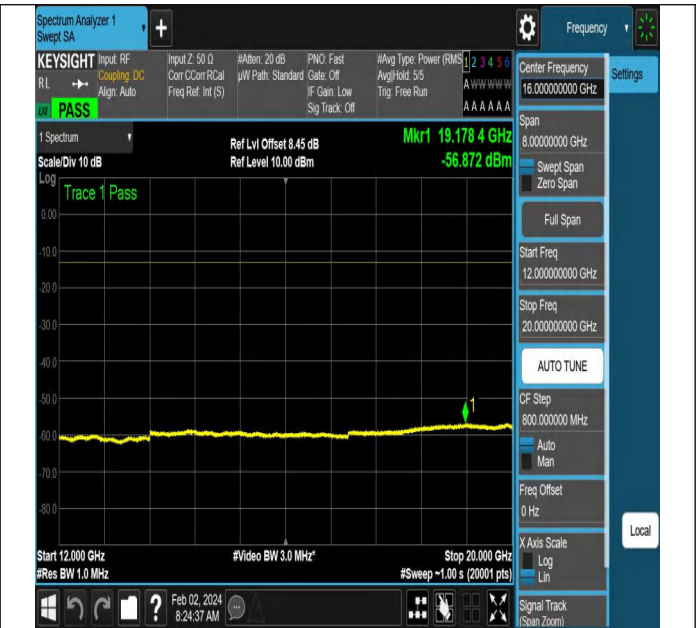
NTNV-N66-PC3-15-10-H-DFT-QPSK-Edge_1RB_Left-Ant1-P
