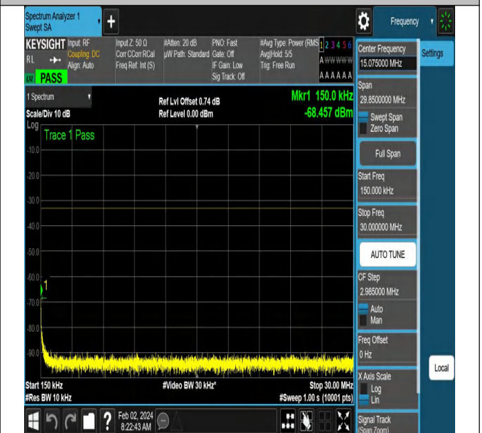
NTNV-N66-PC3-15-10-H-DFT-PI2BPSK-Edge_1RB_Right-Ant
