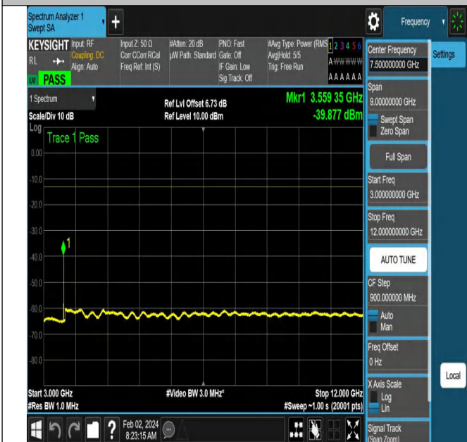
NTNV-N66-PC3-15-10-H-DFT-PI2BPSK-Edge_1RB_Right-Ant 1-PASS
