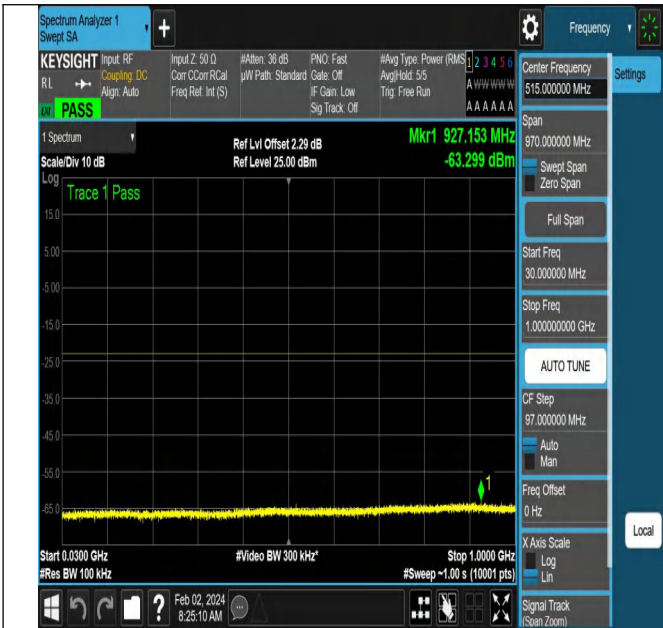
NTNV-N66-PC3-15-10-H-DFT-QPSK-Edge_1RB_Right-Ant1-
