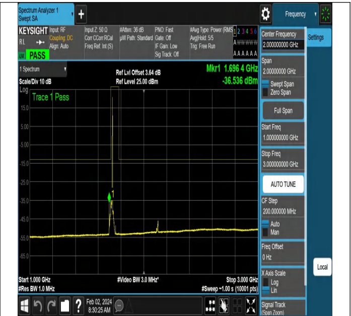
NTNV-N66-PC3-15-15-L-DFT-PI2BPSK-Edge_1RB_Right-Ant 1-PASS
