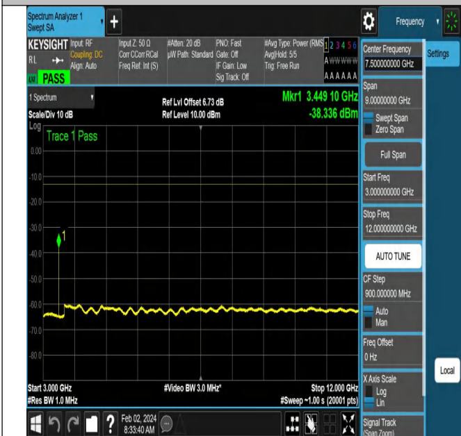
NTNV-N66-PC3-15-15-L-DFT-QPSK-Edge_1RB_Right-Ant1-P
