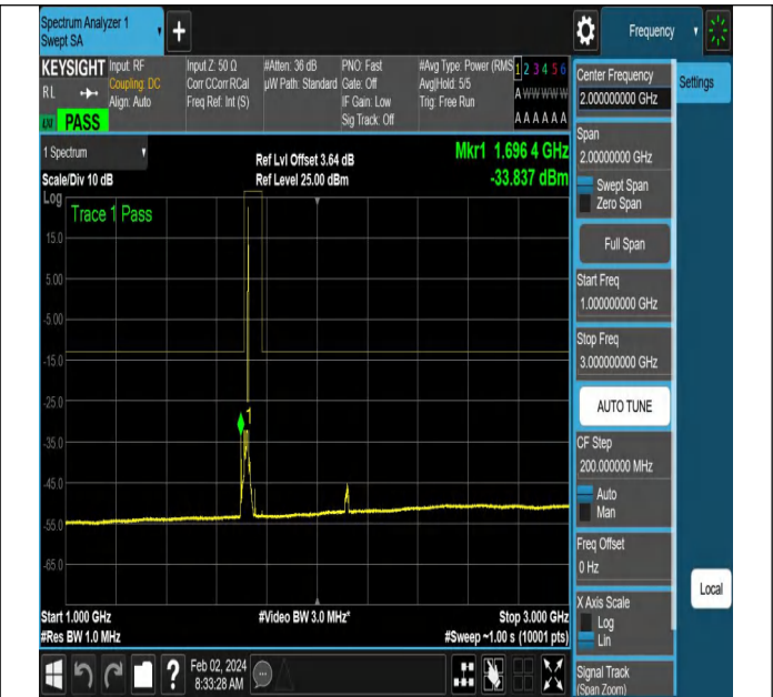
NTNV-N66-PC3-15-15-L-DFT-QPSK-Edge_1RB_Right-Ant1-P
