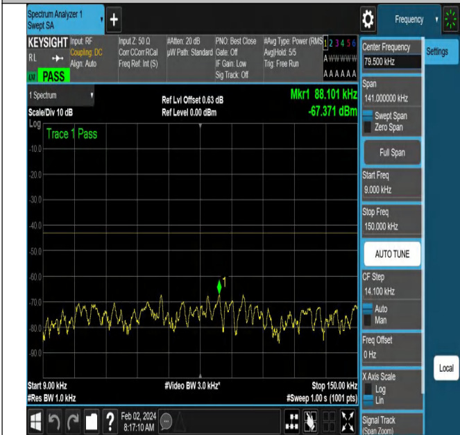
NTNV-N66-PC3-15-10-M-DFT-QPSK-Edge_1RB_Right-Ant1-P
