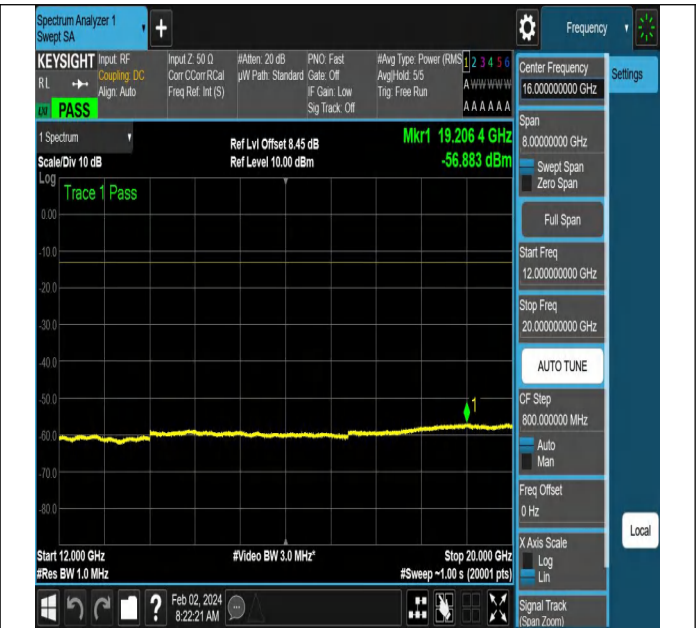
NTNV-N66-PC3-15-10-H-DFT-PI2BPSK-Edge_1RB_Left-Ant1
