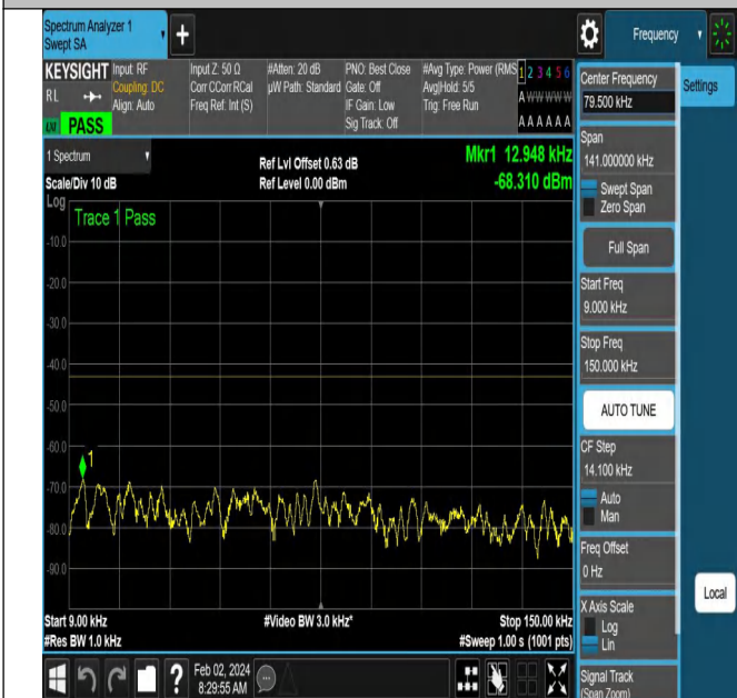
NTNV-N66-PC3-15-15-L-DFT-PI2BPSK-Edge_1RB_Right-Ant
