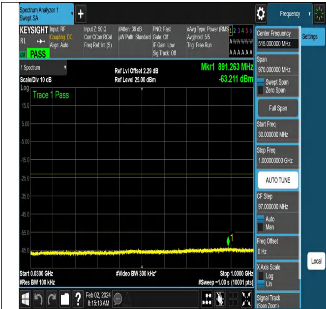
NTNV-N66-PC3-15-10-M-DFT-PI2BPSK-Edge_1RB_Right-An t1-PASS
