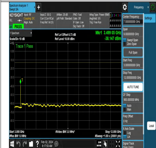
NTNV-N66-PC3-15-10-M-DFT-QPSK-Edge_1RB_Right-Ant1-
