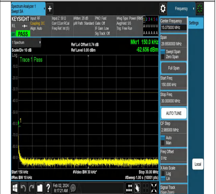
NTNV-N66-PC3-15-10-M-DFT-QPSK-Edge_1RB_Right-Ant1-P
