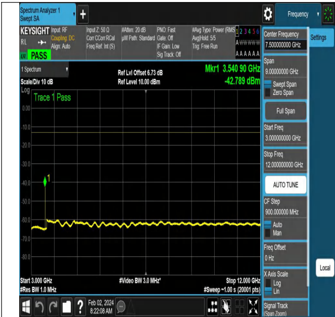
NTNV-N66-PC3-15-10-H-DFT-PI2BPSK-Edge_1RB_Left-Ant1
