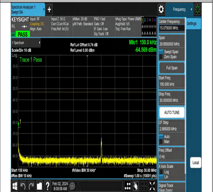
NTNV-N66-PC3-15-10-L-DFT-QPSK-Edge_1RB_Right-Ant1-P
