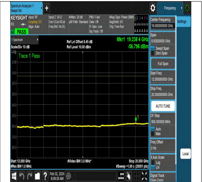
NTNV-N66-PC3-15-10-L-DFT-QPSK-Edge_1RB_Left-Ant1-PA
