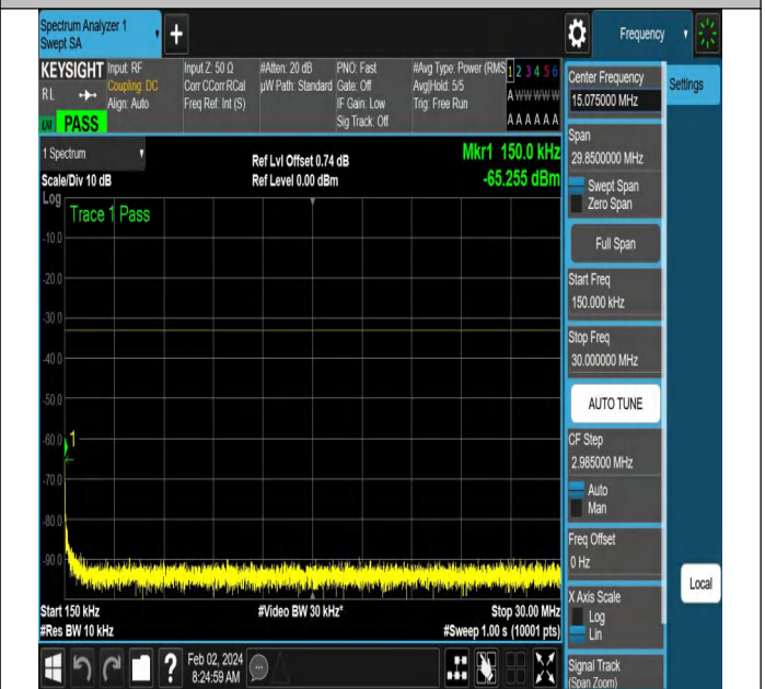
NTNV-N66-PC3-15-10-H-DFT-QPSK-Edge_1RB_Right-Ant1-
