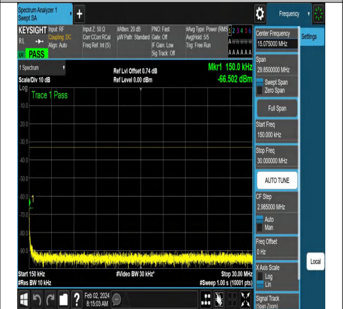
NTNV-N66-PC3-15-10-M-DFT-PI2BPSK-Edge_1RB_Right-An t1-PASS
