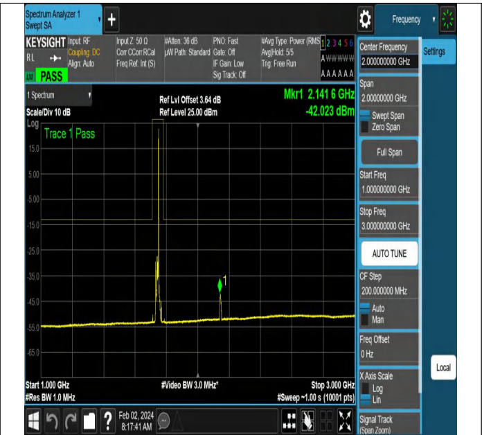
NTNV-N66-PC3-15-10-M-DFT-QPSK-Edge_1RB_Right-Ant1-
