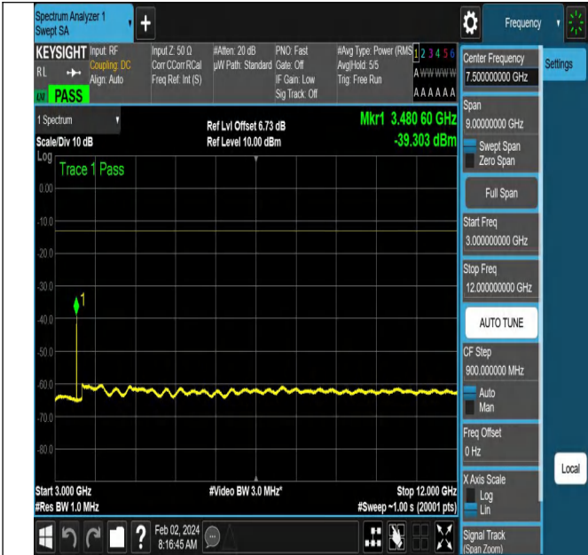
NTNV-N66-PC3-15-10-M-DFT-QPSK-Edge_1RB_Left-Ant1-P
