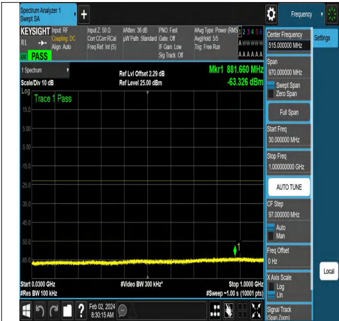
NTNV-N66-PC3-15-15-L-DFT-PI2BPSK-Edge_1RB_Right-Ant 1-PASS
