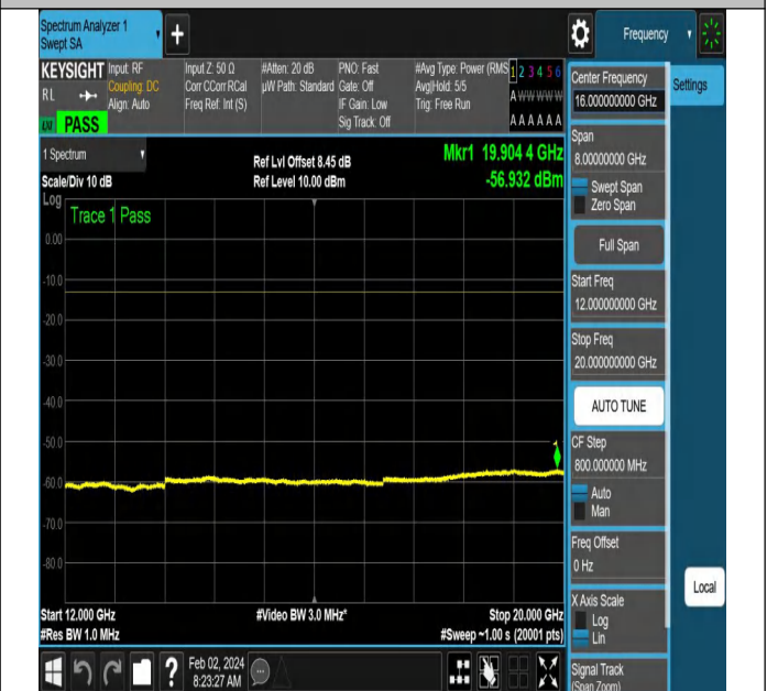
NTNV-N66-PC3-15-10-H-DFT-PI2BPSK-Edge_1RB_Right-Ant 1-PASS
