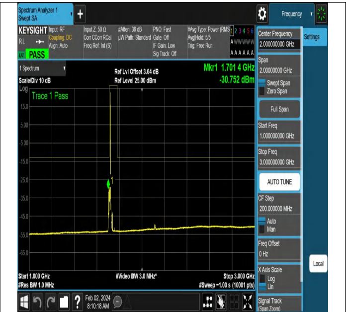
NTNV-N66-PC3-15-10-L-DFT-QPSK-Edge_1RB_Right-Ant1-P
