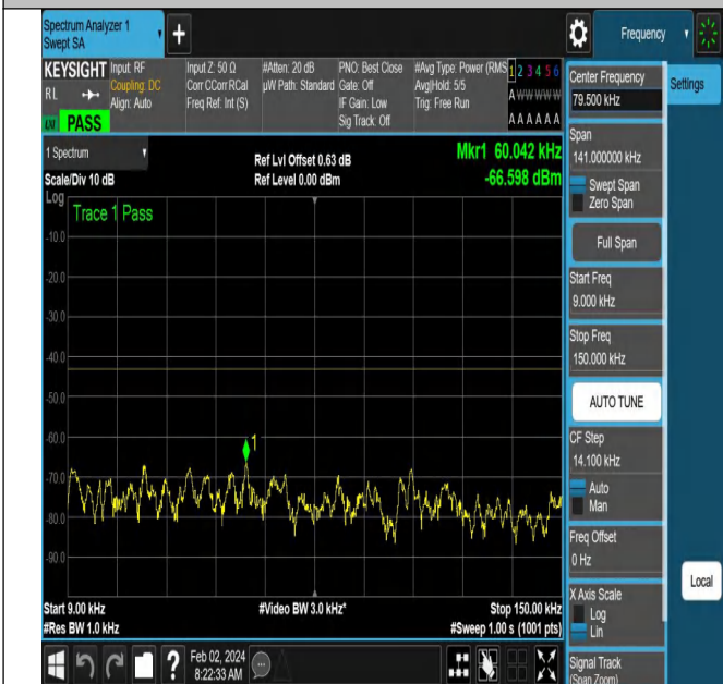
NTNV-N66-PC3-15-10-H-DFT-PI2BPSK-Edge_1RB_Right-Ant
