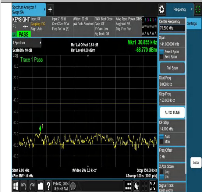
NTNV-N66-PC3-15-10-H-DFT-QPSK-Edge_1RB_Right-Ant1-
