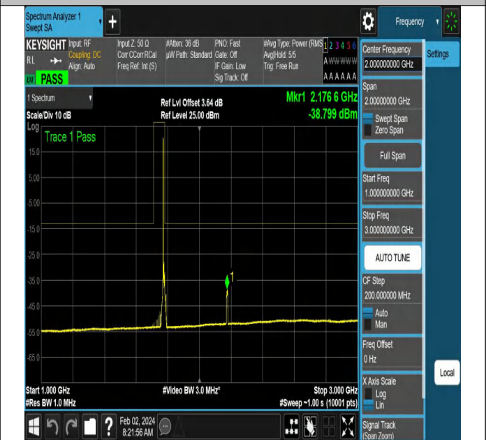
NTNV-N66-PC3-15-10-H-DFT-PI2BPSK-Edge_1RB_Left-Ant1
