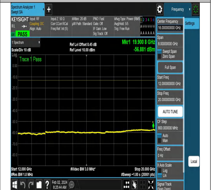
NTNV-N66-PC3-15-10-H-DFT-QPSK-Edge_1RB_Right-Ant1-
