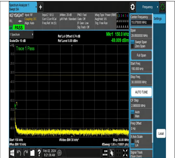
NTNV-N66-PC3-15-10-H-DFT-PI2BPSK-Edge_1RB_Left-Ant1
