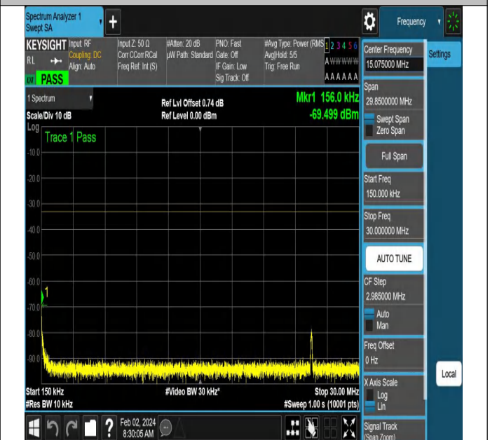
NTNV-N66-PC3-15-15-L-DFT-PI2BPSK-Edge_1RB_Right-Ant
