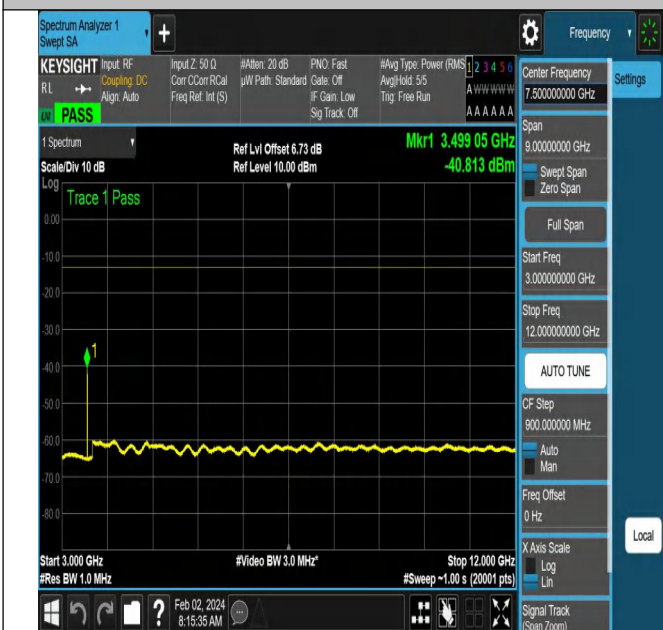
NTNV-N66-PC3-15-10-M-DFT-PI2BPSK-Edge_1RB_Right-An t1-PASS
