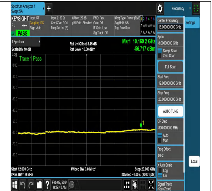
NTNV-N66-PC3-15-15-L-DFT-PI2BPSK-Edge_1RB_Left-Ant1-
