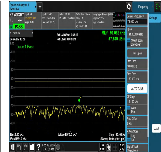
NTNV-N66-PC3-15-5-L-DFT-QPSK-Edge_1RB_Left-Ant1-PAS
