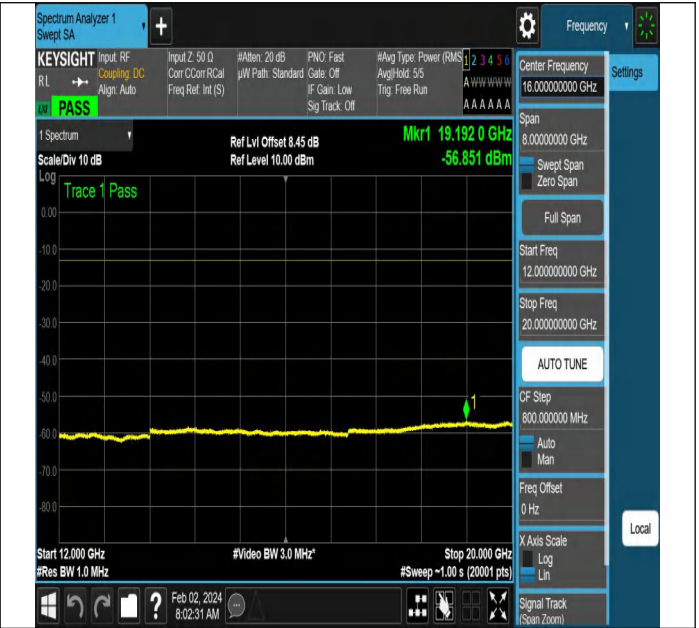
NTNV-N66-PC3-15-5-H-DFT-QPSK-Edge_1RB_Left-Ant1-PA
