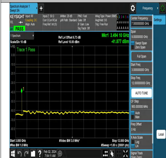
NTNV-N66-PC3-15-5-M-DFT-PI2BPSK-Edge_1RB_Right-Ant 1-PASS
