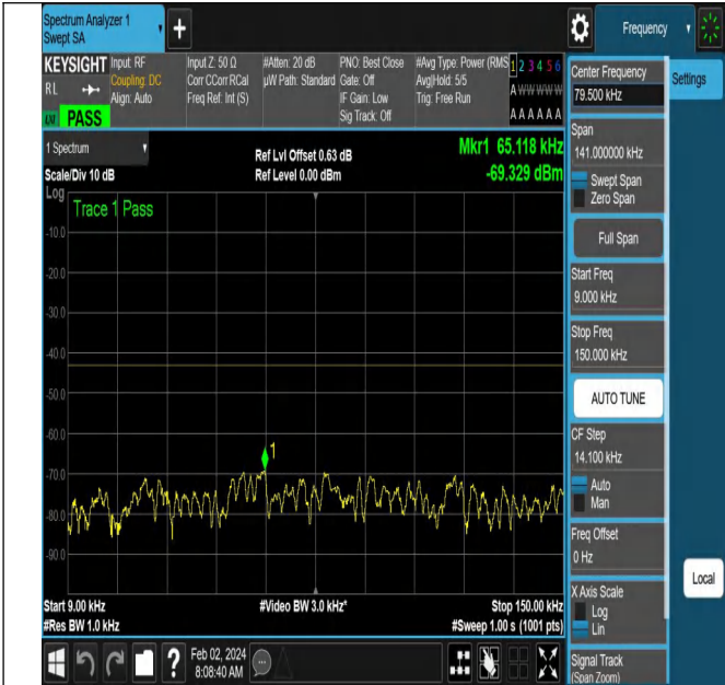
NTNV-N66-PC3-15-10-L-DFT-QPSK-Edge_1RB_Left-Ant1-PA
