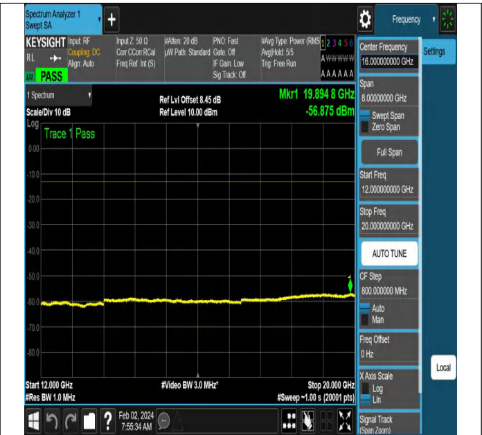
NTNV-N66-PC3-15-5-M-DFT-QPSK-Edge_1RB_Left-Ant1-PA SS
