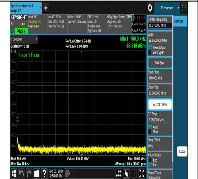
NTNV-N66-PC3-15-5-M-DFT-QPSK-Edge_1RB_Right-Ant1-P ASS
