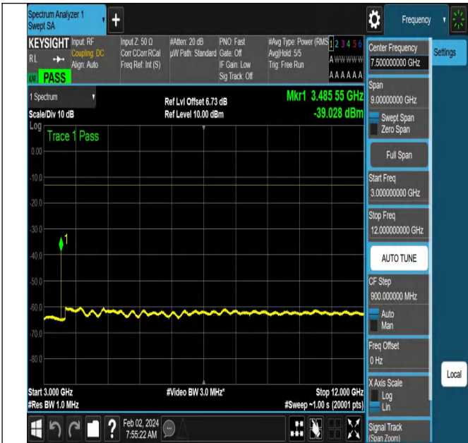
NTNV-N66-PC3-15-5-M-DFT-QPSK-Edge_1RB_Left-Ant1-PA SS
