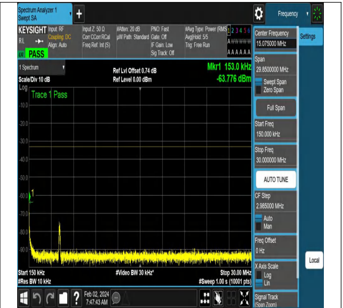
NTNV-N66-PC3-15-5-L-DFT-QPSK-Edge_1RB_Left-Ant1-PAS
