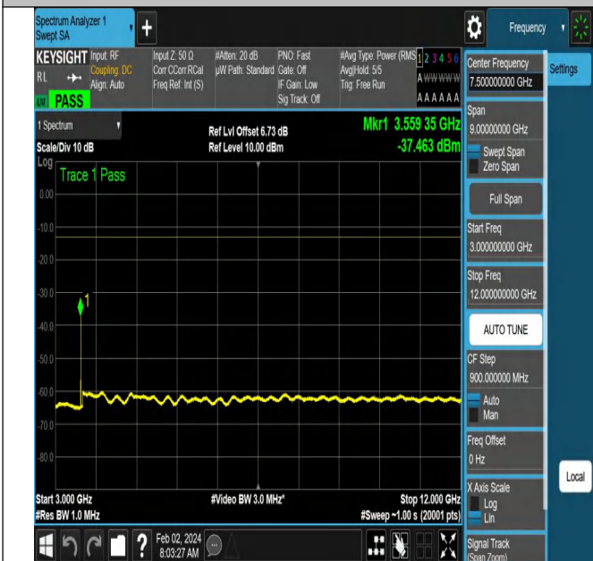
NTNV-N66-PC3-15-5-H-DFT-QPSK-Edge_1RB_Right-Ant1-P
