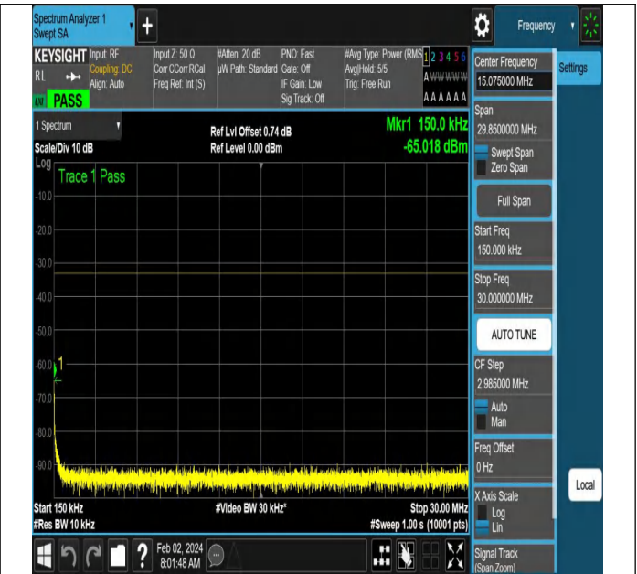
NTNV-N66-PC3-15-5-H-DFT-QPSK-Edge_1RB_Left-Ant1-PA
