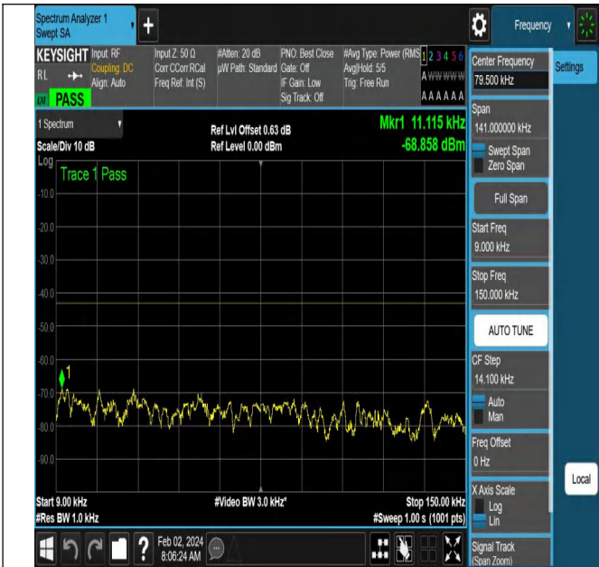
NTNV-N66-PC3-15-10-L-DFT-PI2BPSK-Edge_1RB_Left-Ant1- PASS
