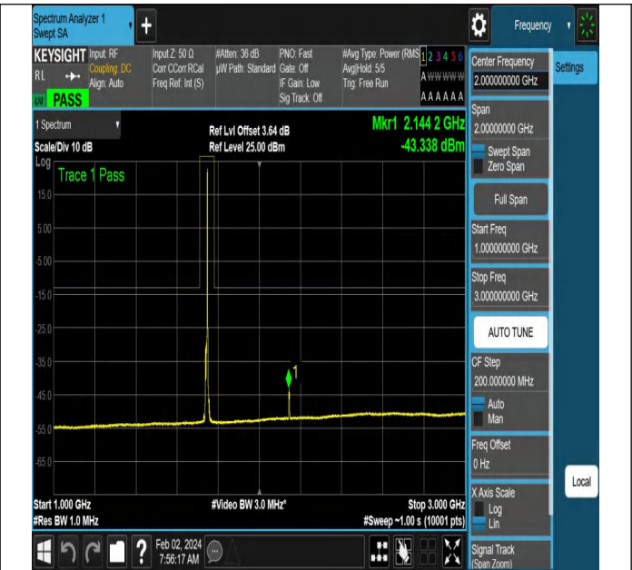
NTNV-N66-PC3-15-5-M-DFT-QPSK-Edge_1RB_Right-Ant1-P
