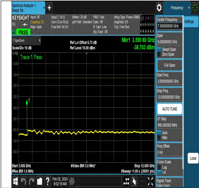
NTNV-N66-PC3-15-5-H-DFT-QPSK-Edge_1RB_Left-Ant1-PA
