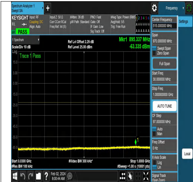
NTNV-N66-PC3-15-5-H-DFT-PI2BPSK-Edge_1RB_Right-Ant1 -PASS
