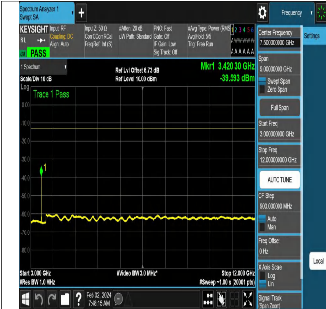
NTNV-N66-PC3-15-5-L-DFT-QPSK-Edge_1RB_Left-Ant1-PAS
