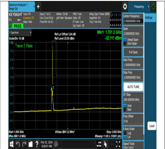
NTNV-N66-PC3-15-10-L-DFT-PI2BPSK-Edge_1RB_Right-Ant 1-PASS
