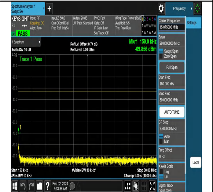
NTNV-N66-PC3-15-5-M-DFT-PI2BPSK-Edge_1RB_Right-Ant 1-PASS
