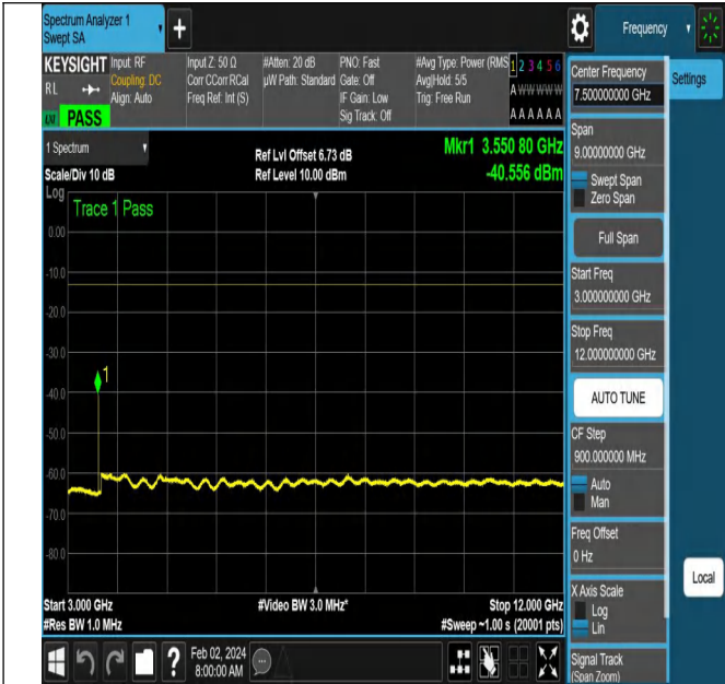
NTNV-N66-PC3-15-5-H-DFT-PI2BPSK-Edge_1RB_Left-Ant1-
