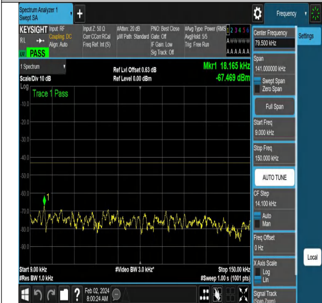
NTNV-N66-PC3-15-5-H-DFT-PI2BPSK-Edge_1RB_Right-Ant1
