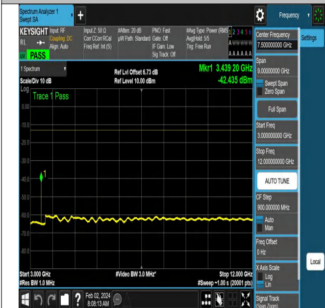
NTNV-N66-PC3-15-10-L-DFT-PI2BPSK-Edge_1RB_Right-Ant 1-PASS
