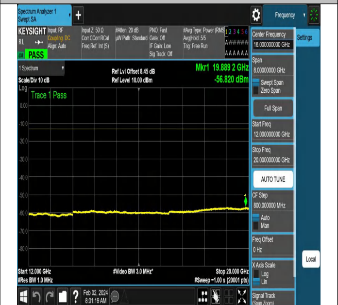
NTNV-N66-PC3-15-5-H-DFT-PI2BPSK-Edge_1RB_Right-Ant1 -PASS
