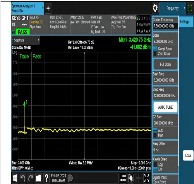
NTNV-N66-PC3-15-10-L-DFT-PI2BPSK-Edge_1RB_Left-Ant1-1 PASS
