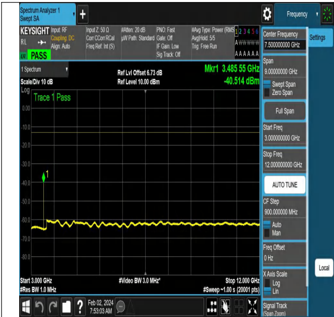
NTNV-N66-PC3-15-5-M-DFT-PI2BPSK-Edge_1RB_Left-Ant1- PASS
