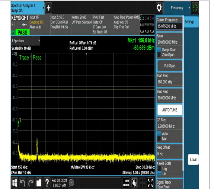
NTNV-N66-PC3-15-10-L-DFT-QPSK-Edge_1RB_Left-Ant1-PA
