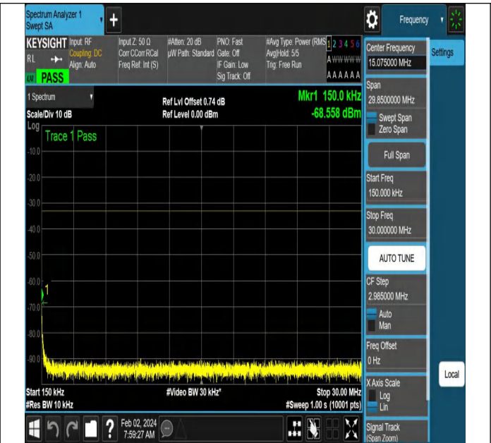
NTNV-N66-PC3-15-5-H-DFT-PI2BPSK-Edge_1RB_Left-Ant1- PASS
