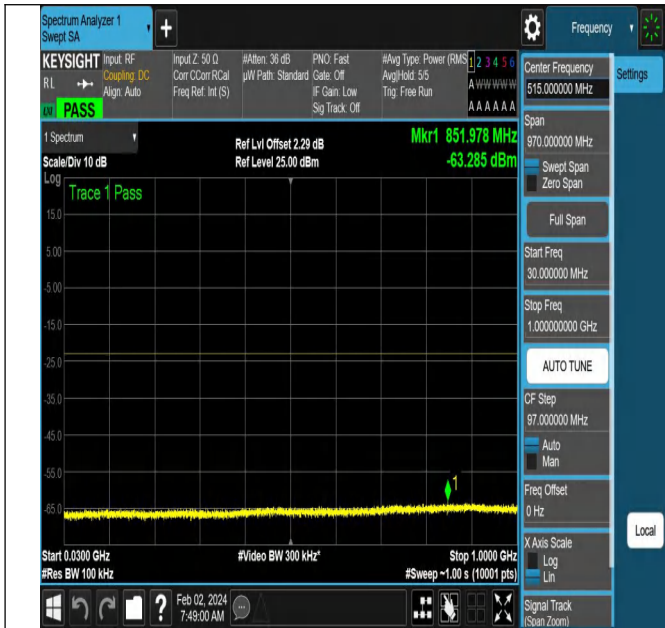
NTNV-N66-PC3-15-5-L-DFT-QPSK-Edge_1RB_Right-Ant1-PA
