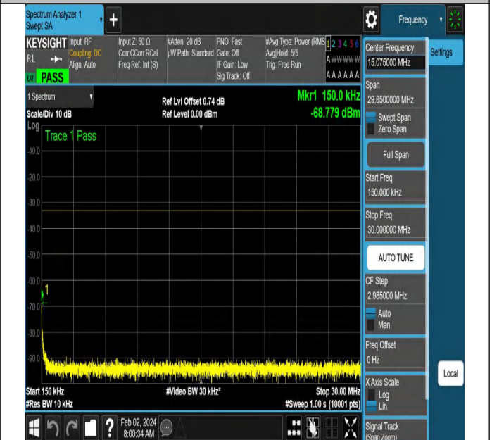
NTNV-N66-PC3-15-5-H-DFT-PI2BPSK-Edge_1RB_Right-Ant1
