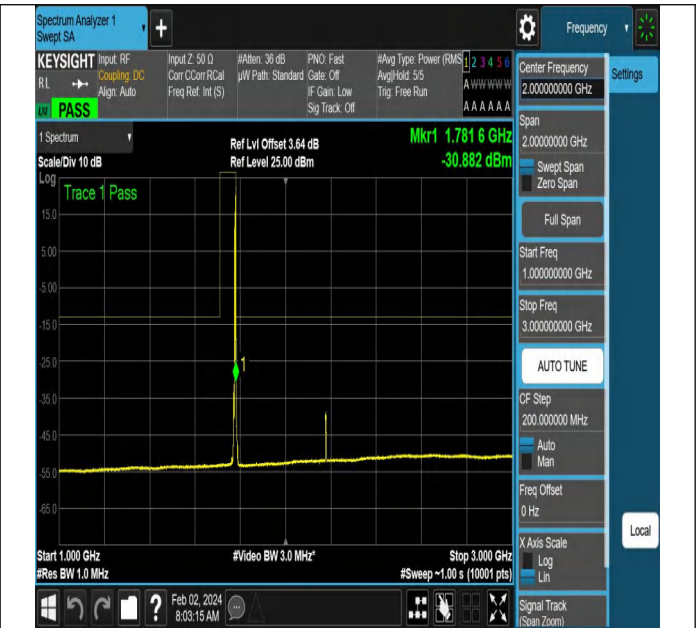
NTNV-N66-PC3-15-5-H-DFT-QPSK-Edge_1RB_Right-Ant1-P
