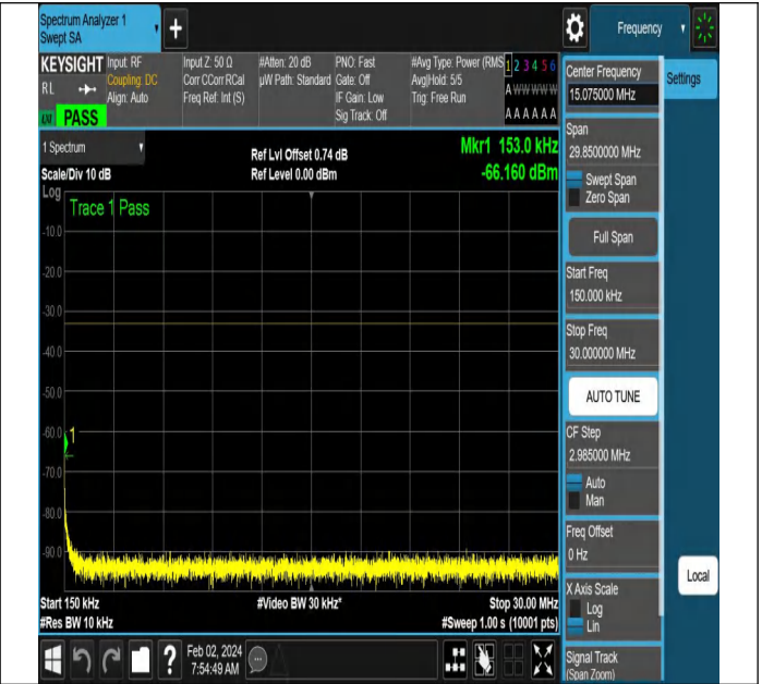
NTNV-N66-PC3-15-5-M-DFT-QPSK-Edge_1RB_Left-Ant1-PA SS
