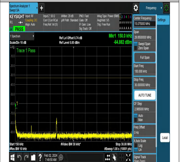
NTNV-N66-PC3-15-5-L-DFT-QPSK-Edge_1RB_Right-Ant1-PA
