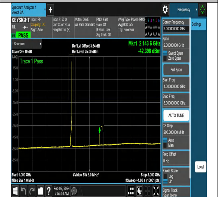
NTNV-N66-PC3-15-5-M-DFT-PI2BPSK-Edge_1RB_Left-Ant1- PASS
