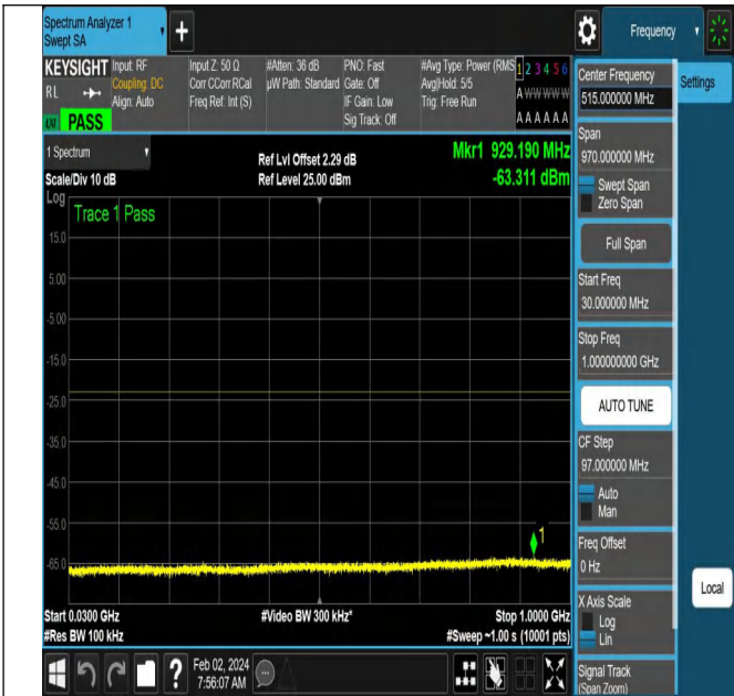
NTNV-N66-PC3-15-5-M-DFT-QPSK-Edge_1RB_Right-Ant1-P
