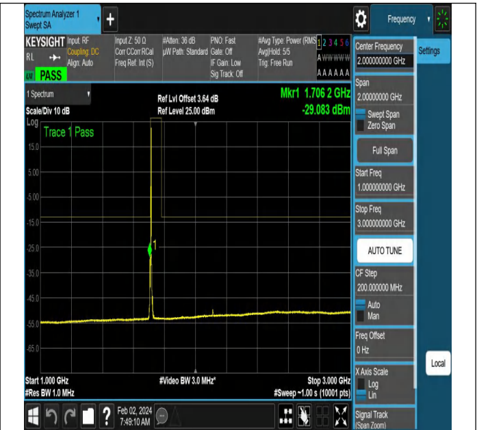
NTNV-N66-PC3-15-5-L-DFT-QPSK-Edge_1RB_Right-Ant1-PA
