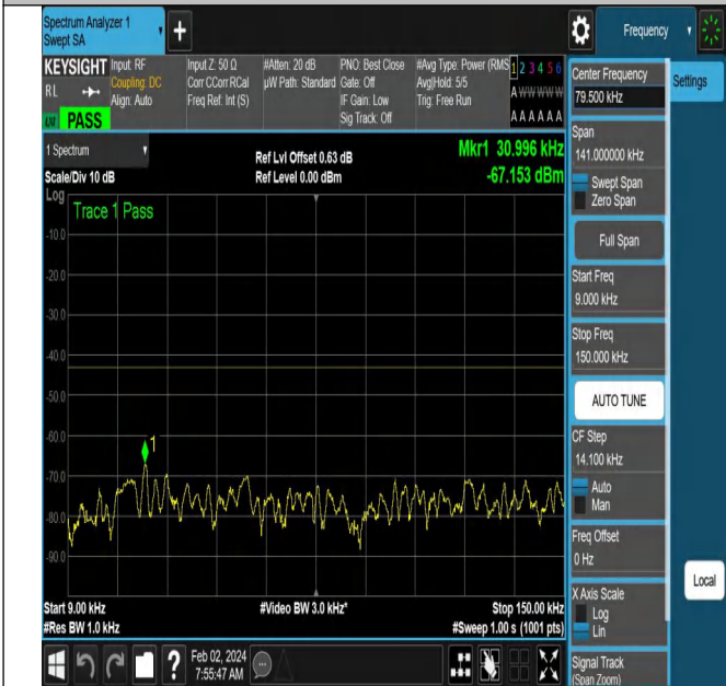
NTNV-N66-PC3-15-5-M-DFT-QPSK-Edge_1RB_Right-Ant1-P ASS
