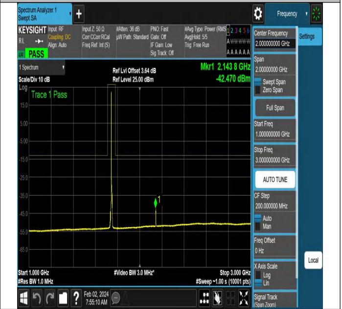
NTNV-N66-PC3-15-5-M-DFT-QPSK-Edge_1RB_Left-Ant1-PA SS
