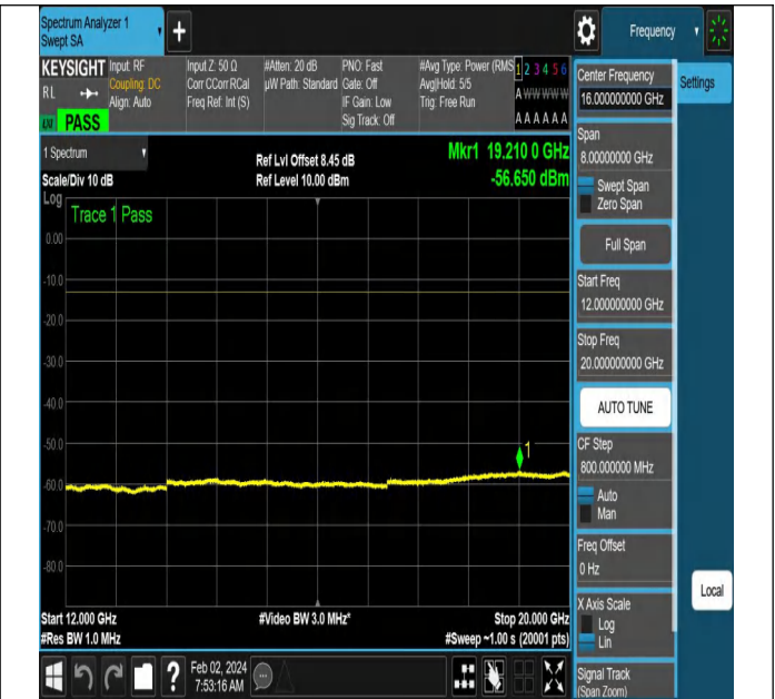
NTNV-N66-PC3-15-5-M-DFT-PI2BPSK-Edge_1RB_Left-Ant1- PASS
